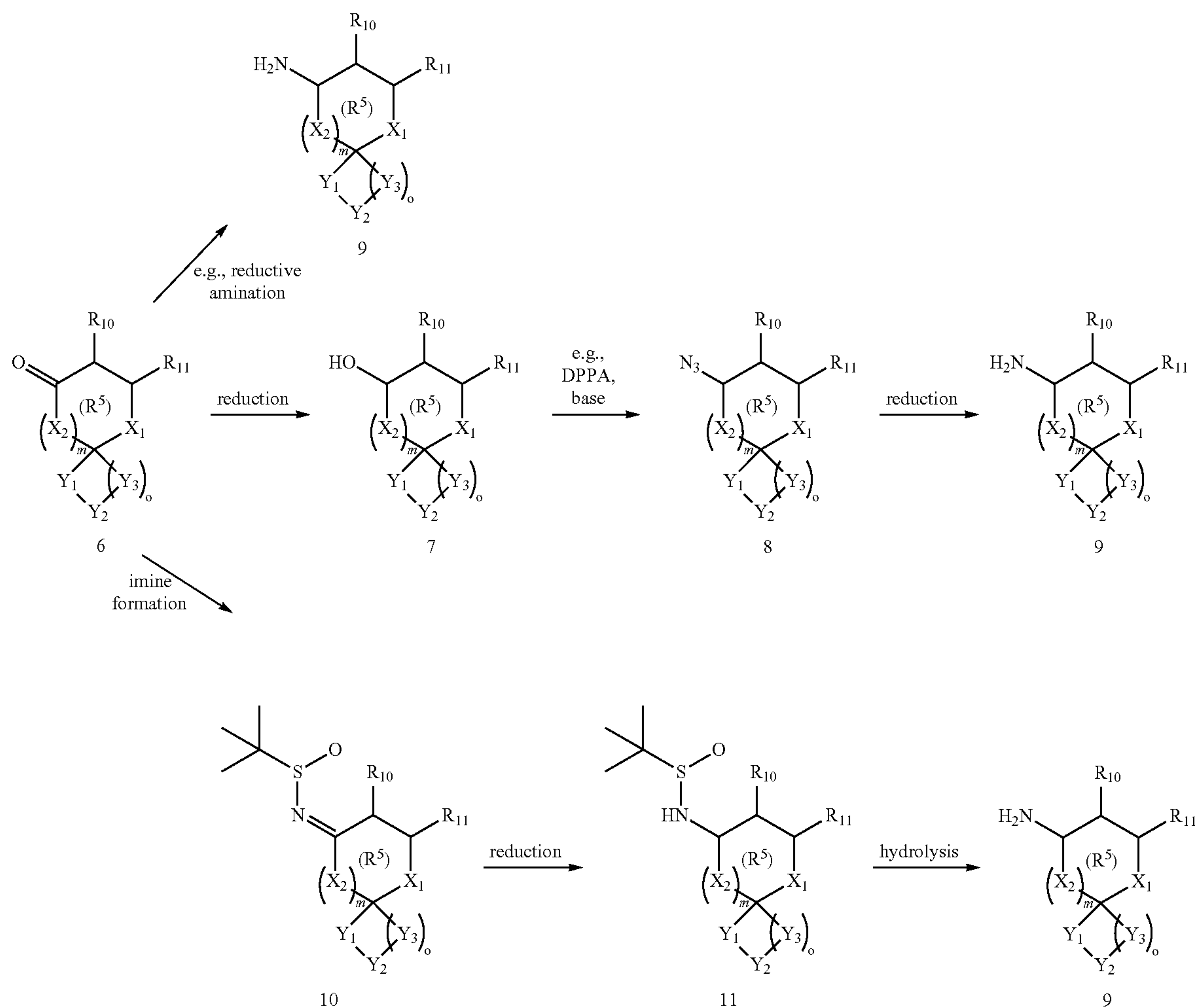
Scheme 3
