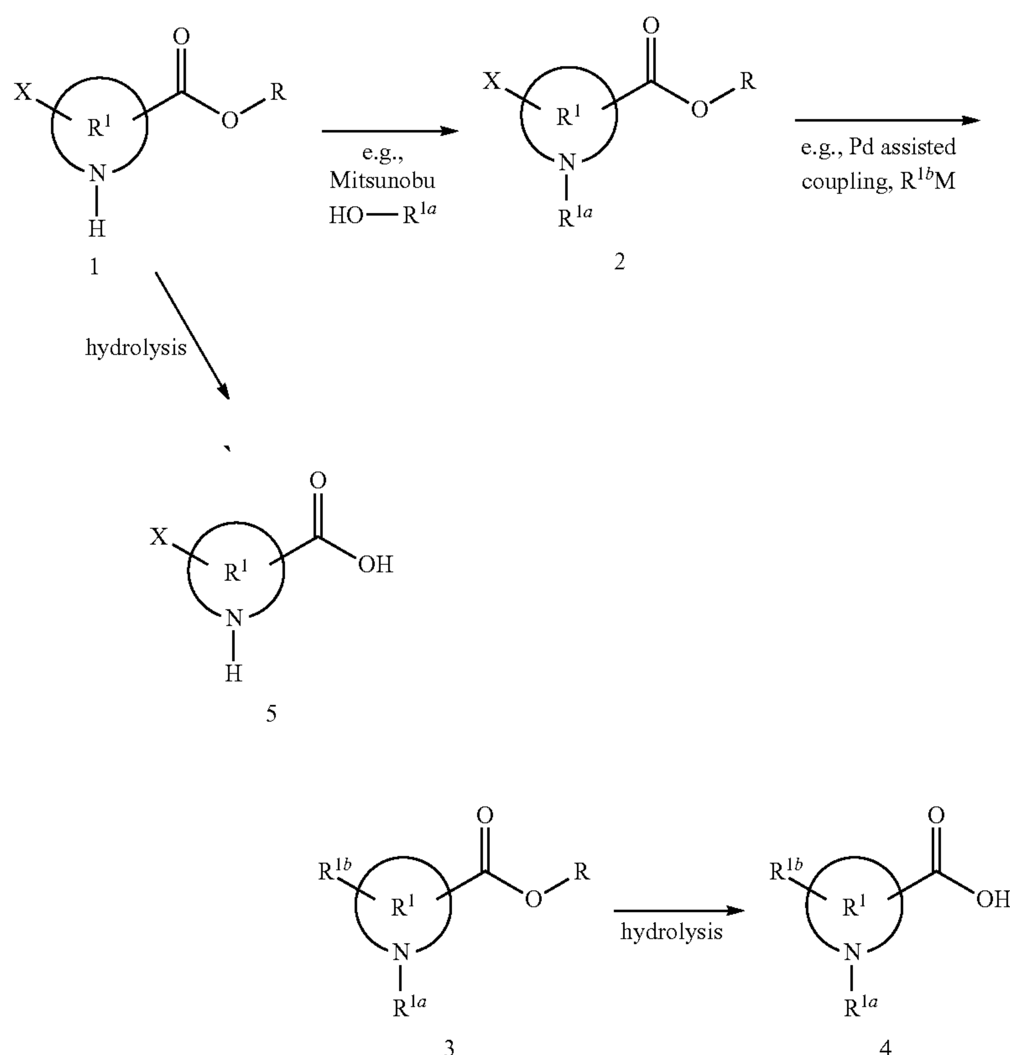
Scheme 1
