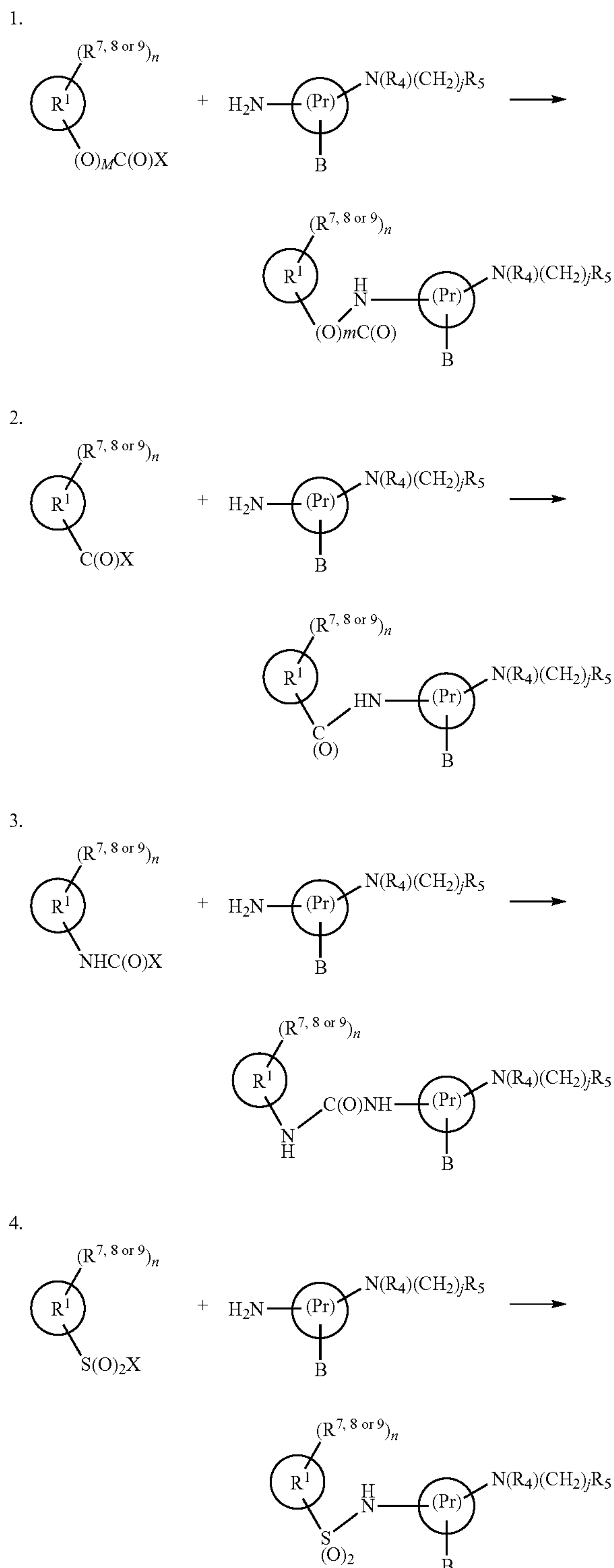
Scheme 2
