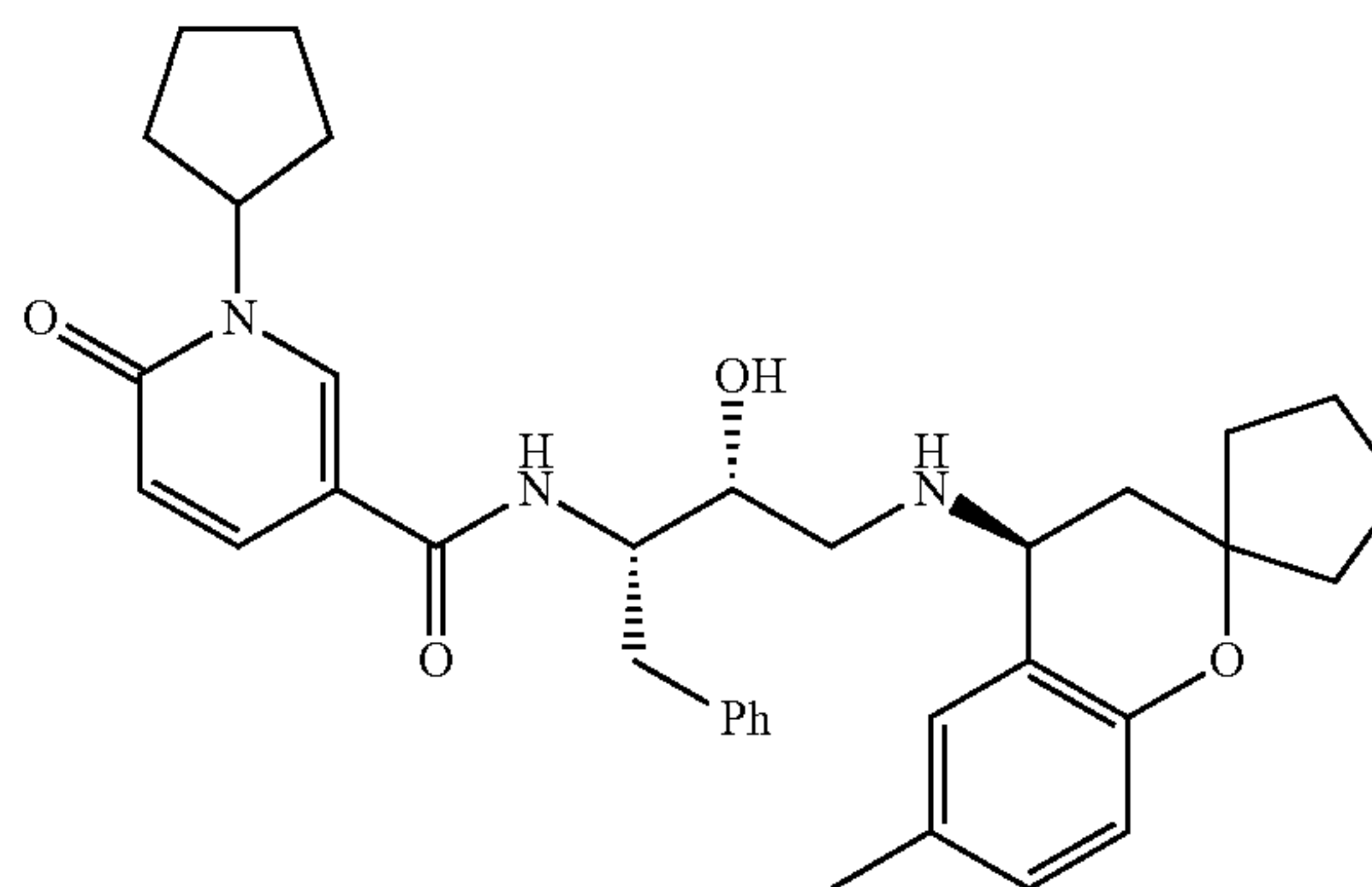
1-cyclopentyl-N-((2S,3R)-4-((S)-2,2-spirocyclopentyl-6-methylchroman-4-ylamino)-3-hydroxy-1-phenylbutan-2-yl)-6-oxo-1,6-dihydropyridine-3-carboxamide (MS m/z: 570 (100%, M+1))
