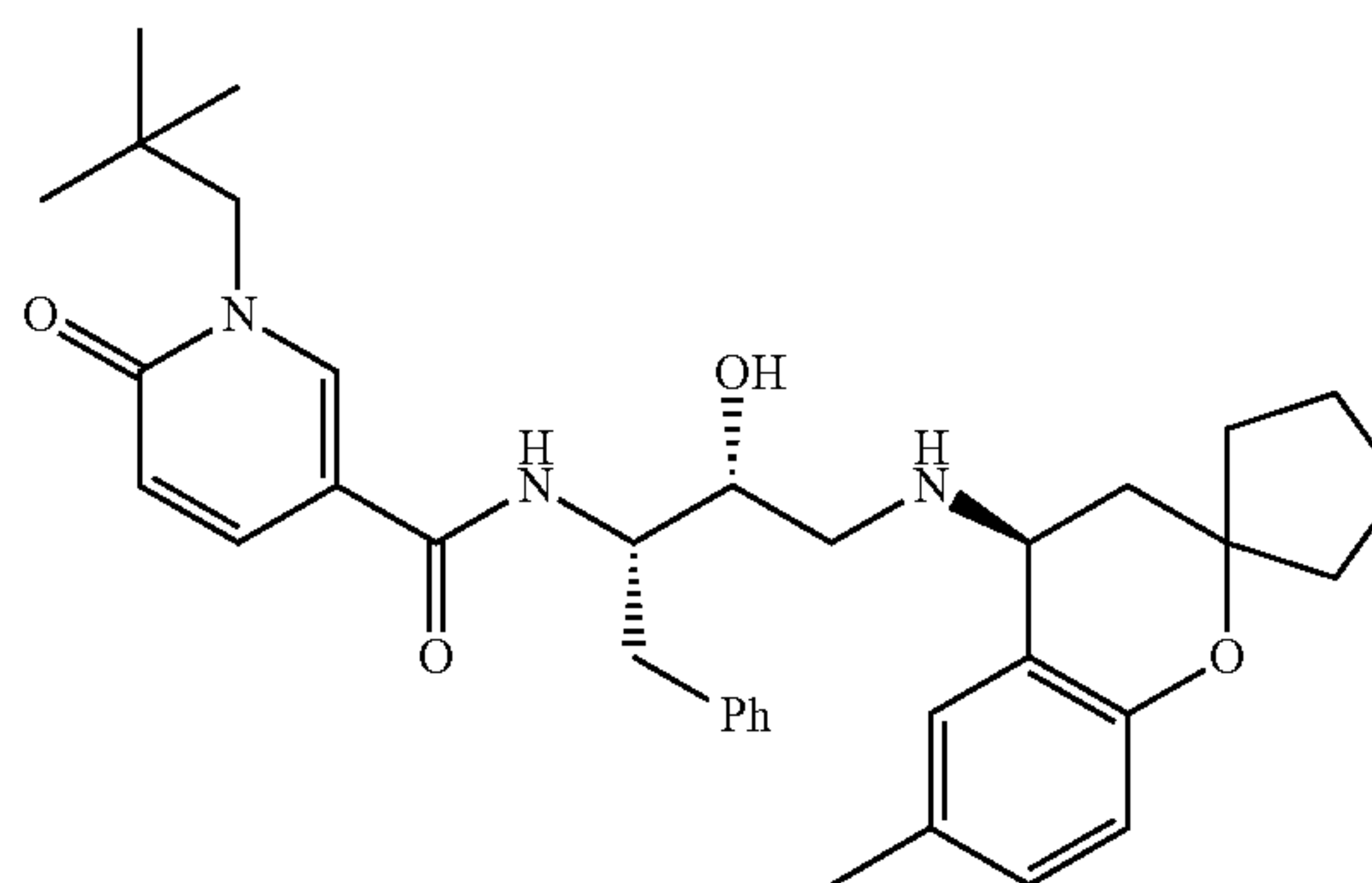
N-((2S,3R)-4-((S)-2,2-spirocyclopentyl-6-methylchroman-4-ylamino)-3-hydroxy-1-phenylbutan-2-yl)-1-neopentyl-6-oxo-1,6-dihydropyridine-3-carboxamide (MS m/z: 572 (100%, M+1))
