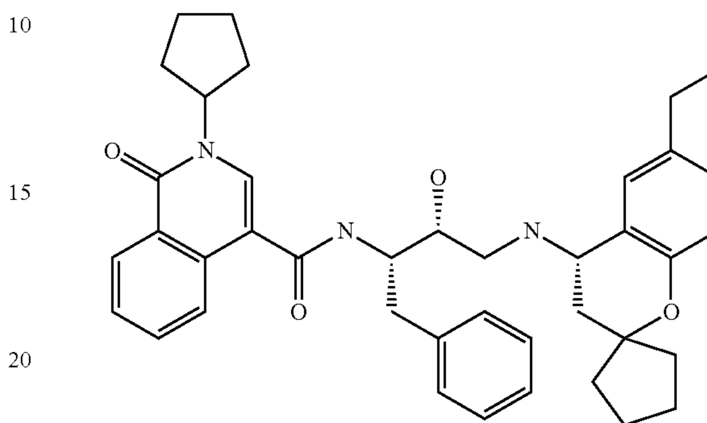
2-cyclopentyl-N-((2S,3R)-4-((S)-6-ethyl-2,2-spirocyclopentylchroman-4-ylamino)-3-hydroxy-1-phenylbutan-2-yl)-1-oxo-1,2-dihydroisoquinoline-4-carboxamide
