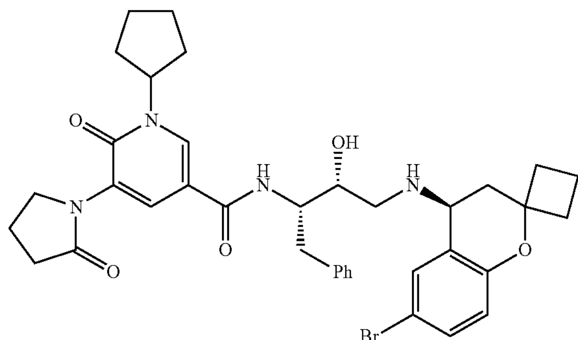
N-((2S,3R)-4-((S)-6-bromo-2,2-spirocyclobutylchroman-4-ylamino)-3-hydroxy-1-phenylbutan-2-yl)-1-cyclopentyl-6-oxo-5-(2-oxopyrrolidin-1-yl)-1,6-dihydropyridine-3-carboxamide
