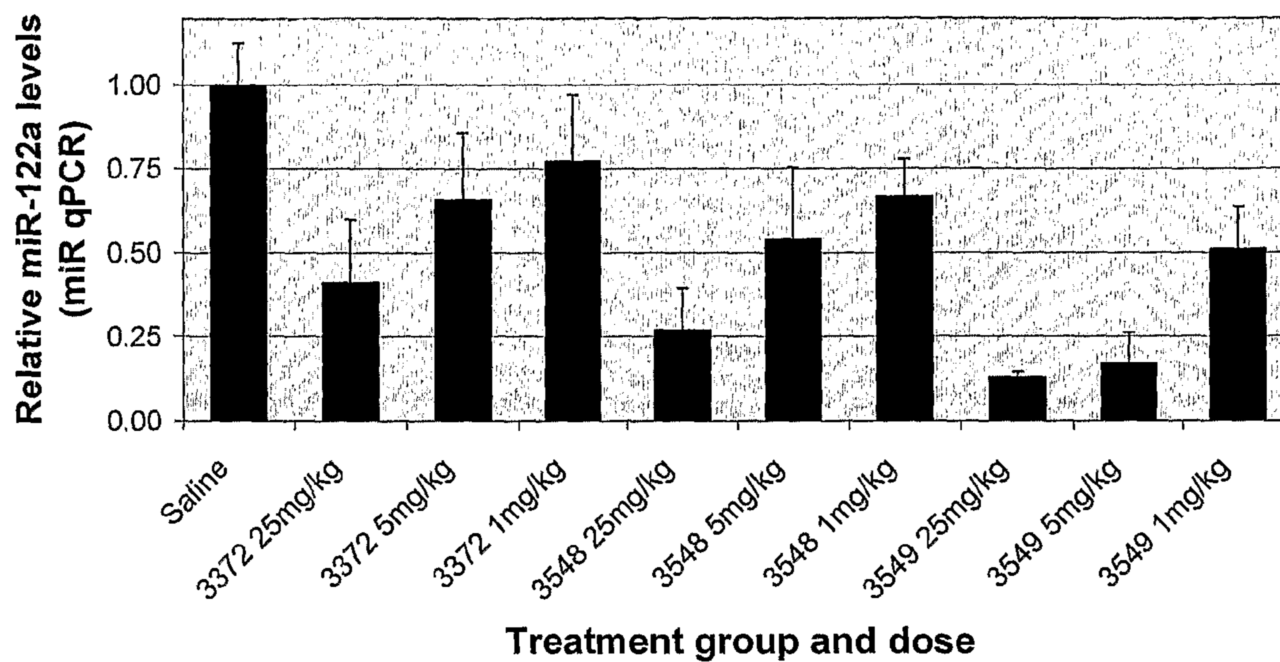
miR-122a levels in mice livers after treatment with different LNA-antimiRs
