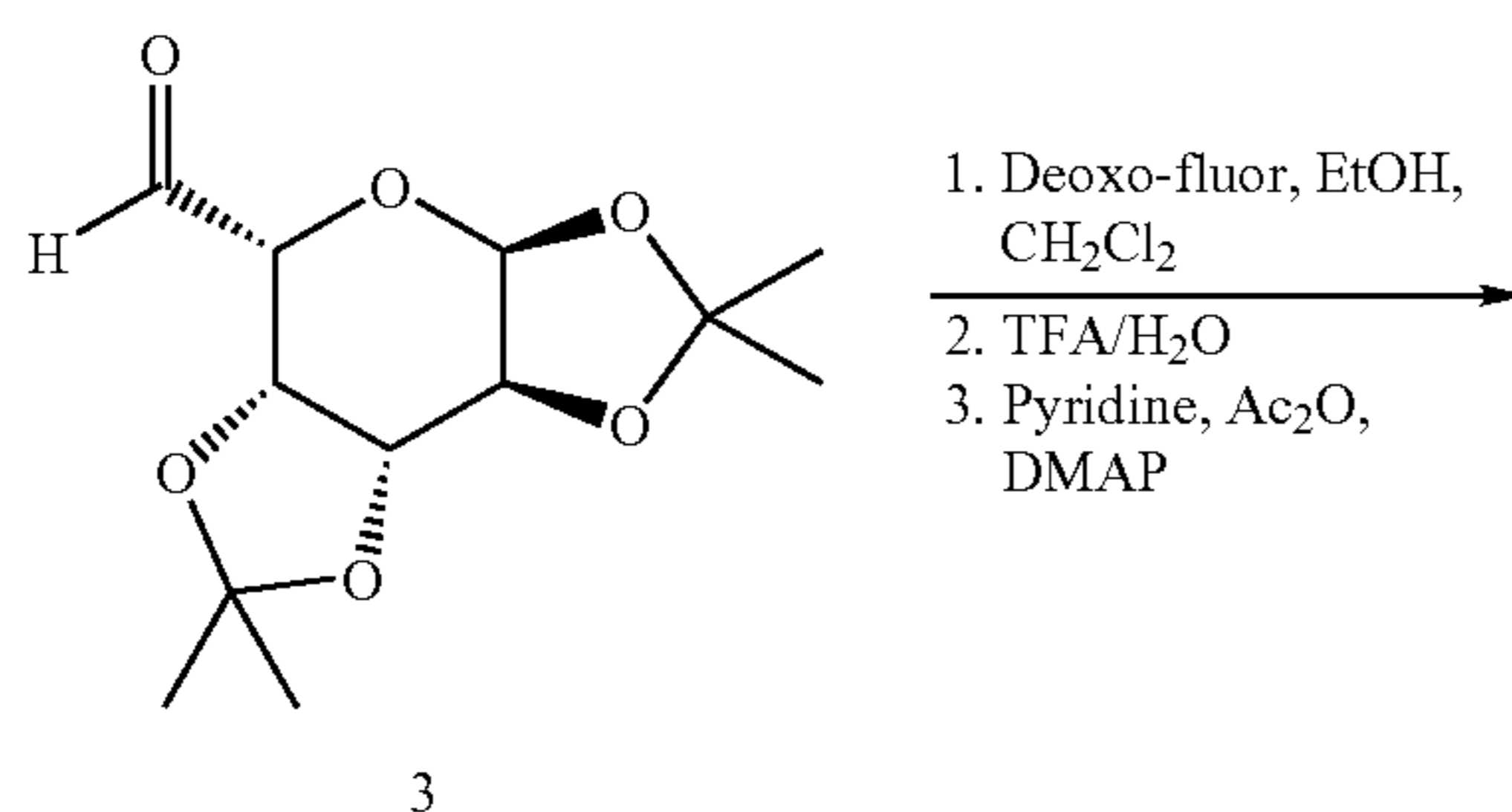
Scheme 15
