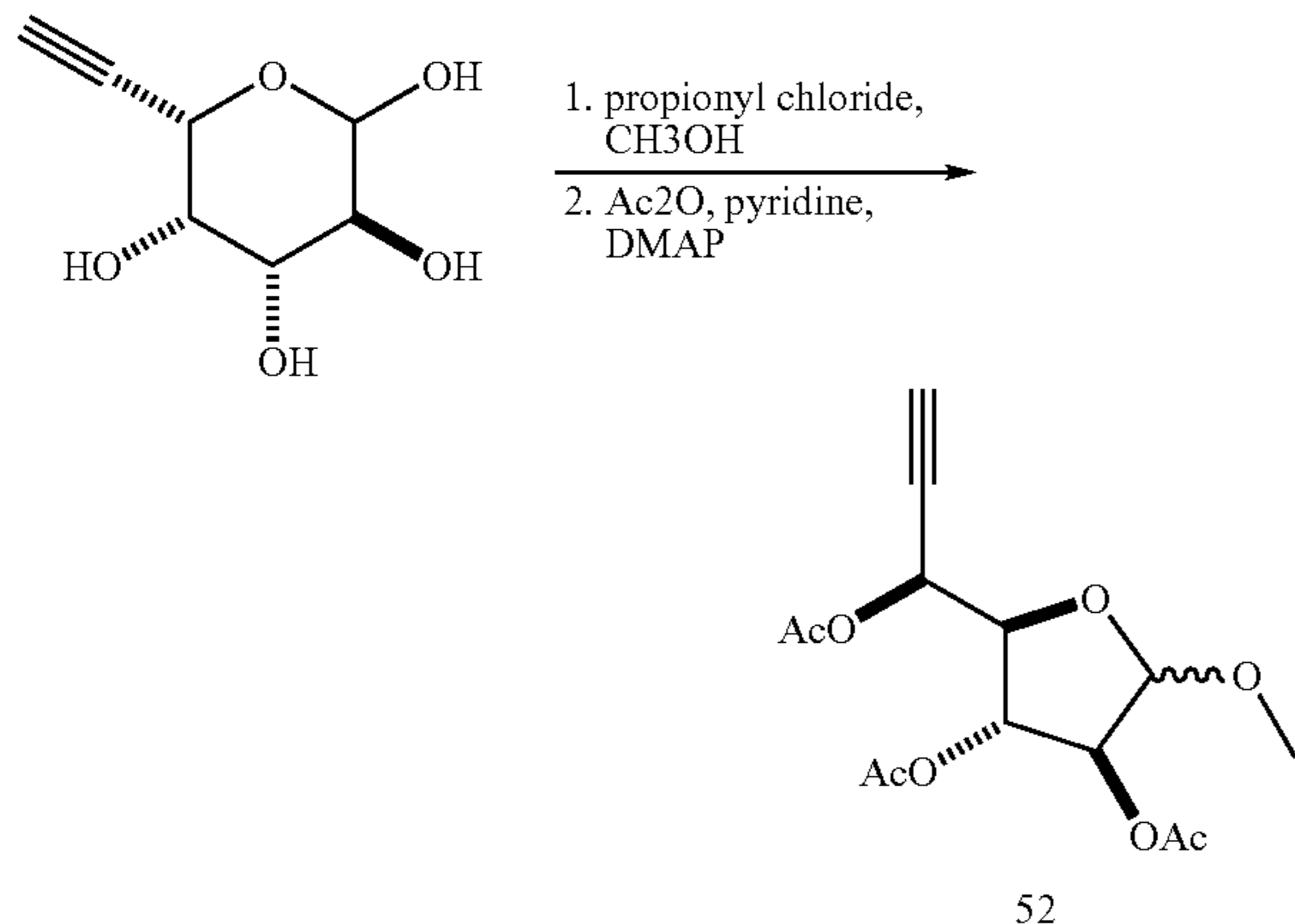
Scheme 14
