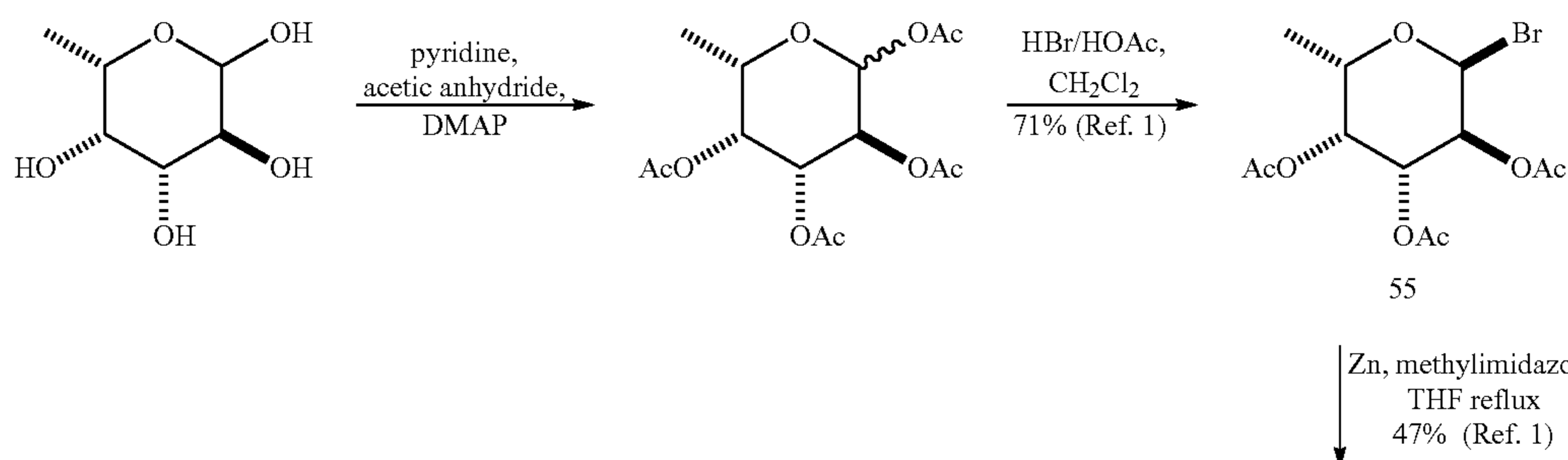
Scheme 16
