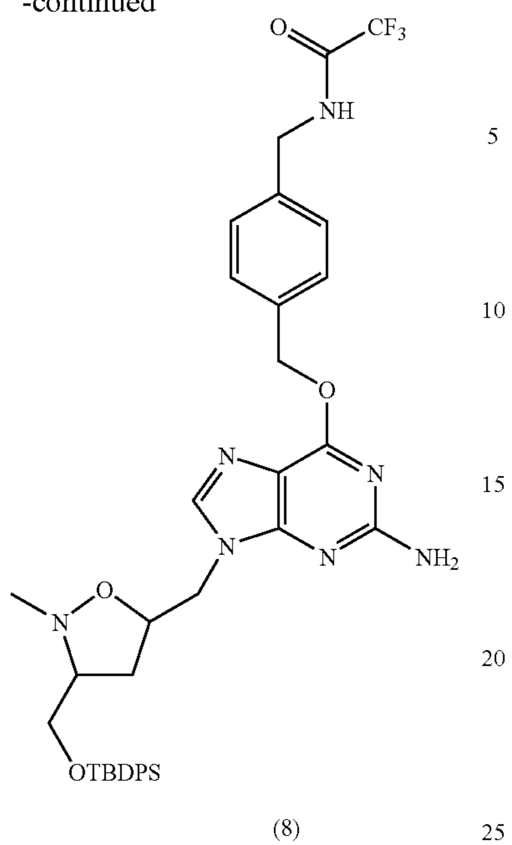
Scheme 5
