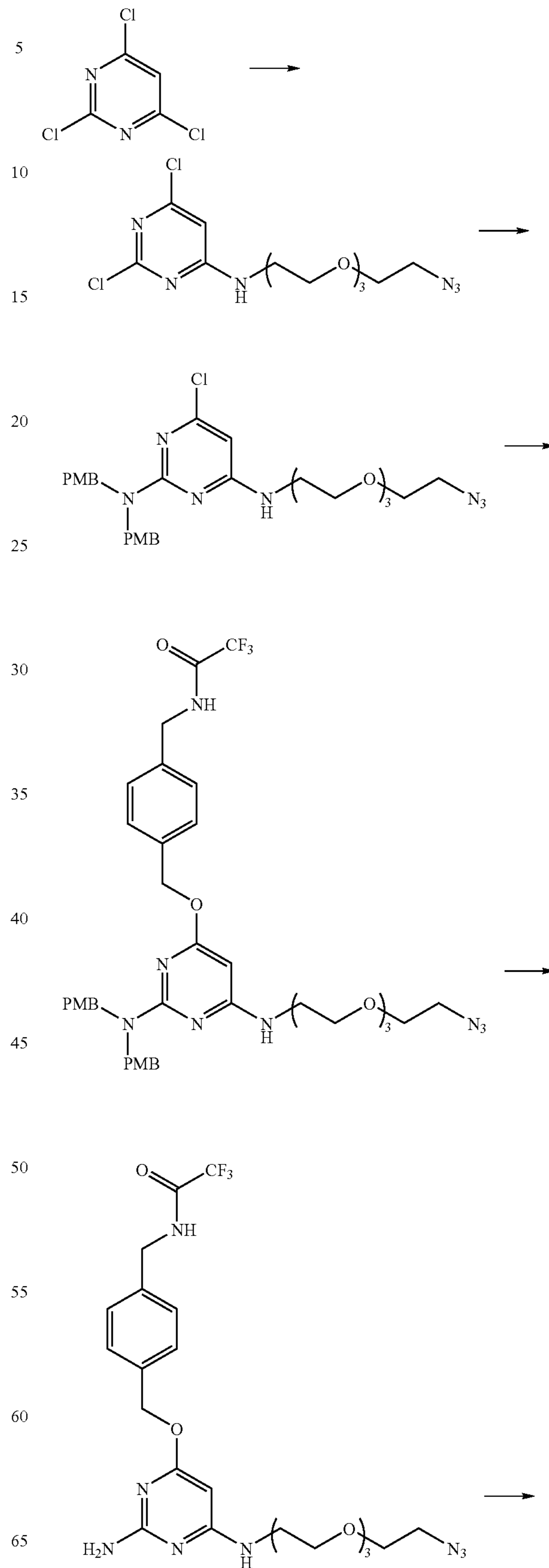
Scheme 9
