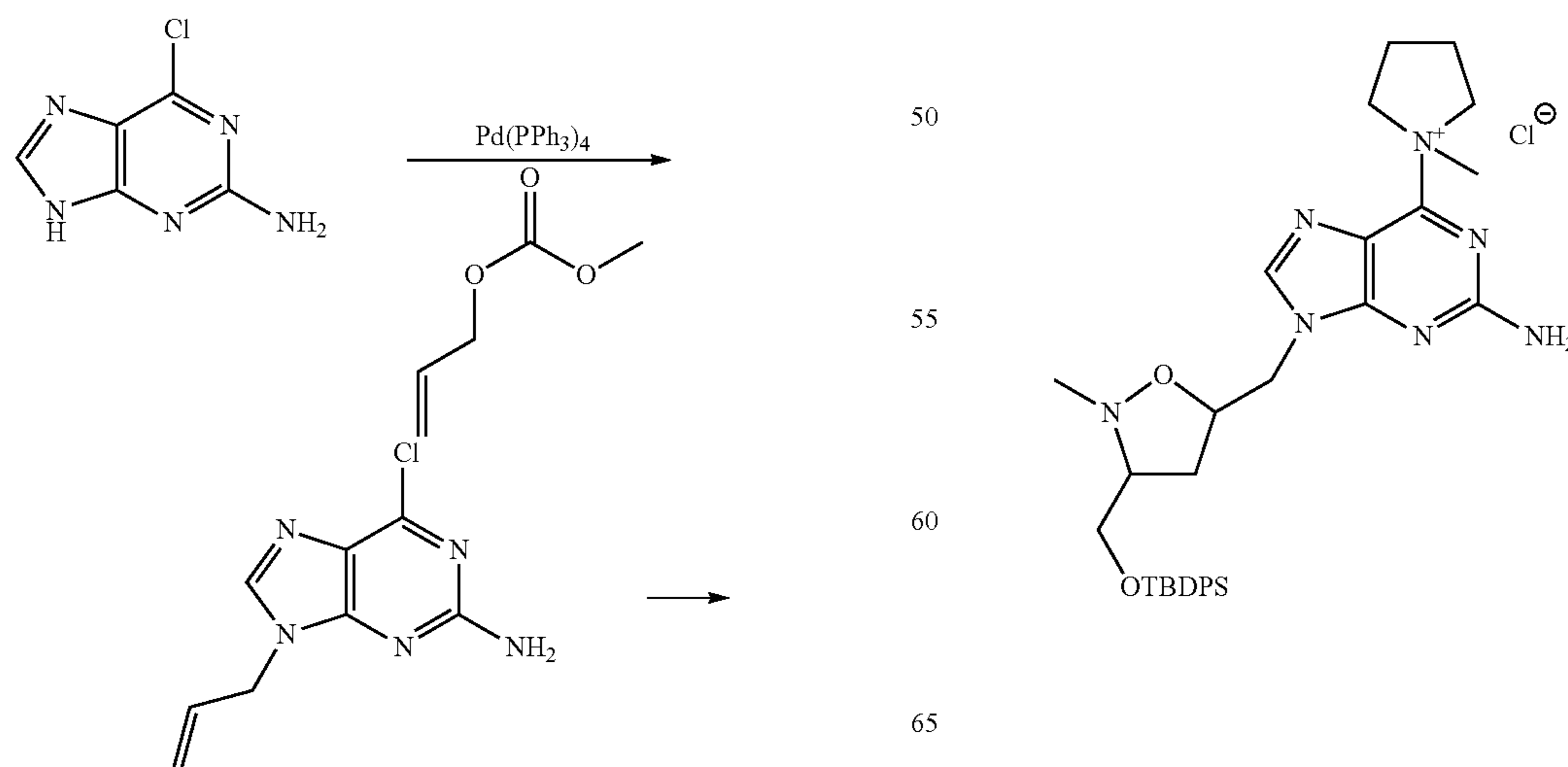
Scheme 4
