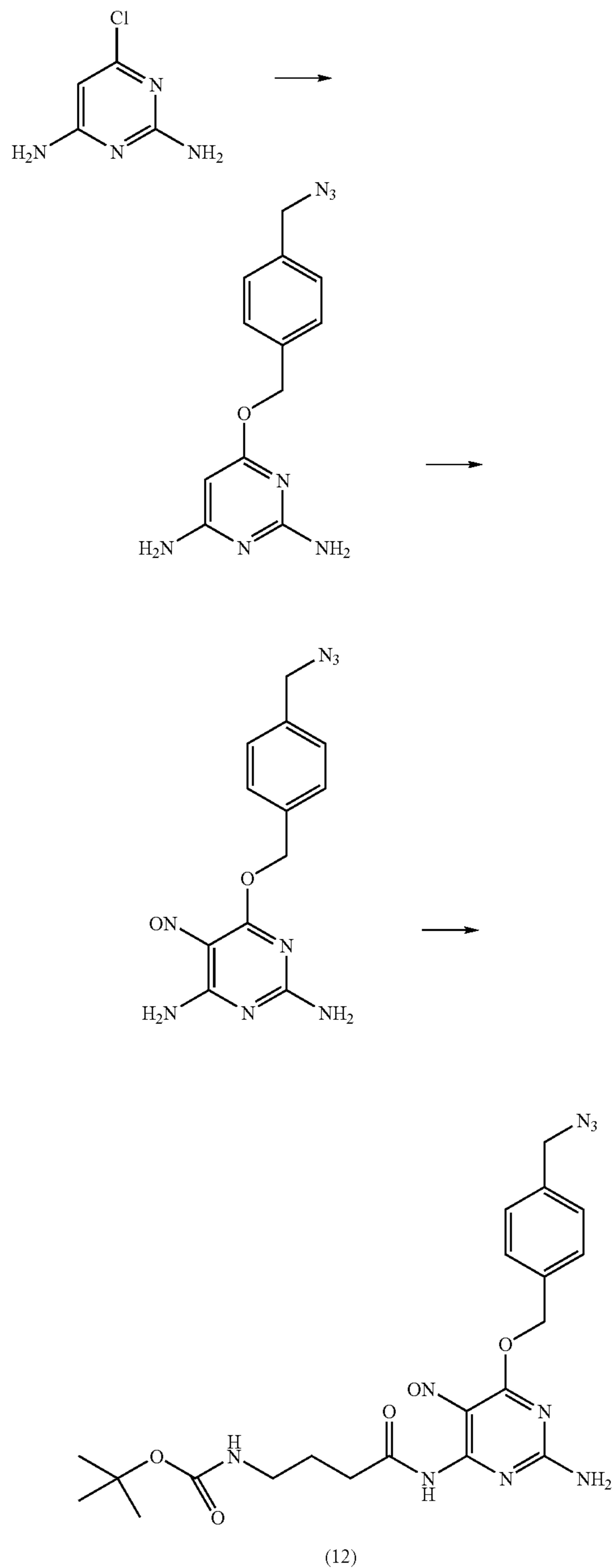
Scheme 8
