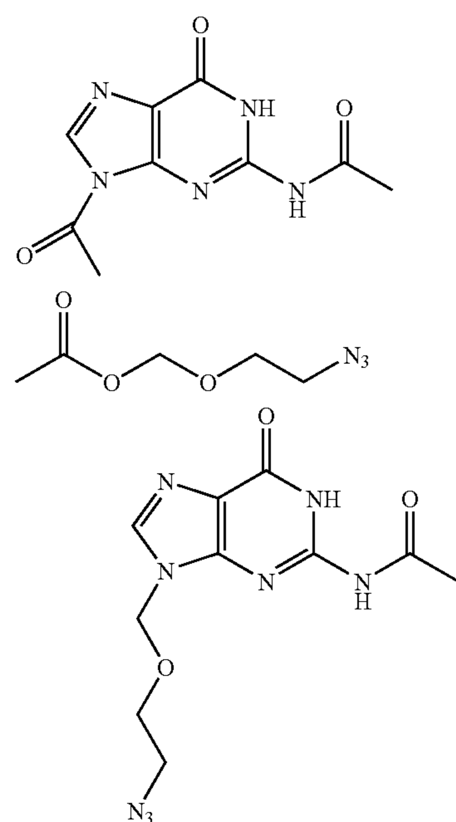
Scheme 1
