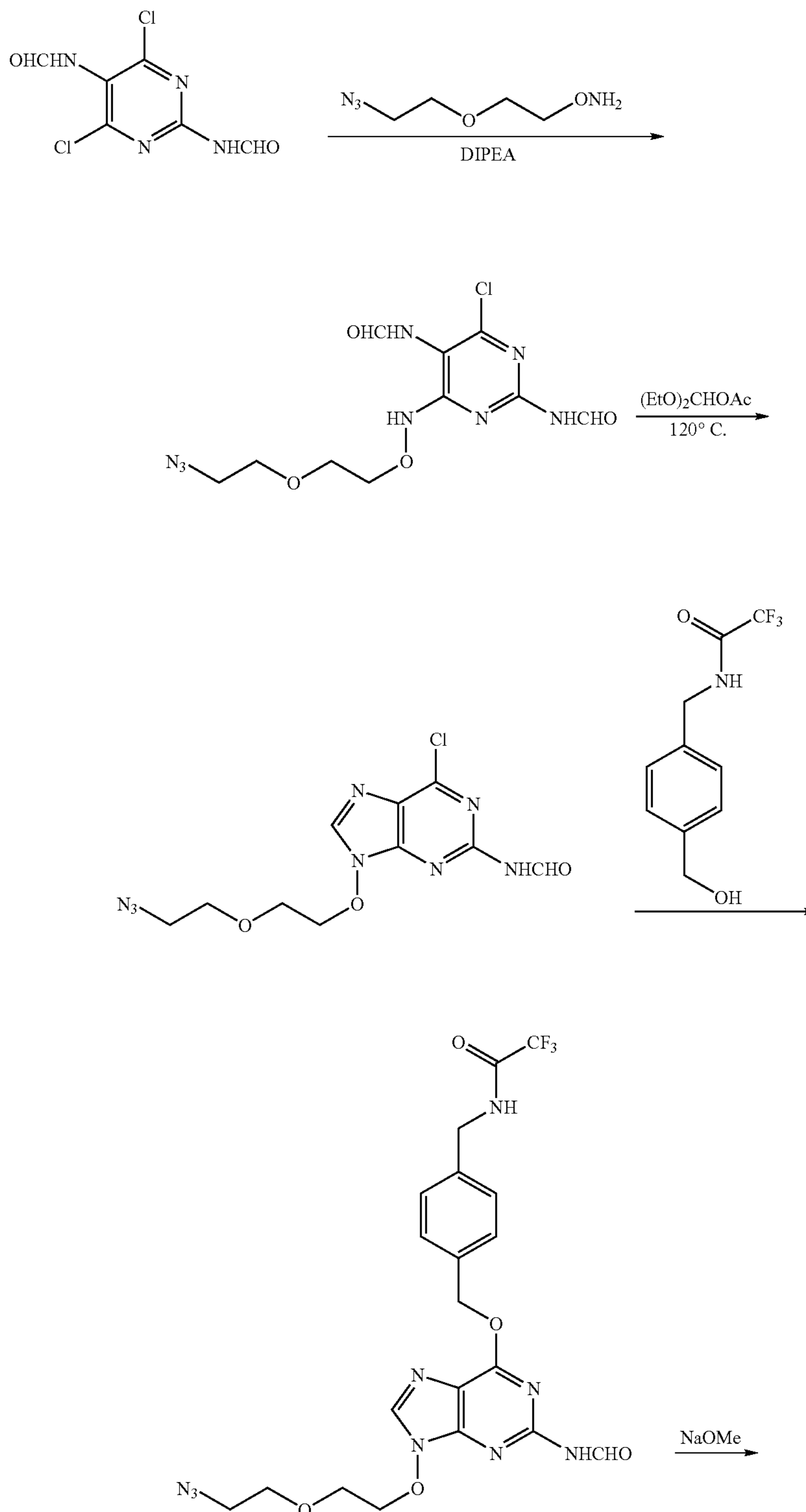
Scheme 2
