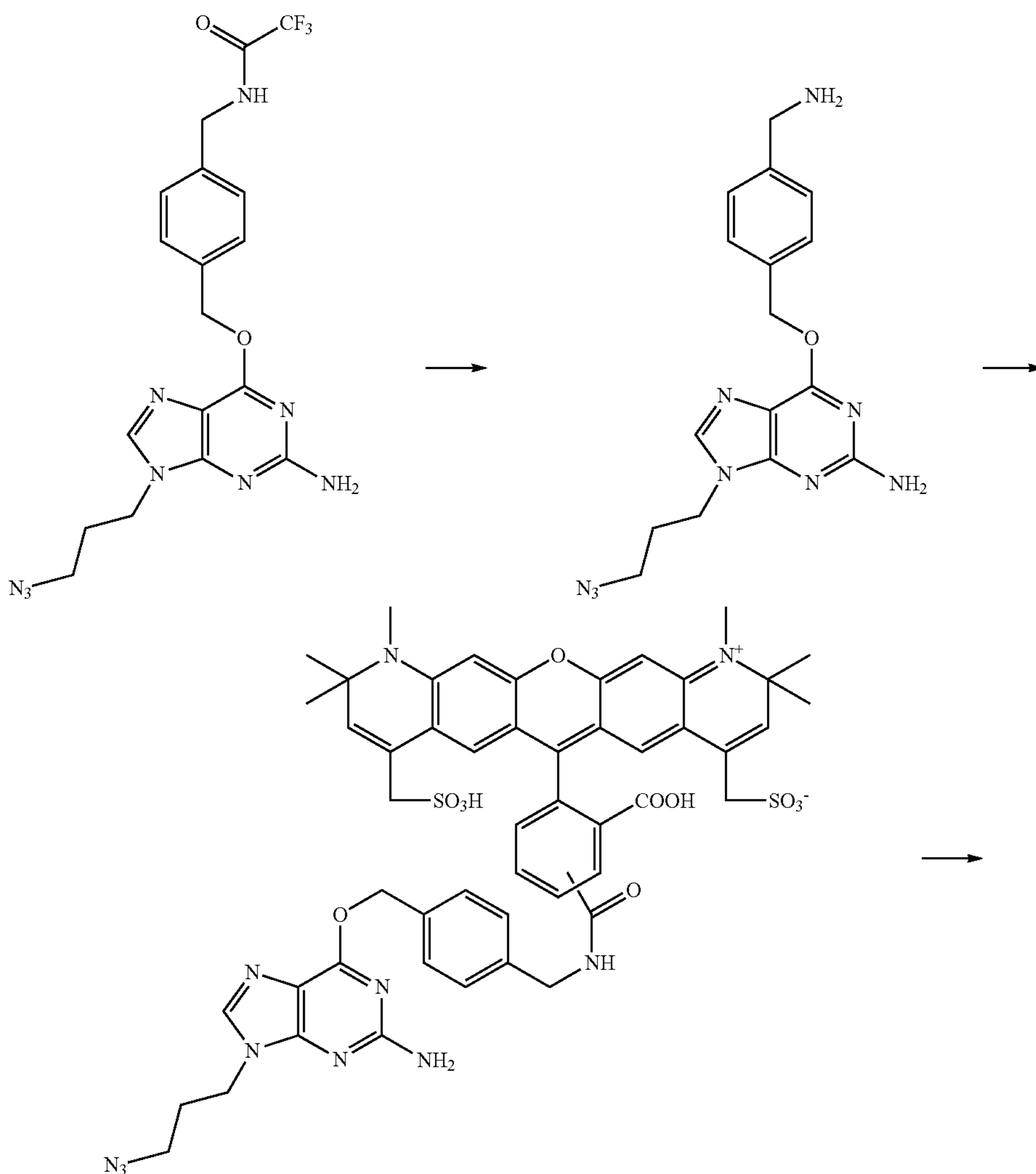
Scheme 5
