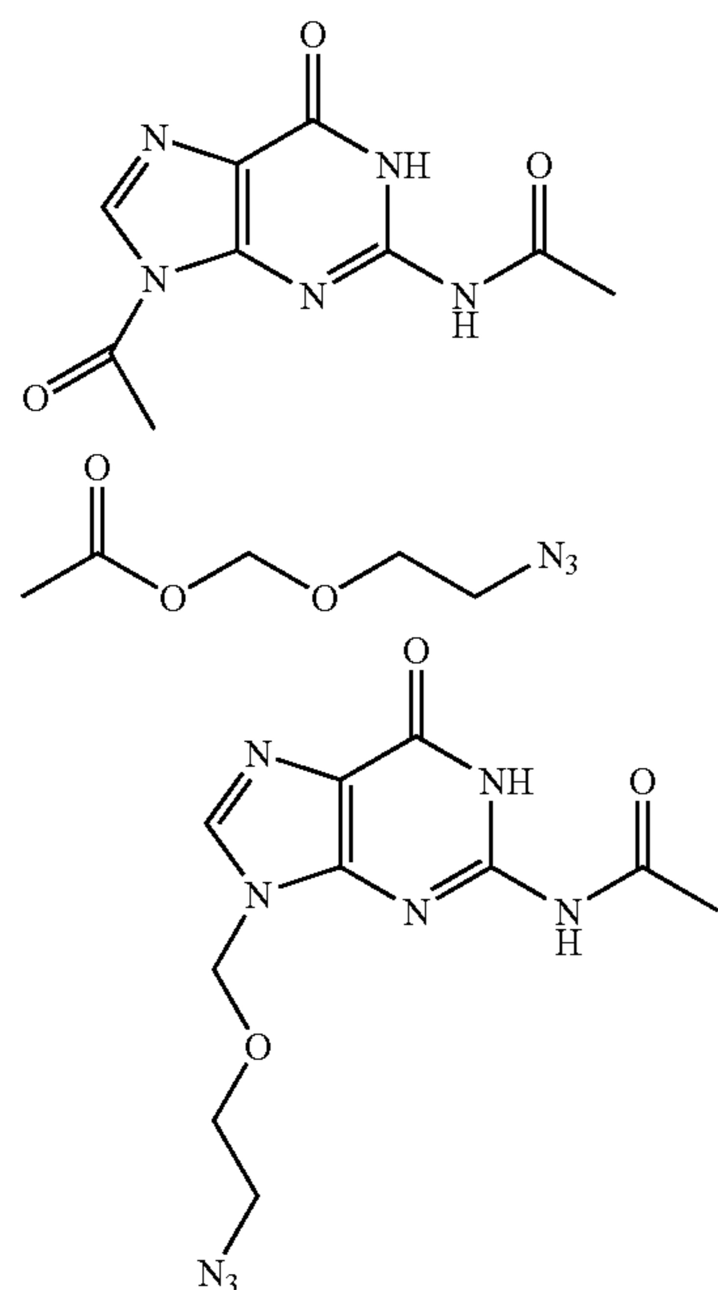
Scheme 1
