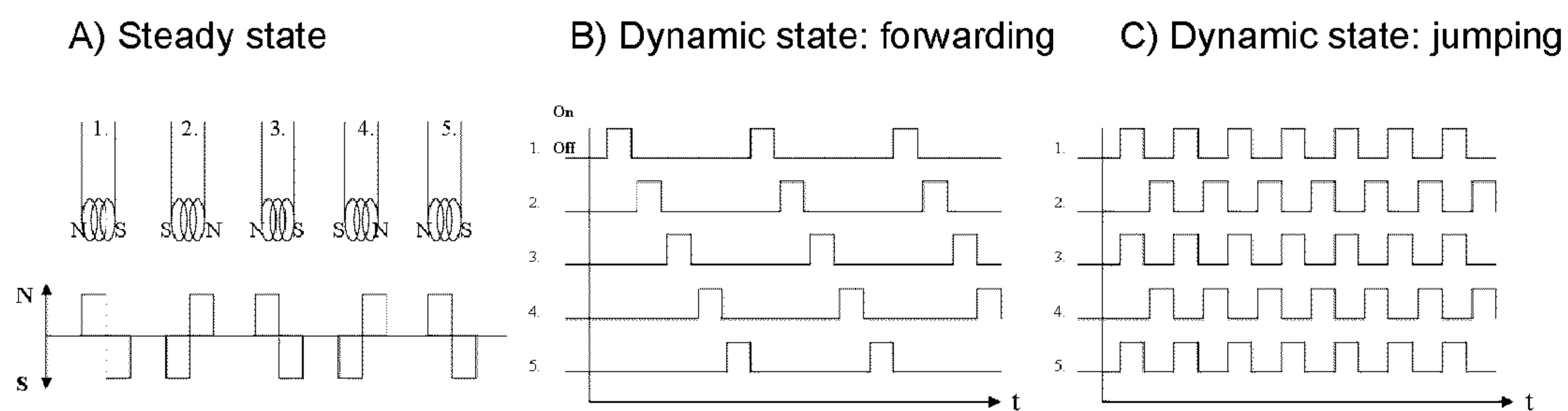
Phased Array Connect & Switch Timing Schematic
