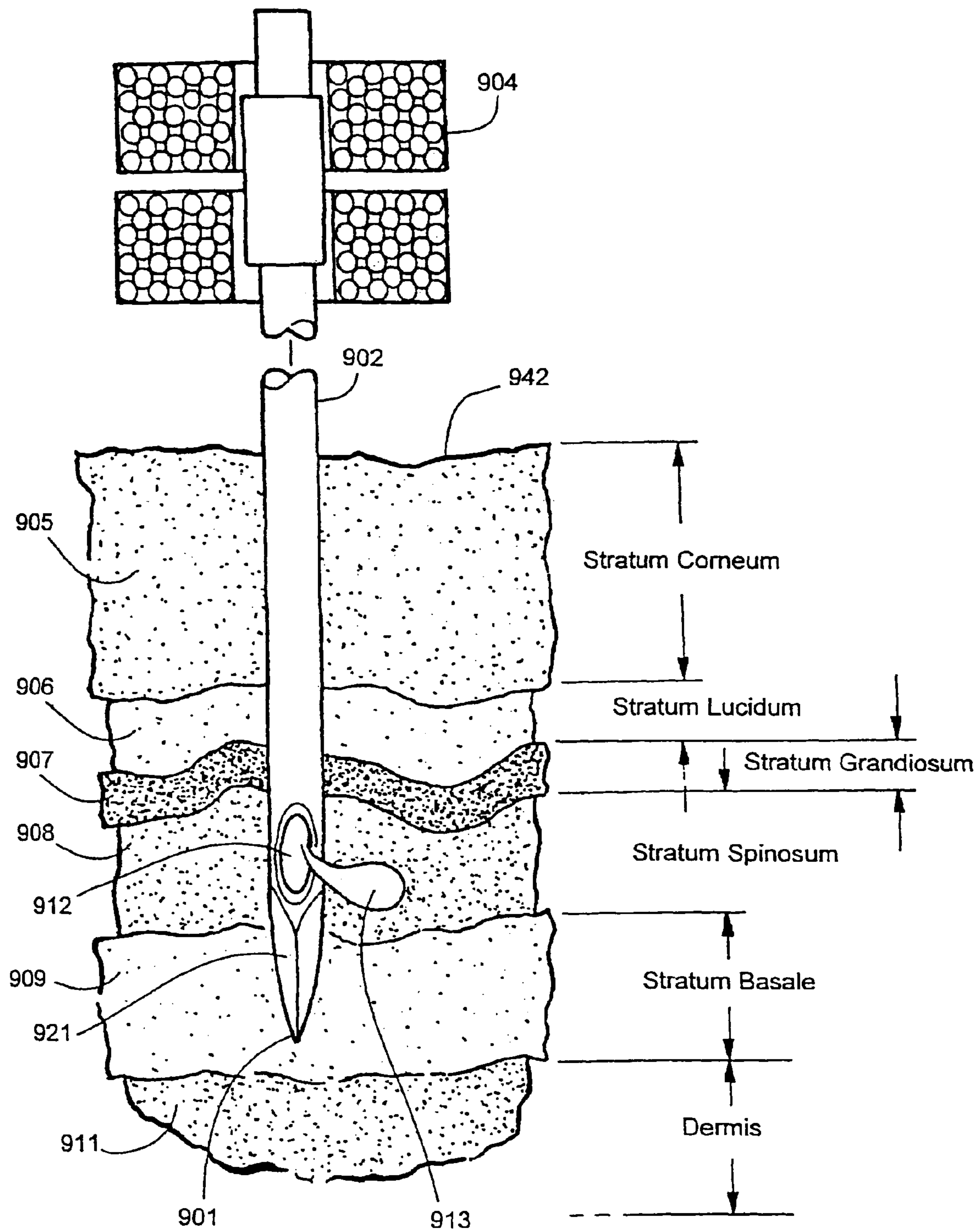
Syringe Needle
