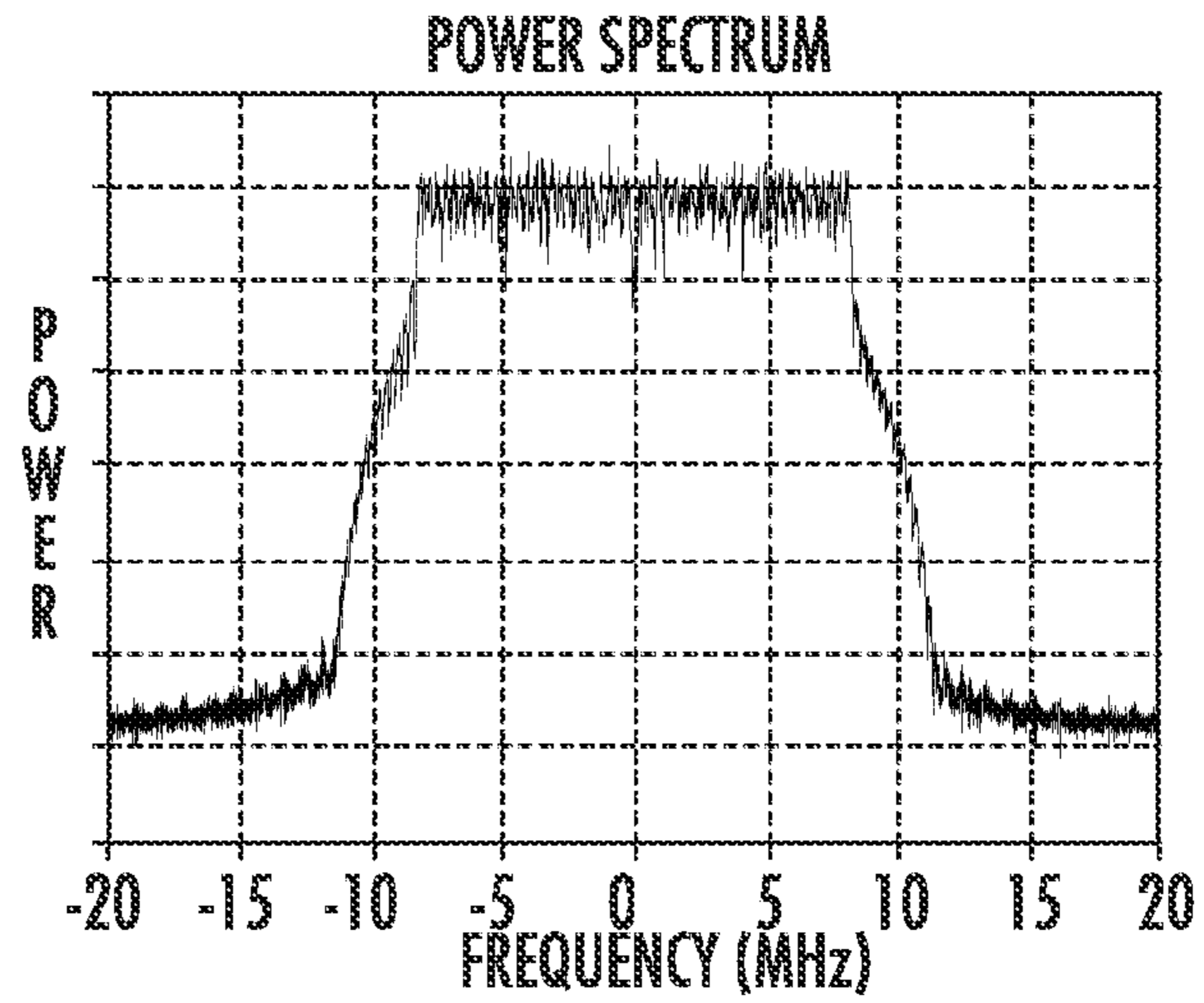
TYPICAL OFDM SPECTRUM (POWER)
