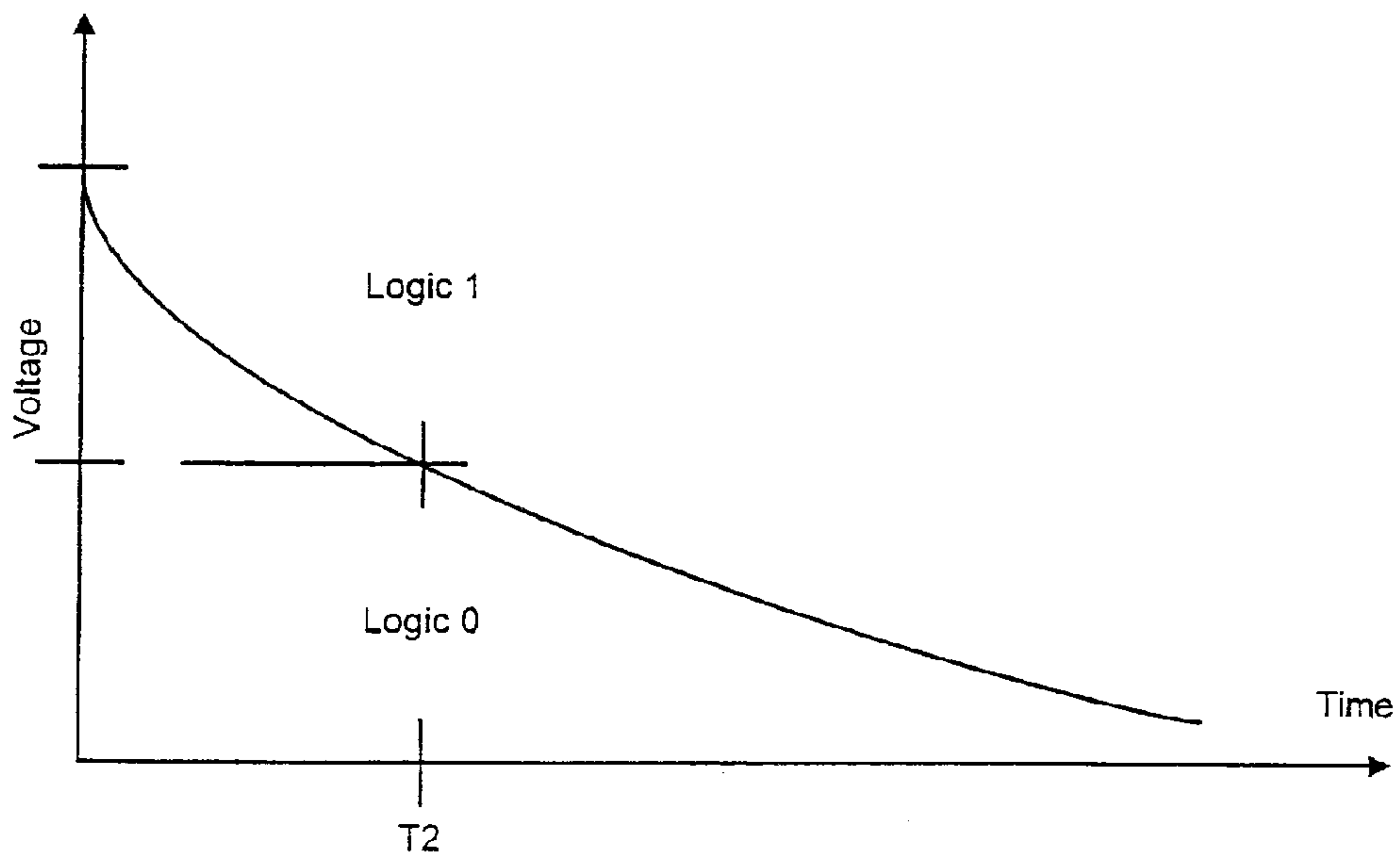
Figure 4(b) Discharge Waveform of Valid DRAM Bit
