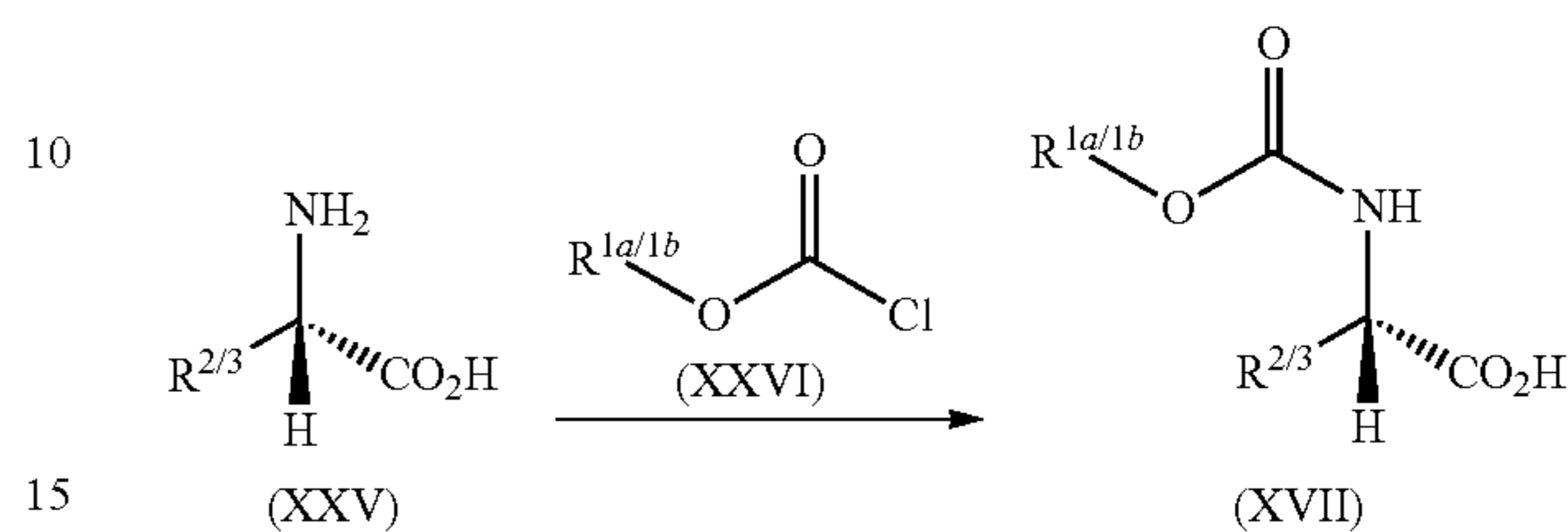
Scheme 4. Conversion of Deuterated tert-Leucine to Corresponding Carbamate.
