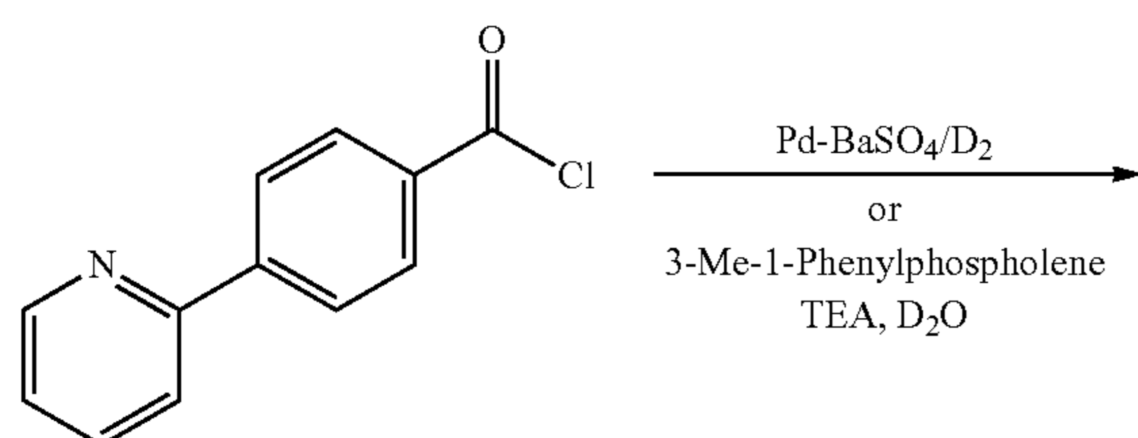
Scheme 2. Preparation of Deuterated Intermediate X
