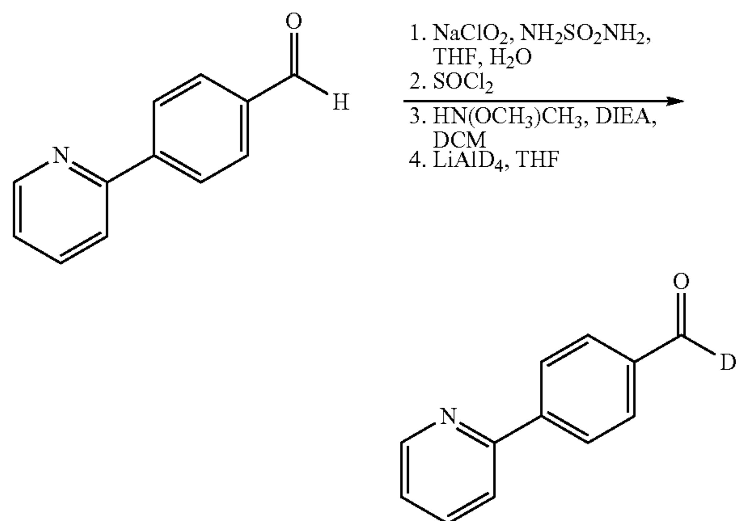
Scheme 2b. Alternative Preparation of Deuterated Intermediate X.
