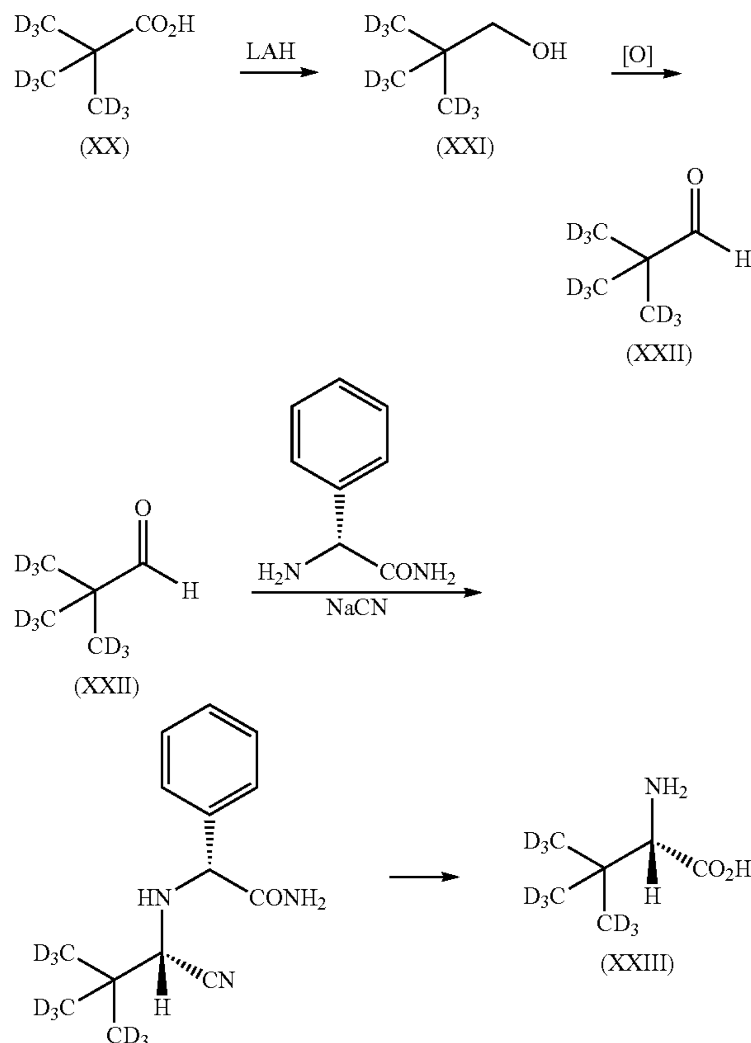
Scheme 3. Route to Prepare Deuterated tert-Leucine (XXIII).
