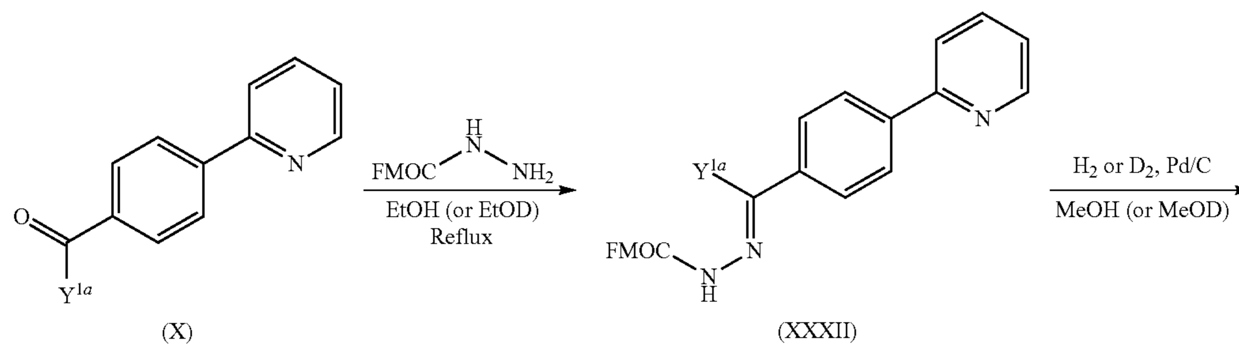
Scheme 1c. General Route for Incorporating Different R and Y Groups.
