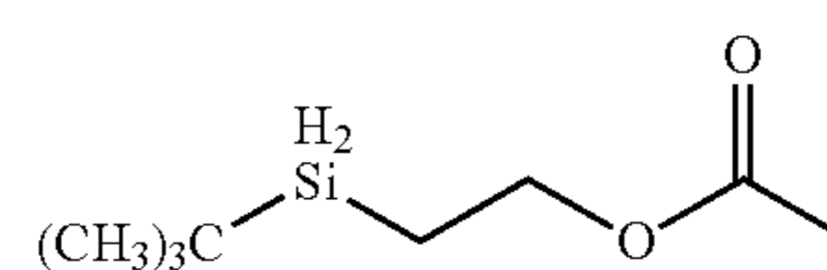
TBDMS
