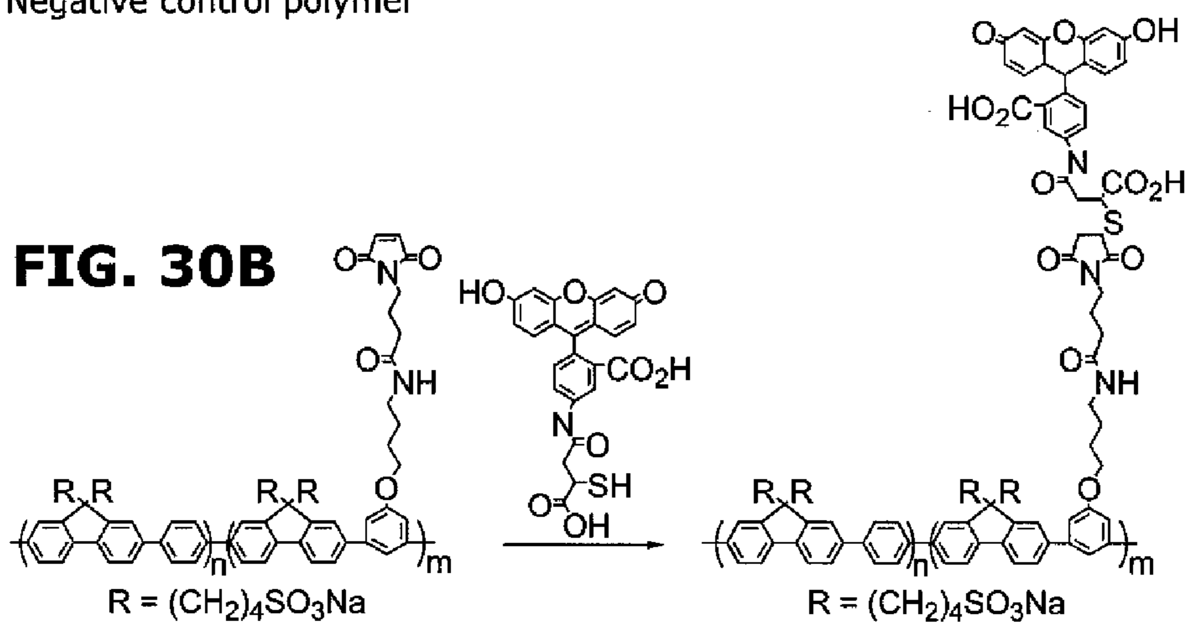
Maleimide-functionalized polymer
