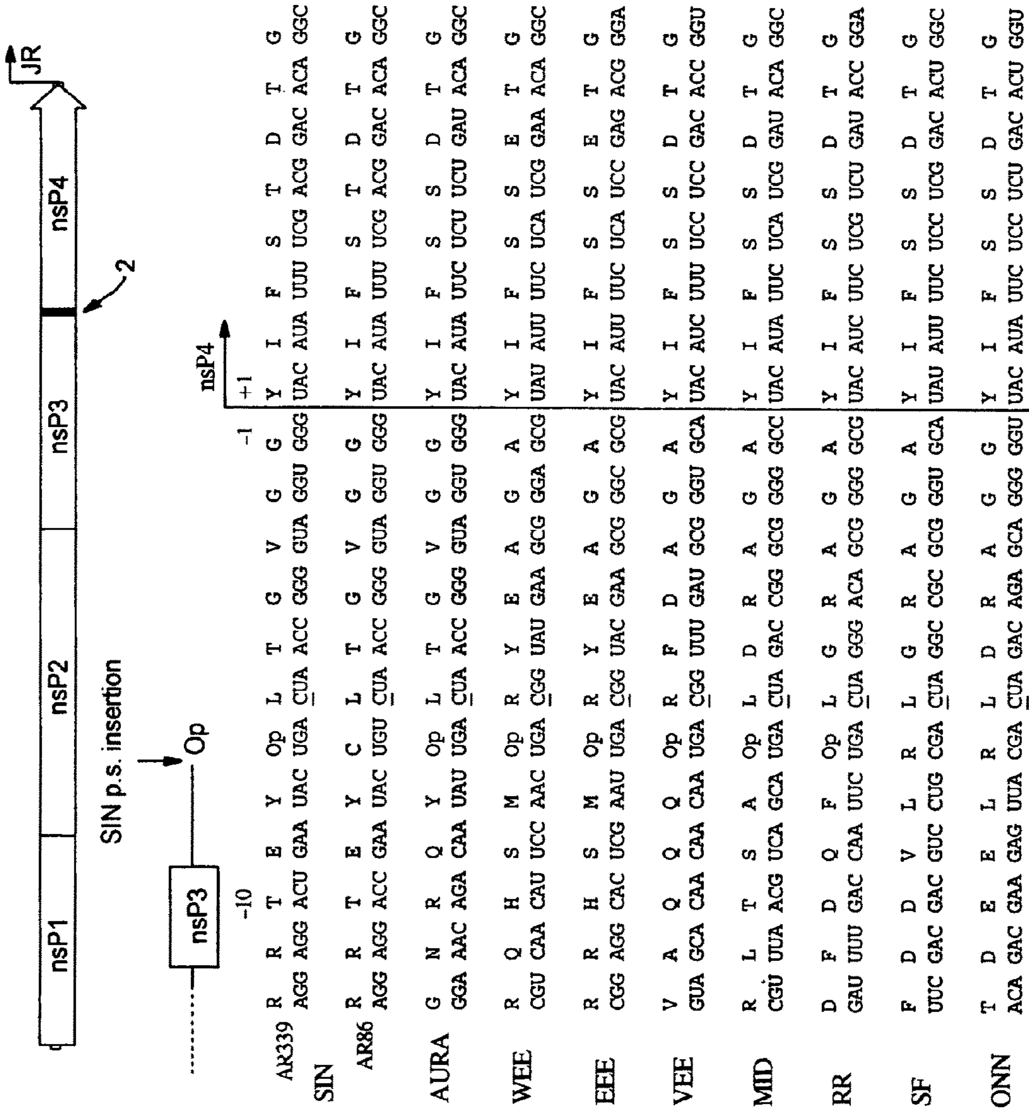
SIN/Vee packaging chimera #3: Insertion at carboxy-terminus of VEE nsP3
