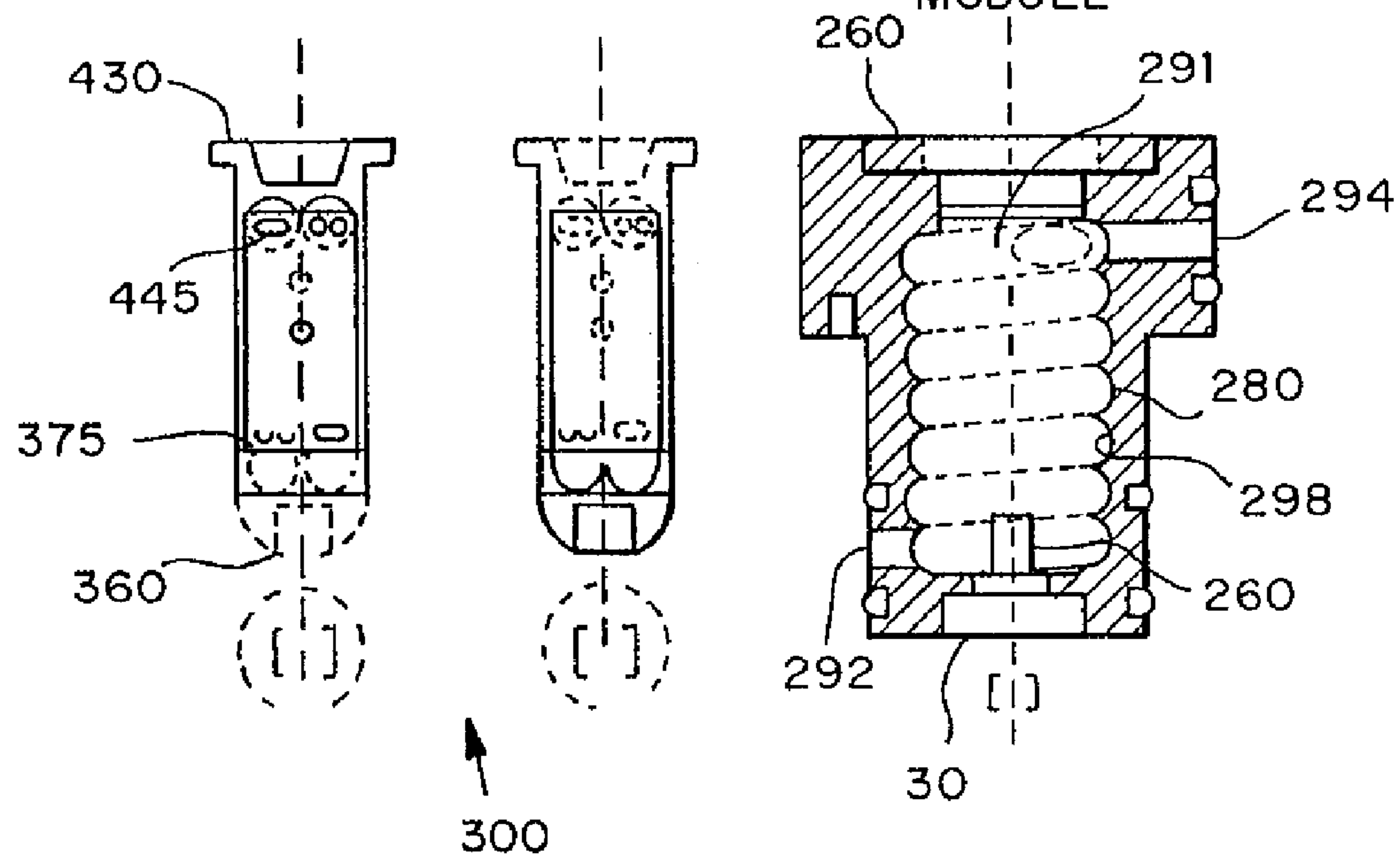
FIG. 18 PARTICLE ENTRAINMENT TURBOCELL MODULE
