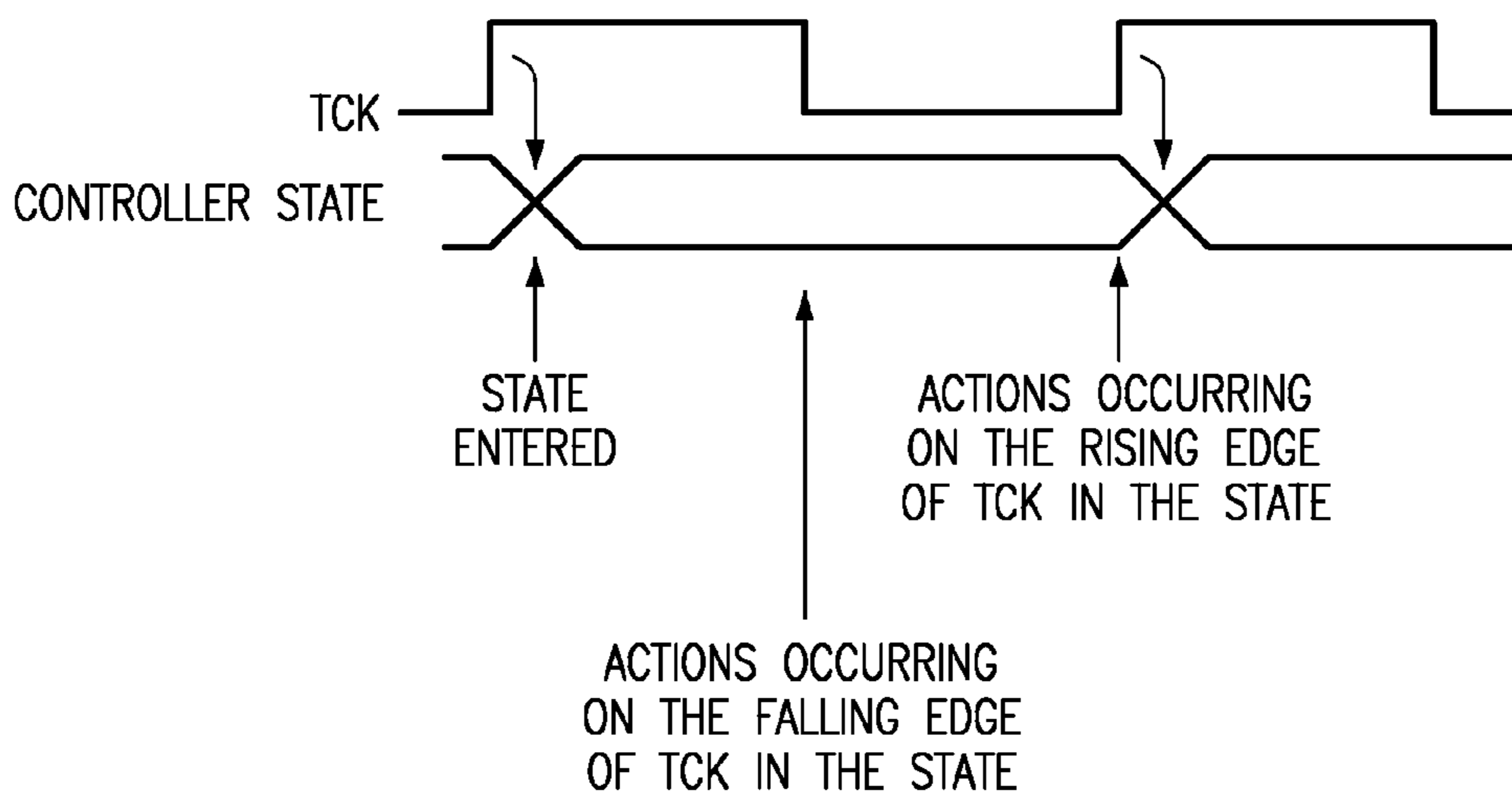
FIG. 15 (PRIOR ART)
