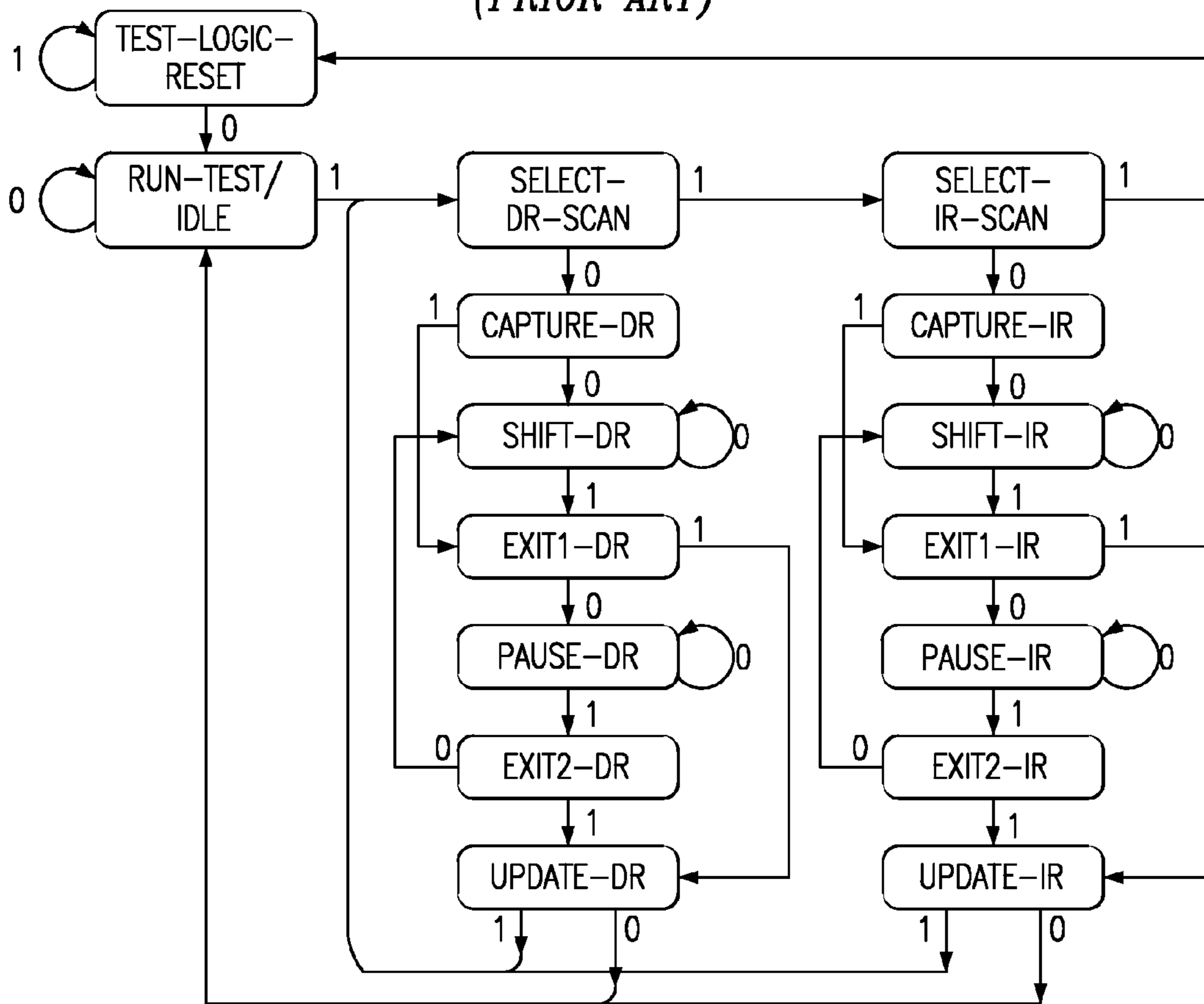
FIG. 14 (PRIOR ART)
