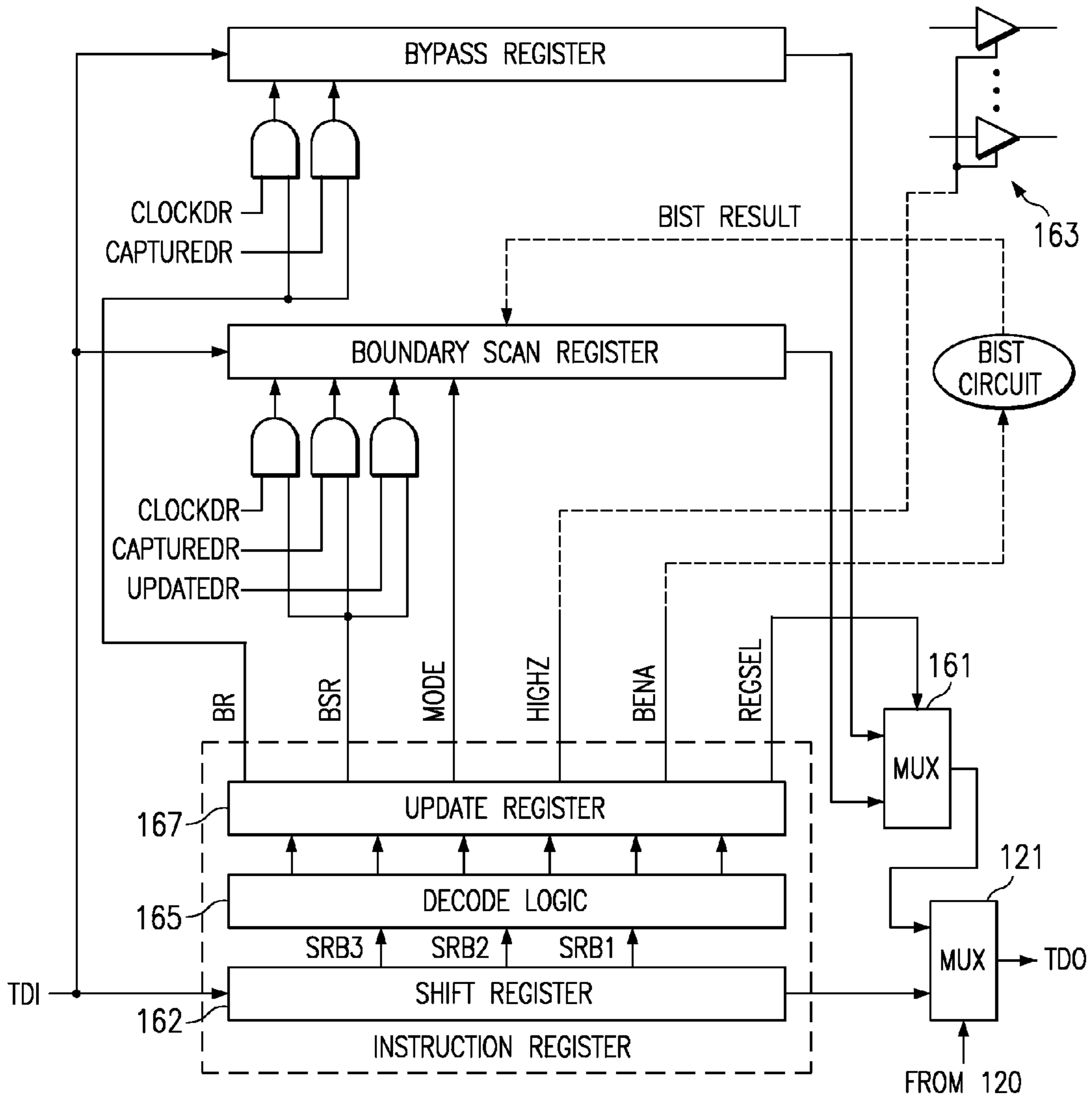
FIG. 16 (PRIOR ART)
