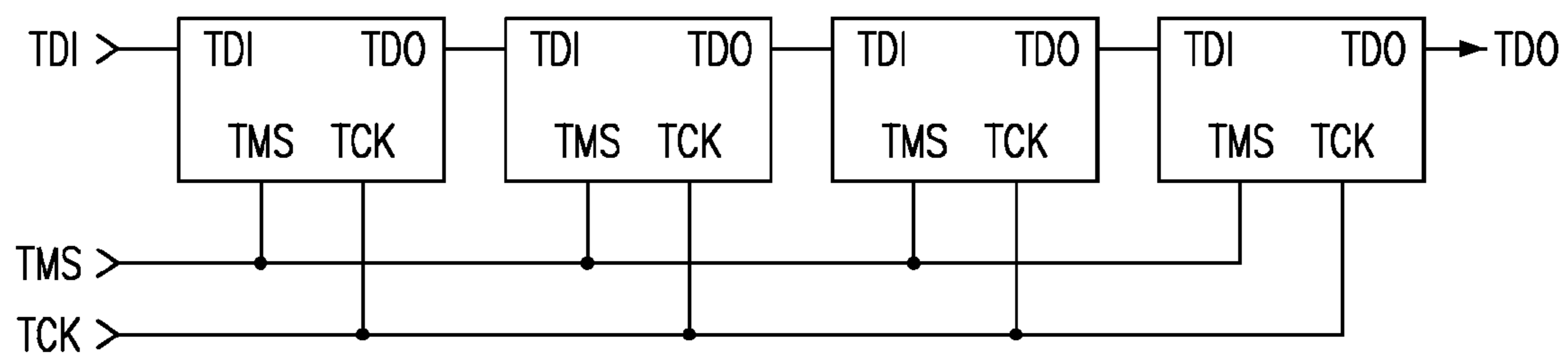
FIG. 13 (PRIOR ART)
