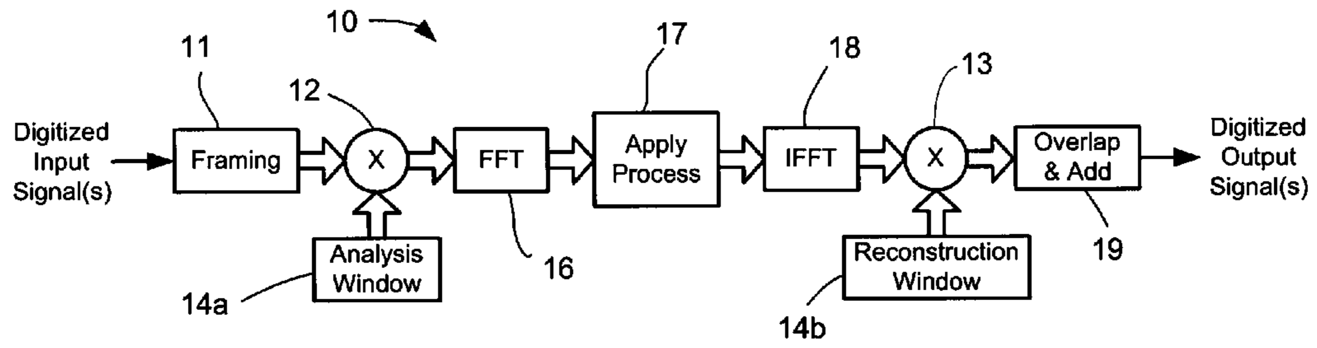
FIG. 1 (PRIOR ART)
