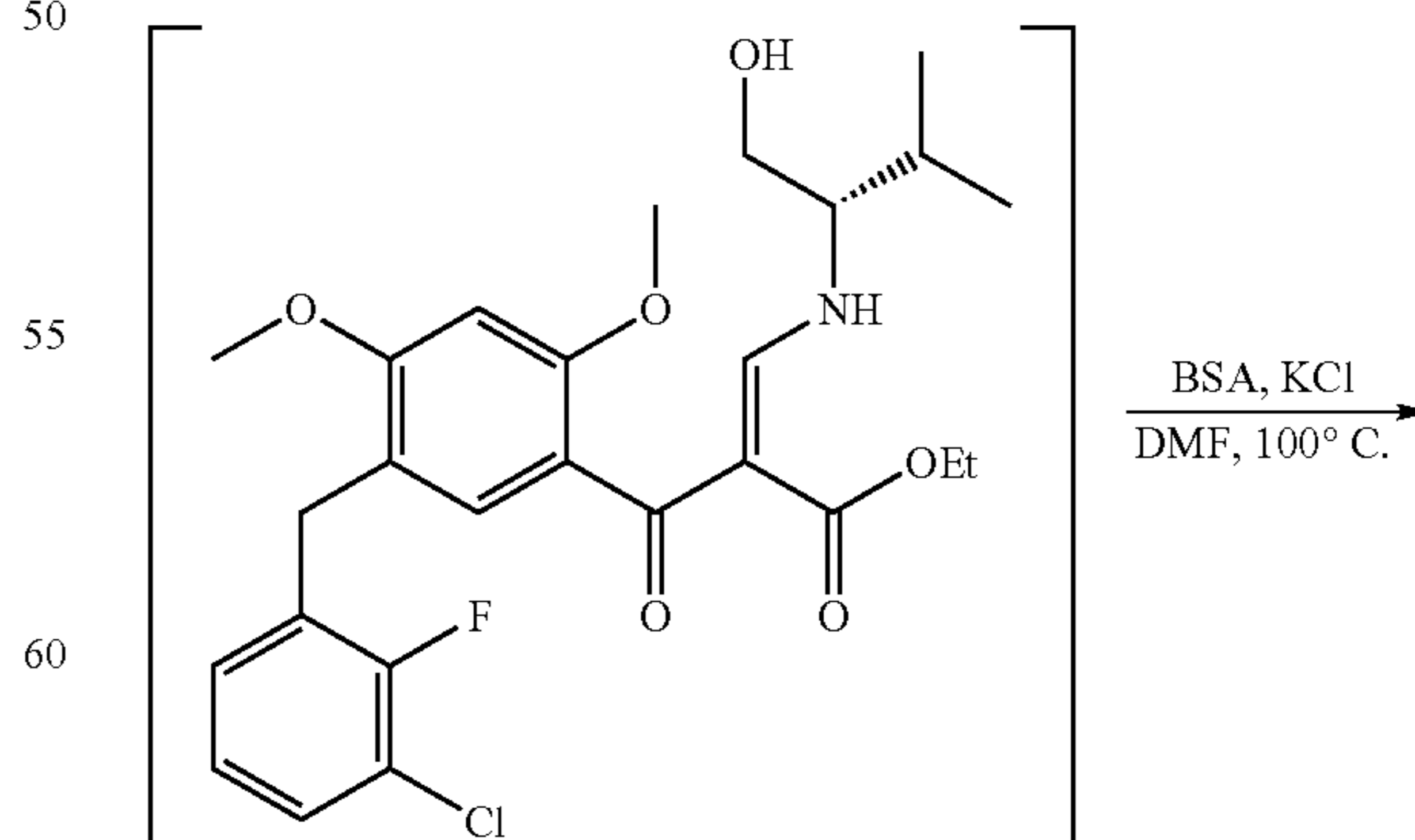
Compound 8a C 26 H 31 ClFNO 6 Mol. Wt.: 507.98
