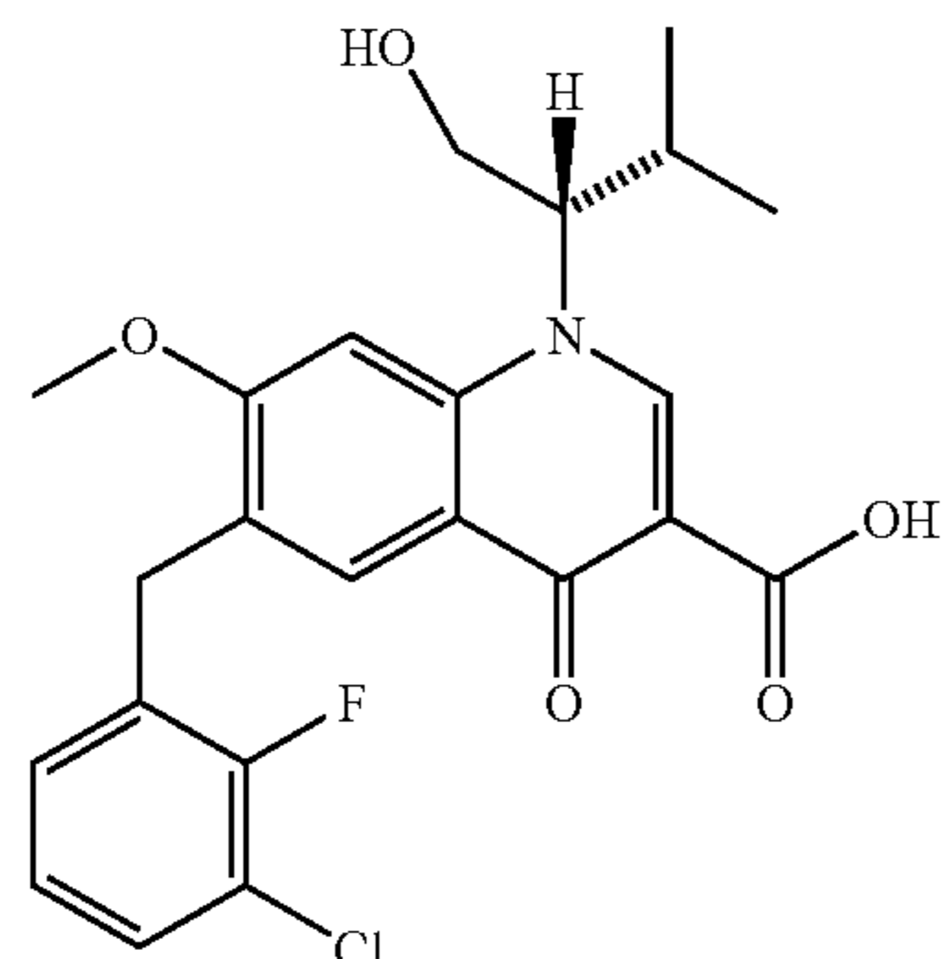
Compound 10, \gamma -form C_{23}H_{23}ClFNO_5 Mol. Wt.: 447.88
