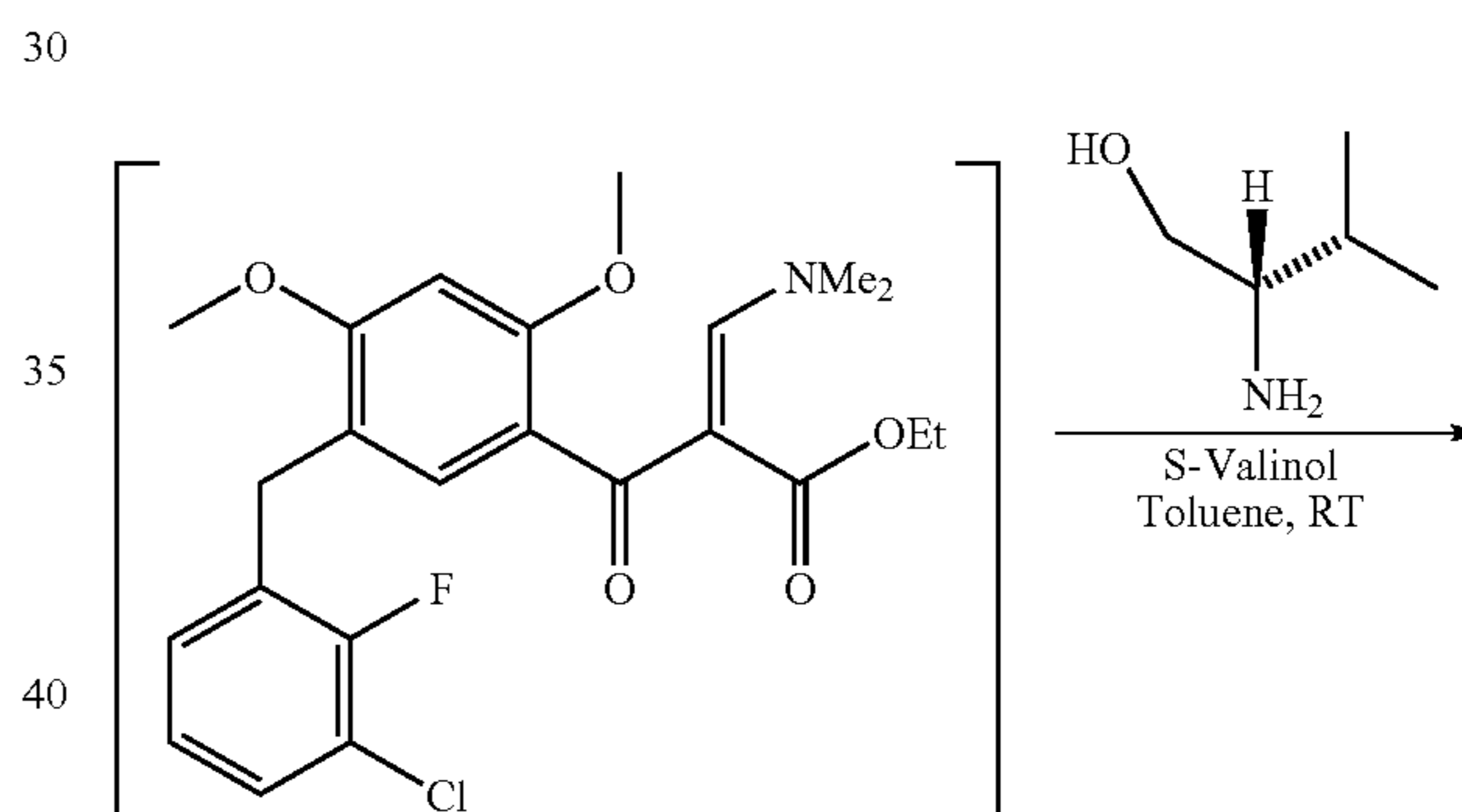
Compound 7a C 23 H 25 ClFNO 5 Mol. Wt.: 449.9
