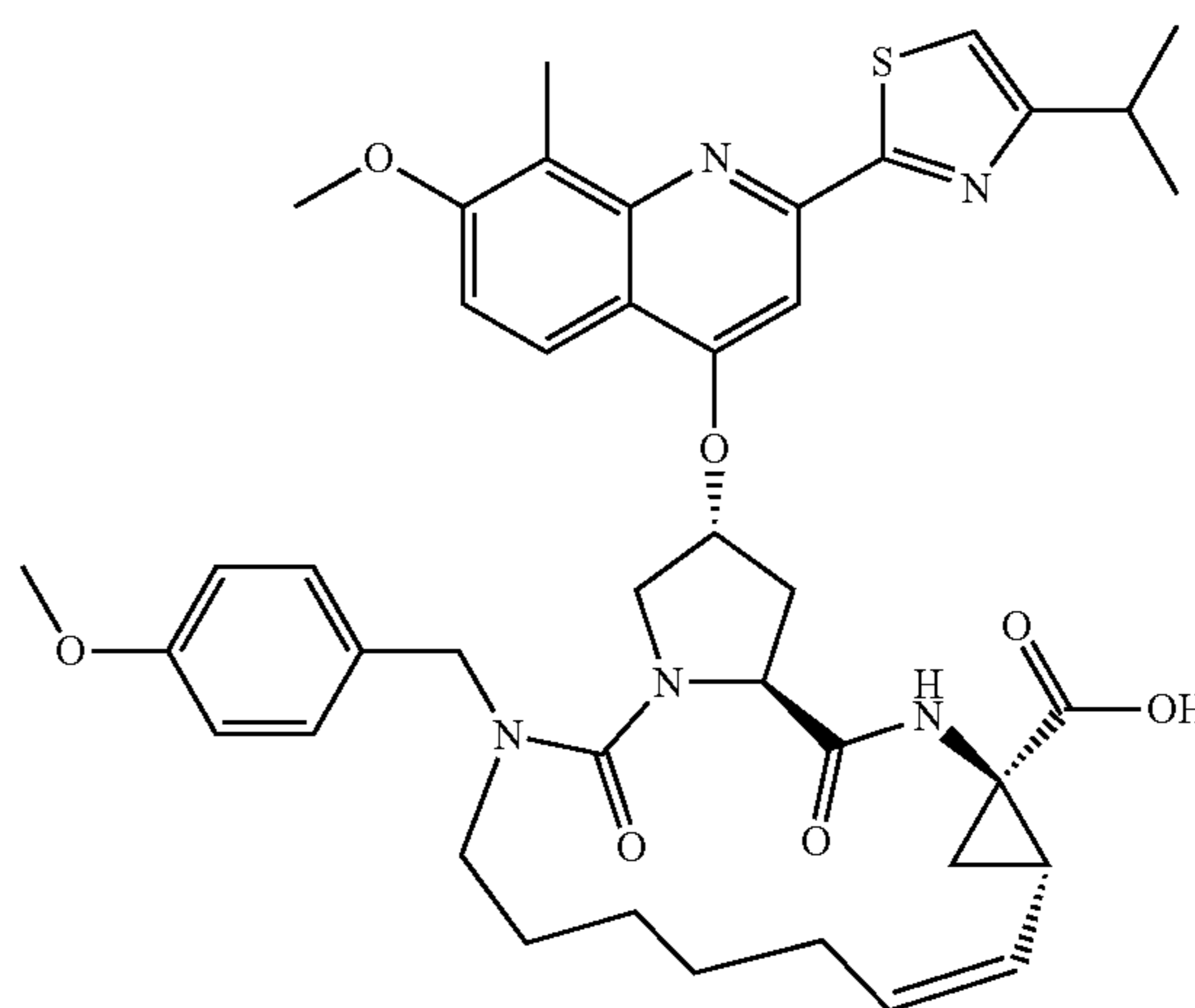
18-[2-(4-Isopropyl-thiazol-2-yl)-7-methoxy-8-methyl-quinolin-4-yloxy]-14-(4-methoxybenzyl)-2,15-dioxo-3,14,16-triaza-tricyclo[14.3.0.0*4,6]nonadec-7-ene-4-carboxylic acid (138)
