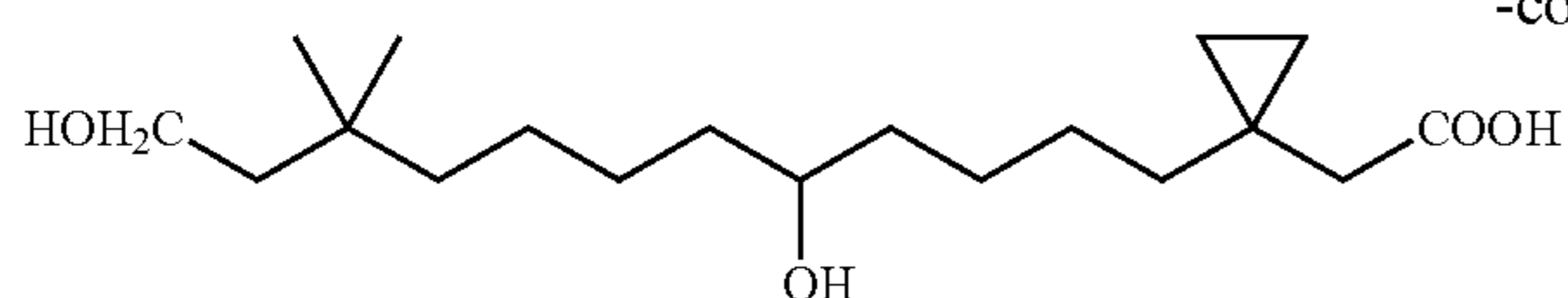
[1-(5,12-Dihydroxy-10,10-dimethyl-dodecyl)-cyclopropyl]-acetic acid
