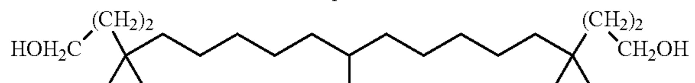
15-[1-(3-Hydroxy-propyl)-cyclopropyl]-4,4-dimethyl-pentadecane-1,10-diol Compound 79
