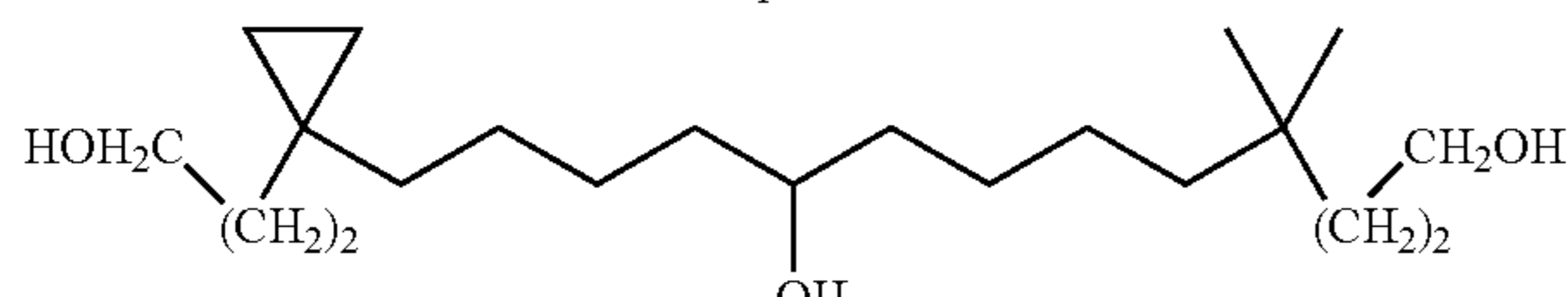
13-[1-(3-Hydroxy-propyl)-cyclopropyl]-4,4-dimethyl-tridecane-1,9-diol Compound 75
