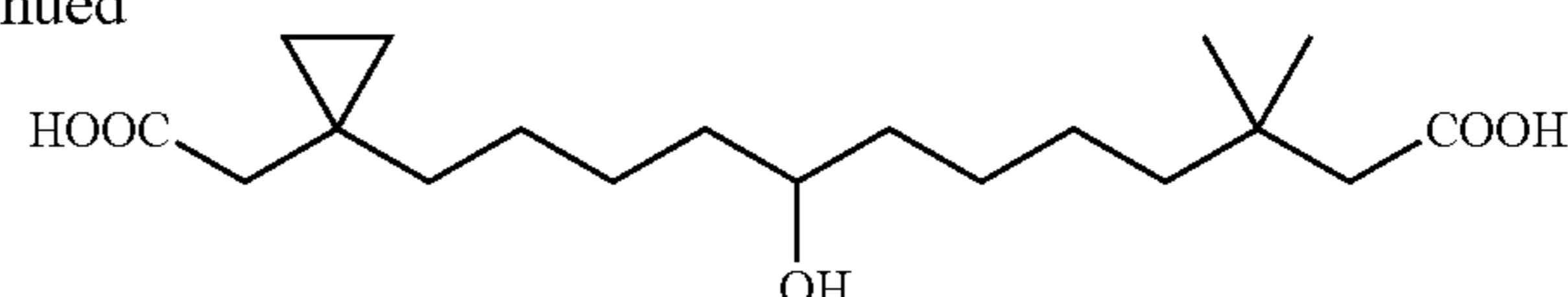
12-(1-Carboxymethyl-cyclopropyl)-8-hydroxy-3,3-dimethyl-dodecanoic acid
