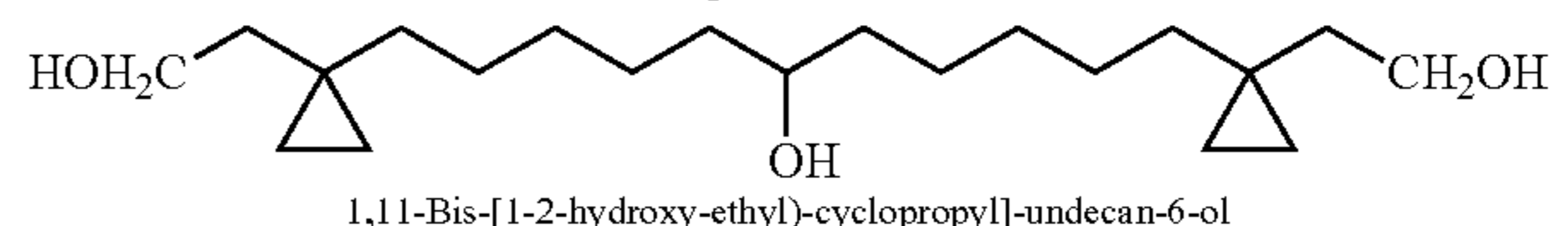
1,11-Bis-[1-(2-hydroxy-ethyl)-cyclopropyl]-undecan-6-ol Compound 28
