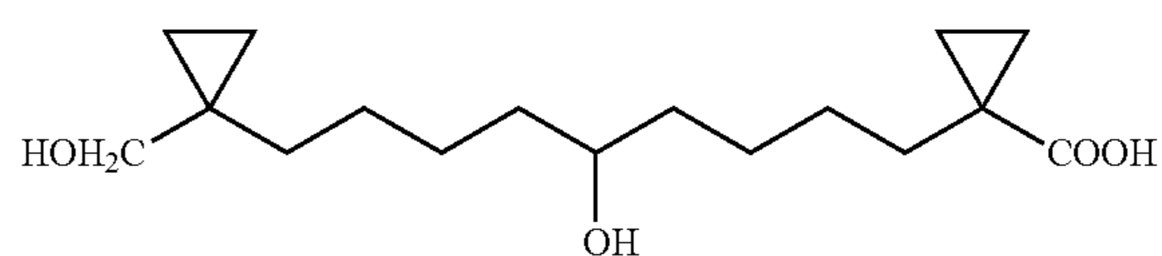
1-[5-Hydroxy-9-(1-hydroxymethyl-cyclopropyl)-nonyl]-cyclopropanecarboxylic acid
