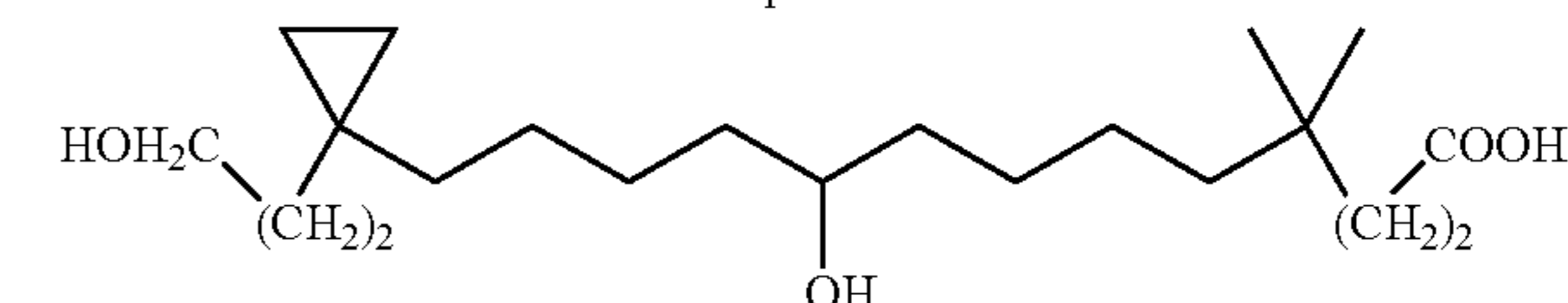
4,4-Dimethyl-9-hydroxy-13-[1-(3-hydroxypropyl)-cyclopropyl]-tridecanoic acid
