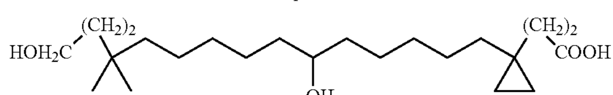
3-[1-(6,15-Dihydroxy-12,12-dimethyl-pentadecyl)-cyclopropyl]-propionic acid
