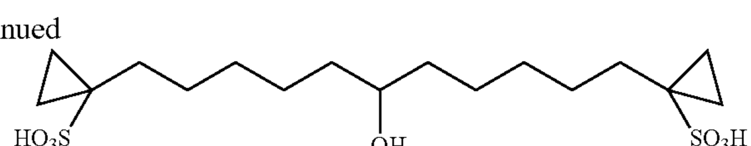
1,11-Bis-(1-sulfonyloxy-cyclopropyl)-undecan-6-ol Compound 20
