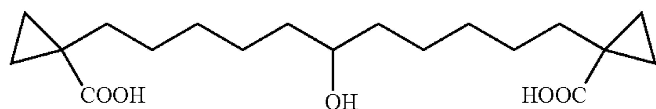
1,11-Bis-(1-carboxy-cyclopropyl)-undecan-6-ol
