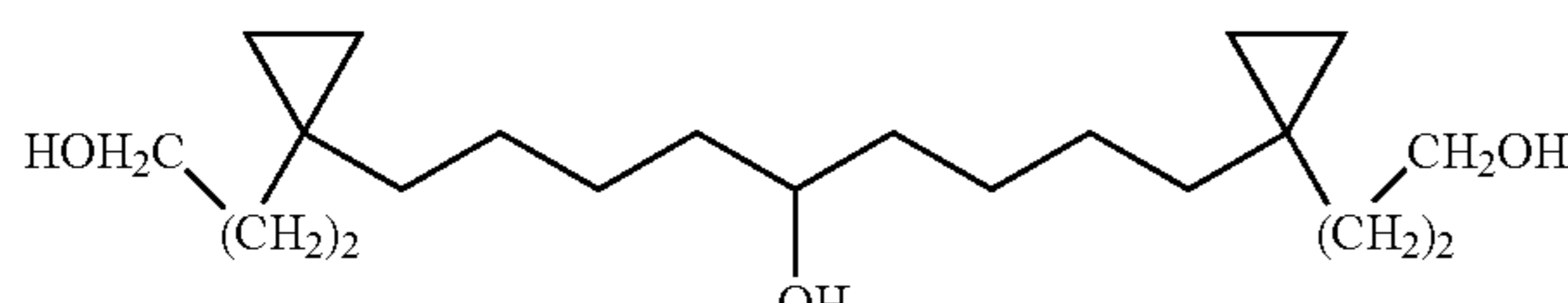
1,9-Bis-[1-(3-hydroxy-propyl)-cyclopropyl]-nonan-5-ol Compound 31
