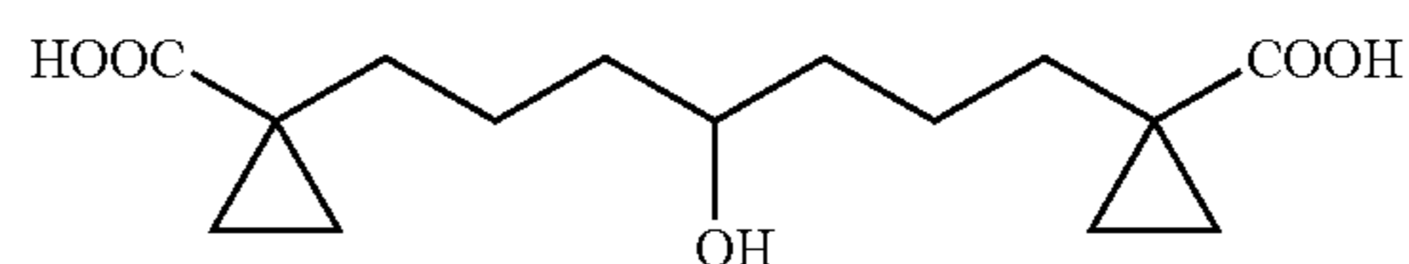
1,7-Bis-(1-carboxy-cyclopropyl)-heptan-4-ol
