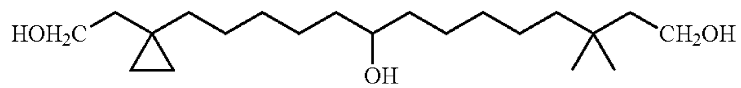
14-[1-(2-Hydroxy-ethyl)-cyclopropyl]-3,3-dimethyl-tetradecane-1,9-diol Compound 71
