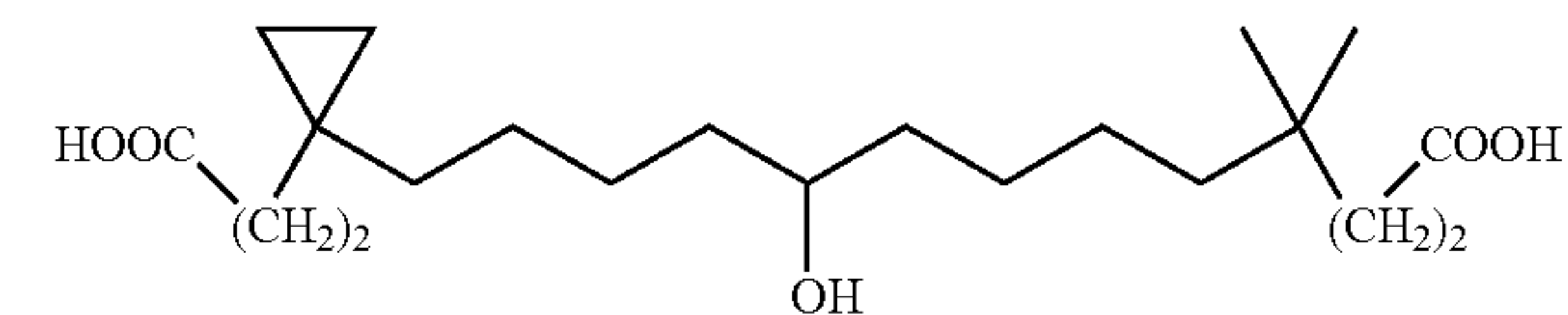
13-[1-(2-Carboxyethyl)-cyclopropyl]-9-hydroxy-4,4-dimethyl-tridecanoic acid
