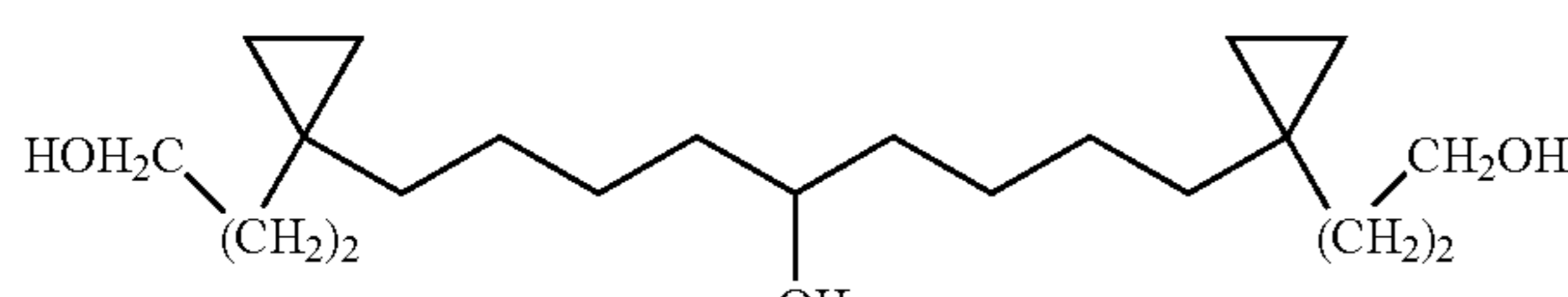
1,9-Bis-[1-(3-hydroxy-propyl)-cyclopropyl]-nonan-5-ol Compound 31
