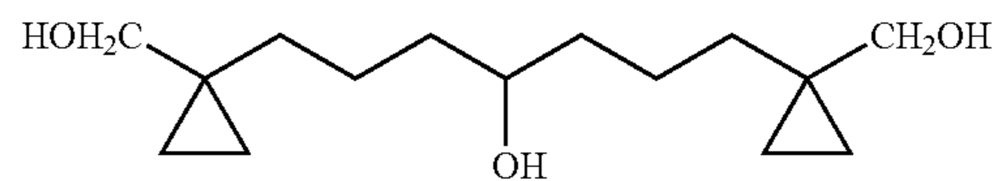
1,7-Bis-(1-hydroxymethyl-cyclopropyl)-heptan-4-ol
