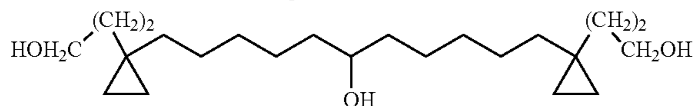
1,11-Bis-[1-(3-hydroxy-propyl)-cyclopropyl]-undecan-6-ol Compound 37
