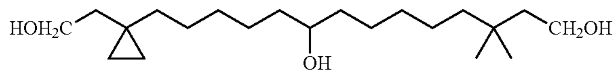
14-[1-(2-Hydroxy-ethyl)-cyclopropyl]-3,3-dimethyl-tetradecane-1,9-diol
