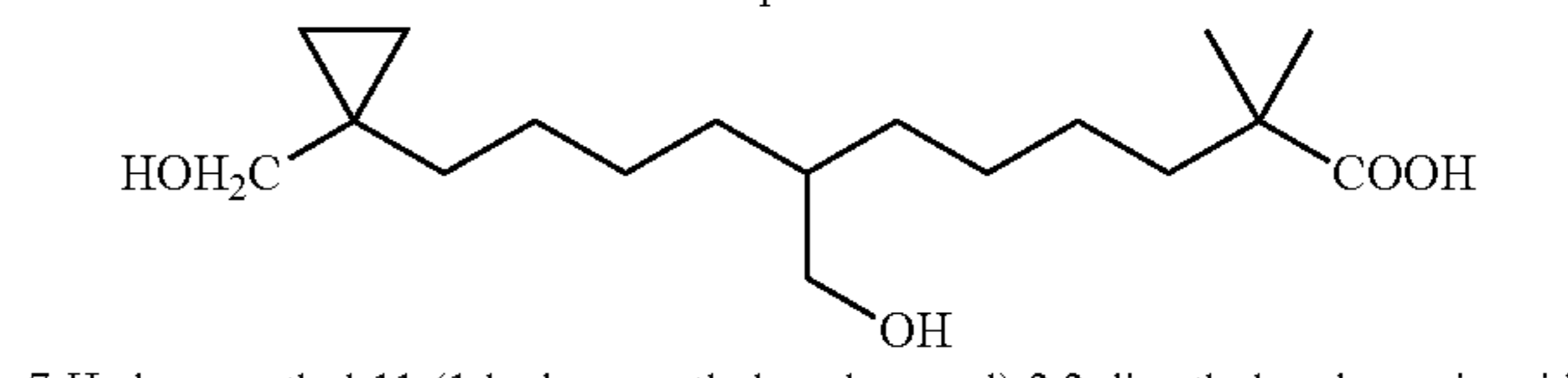
7-Hydroxymethyl-11-(1-hydroxymethyl-cyclopropyl)-2,2-dimethyl-undecanoic acid
