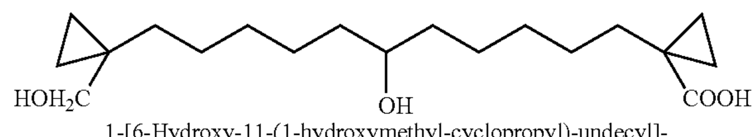
1-[6-Hydroxy-11-(1-hydroxymethyl-cyclopropyl)-undecyl]-cyclopropanecarboxylic acid
