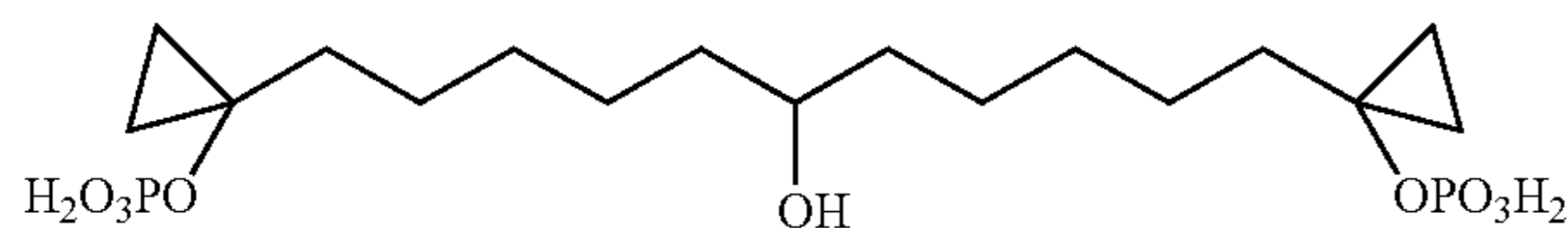
1,9-Bis-(1-phosphonoxy-cyclopropyl)-nonan-5-ol Compound 21
