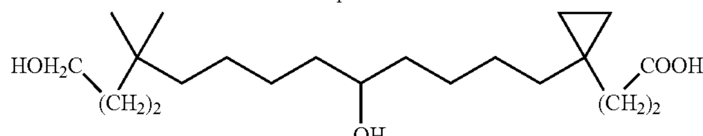
3-[1-(5,13-Dihydroxy-10,10-dimethyl-tridecyl)-cyclopropyl]-propionic acid
