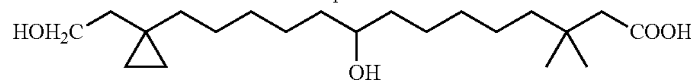
9-Hydroxy-14-[1-(2-hydroxy-ethyl)-cyclopropyl]-3,3-dimethyl-tetradecanoic acid
