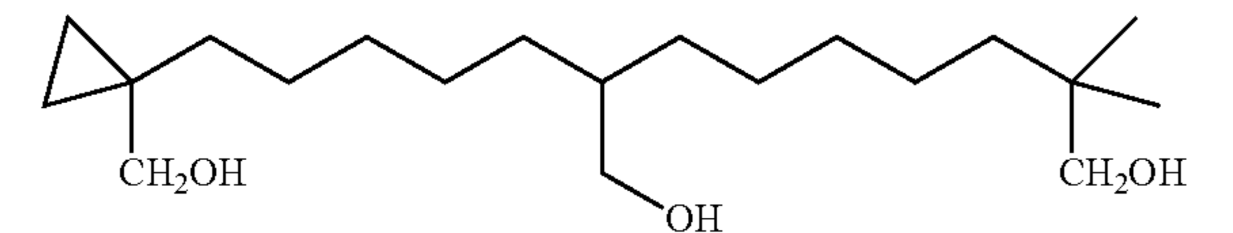
8-[5-(1-Hydroxymethyl-cyclopropyl)-pentyl]-2,2-dimethyl-nonane-1,9-diol Compound 87
