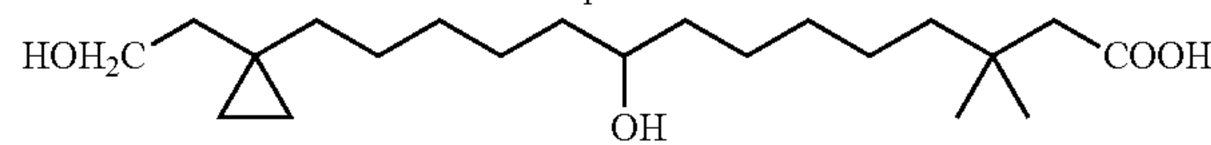
9-Hydroxy-14-[1-(2-hydroxy-ethyl)-cyclopropyl]-3,3-dimethyl-tetradecanoic acid
