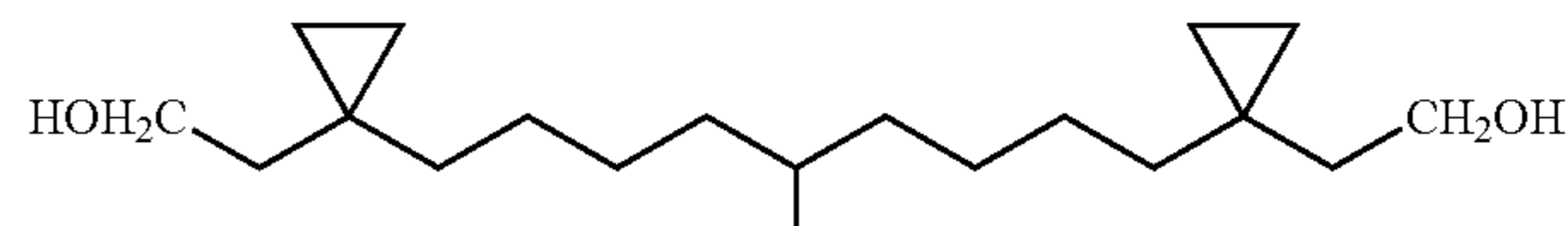
1,9-Bis-(2-hydroxy-ethyl)-cyclopropyl]-nonan-5-ol Compound 22
