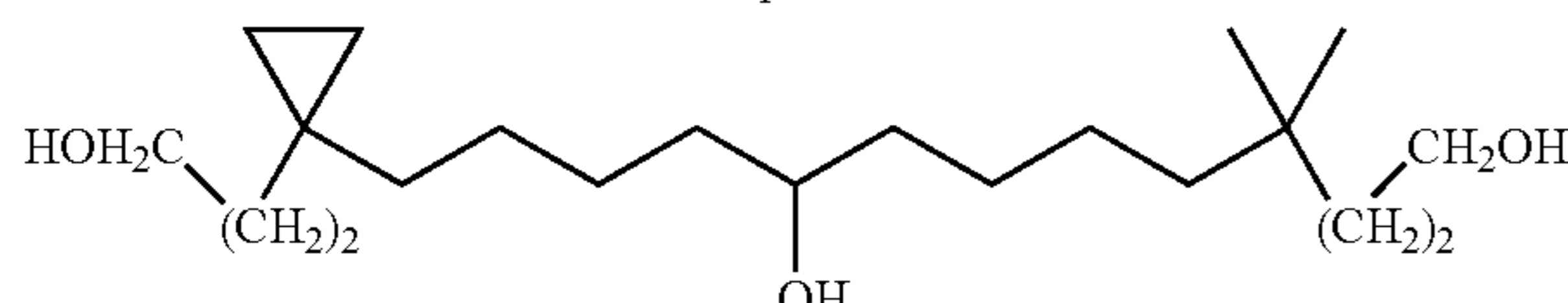
13-[1-(3-Hydroxy-propyl)-cyclopropyl]-4,4-dimethyl-tridecane-1,9-diol
