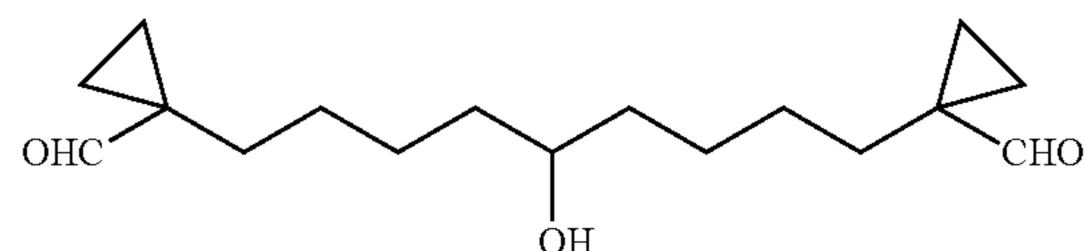
1,9-Bis-(1-oxa-cyclopropyl)-nonan-5-ol
