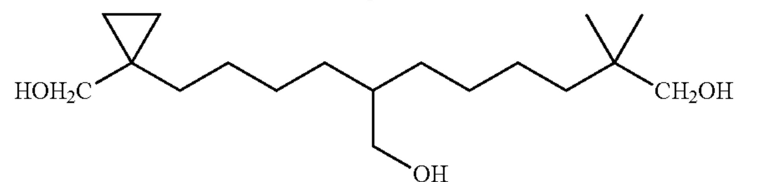
7-[4-(1-Hydroxymethyl-cyclopropyl)-butyl]-2,2-dimethyl-octane-1,8-diol
