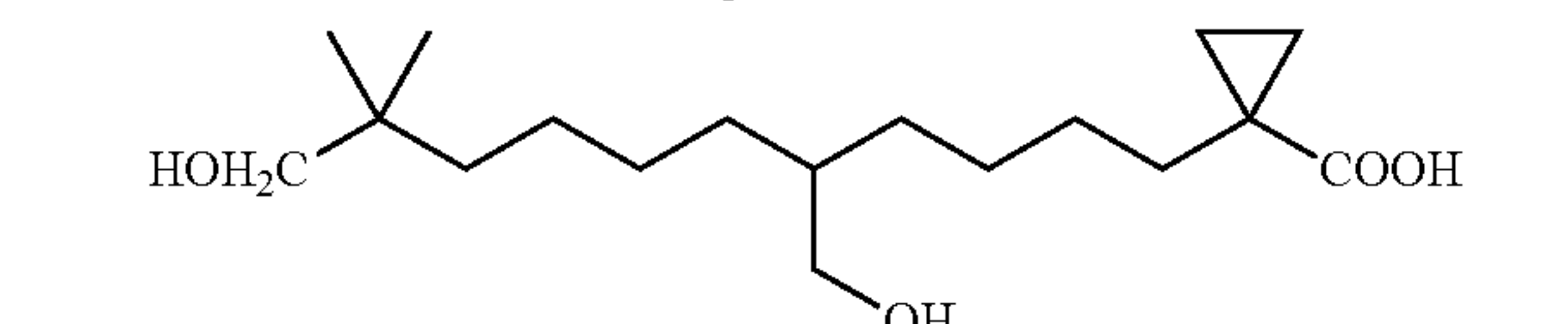
1-(11-Hydroxy-5-hydroxymethyl-10,10-dimethyl-undecyl)-cyclopropanecarboxylic acid
