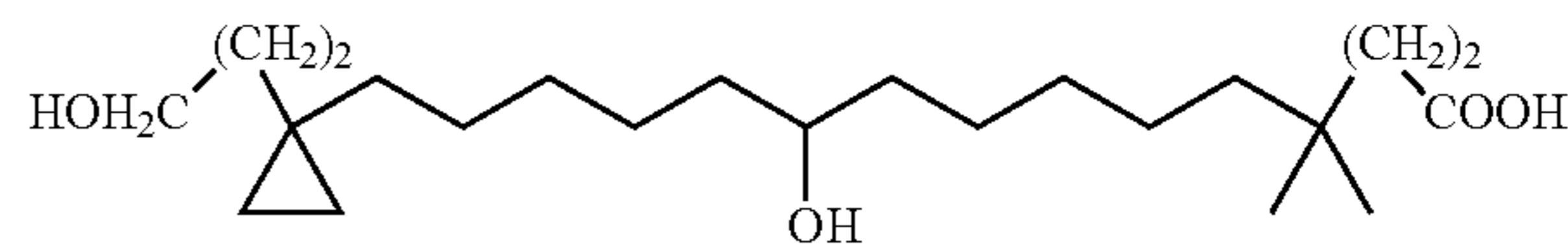
4,4-Dimethyl-10-hydroxy-15-[1-(3-hydroxy-propyl)-cyclopropyl]-pentadecanoic acid
