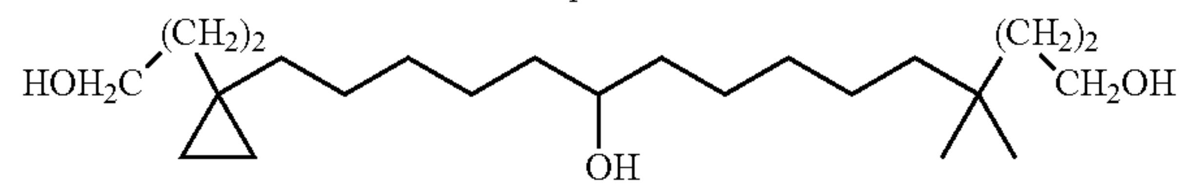
15-[1-(3-Hydroxy-propyl)-cyclopropyl]-4,4-dimethyl-pentadecane-1,10-diol
