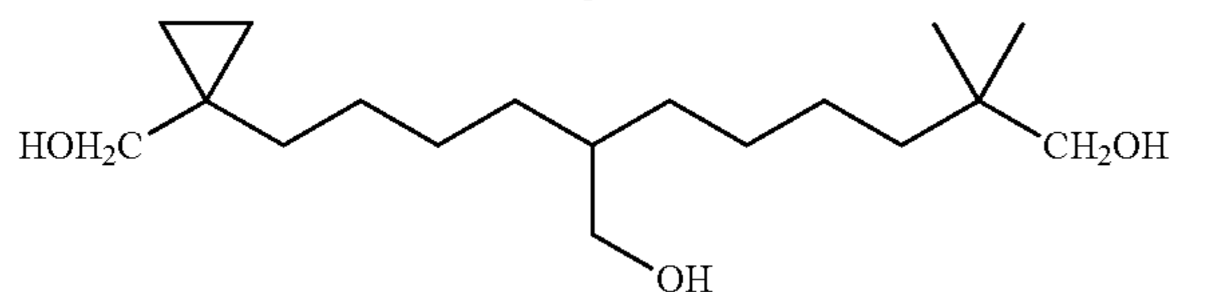
7-[4-(1-Hydroxymethyl-cyclopropyl)-butyl]-2,2-dimethyl-octane-1,8-diol
