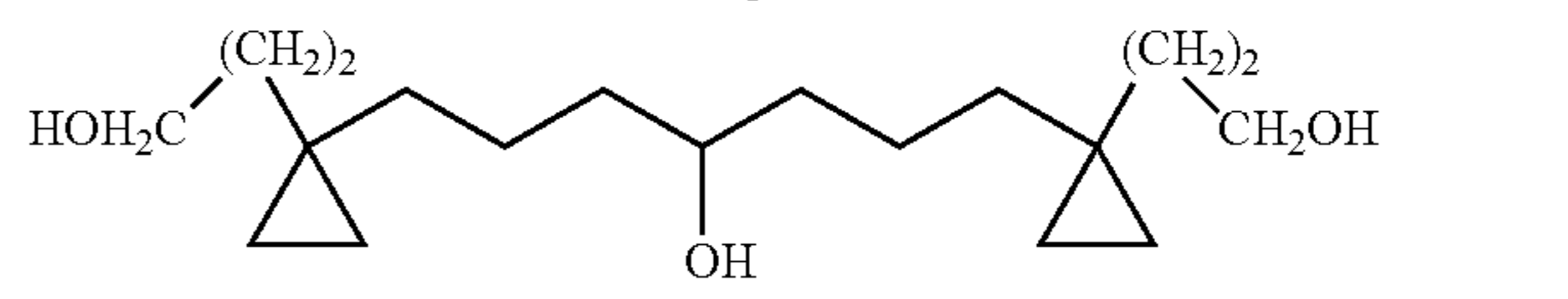
1,7-Bis-[1-(3-hydroxy-propyl)-cyclopropyl]-heptan-4-ol Compound 34
