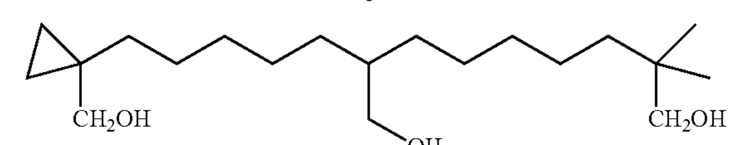
8-[5-(1-Hydroxymethyl-cyclopropyl)-pentyl]-2,2-dimethyl-nonane-1,9-diol
