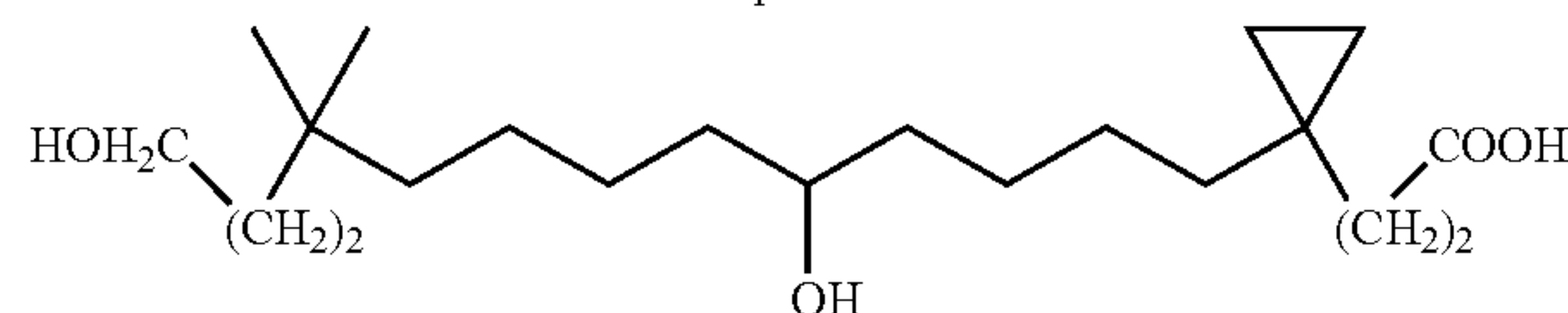
3-[1-(5,13-Dihydroxy-10,10-dimethyl-tridecyl)-cyclopropyl]-propionic acid
