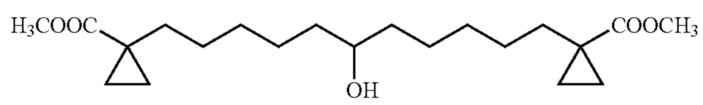
1,11-Bis-(1-carbomethoxy-cyclopropyl)-undecan-6-ol
