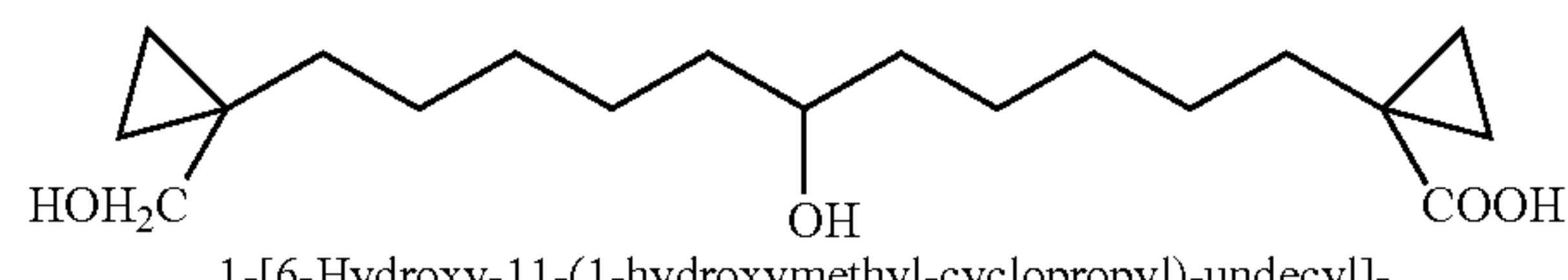
1-[6-Hydroxy-11-(1-hydroxymethyl-cyclopropyl)-undecyl]-cyclopropanecarboxylic acid
