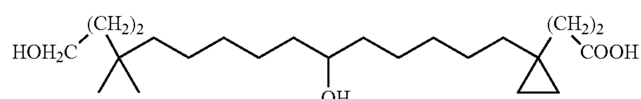
3-[1-(6,15-Dihydroxy-12,12-dimethyl-pentadecyl)-cyclopropyl]-propionic acid
