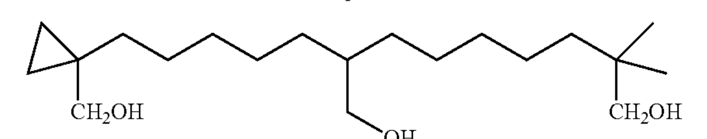
8-[5-(1-Hydroxymethyl-cyclopropyl)-pentyl]-2,2-dimethyl-nonane-1,9-diol
