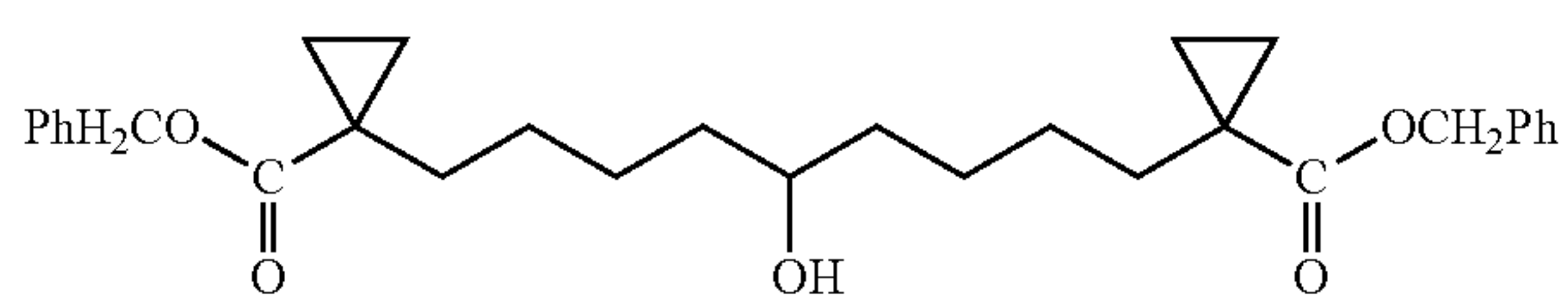
1,9-Bis-(1-benzyloxycarbonyl-cyclopropyl)-nonan-5-ol
