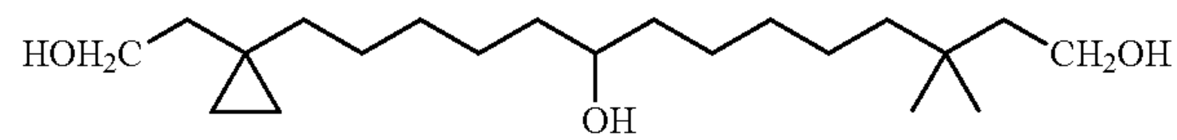
14-[1-(2-Hydroxy-ethyl)-cyclopropyl]-3,3-dimethyl-tetradecane-1,9-diol
