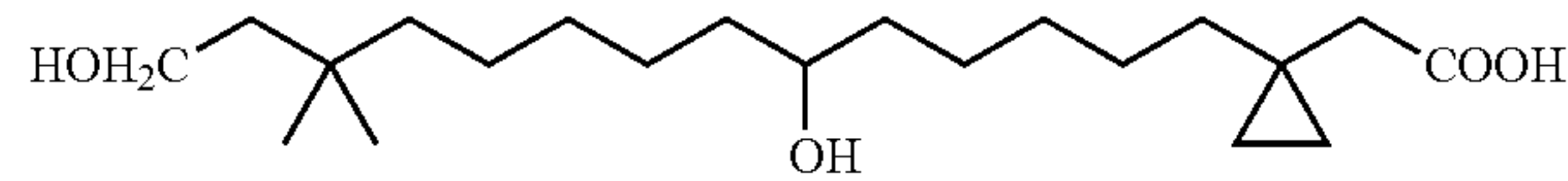
[1-(6,14-Dihydroxy-12,12-dimethyl-tetradecyl)-cyclopropyl]-acetic acid
