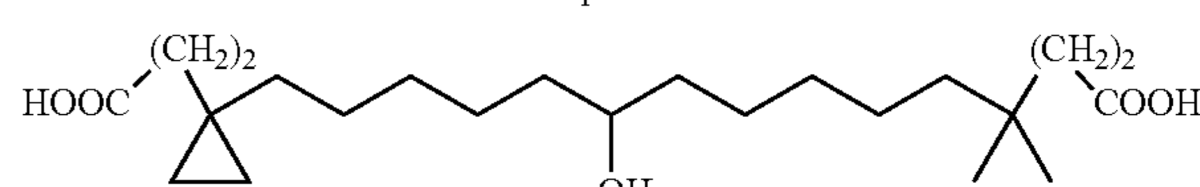
15-[1-(2-Carboxyethyl)-cyclopropyl]-10-hydroxy-4,4-dimethyl-tridecanoic acid
