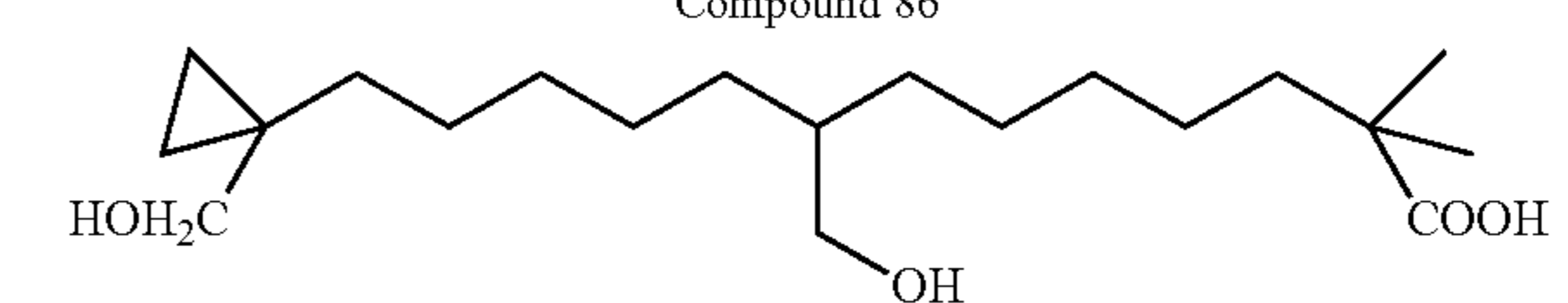
8-Hydroxymethyl-13-(1-hydroxymethyl-cyclopropyl)-2,2-dimethyl-tridecanoic acid
