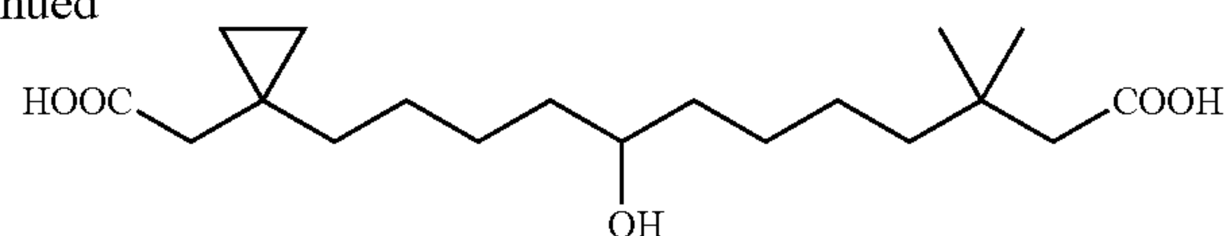
12-(1-Carboxymethyl-cyclopropyl)-8-hydroxy-3,3-dimethyl-dodecanoic acid
