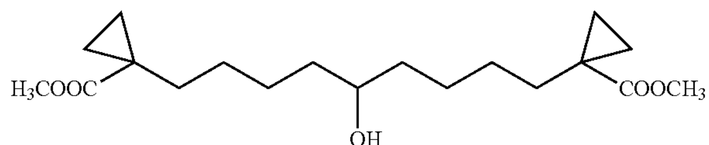
1,9-Bis-(1-carbomethoxy-cyclopropyl)-nonan-5-ol
