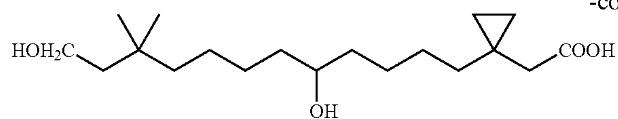
[1-(5,12-Dihydroxy-10,10-dimethyl-dodecyl)-cyclopropyl]-acetic acid
