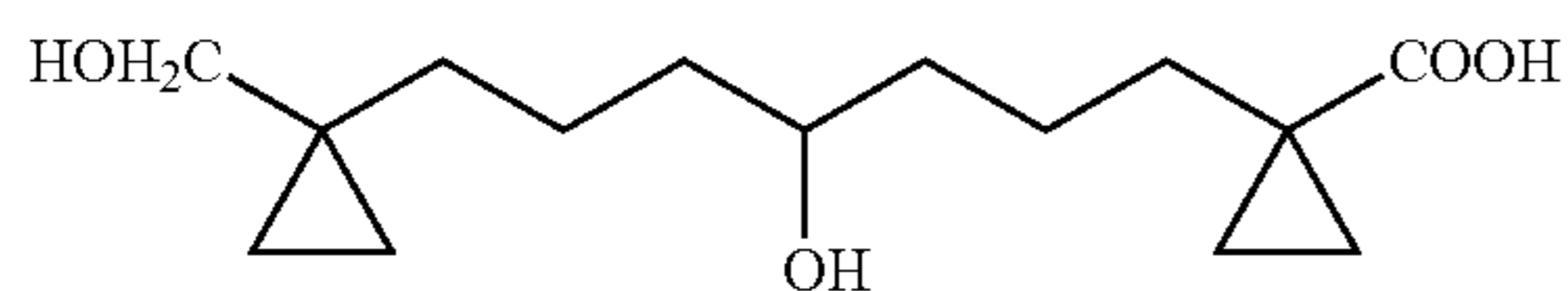
1-[4-Hydroxy-7-(1-hydroxymethyl-cyclopropyl)-heptyl]-cyclopropanecarboxylic acid
