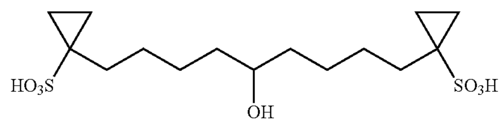
1,9-Bis-(1-sulfonyloxy-cyclopropyl)-nonan-5-ol
