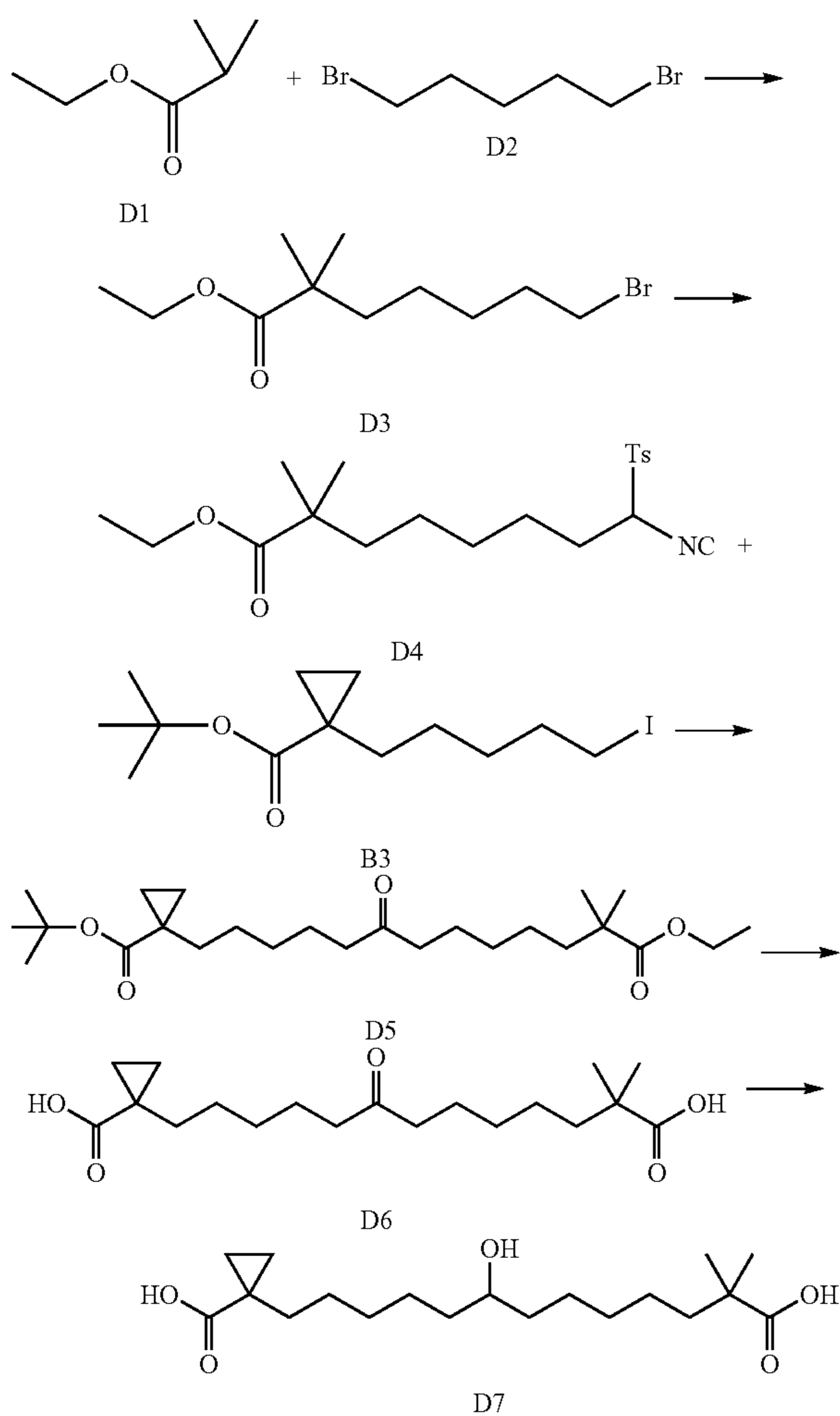
6.16 Ethyl 7-bromo-2,2-dimethylheptanoate
