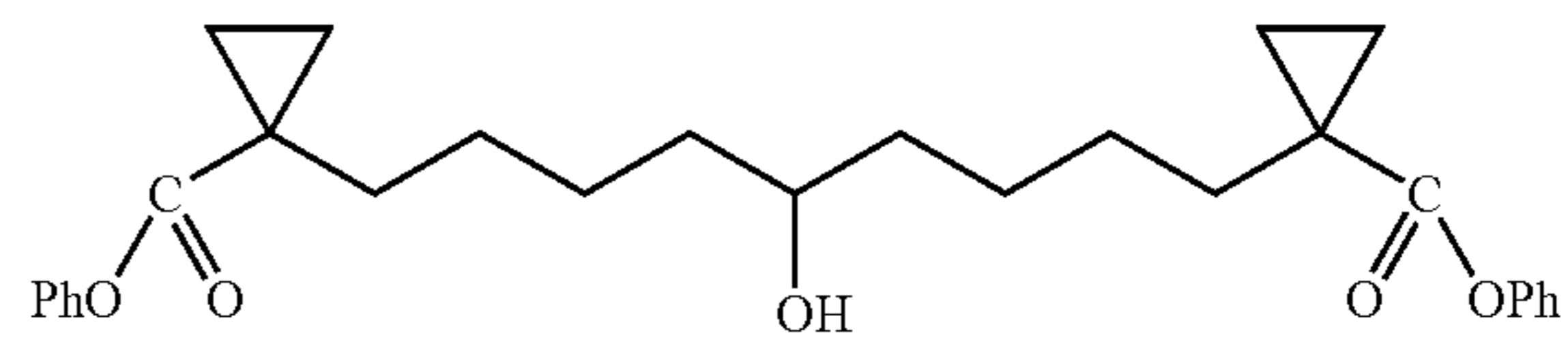
1,9-Bis-(1-phenoxy-carbonyl-cyclopropyl)-nonan-5-ol
