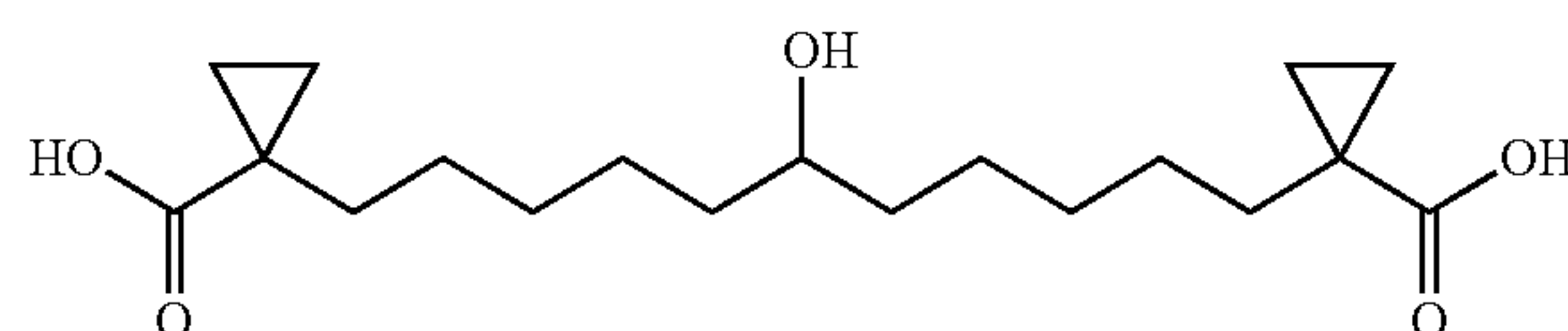
Compound B
