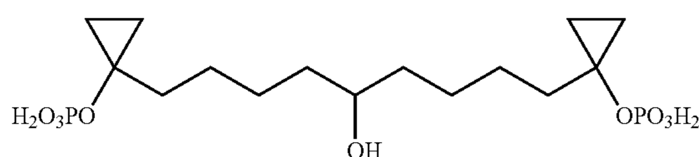
1,9-Bis-(1-phosphonoxy-cyclopropyl)-nonan-5-ol
