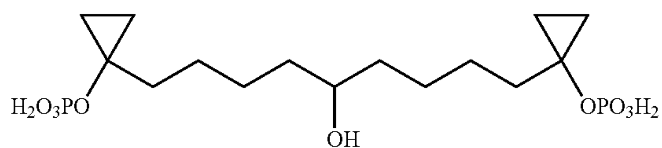
1,9-Bis-(1-phosphonoxy-cyclopropyl)-nonan-5-ol
