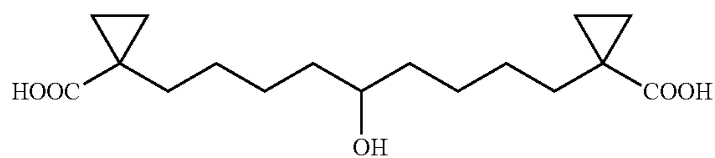
1,9-Bis-(1-carboxy-cyclopropyl)-nonan-5-ol
