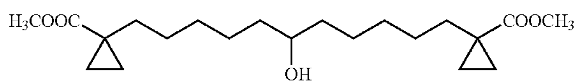
1,11-Bis-(1-carbomethoxy-cyclopropyl)-undecan-6-ol
