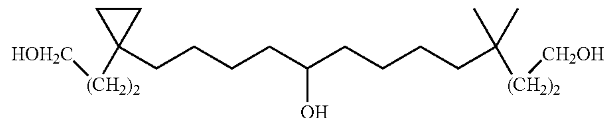
13-[1-(3-Hydroxy-propyl)-cyclopropyl]-4,4-dimethyl-tridecane-1,9-diol
