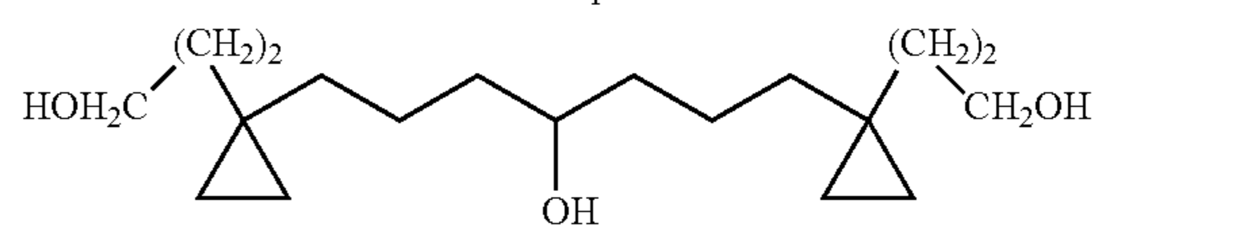
1,7-Bis-[1-(3-hydroxy-propyl)-cyclopropyl]-heptan-4-ol Compound 34
