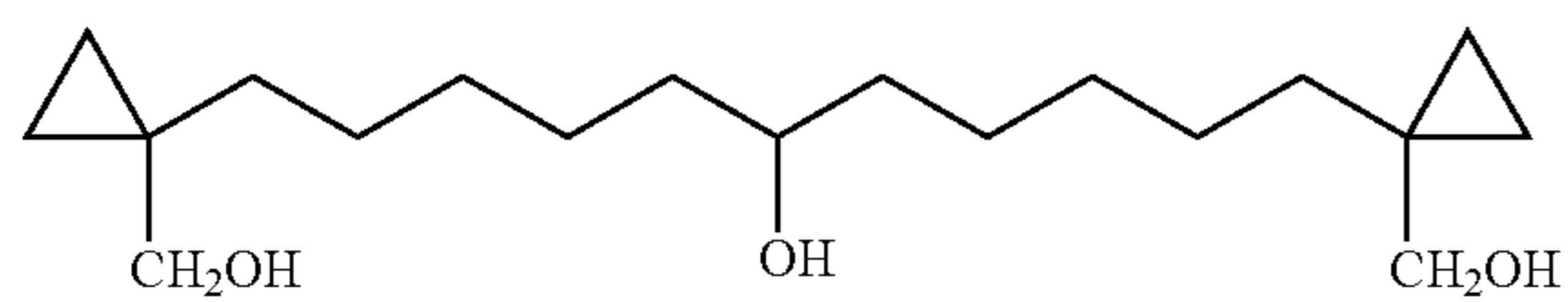
1,11-Bis-(1-hydroxymethyl-cyclopropyl)-undecan-6-ol
