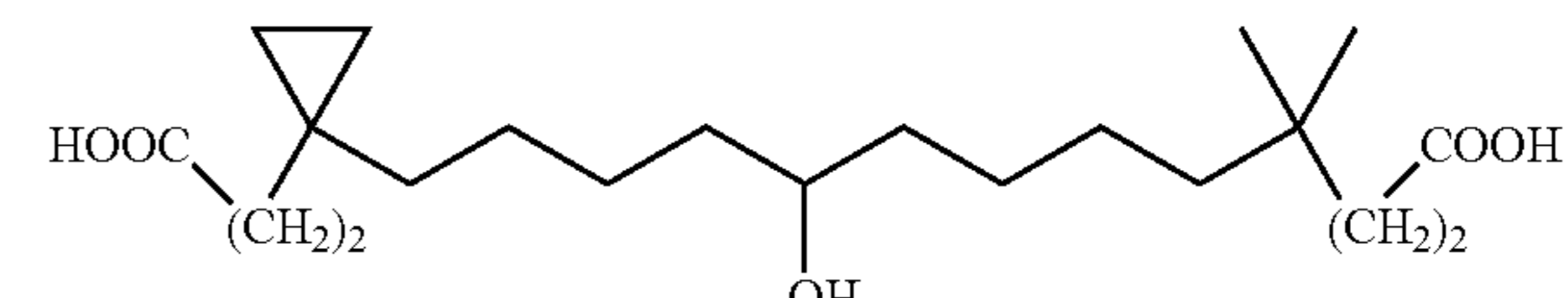
13-[1-(2-Carboxyethyl)-cyclopropyl]-9-hydroxy-4,4-dimethyl-tridecanoic acid Compound 78
