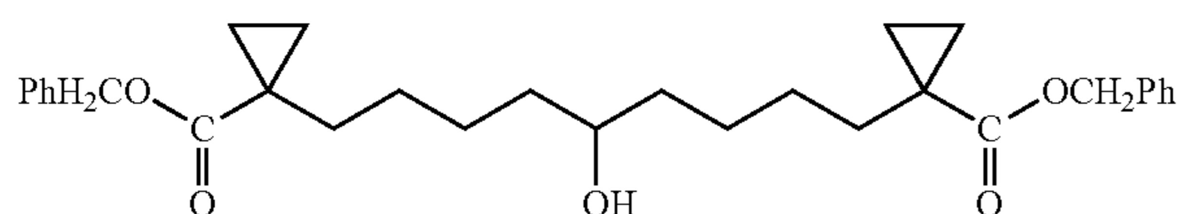
1,9-Bis-(1-benzyloxycarbonyl-cyclopropyl)-nonan-5-ol
