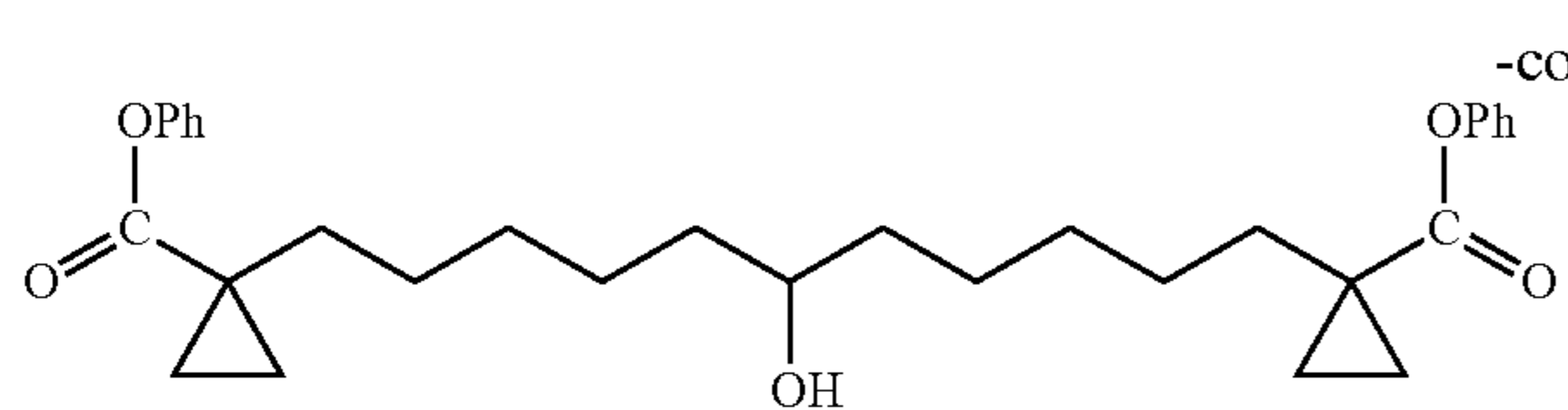
1,11-Bis-(1-phenoxy-carbonyl-cyclopropyl)-undecan-6-ol Compound 19
