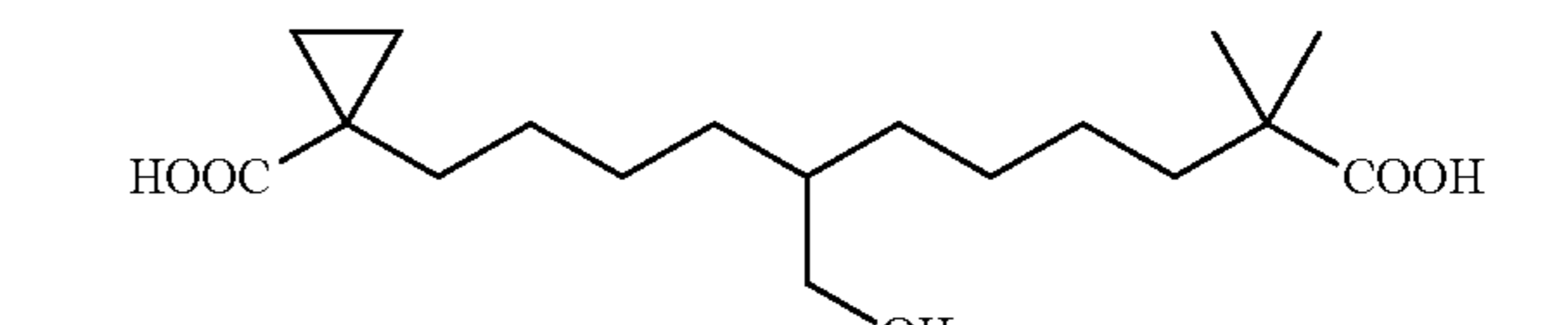
1-(1,0-Carboxy-5-hydroxymethyl-10-methyl-undecyl)-cyclopropanecarboxylic acid
