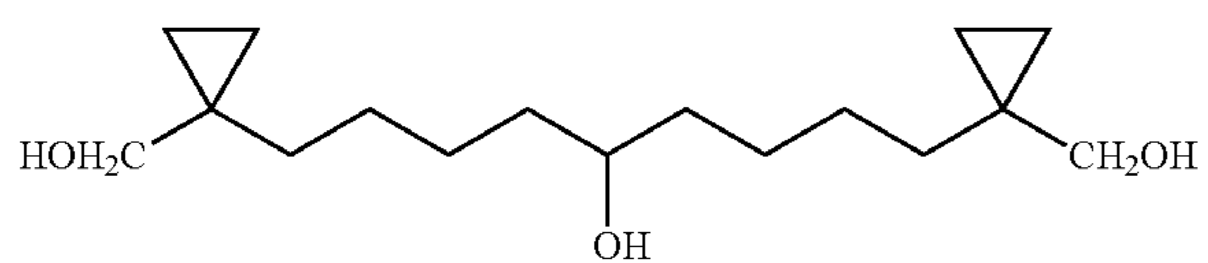
1,9-Bis-(1-hydroxymethyl-cyclopropyl)-nonan-5-ol
