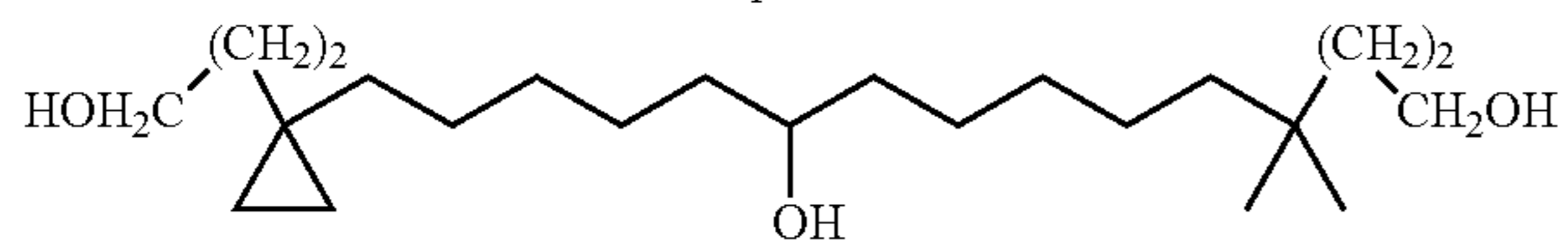
15-[1-(3-Hydroxy-propyl)-cyclopropyl]-4,4-dimethyl-pentadecane-1,10-diol
