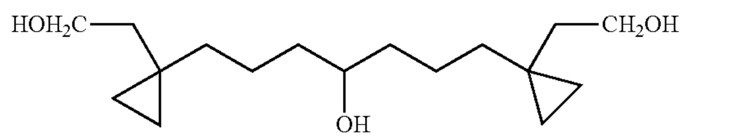
1,7-Bis-[1-(2-hydroxy-ethyl)-cyclopropyl]-heptan-4-ol Compound 25
