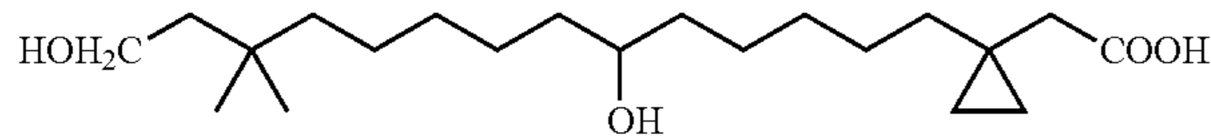
[1-(6,14-Dihydroxy-12,12-dimethyl-tetradecyl)-cyclopropyl]-acetic acid
