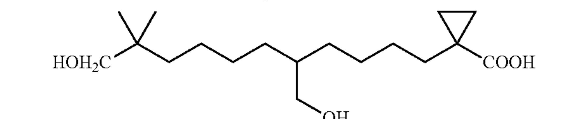
1-(11-Hydroxy-5-hydroxymethyl-10,10-dimethyl-undecyl)-cyclopropanecarboxylic acid
