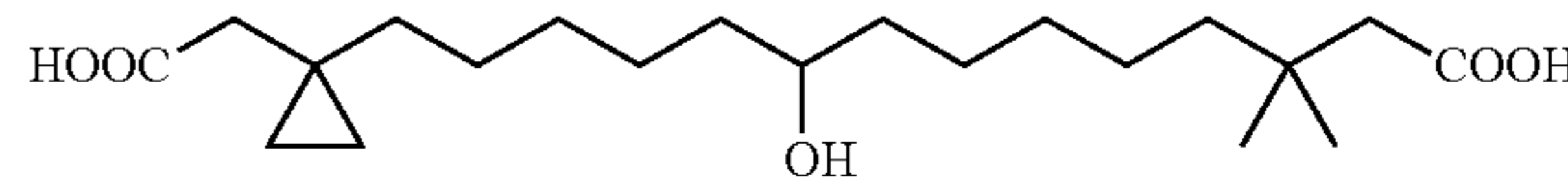
14-(1-Carboxymethyl-cyclopropyl)-9-hydroxy-3,3-dimethyl-tetradecanoic acid
