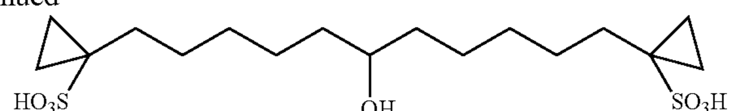
1,11-Bis-(1-sulfonyloxy-cyclopropyl)-undecan-6-ol Compound 20
