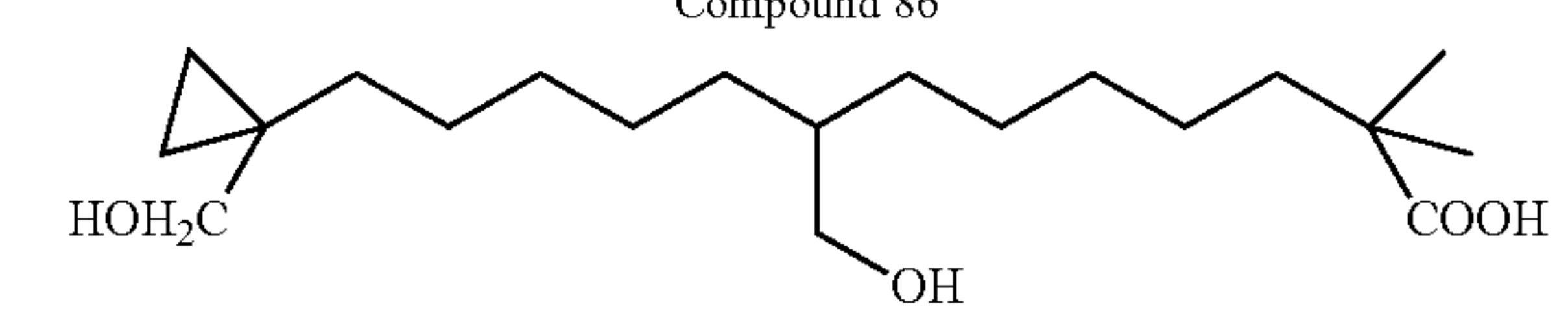
8-Hydroxymethyl-13-(1-hydroxymethyl-cyclopropyl)-2,2-dimethyl-tridecanoic acid
