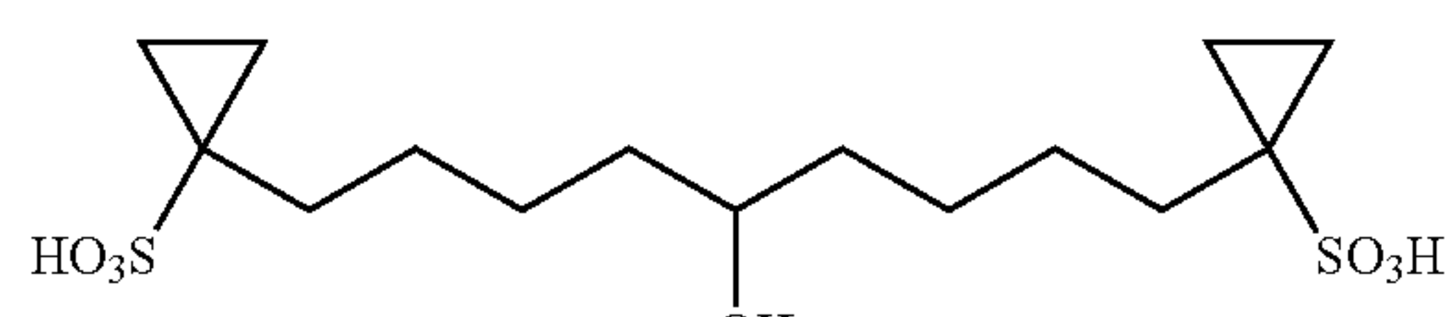
1,9-Bis-(1-sulfonyloxy-cyclopropyl)-nonan-5-ol
