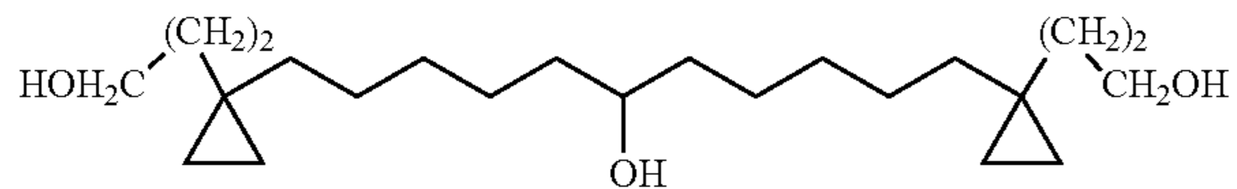
1,11-Bis-[1-(3-hydroxy-propyl)-cyclopropyl]-undecan-6-ol Compound 37
