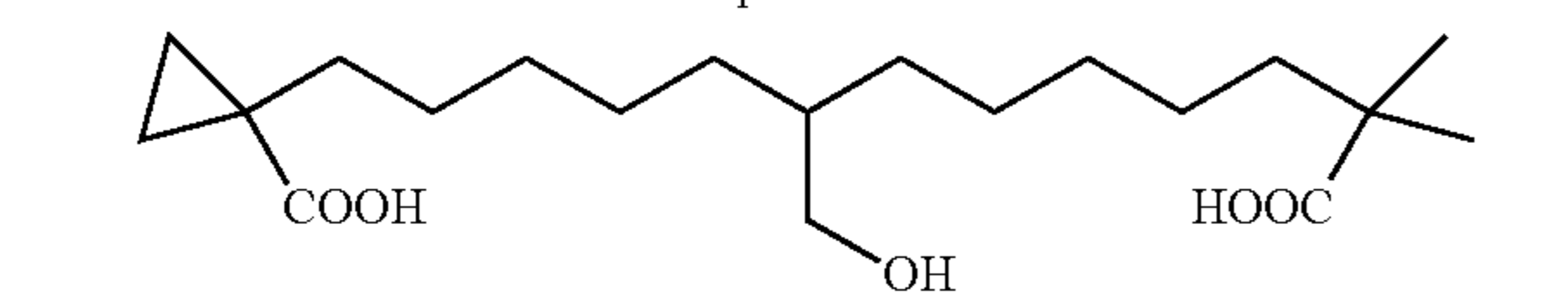
1-(12-Carboxy-6-hydroxymethyl-12-methyl-tridecyl)-cyclopropanecarboxylic acid
