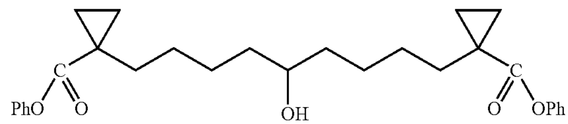
1,9-Bis-(1-phenoxy-carbonyl-cyclopropyl)-nonan-5-ol
