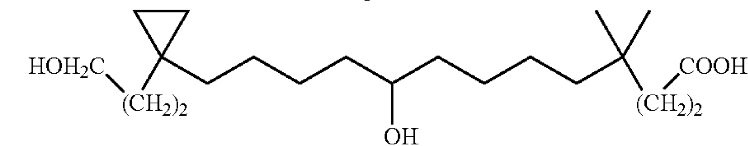
4,4-Dimethyl-9-hydroxy-13-[1-(3-hydroxypropyl)-cyclopropyl]-tridecanoic acid
