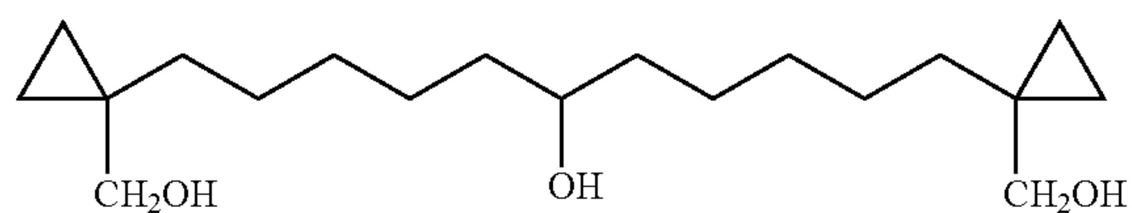
1,11-Bis-(1-hydroxymethyl-cyclopropyl)-undecan-6-ol
