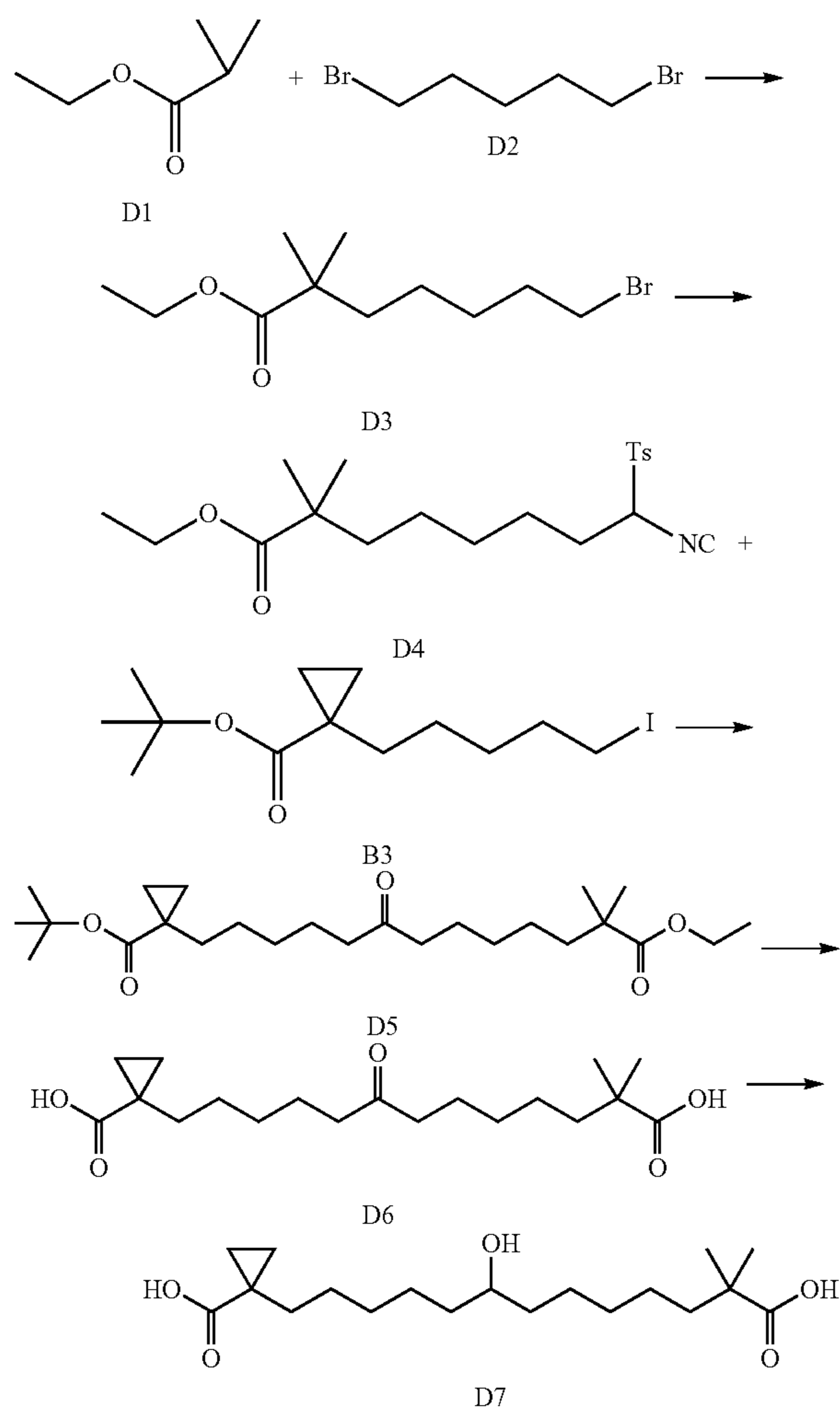
6.16 Ethyl 7-bromo-2,2-dimethylheptanoate
