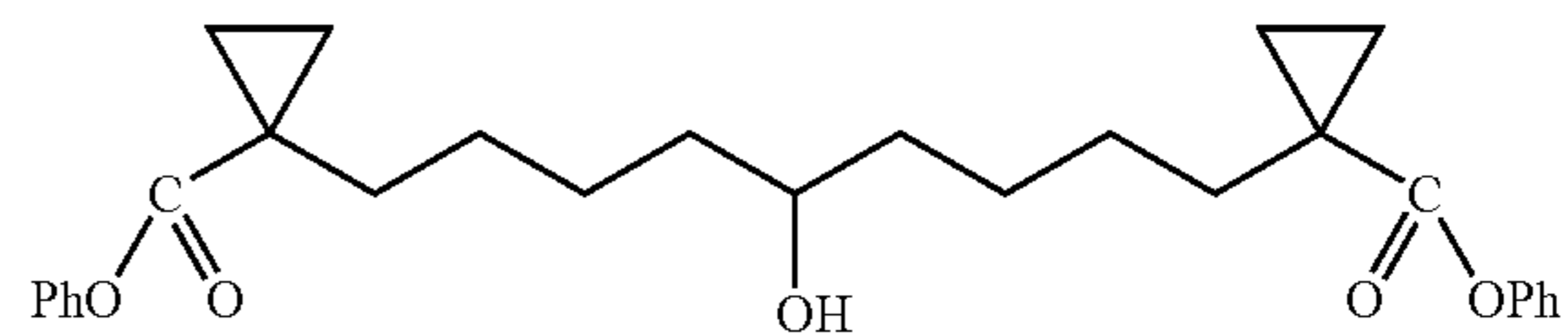
1,9-Bis-(1-phenoxy-carbonyl-cyclopropyl)-nonan-5-ol
