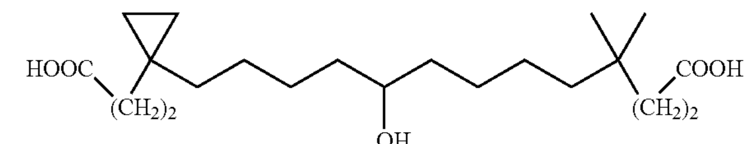
13-[1-(2-Carboxyethyl)-cyclopropyl]-9-hydroxy-4,4-dimethyl-tridecanoic acid
