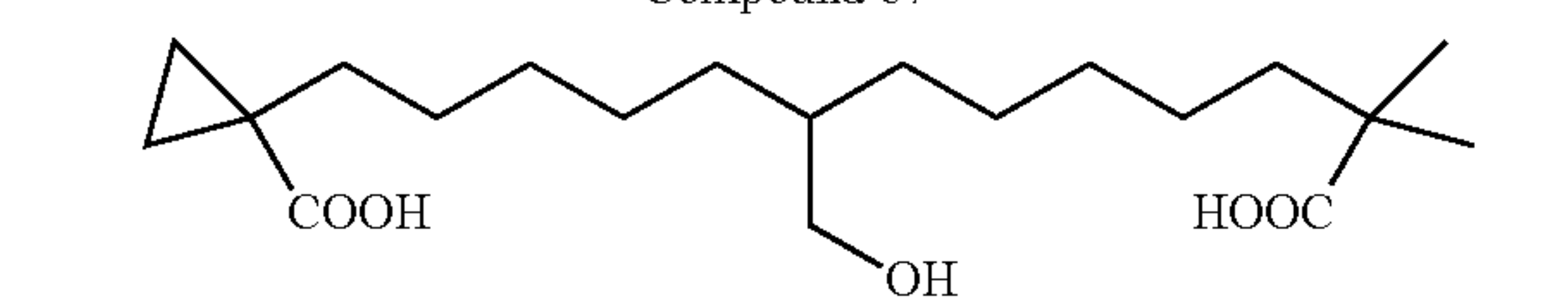
1-(12-Carboxy-6-hydroxymethyl-12-methyl-tridecyl)-cyclopropanecarboxylic acid
