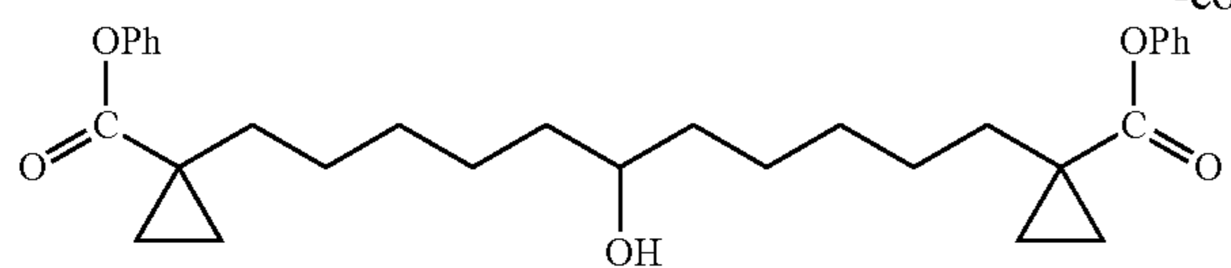
1,11-Bis-(1-phenoxy-carbonyl-cyclopropyl)-undecan-6-ol Compound 19
