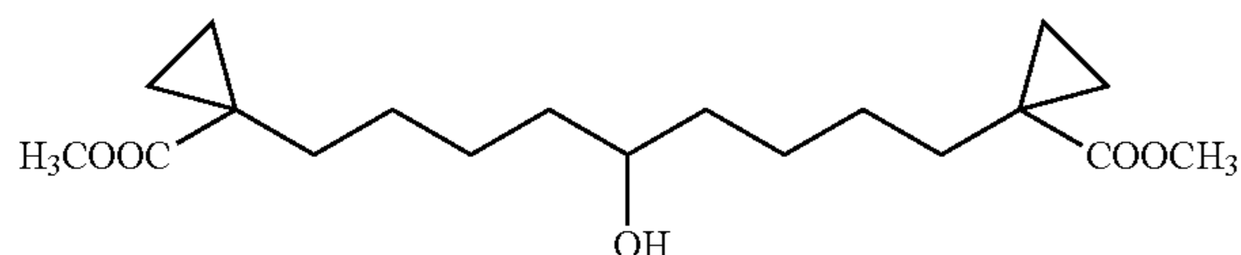
1,9-Bis-(1-carbomethoxy-cyclopropyl)-nonan-5-ol
