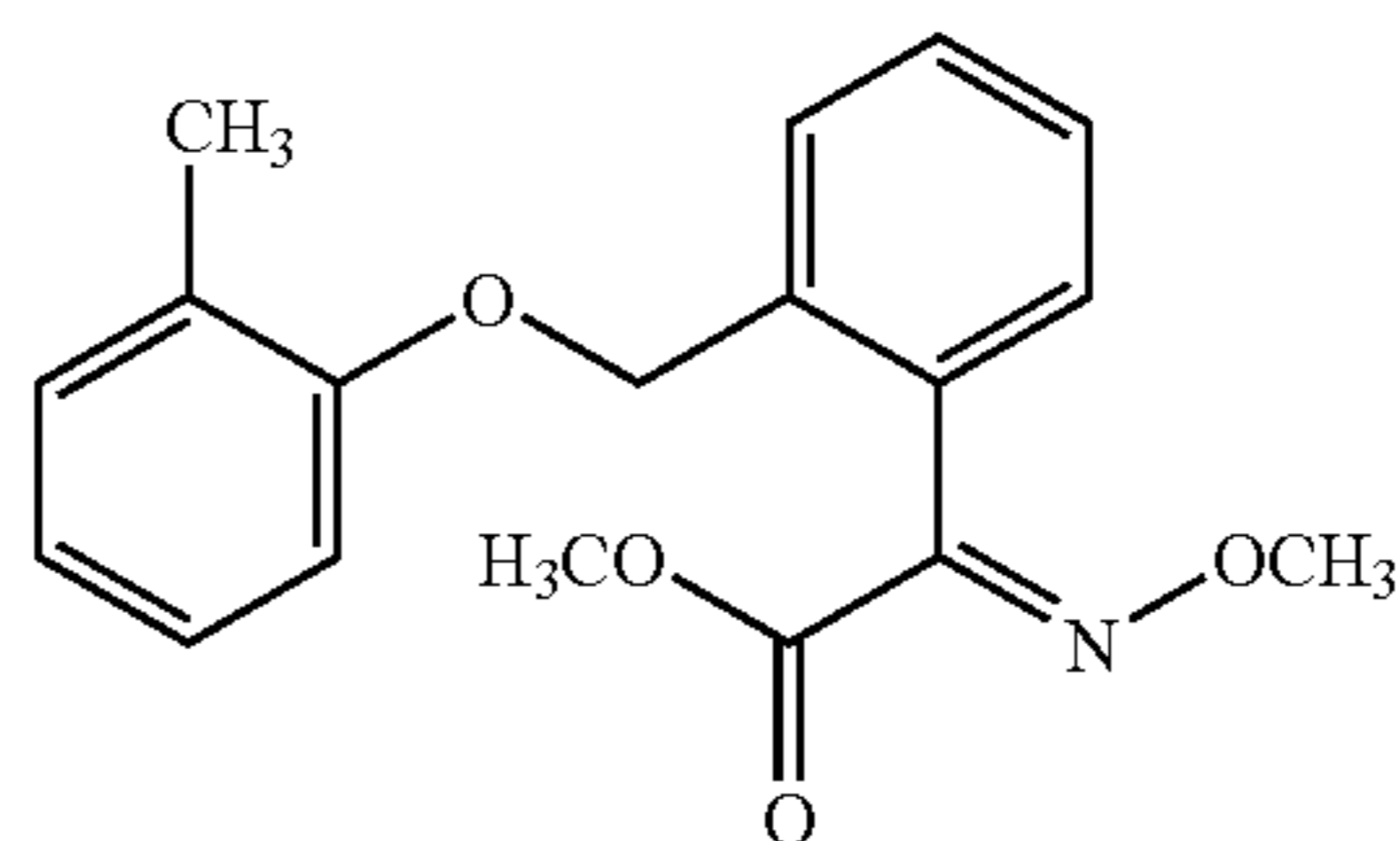
kresoxim-methyl
