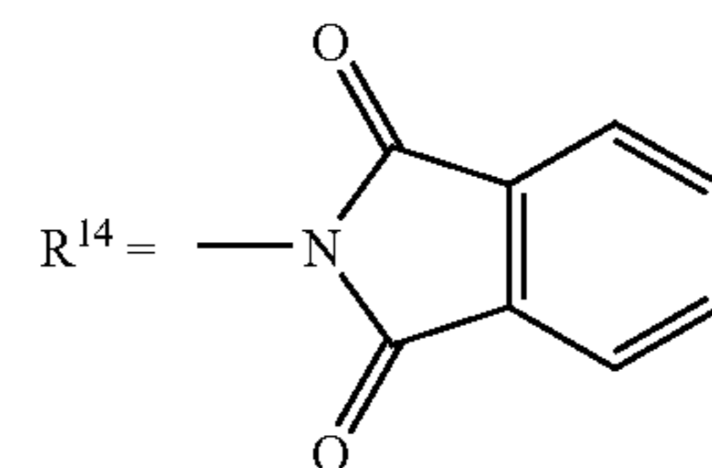
(FOLPET)
