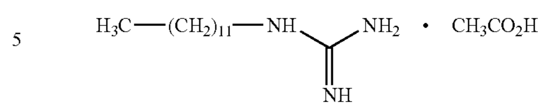
(DODINE)
