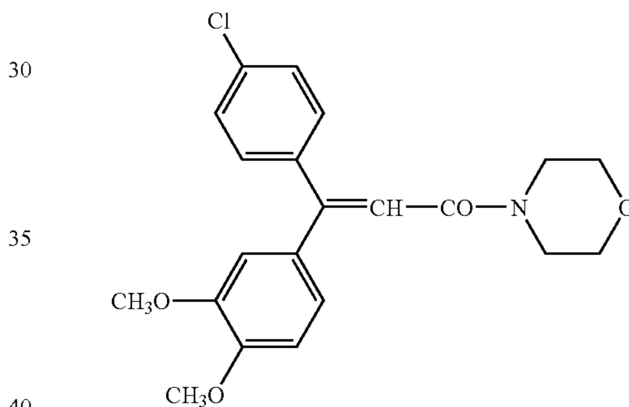
(DIMETHOMORPH)
