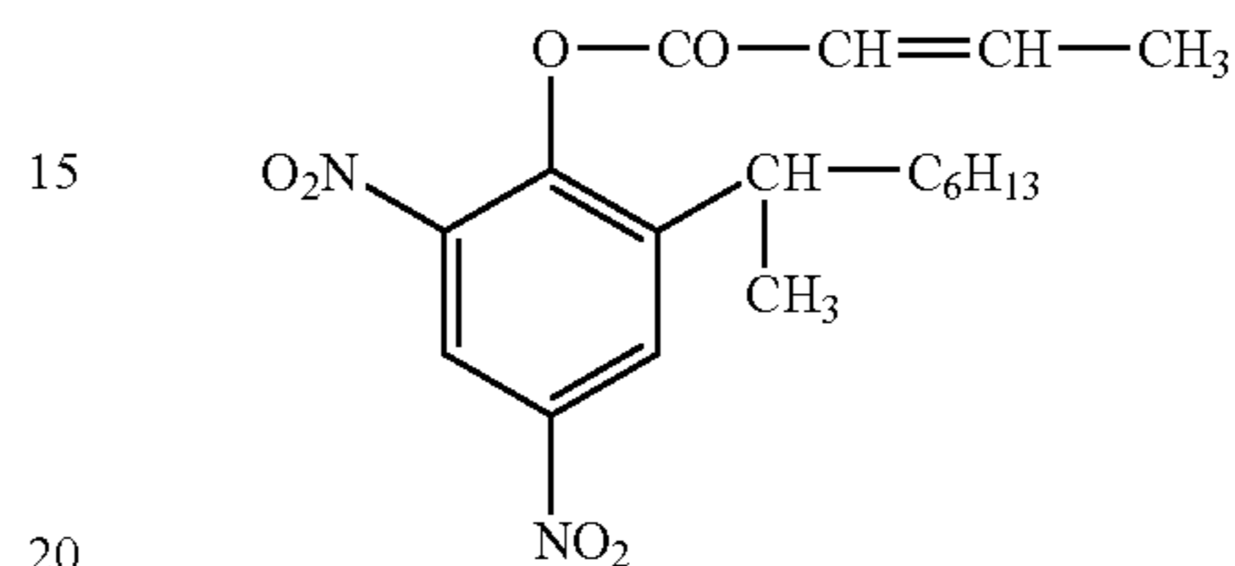
(DINOCAP)
