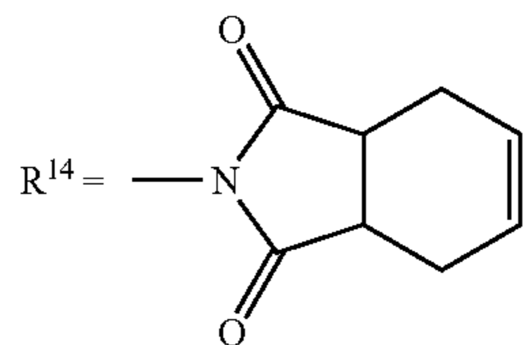
(CAPTAN)
