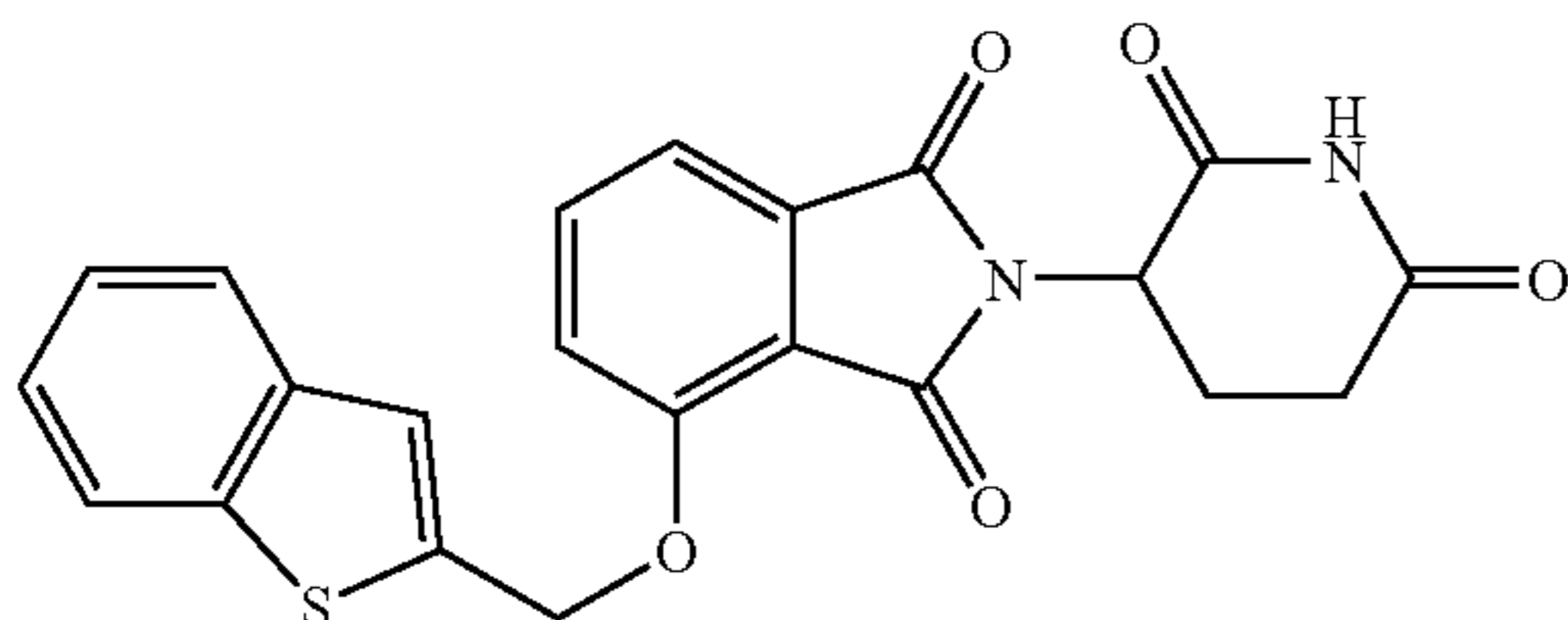
4-(Benzo[b]thiophen-2-ylmethoxy)-2-(2,6-dioxo-piperidin-3-yl)-isoindole-1,3-dione
