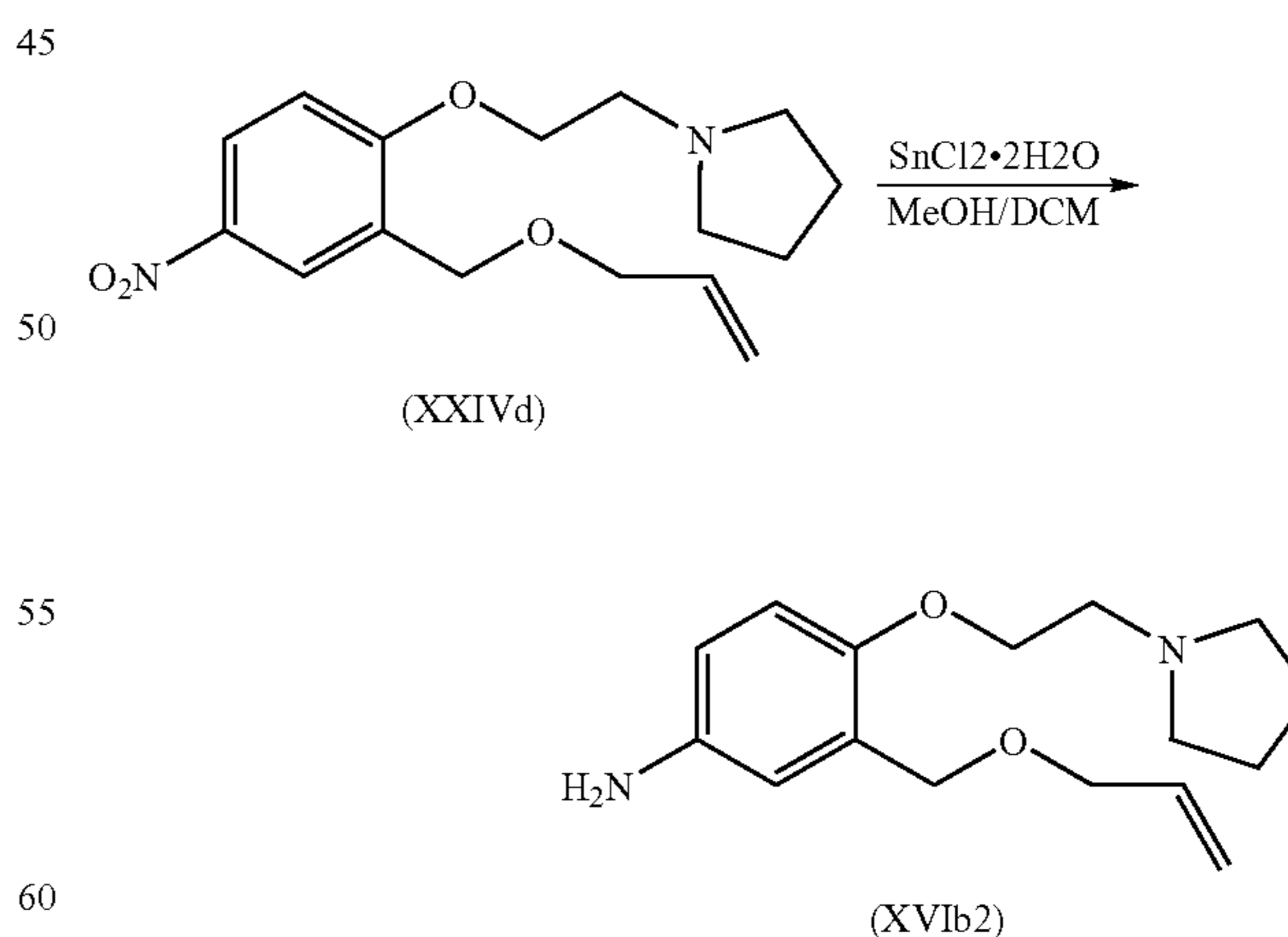
3-Allyloxymethyl-4-(2-pyrrolidin-1-yl-ethoxy)-phenylamine (XVIb2)
