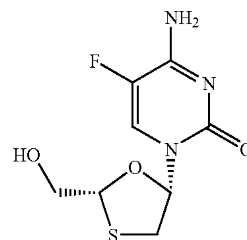
Emtricitabine
