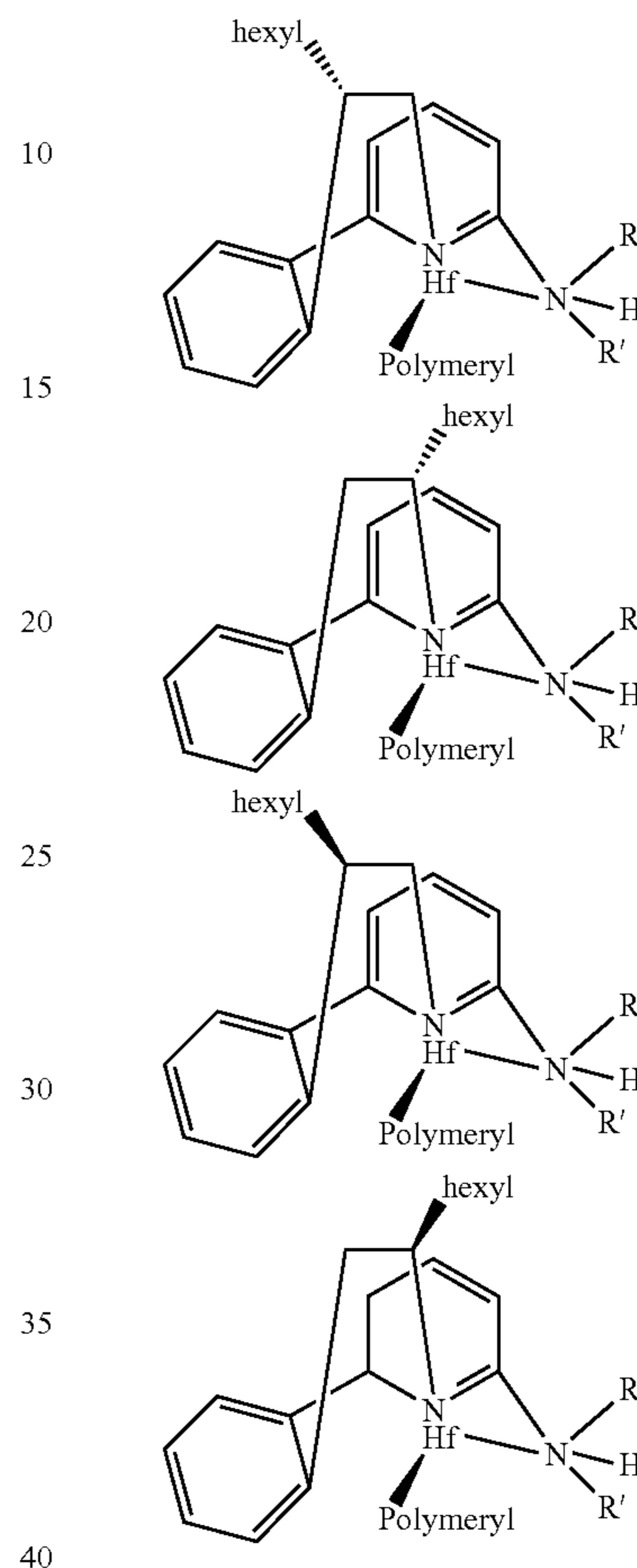
Diagram 2. Four possible octane inserted catalysts.
