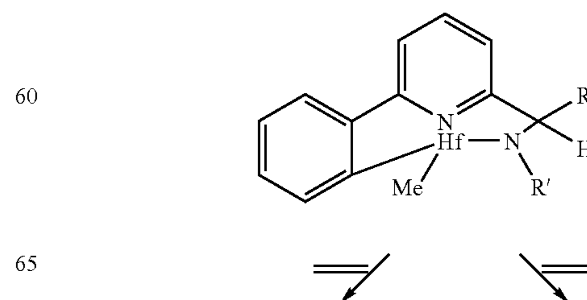
Diagram 3. Ethylene inserting into top and bottom faces of the initial catalyst. Whether these two products are different depends on the symmetry of the catalyst (groups at R and R').
