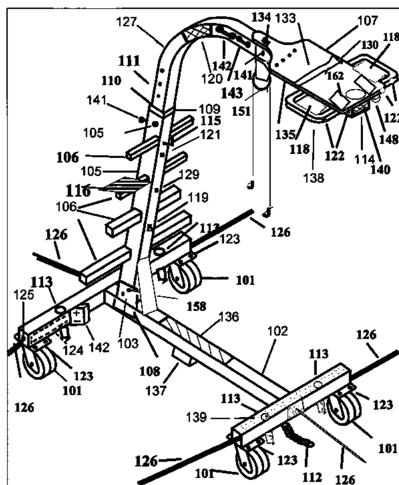
Preferred Embodiment of the Worker Support Stand
