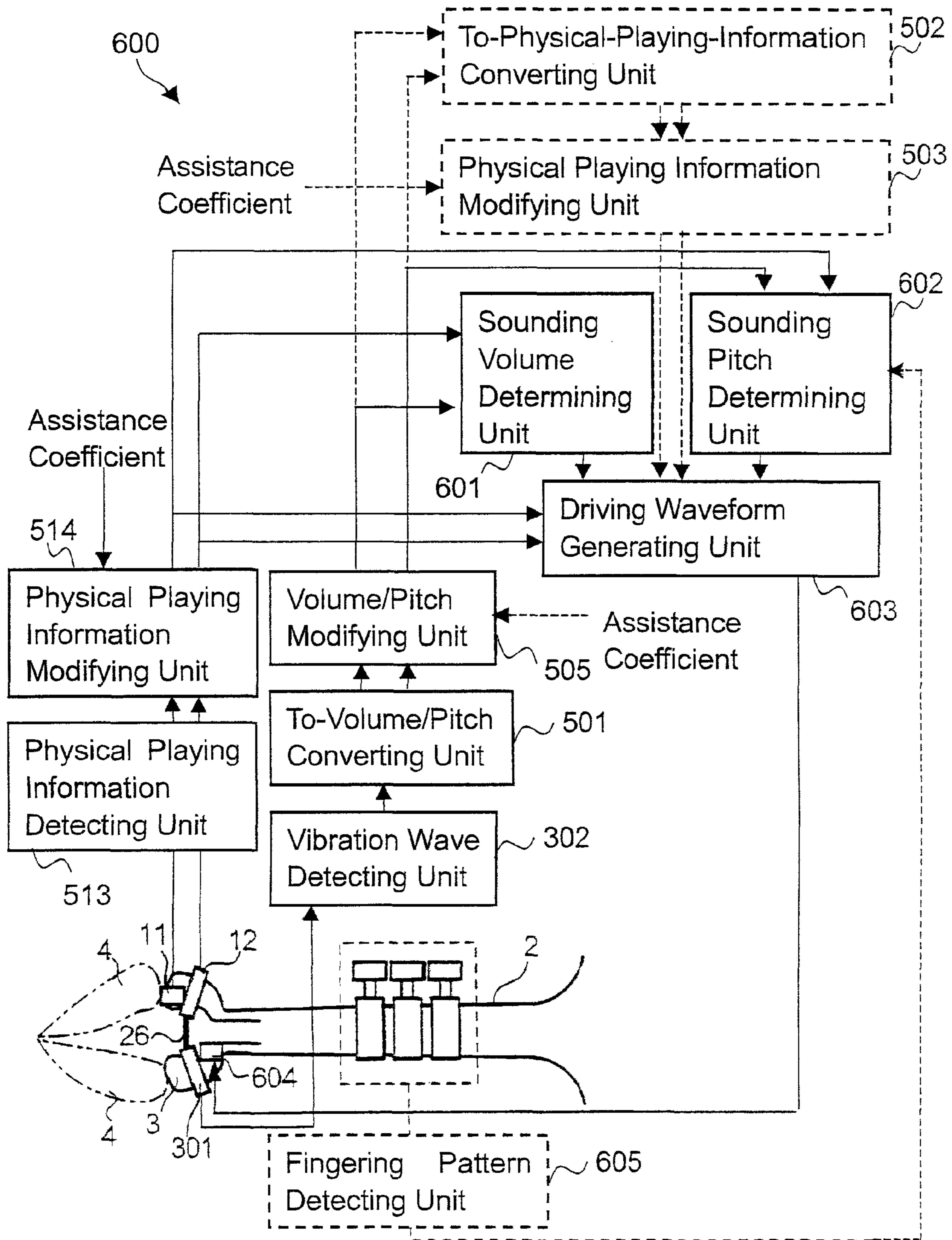
Fig. 9 Configuration of Assisting Apparatus
