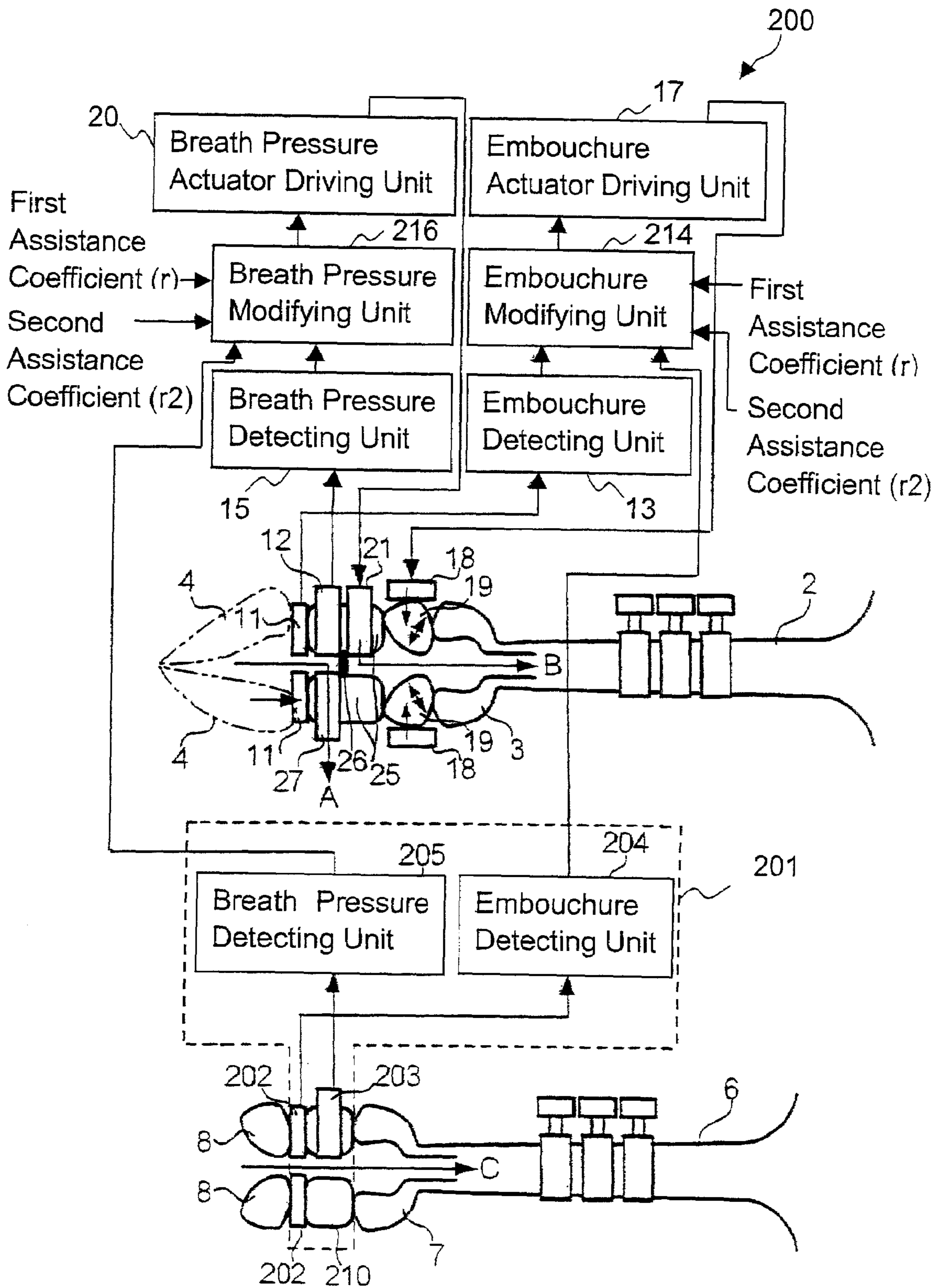
Fig. 3 Configuration of Assisting Apparatus
