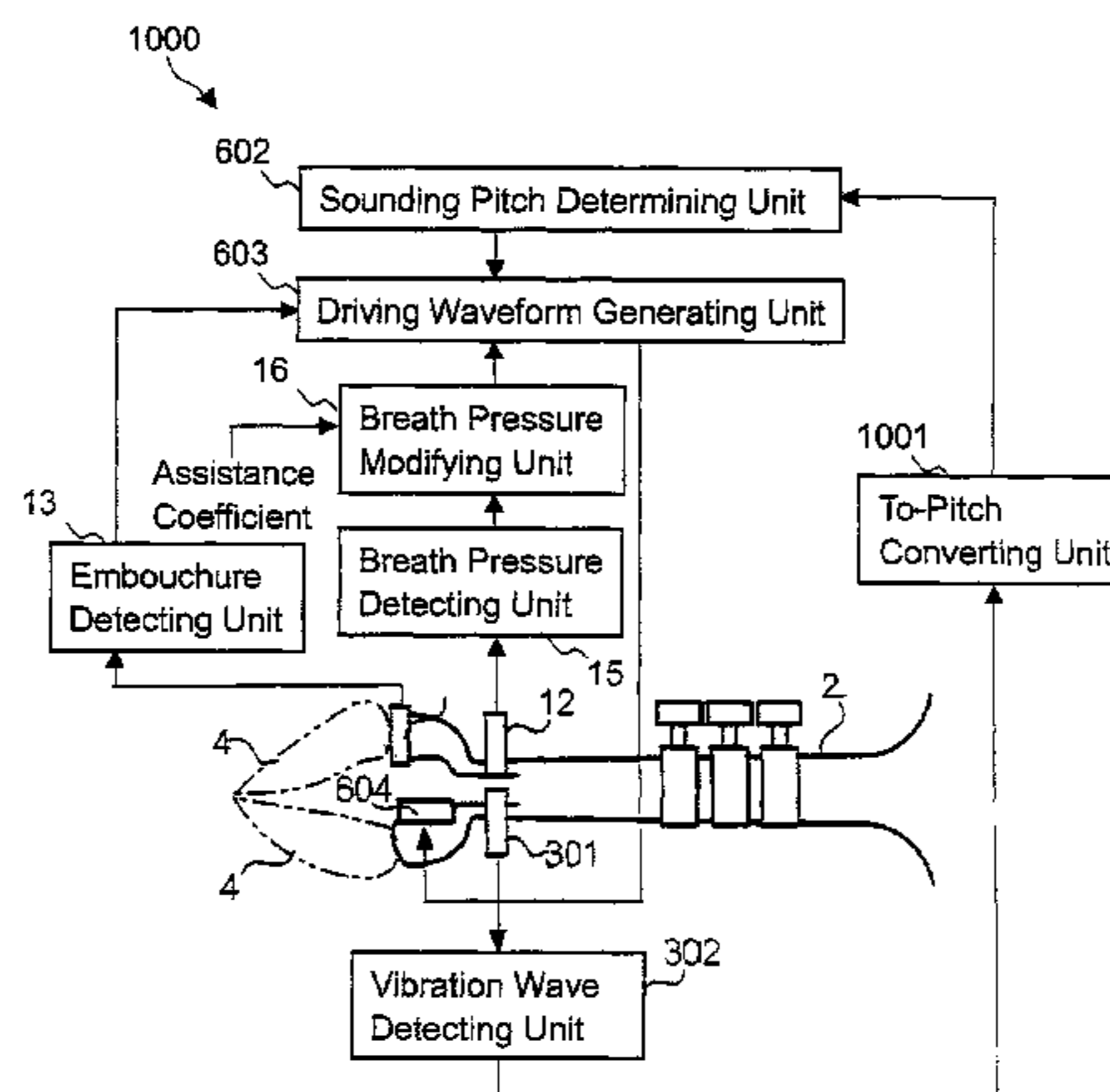
Configuration of Assisting Apparatus
