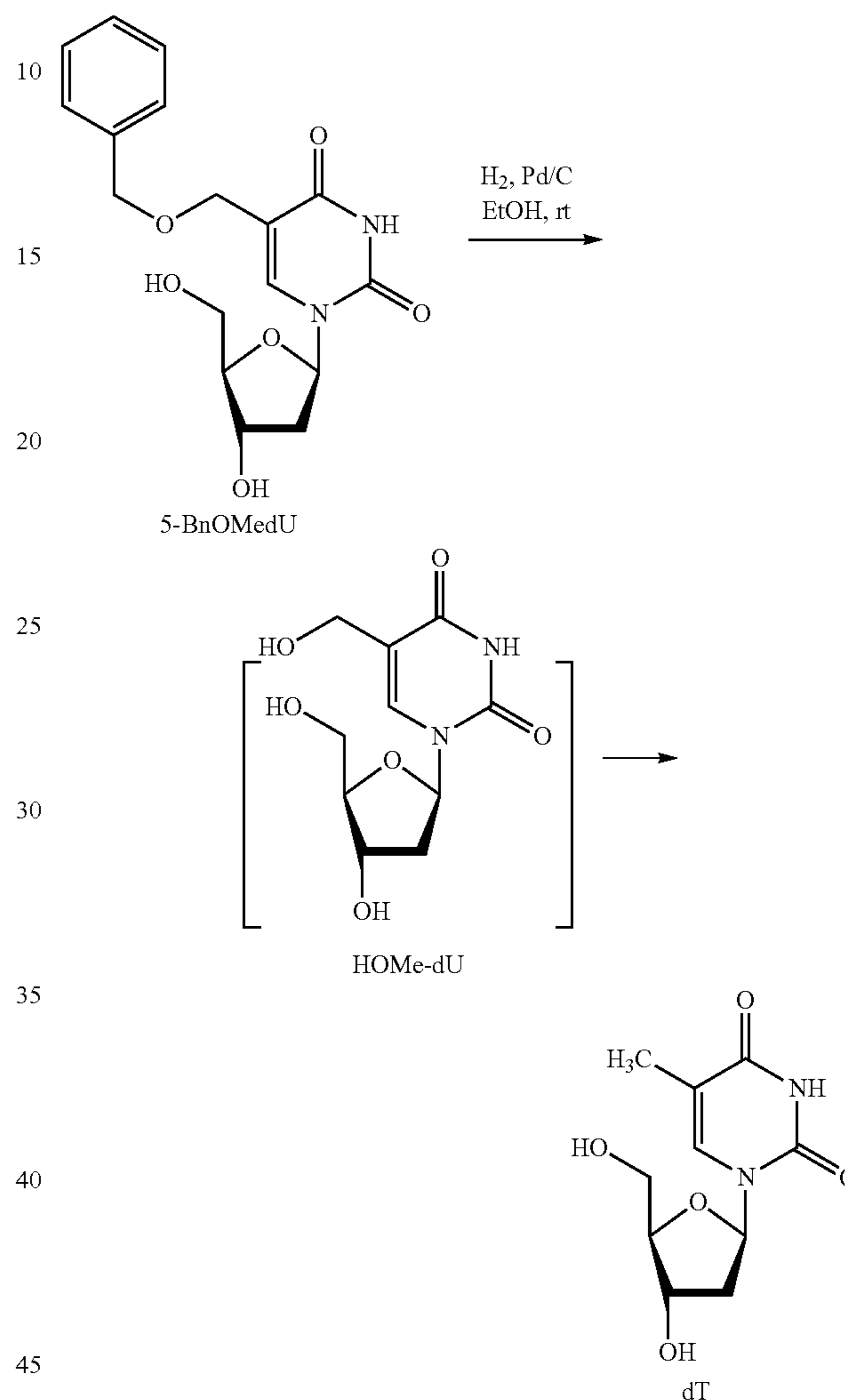
Scheme 42. Catalytic hydrogenolysis of 5-benzyloxymethyl-2'-deoxyuridine
