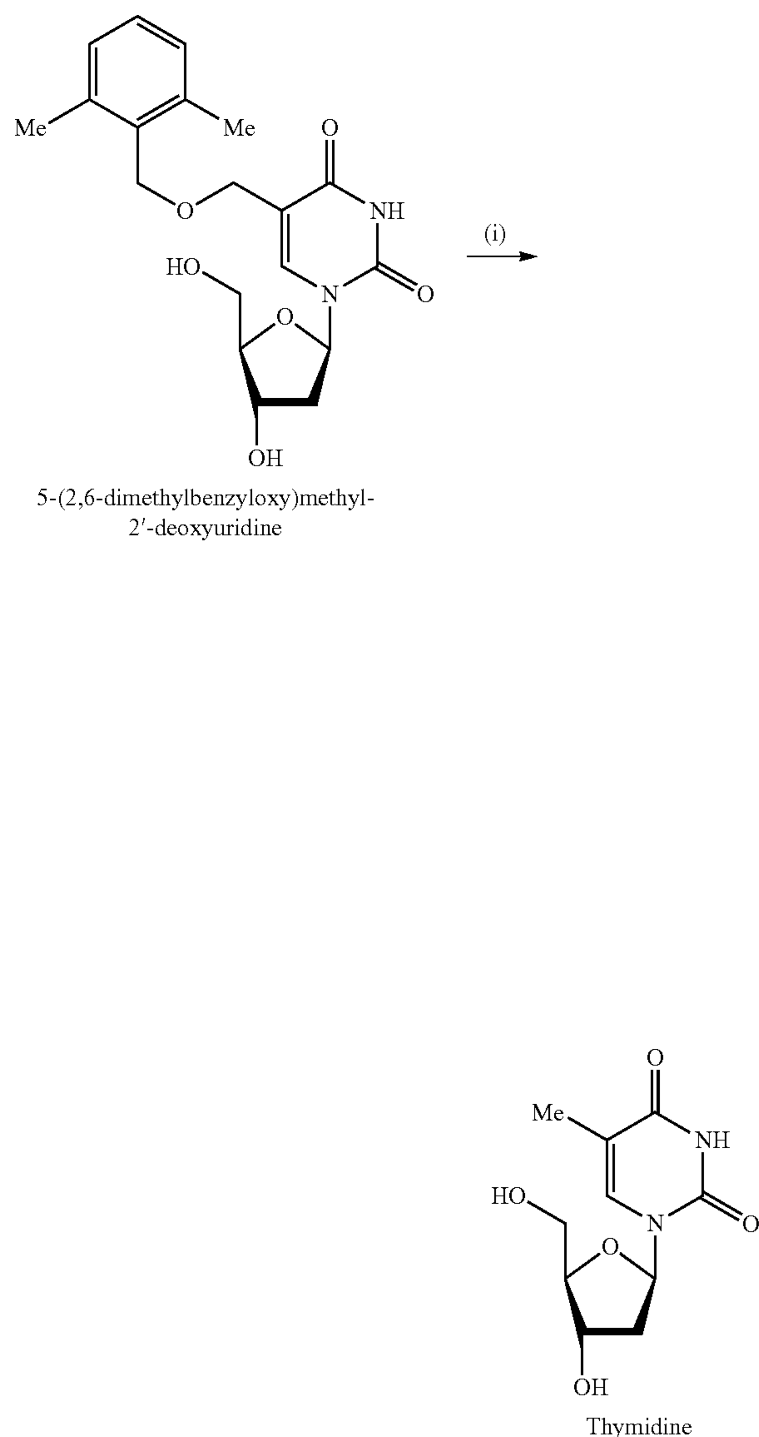
Scheme 41. Chemical cleavage of 5-(2,6-dimethylbenzyloxy)methyl-2'-deoxyuridine
