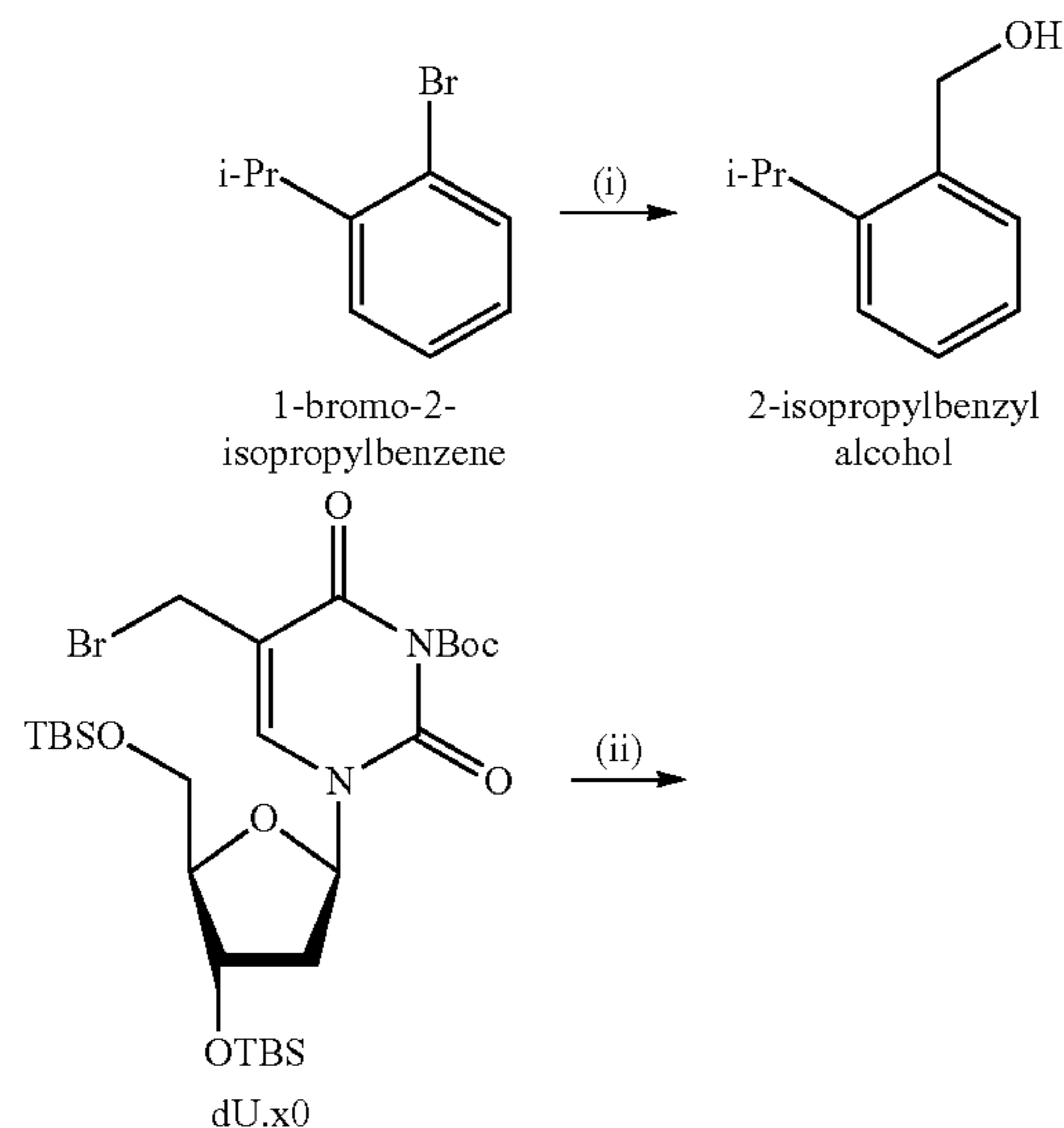
Scheme 33. Synthesis of 5-(2-isopropylbenzyloxy)methyl-2'-deoxyuridine-5'-triphosphate
