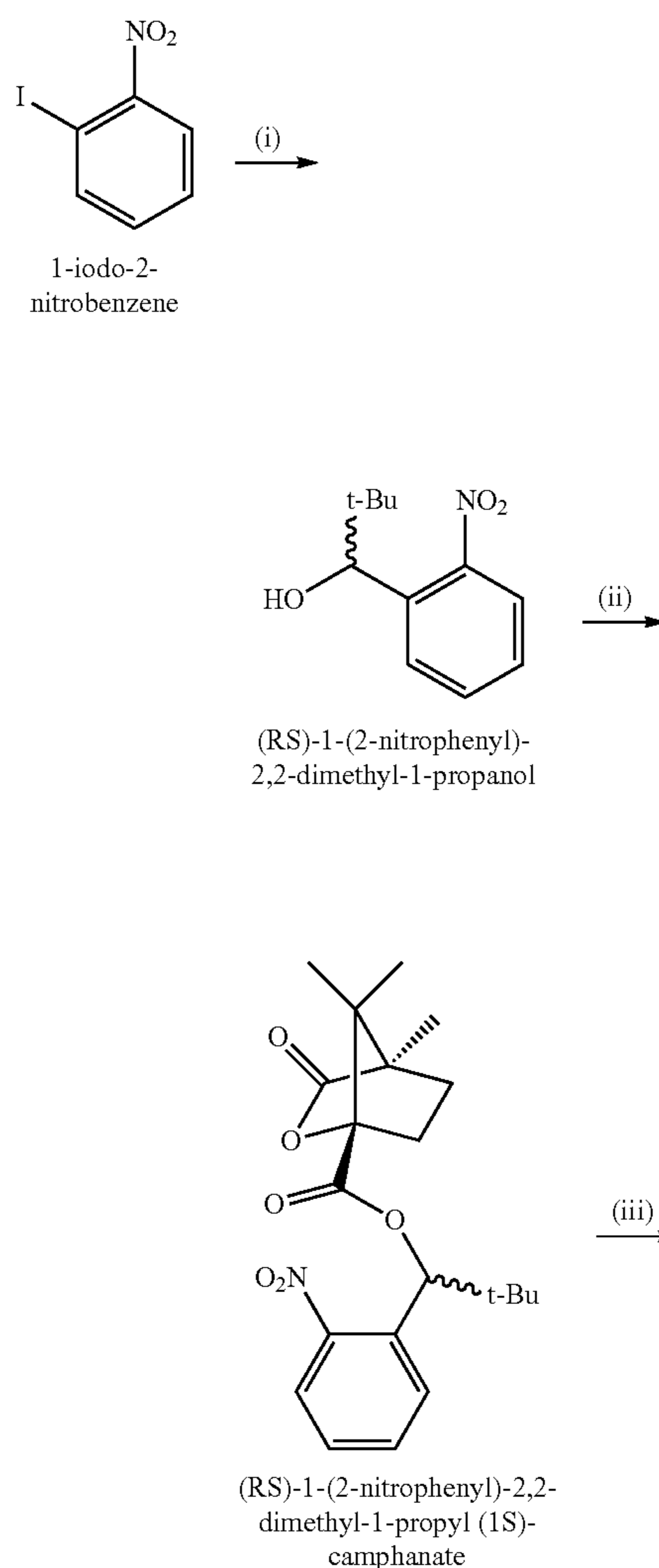
Scheme 5. Synthesis of (RS)-1-(2-nitrophenyl)-2,2-dimethyl-1-propanol and (R or S)-1-(2-nitrophenyl)-2,2-dimethyl-1-propanol.
