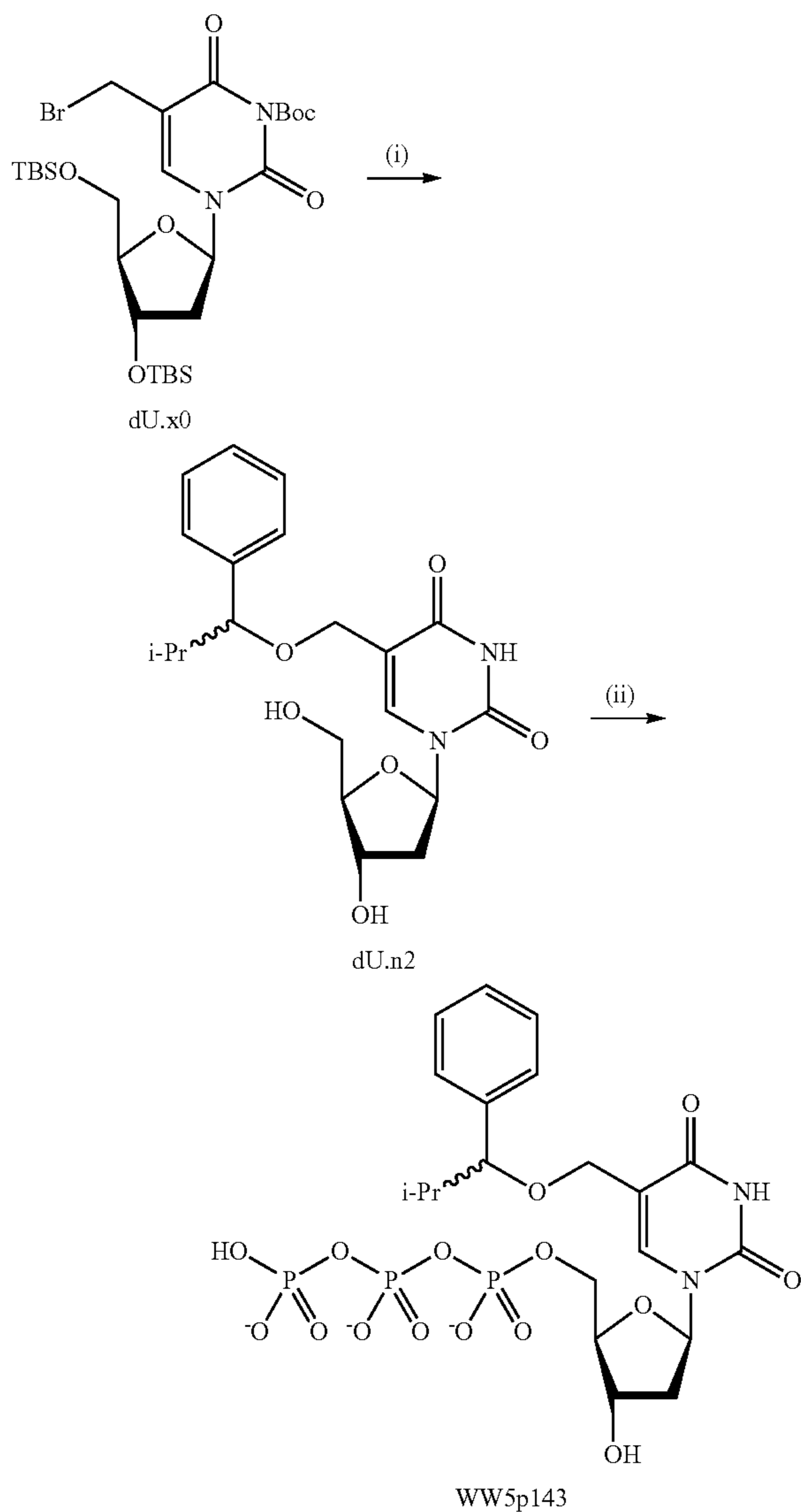
Scheme 31. Synthesis of 5-(1-phenyl-2-methyl-propyloxy)methyl-2'-deoxyuridine-5'-triphosphate.
