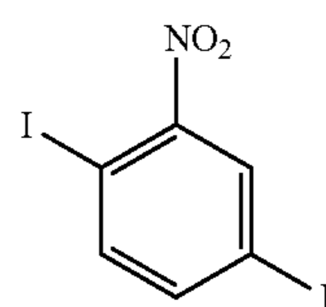
1,4-diiido-2-nitrobenzene
