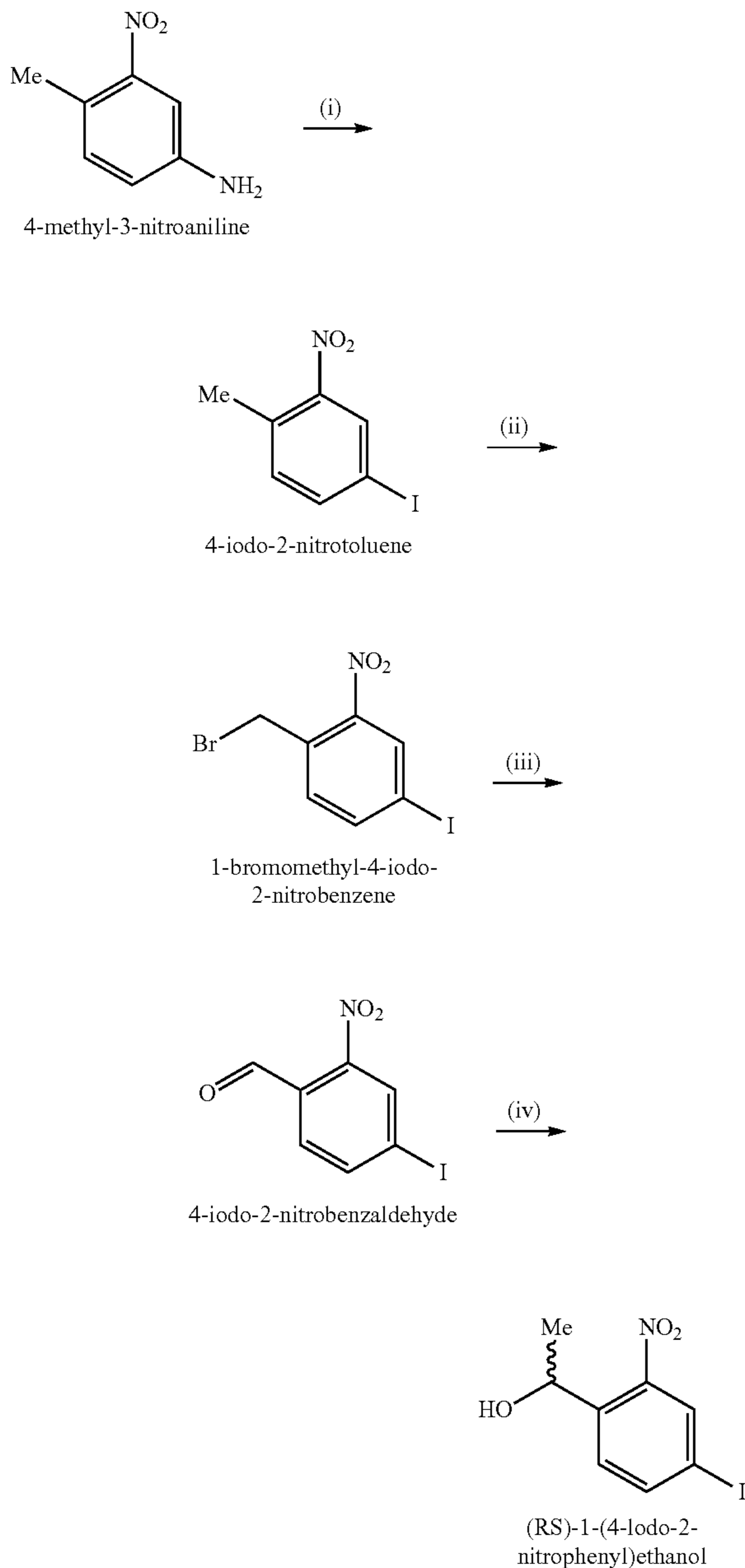
Scheme 2. Synthesis of (RS)-1-(4-iodo-2-nitrophenyl)ethanol:
