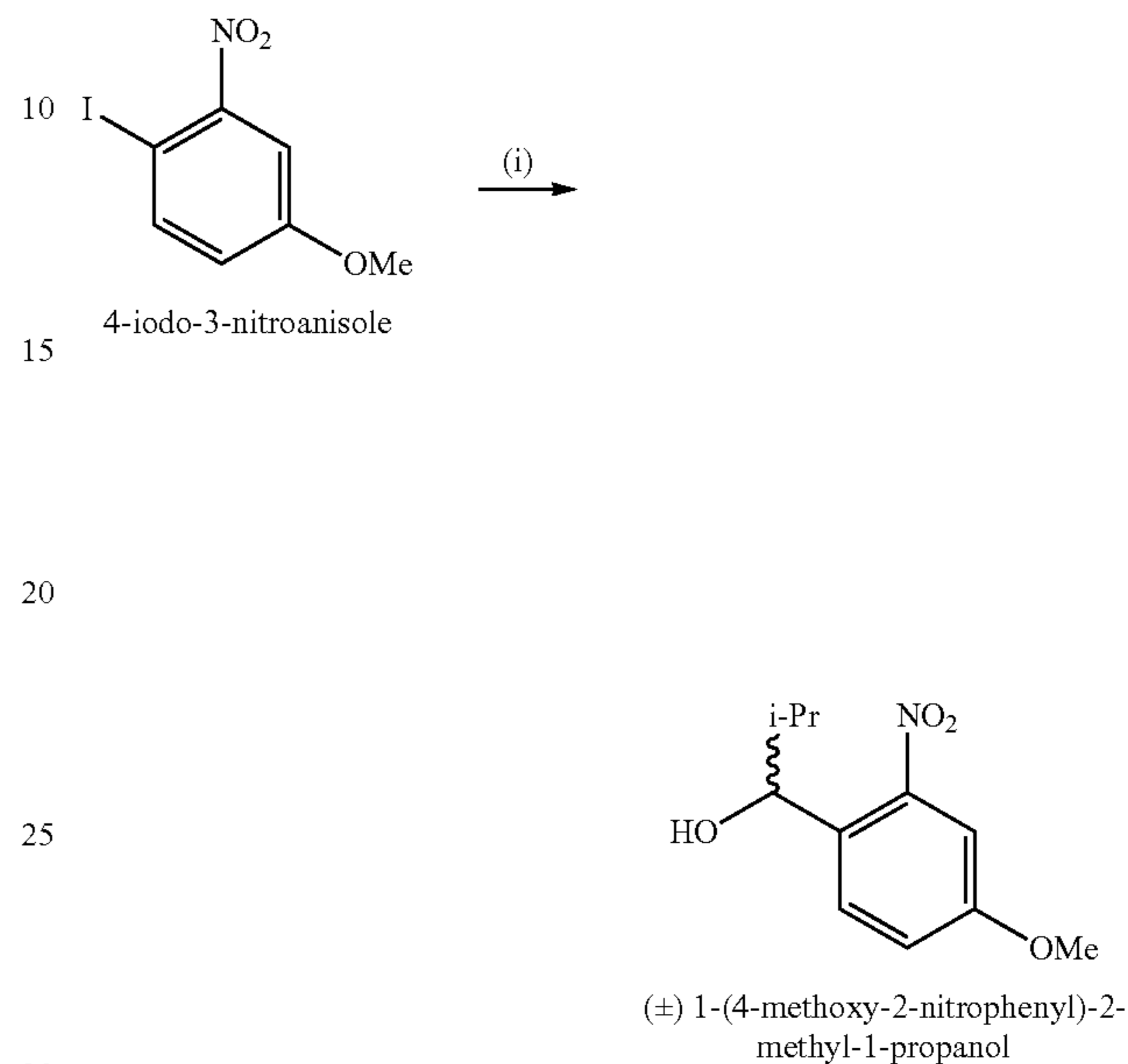
Scheme 8. Synthesis of 1-(4-methoxy-2-nitrophenyl)-2-methyl-1-propanol.
