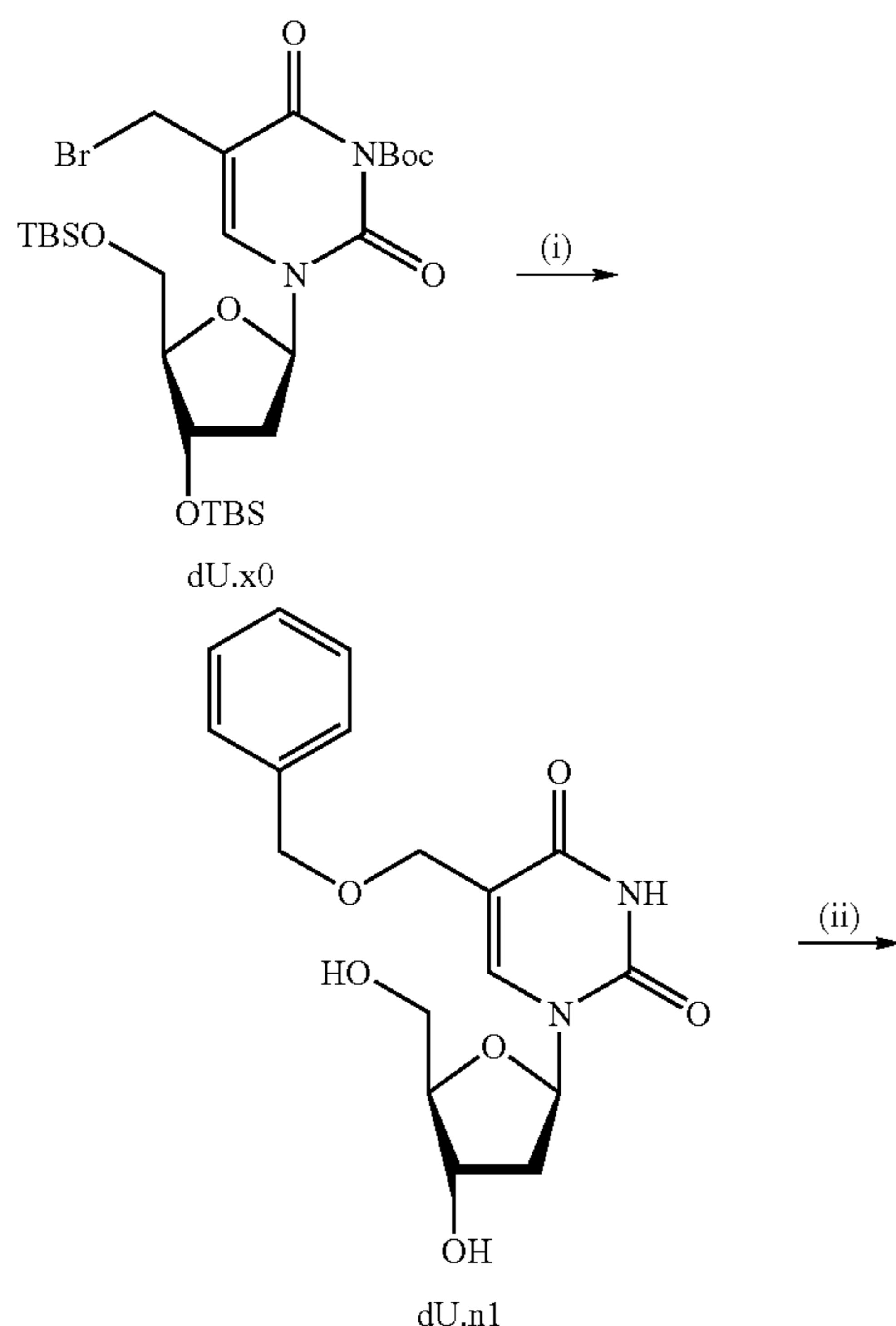
Scheme 30. Synthesis of 5-(benzyloxy)methyl-2'-deoxyuridine-5'-triphosphate.
