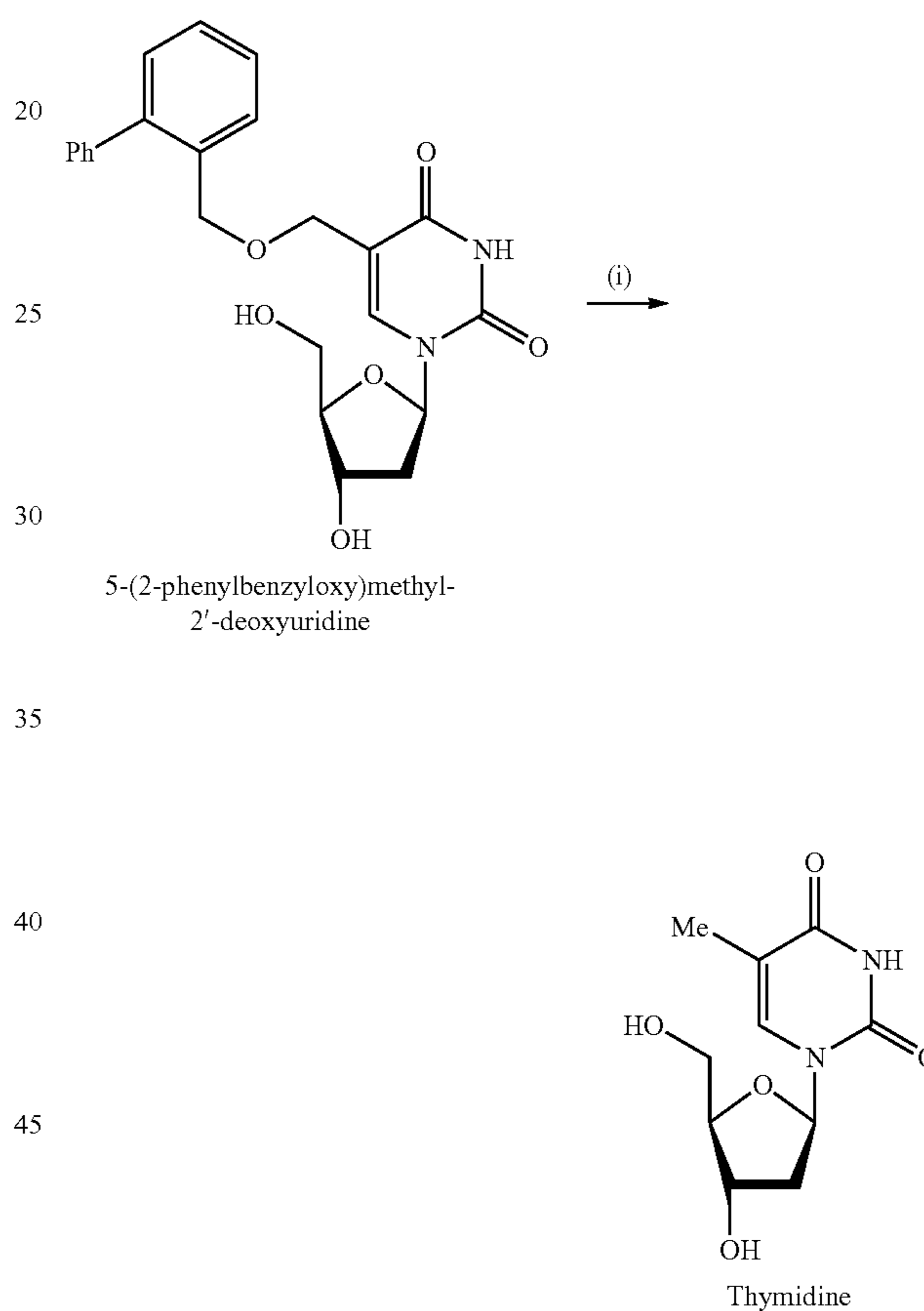
Scheme 40. Chemical cleavage of 5-(2-phenylbenzyloxy)methyl-2'-deoxyuridine
