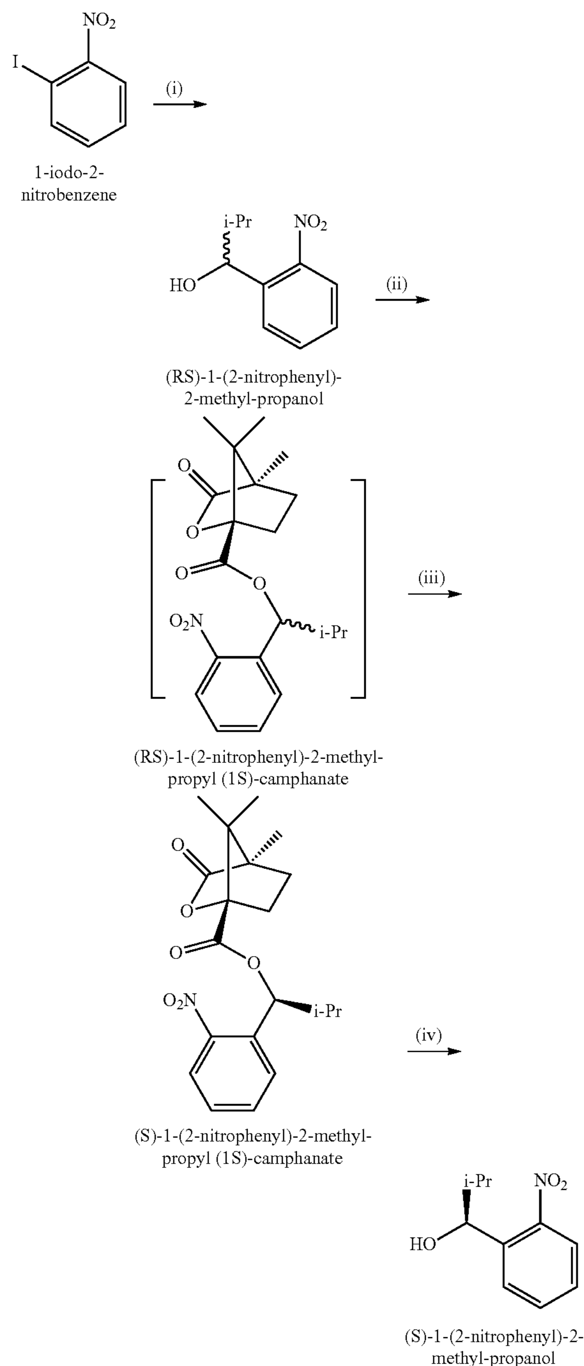
Scheme 3. Synthesis of (RS)-1-(2-nitrophenyl)-2-methyl-1-propanol and (S)-1-(2-nitrophenyl)-2-methyl-1-propanol.
