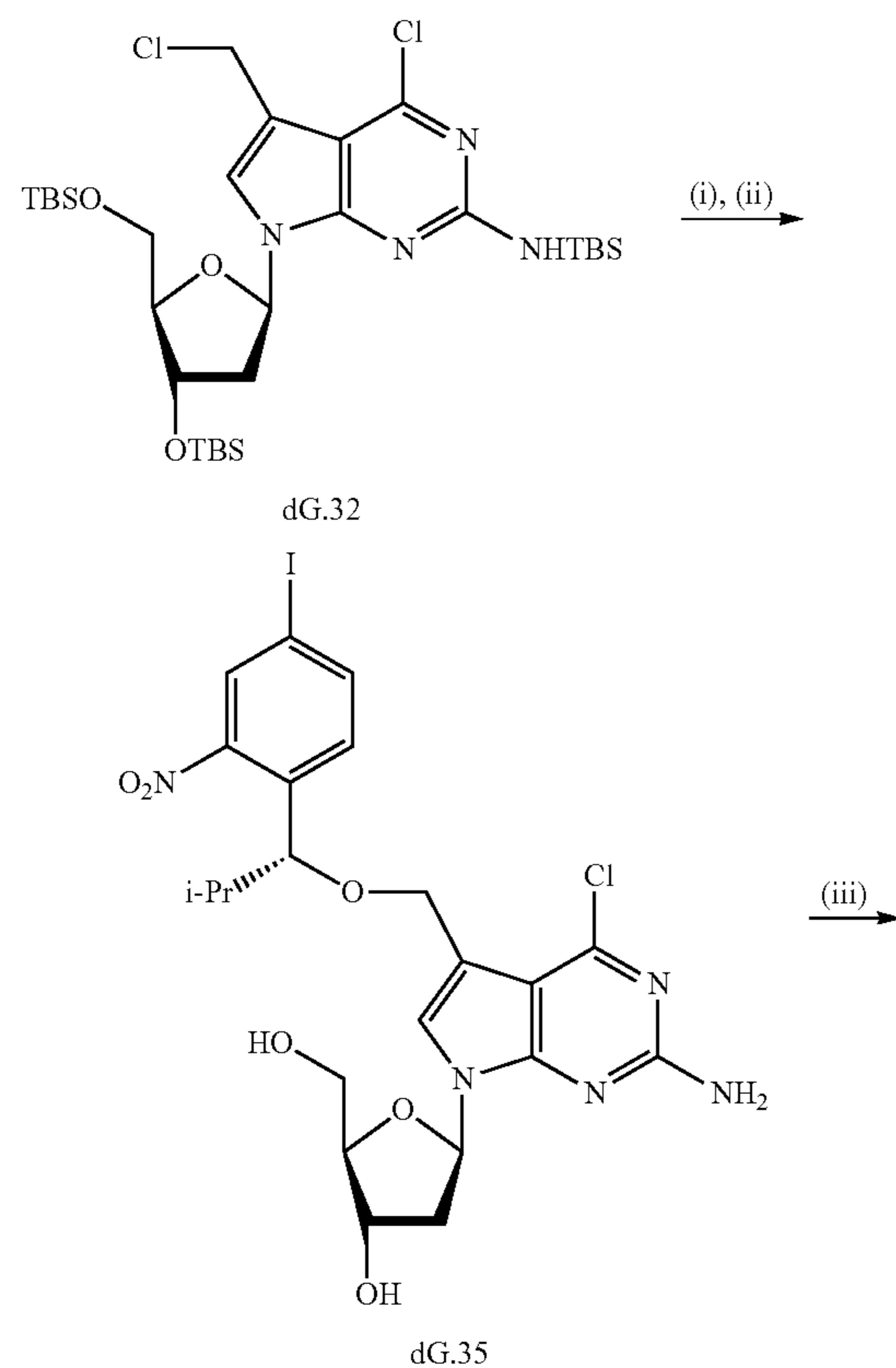
Scheme 22. Synthesis of 6-ROX labeled 7-[(R)-1-[4-(3-amino-1-propynyl)-2-nitrophenyl]-2-methyl-propyloxy]methyl-7-deaza-2'-deoxyguanosine-5'-triphosphate
