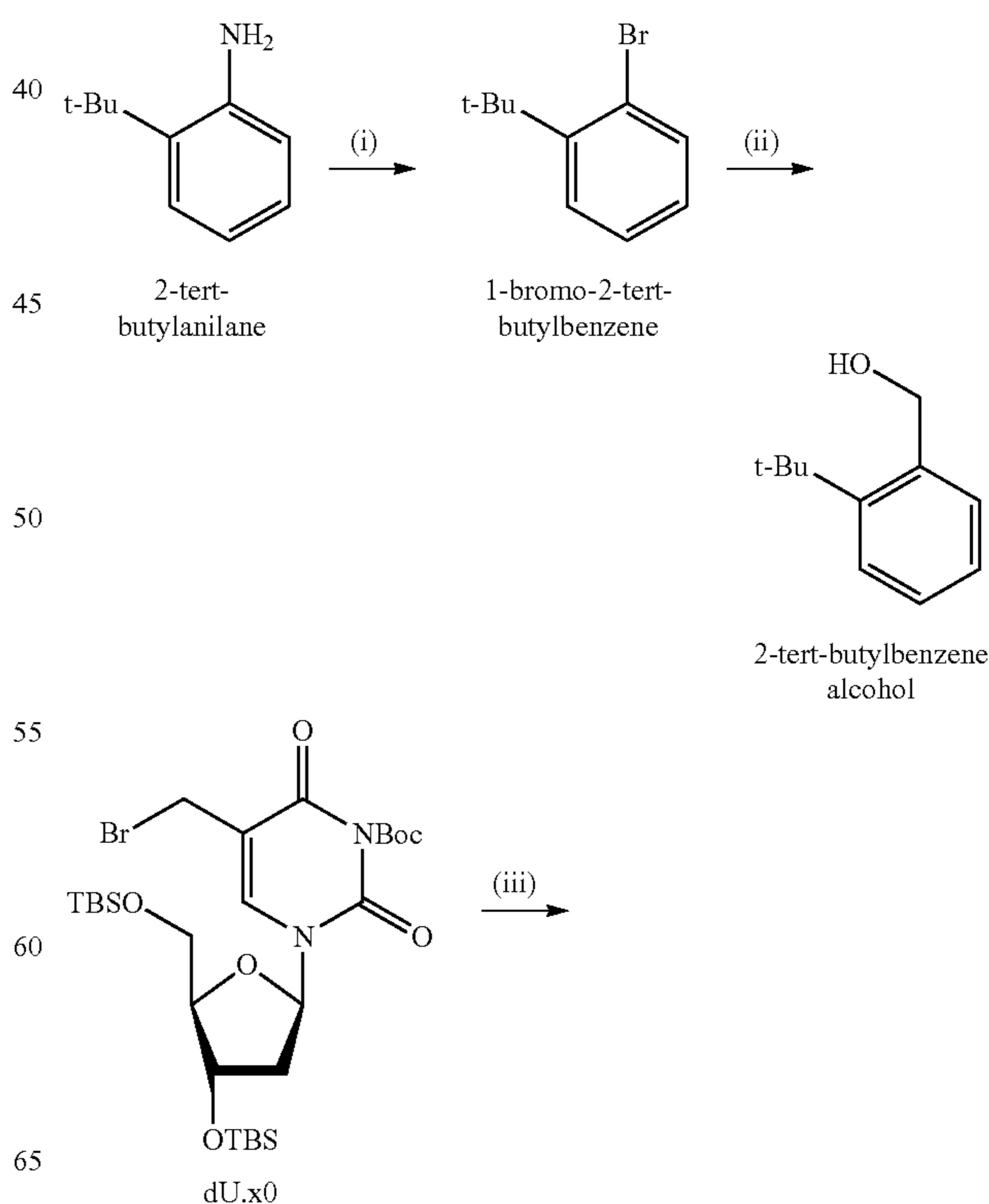
Scheme 34. Synthesis of 5-(2-tert-butylbenzyloxy)methyl-2'-deoxyuridine-5'-triphosphate.
