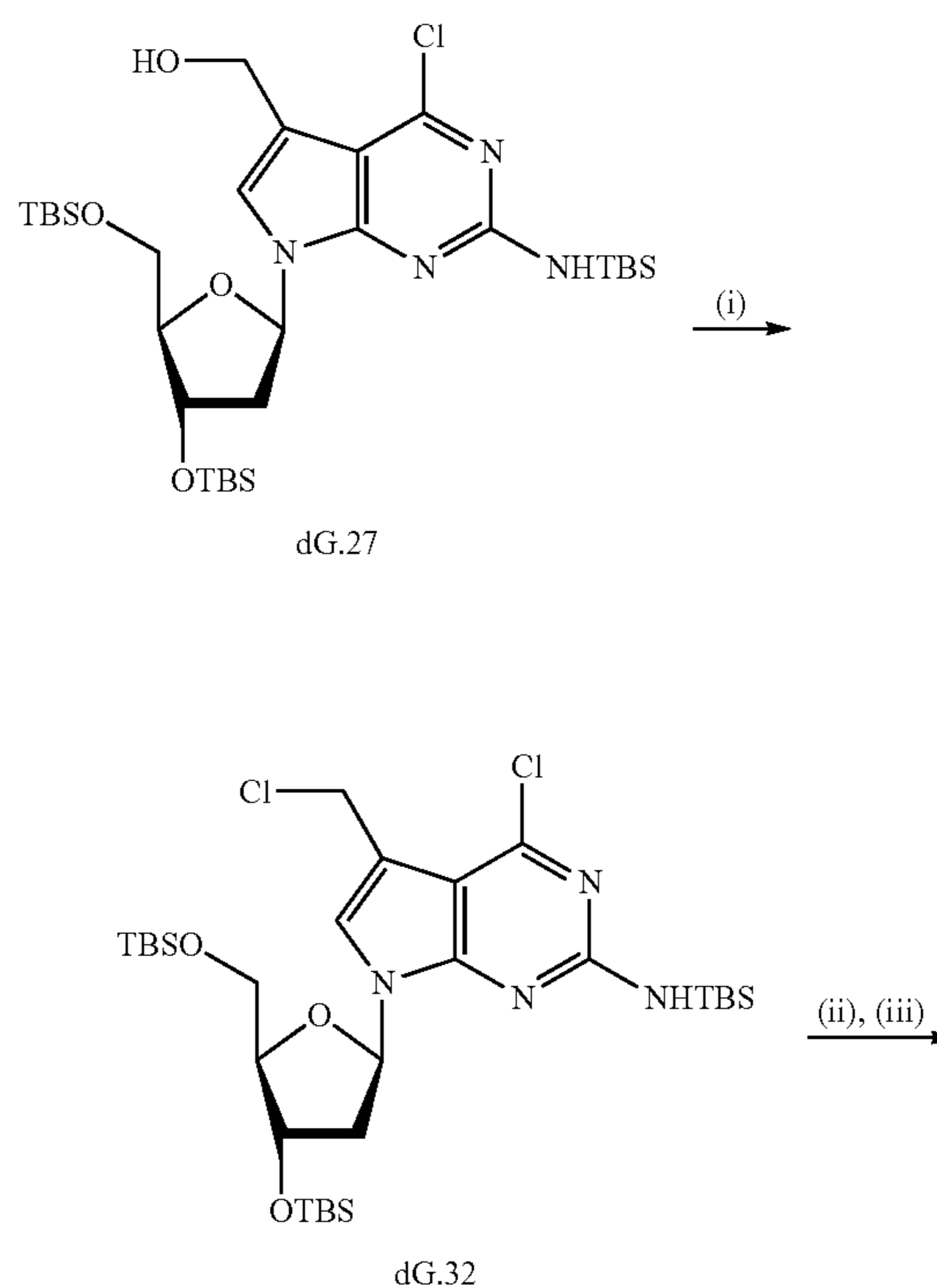
Scheme 21. Synthesis of 7-[1-(2-nitrophenyl)-2-methyl-propyloxy]methyl-7-deaza-2'-deoxyguanosine, 5'-triphosphate.
