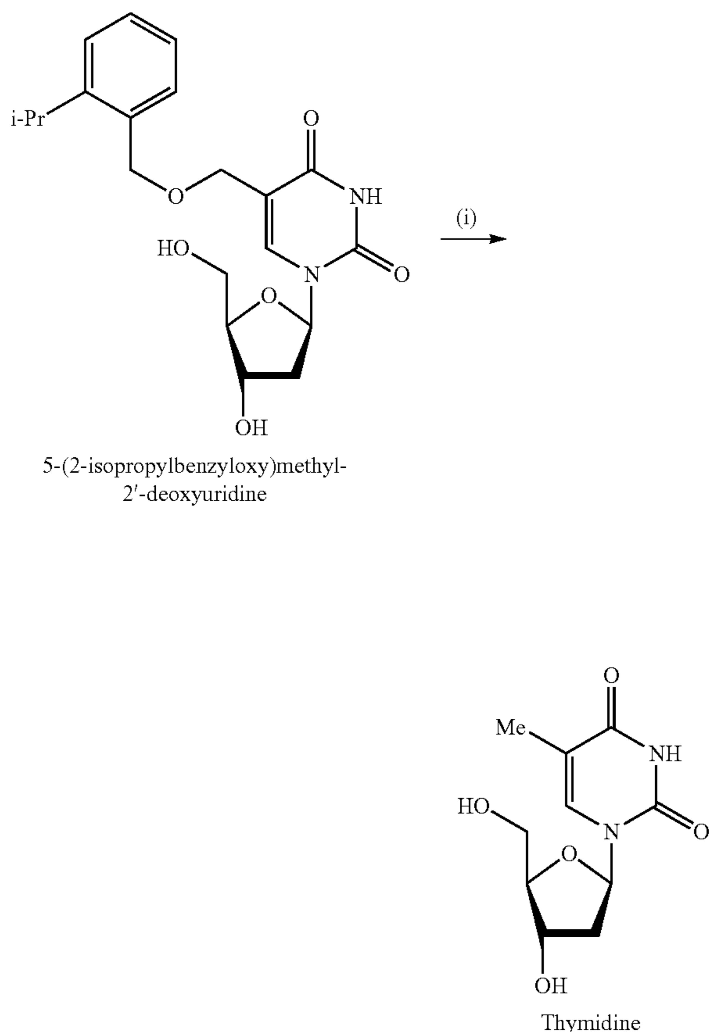
Scheme 39. Chemical cleavage of 5-(2-isopropylbenzyloxy)methyl-2'-deoxyuridine
