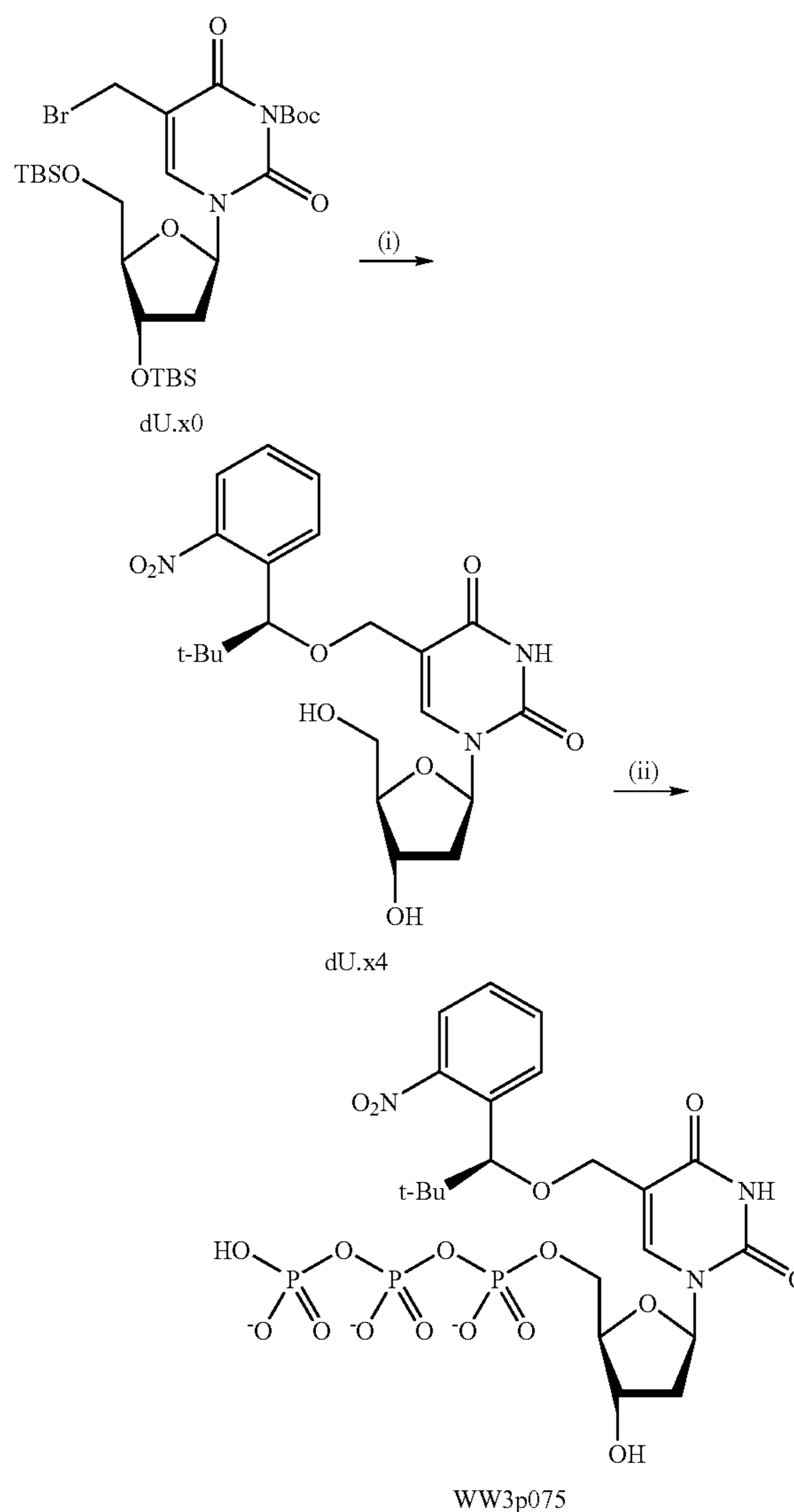
Scheme 12. Synthesis of 5-[(R or S)-1-(2-nitrophenyl)-2,2-dimethyl-1-propyloxy]methyl-2'-deoxyuridine-5'-triphosphate.
