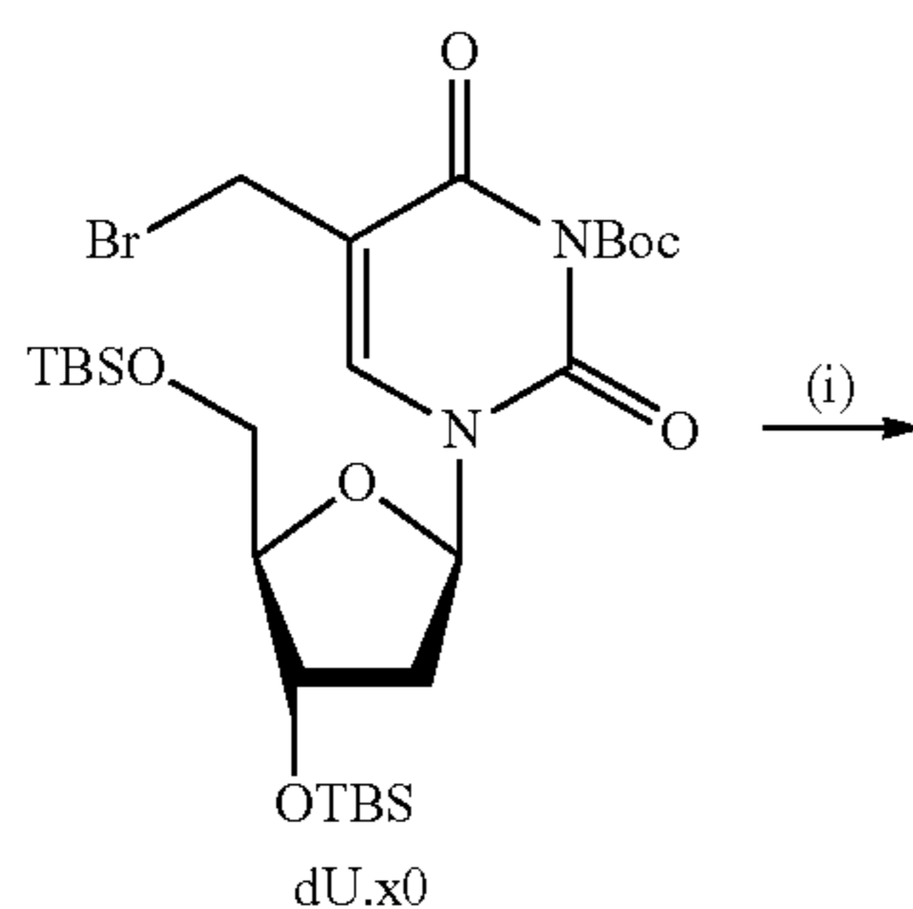
Scheme 13. Synthesis of 5-[(R or S)-1-(2-nitrophenyl)-2,2-dimethyl-1-propyloxy]methyl-2'-deoxycytidine-5'-triphosphate.
