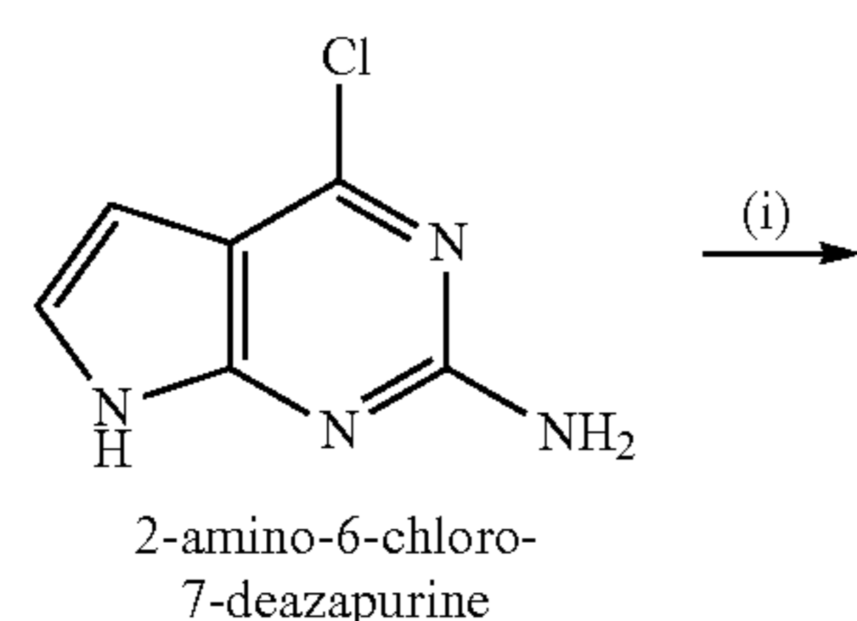
Scheme 19. Synthesis of 7-(2-nitrobenzyloxy)methyl-7-deaza-2'-deoxyguanosine-5'-triphosphate.
