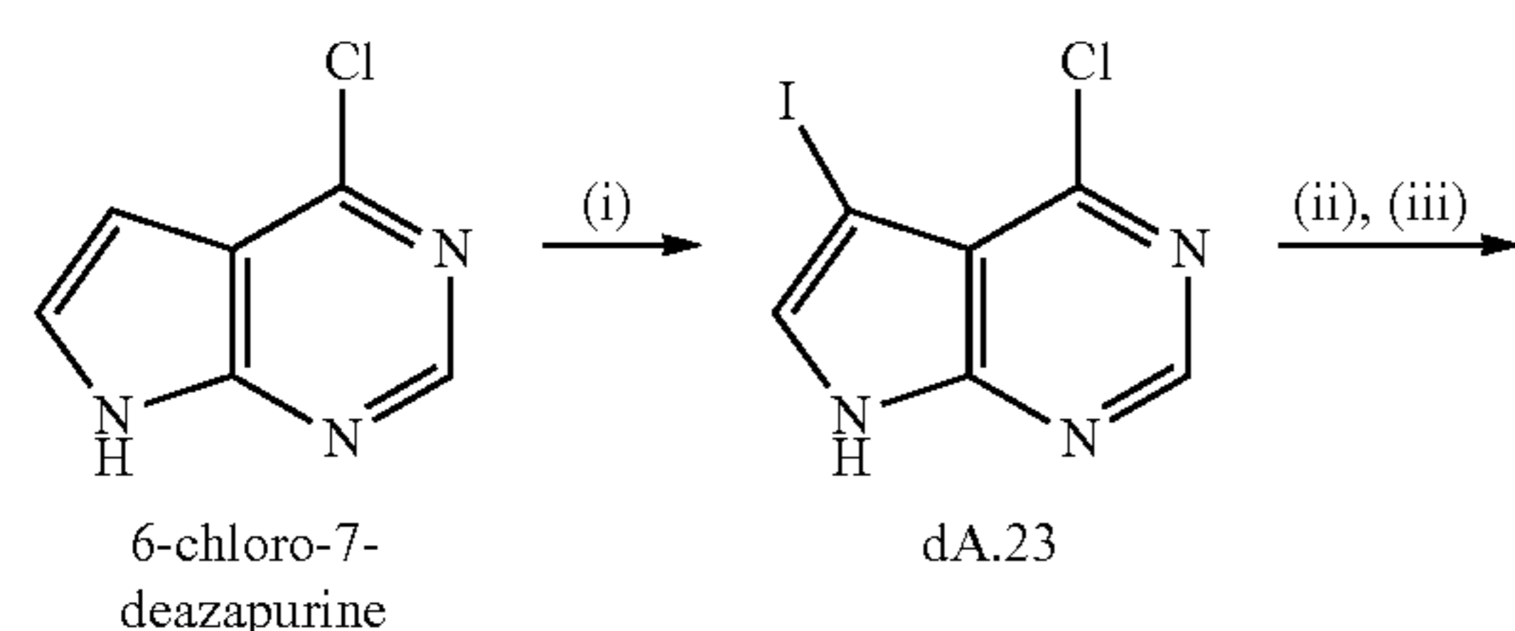
Scheme 24. Synthesis of 7-(2-nitrobenzyloxy)methyl-7-deaza-2'-deoxyadenosine-5'-triphosphate.
