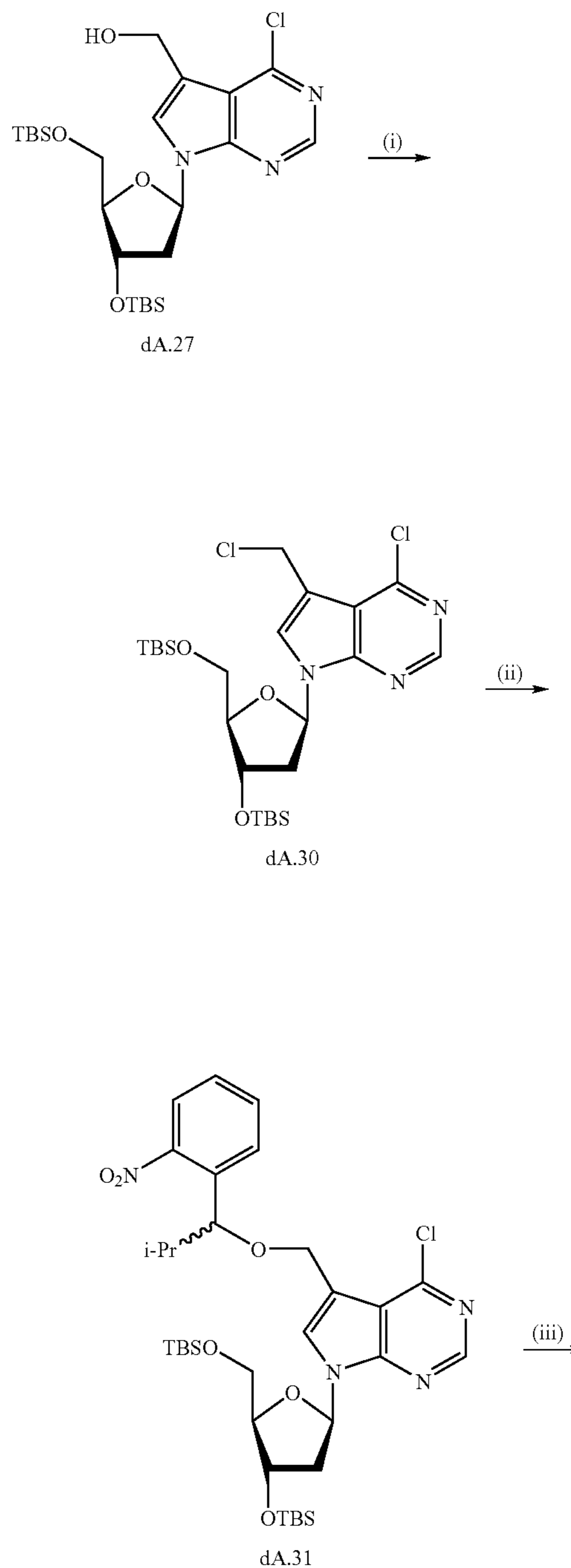
Scheme 25. Synthesis of 7-[1-(2-nitrophenyl)-2-methyl-propyloxy]methyl-7-deaza-2'-deoxyadenosine-5'-triphosphate.
