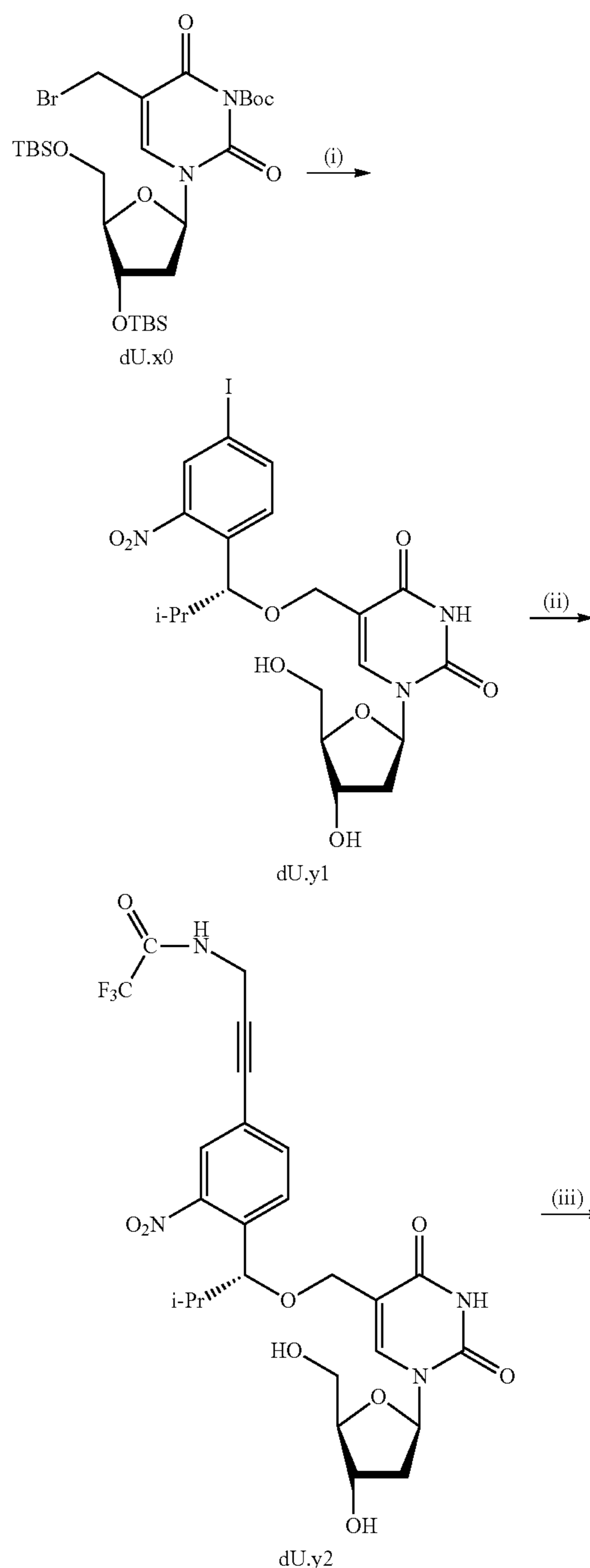
Scheme 14. Synthesis of 6-JOE labeled 5-[(R)-1-[4-(3-amino-1-propynyl)-2-nitrophenyl]-2-methyl-propyloxy]methyl-2'-deoxyuridine-5'-triphosphate.
