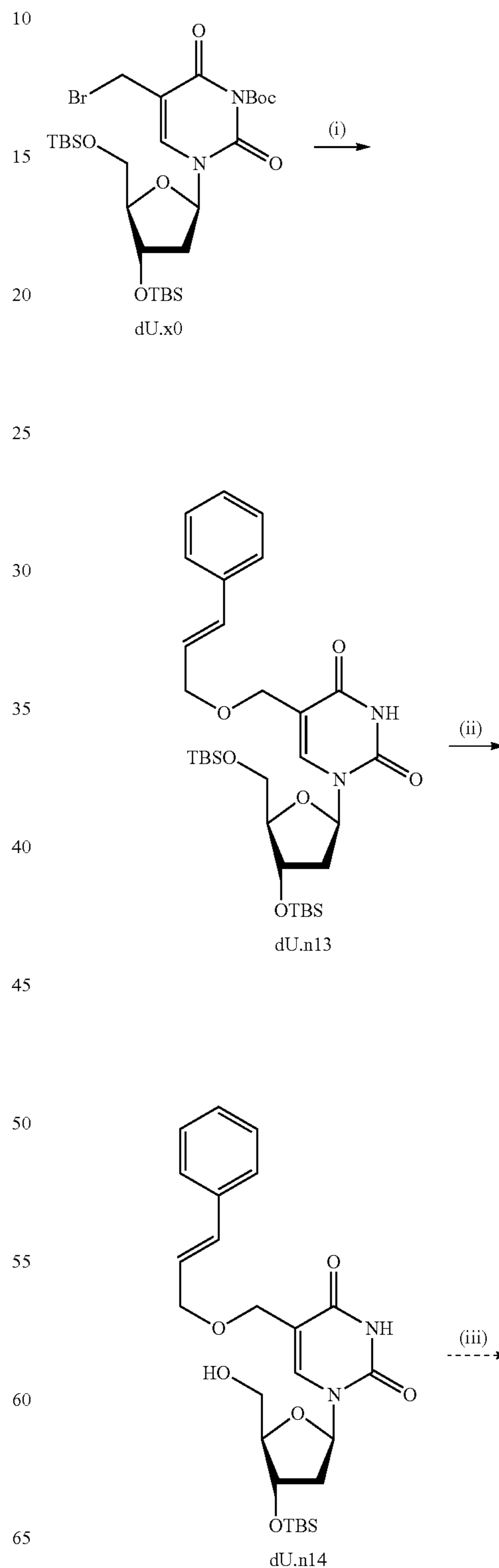
Scheme 37. Synthesis of 5-(3-phenyl-2-propenyloxy)methyl-2'-deoxyuridine-5'-triphosphate.
