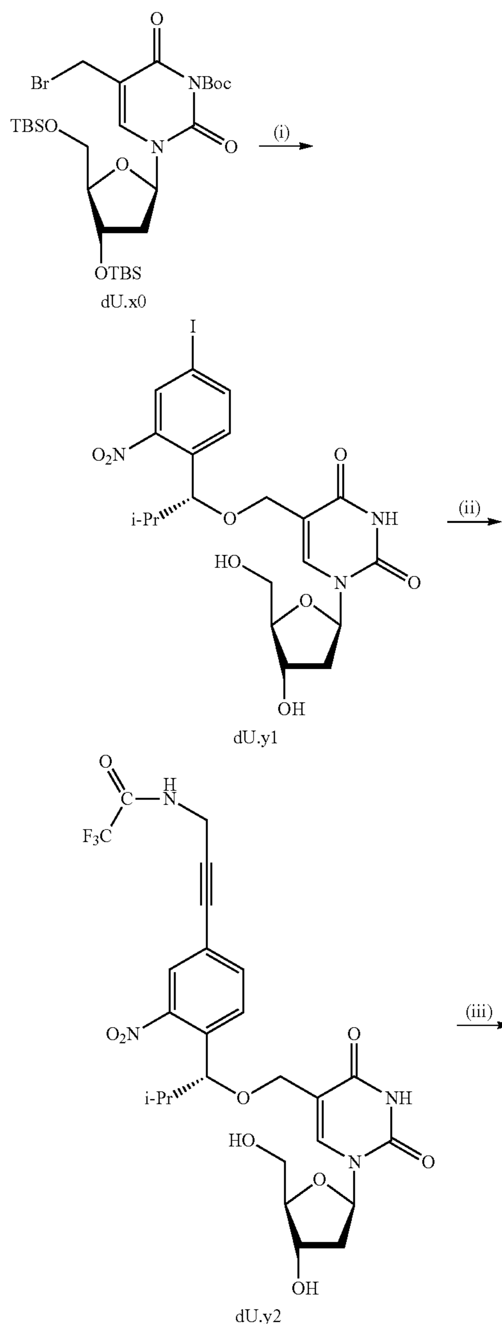
Scheme 14. Synthesis of 6-JOE labeled 5-[(R)-1-[4-(3-amino-1-propynyl)-2-nitrophenyl]-2-methyl-propyloxy]methyl-2'-deoxyuridine-5'-triphosphate.
