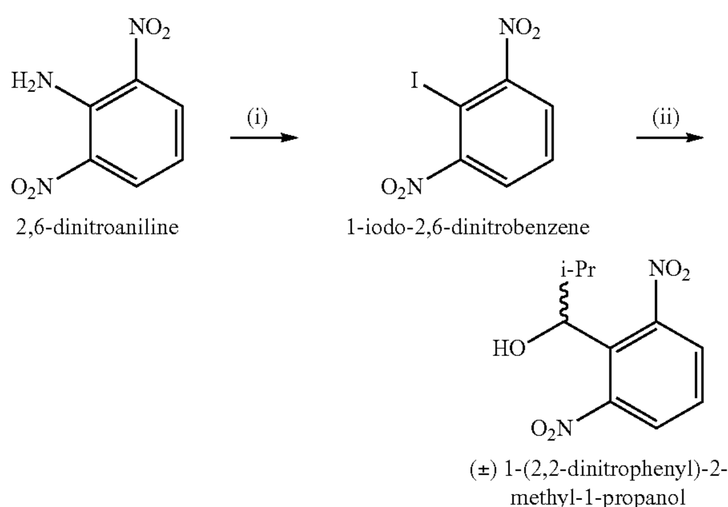
Scheme 7. Synthesis of racemic 1-(2,6-dinitrophenyl)-2-methyl-1-propanol.
