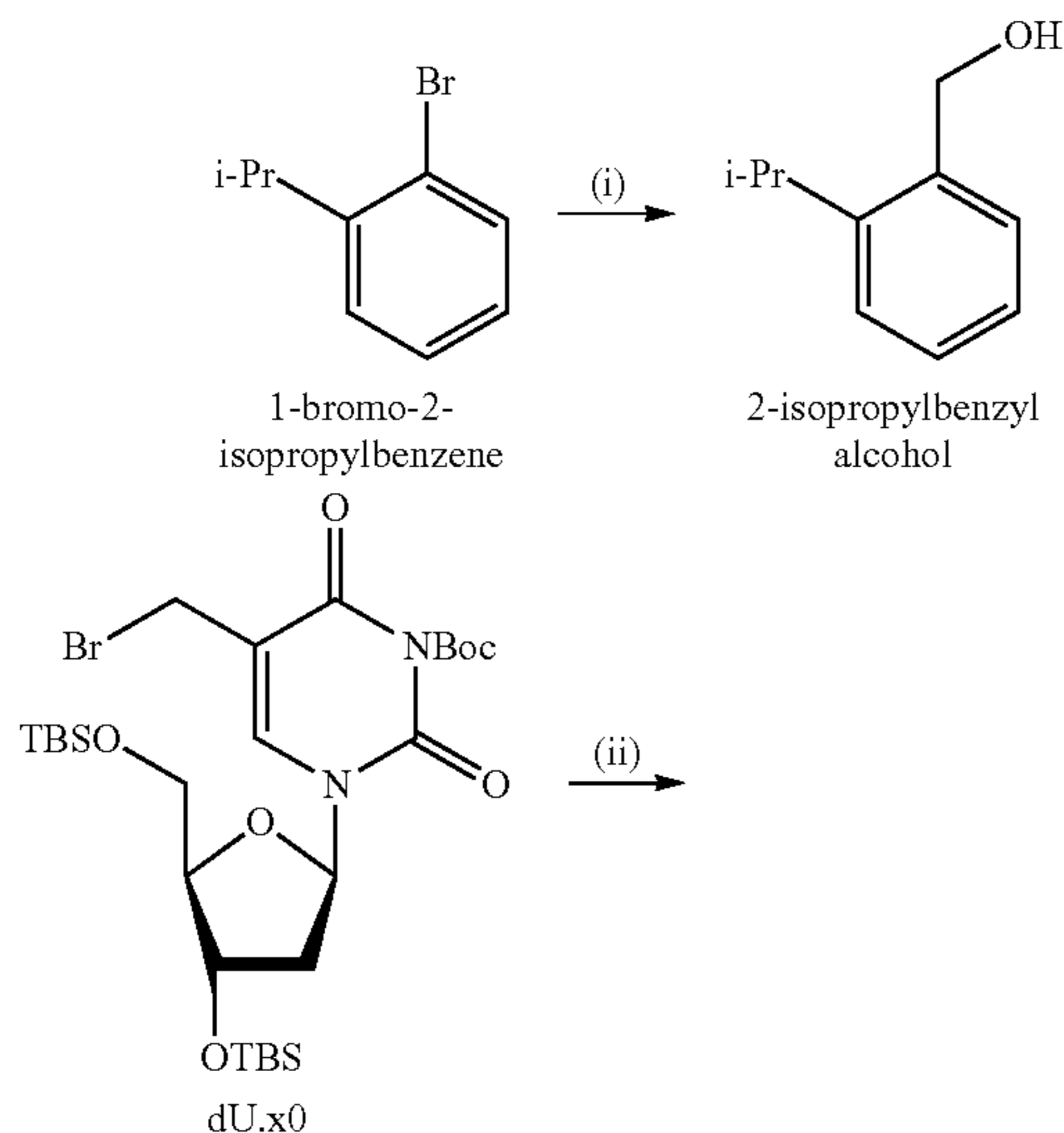
Scheme 33. Synthesis of 5-(2-isopropylbenzyloxy)methyl-2'-deoxyuridine-5'-triphosphate
