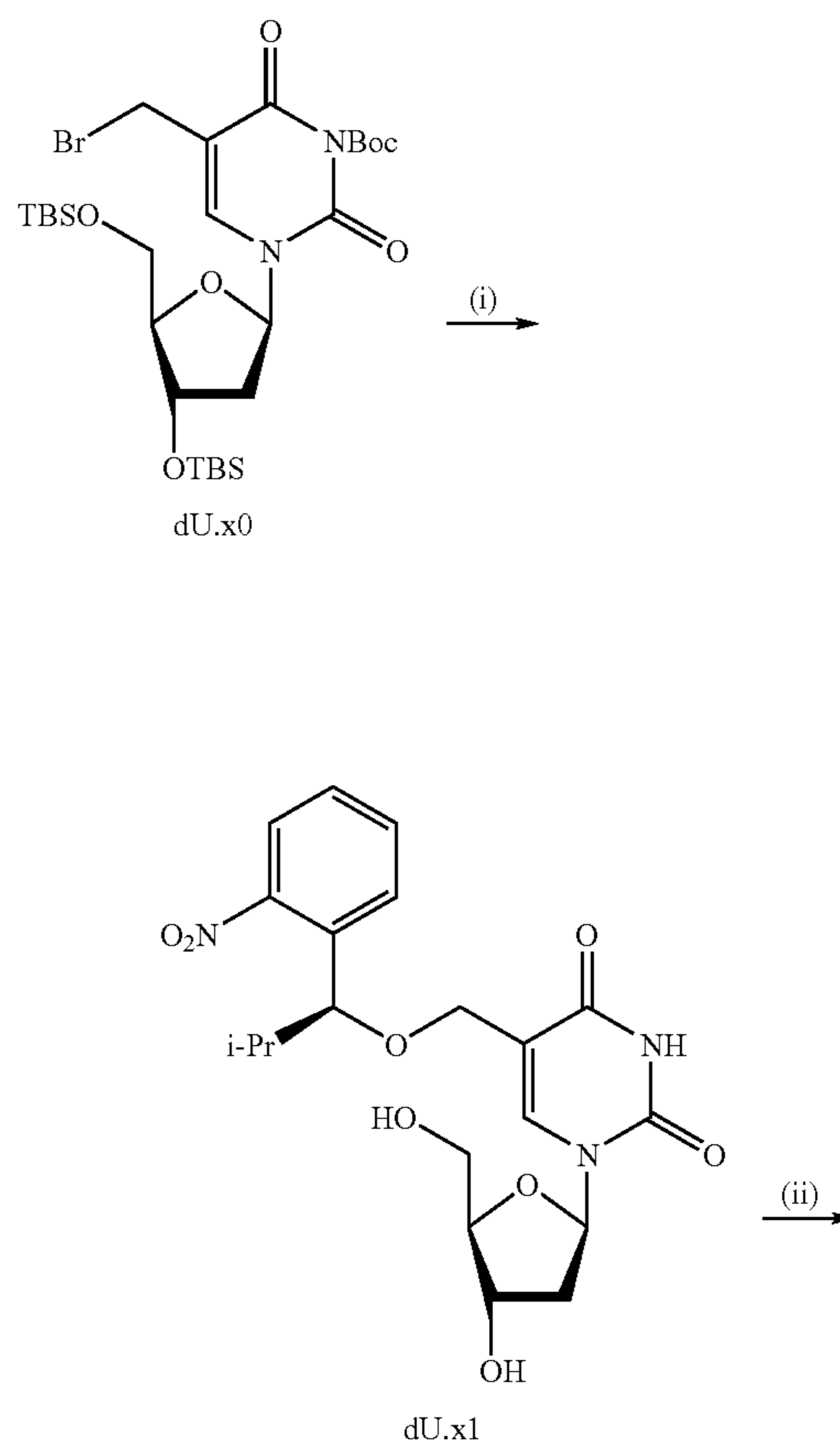
Scheme 10. Synthesis of 5-[(S)-1-(2-nitrophenyl)-2-methyl-propyloxy]methyl-2'-deoxyuridine-5'-triphosphate.
