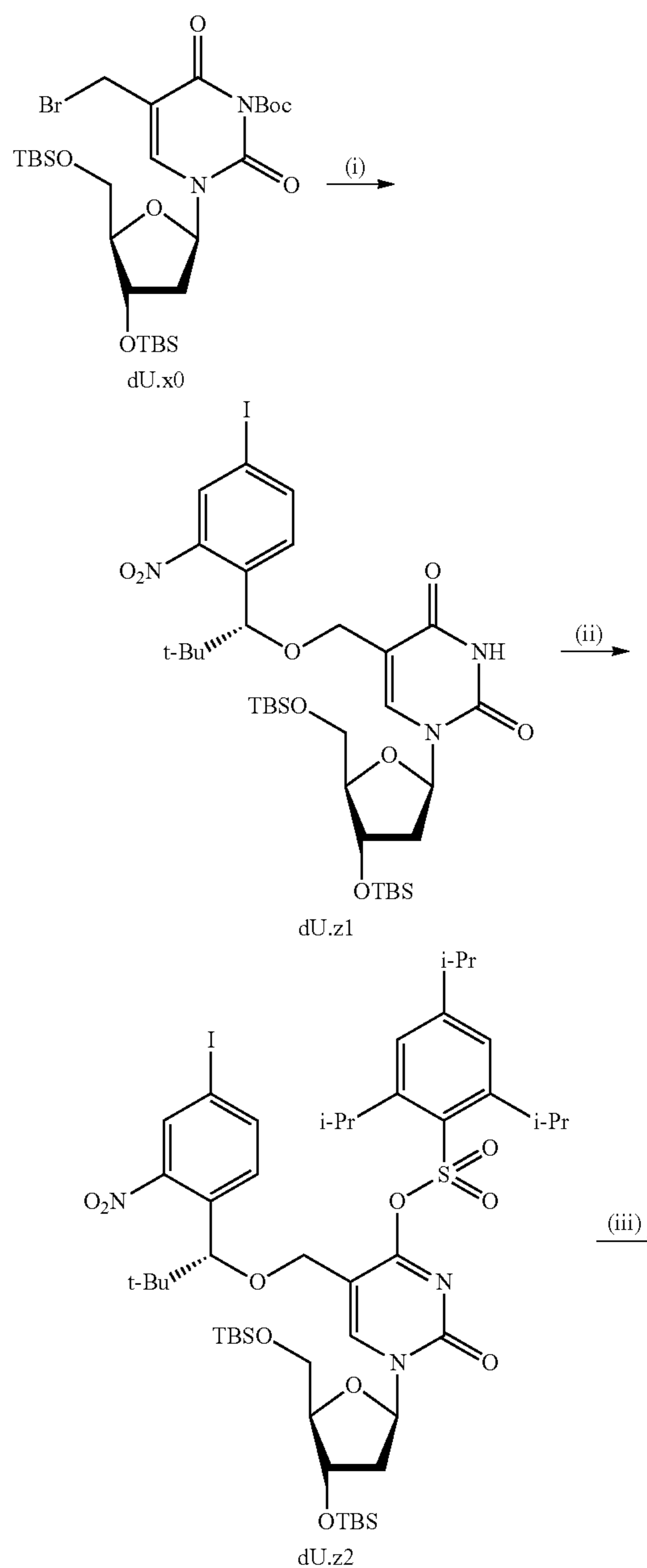
Scheme 17. Synthesis of 6-TAMRA labeled 5-{(R or S)-1-[4-(3-amino-1-propynyl)-2-nitrophenyl]-2,2-dimethyl-propoxy}methyl-2'-deoxycytidine-5'-triphosphate.
