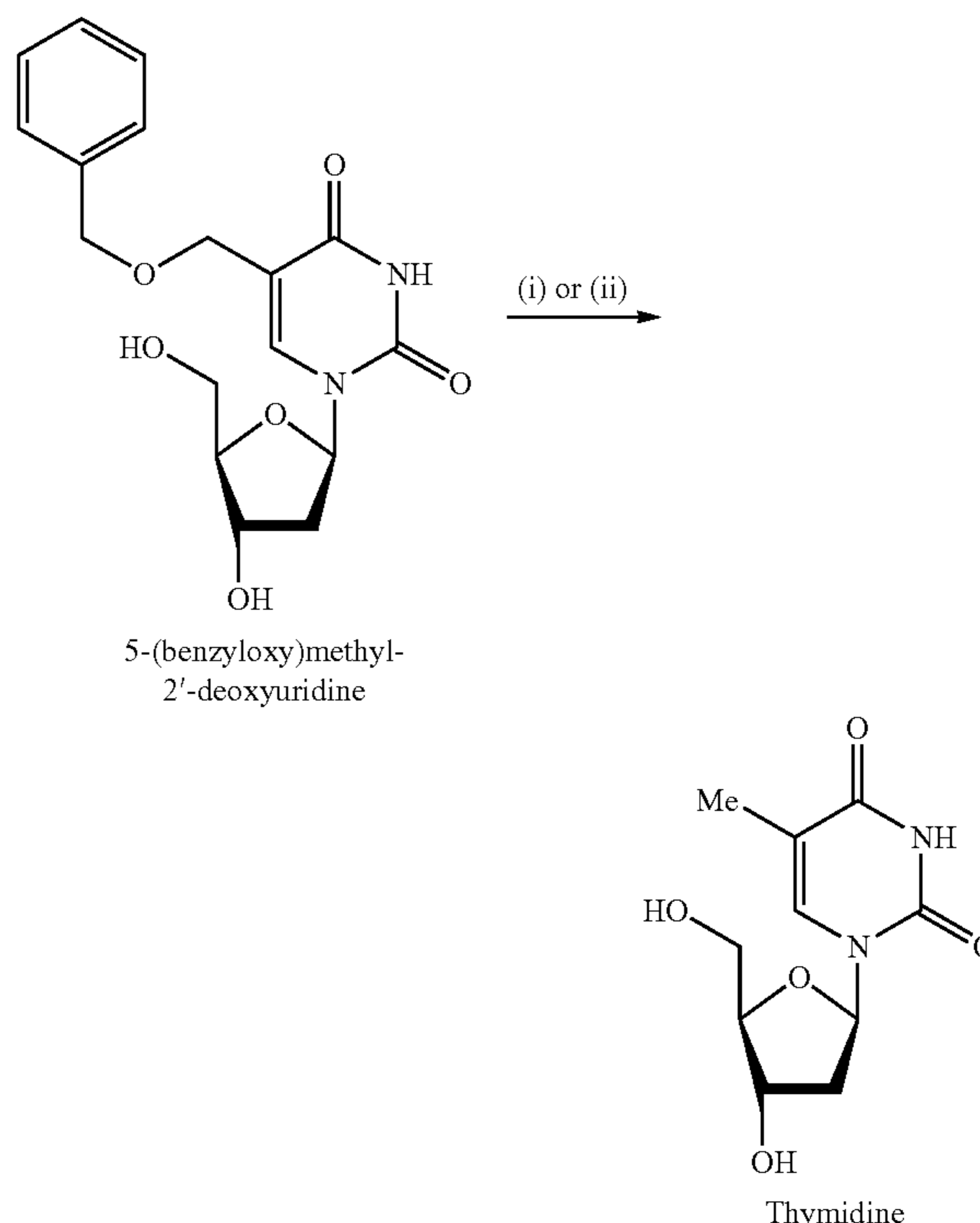
Scheme 38. Chemical cleavage of 5-(benzyloxy)methyl-2'-deoxyuridine.
