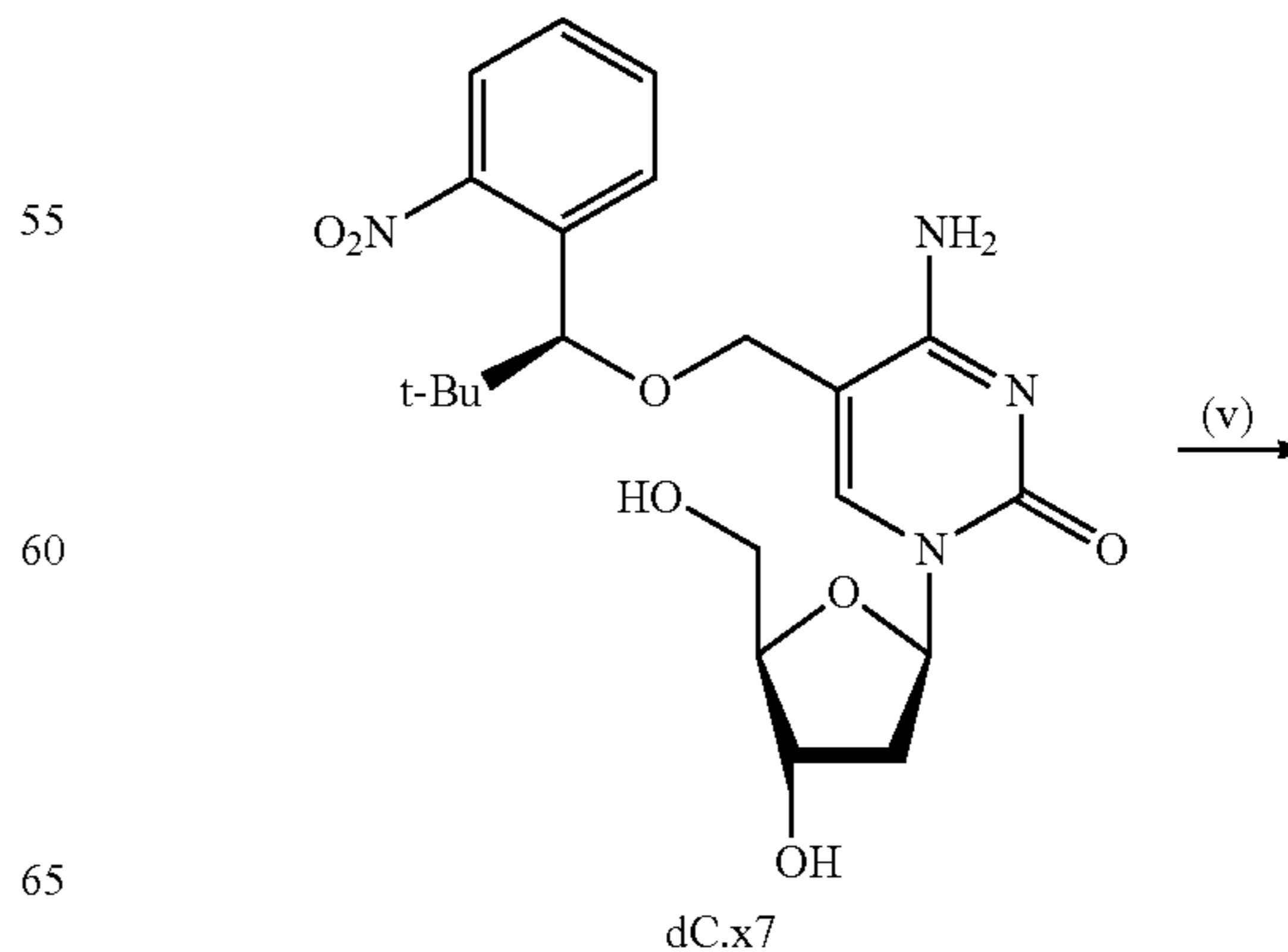
Scheme 13. Synthesis of 5-[(R or S)-1-(2-nitrophenyl)-2,2-dimethyl-1-propyloxy]methyl-2'-deoxycytidine-5'-triphosphate.
