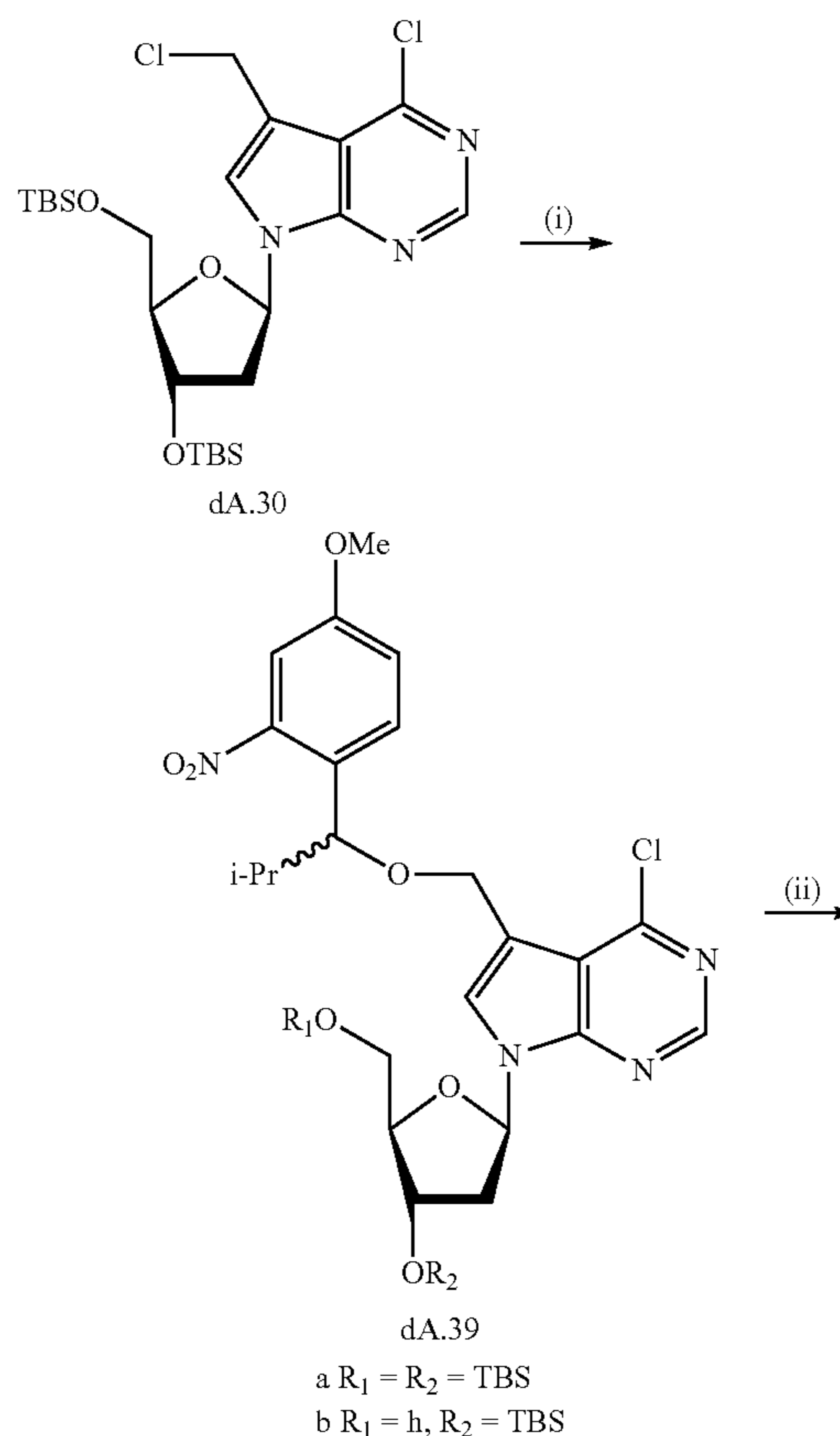
Scheme 29. Synthesis of 7-[1-(4-methoxy-2-nitrophenyl)-2-methyl-propyloxy]methyl-7-deaza-2'-deoxyadenosine-5'-triphosphate.
