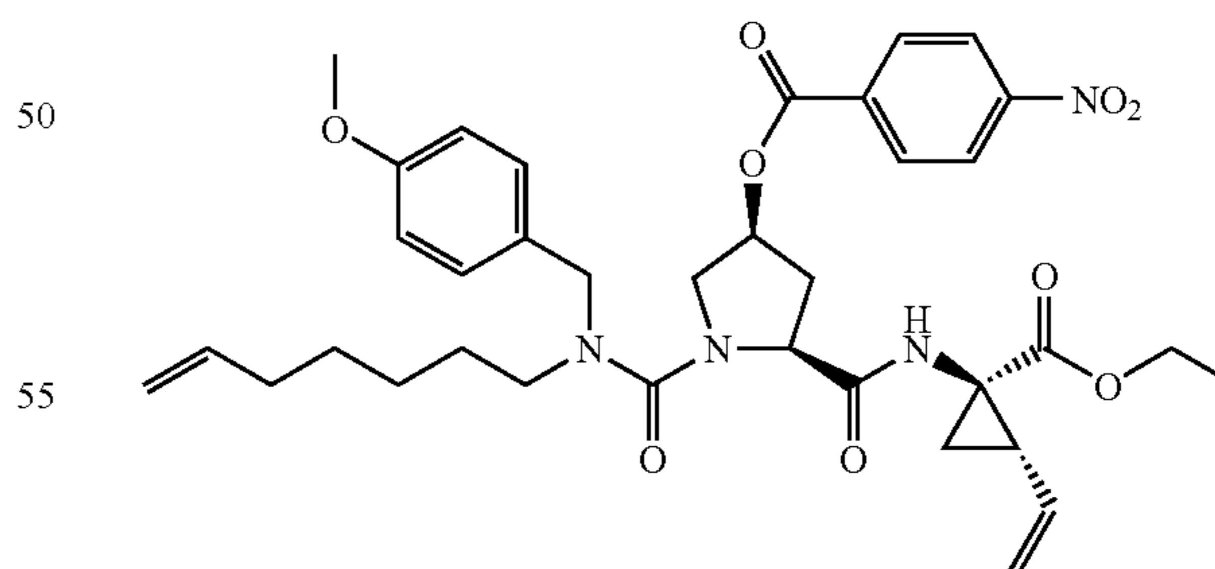
4-Nitro-benzoic acid 5-(1-ethoxycarbonyl-2-vinyl-cyclopropylcarbamoyl)-1-[hept-6-enyl-(4-methoxybenzyl)-carbamoyl]-pyrrolidin-3-yl ester (135)
