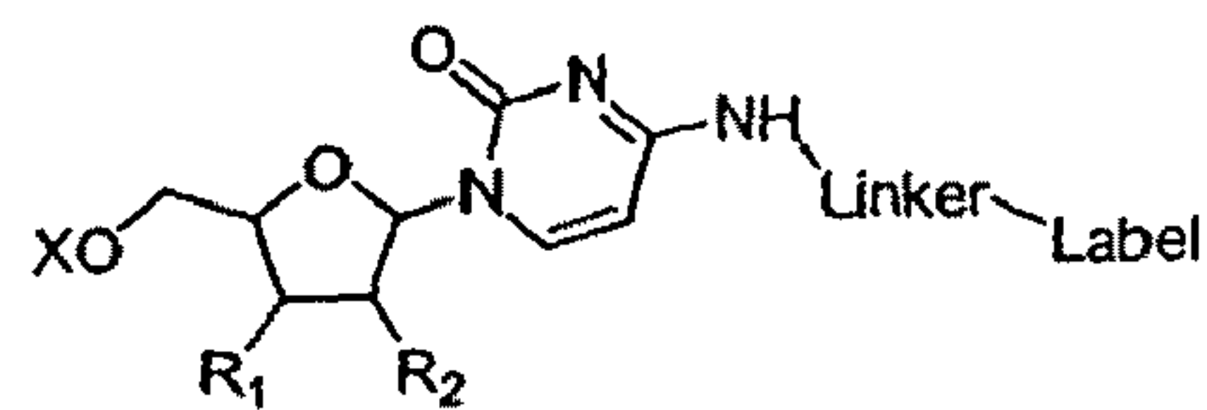
Cytidine N4-linker
