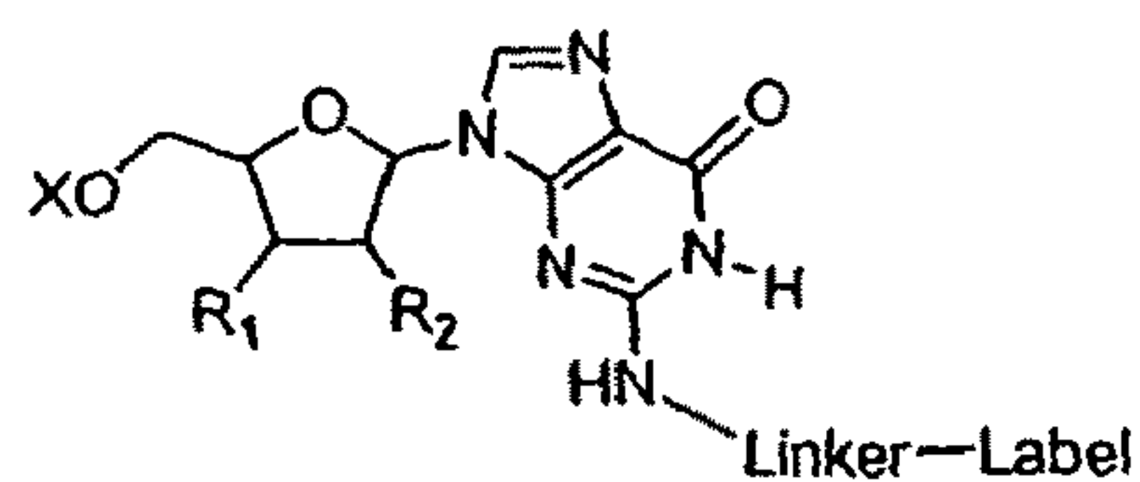
Guanosine N2-linker
