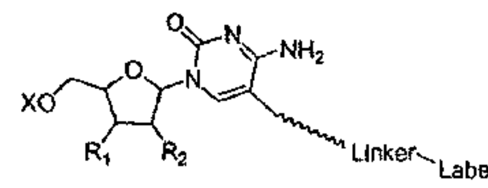
Cytidine C5-linker
