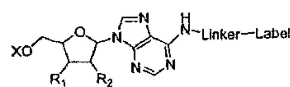
Adenosine N8-linker
