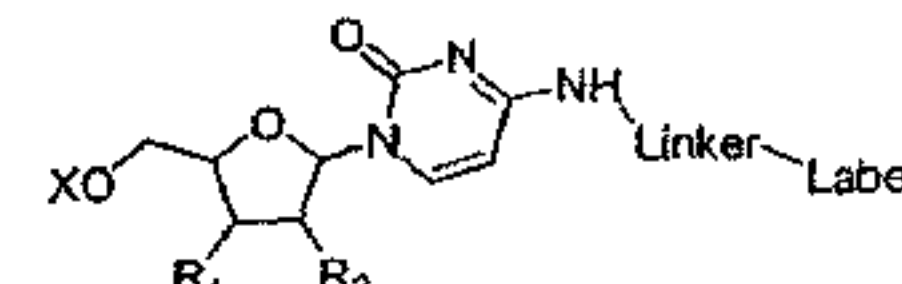
Cytidine N4-linker
