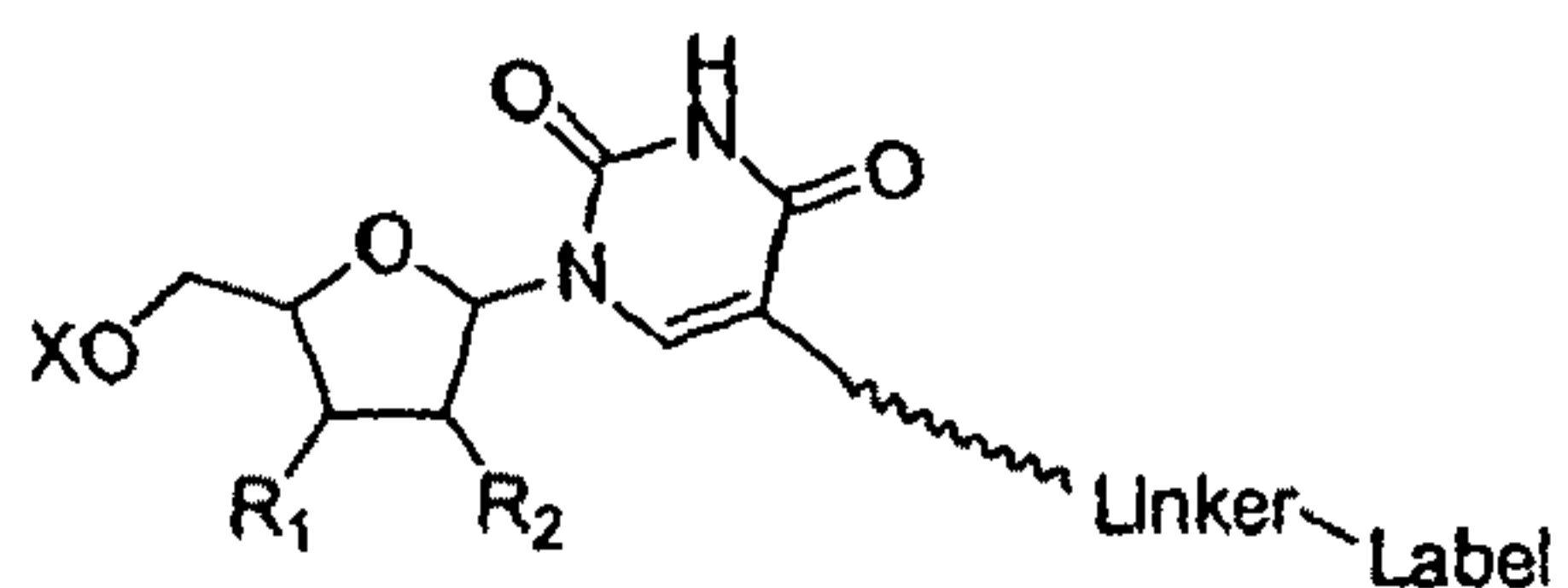
Uridine C5-linker
