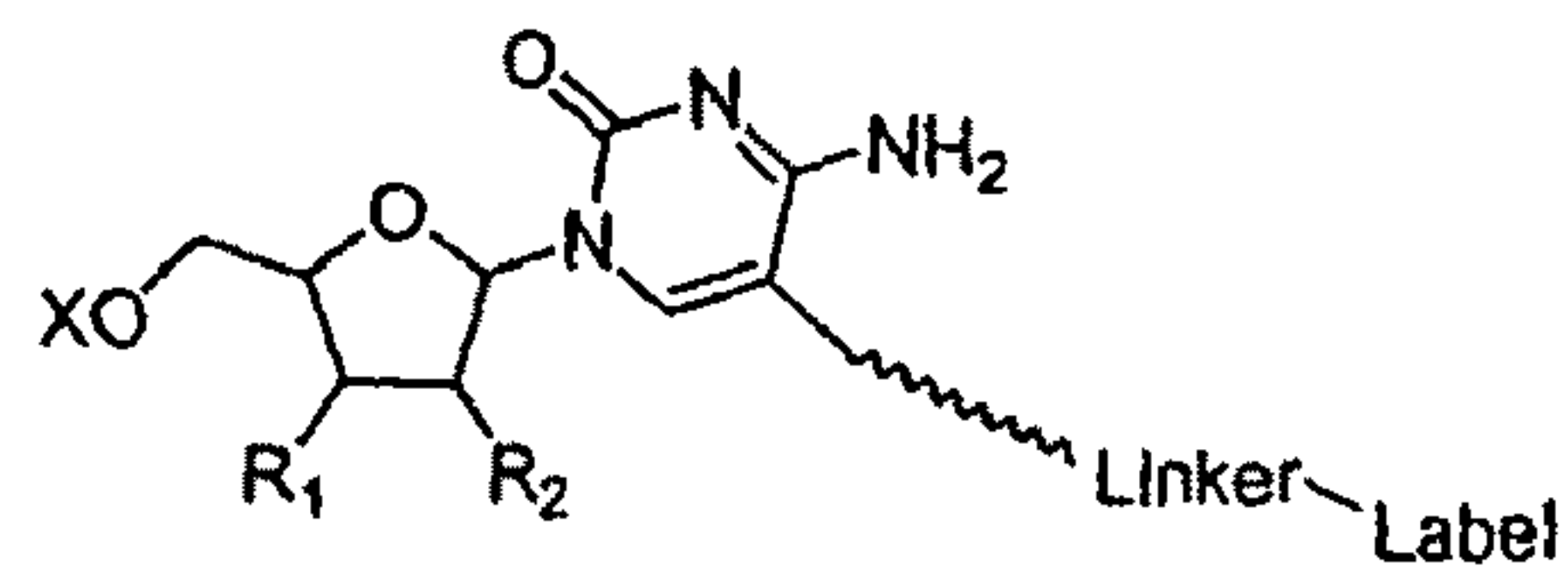
Cytidine C5-linker
