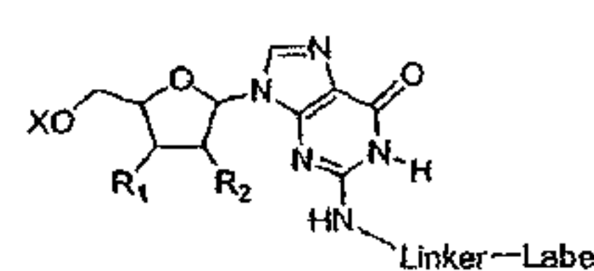
Guanosine N2-linker
