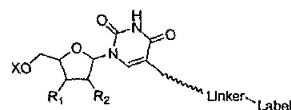
Uridine C5-linker
