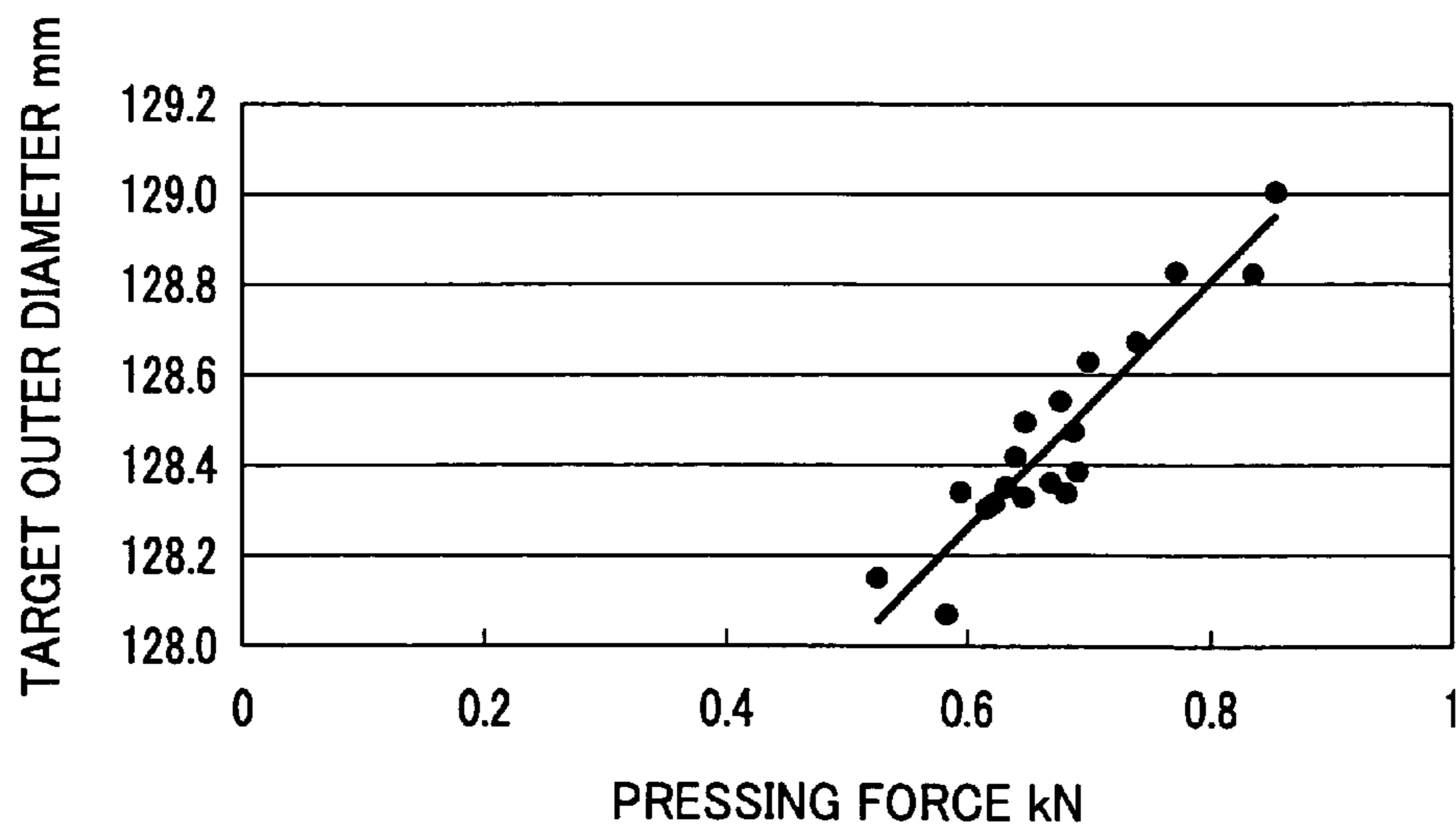
RELATION BETWEEN TARGET OUTER DIAMETER AND PRESSING FORCE
