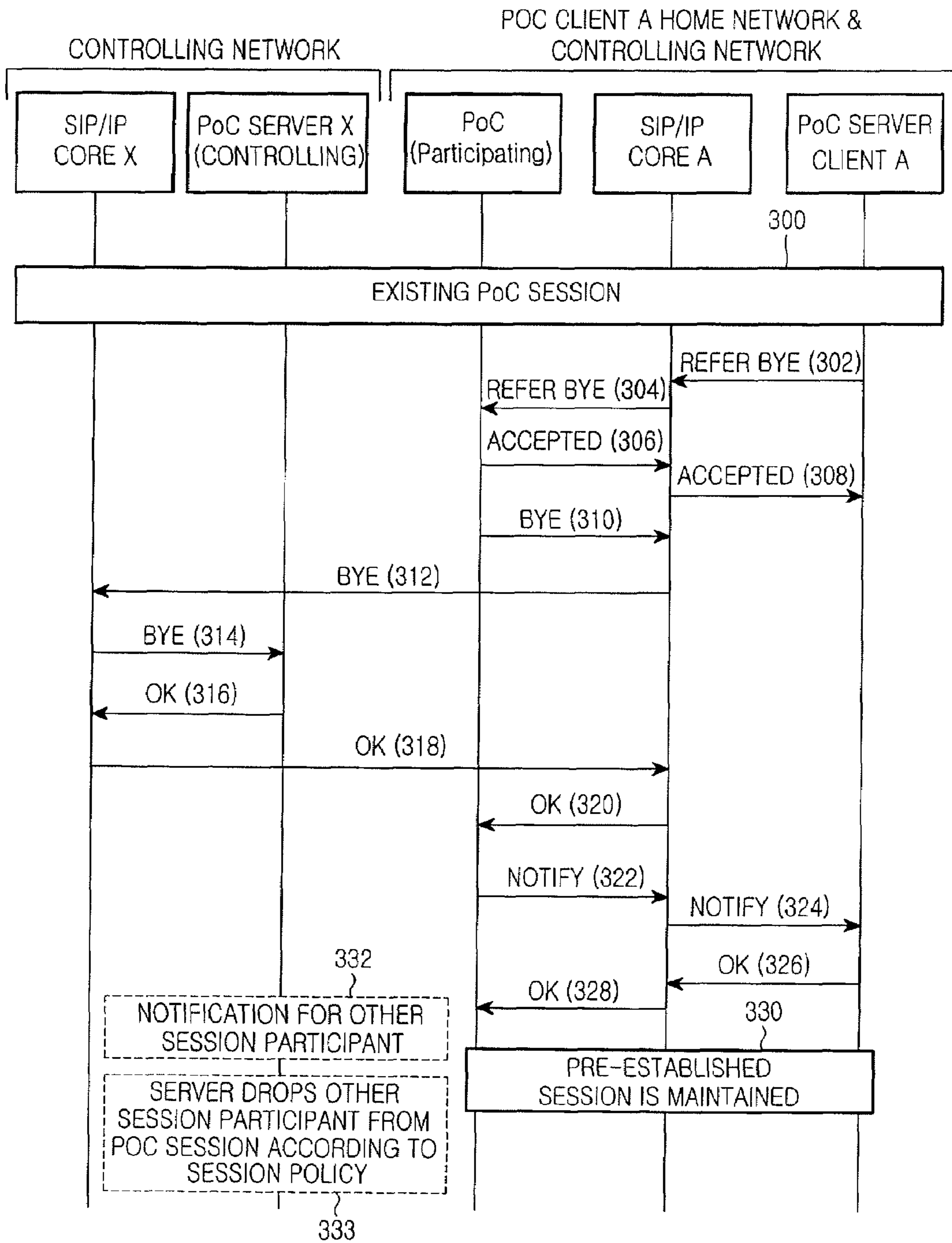
FIG.3 (CONVENTIONAL ART)
