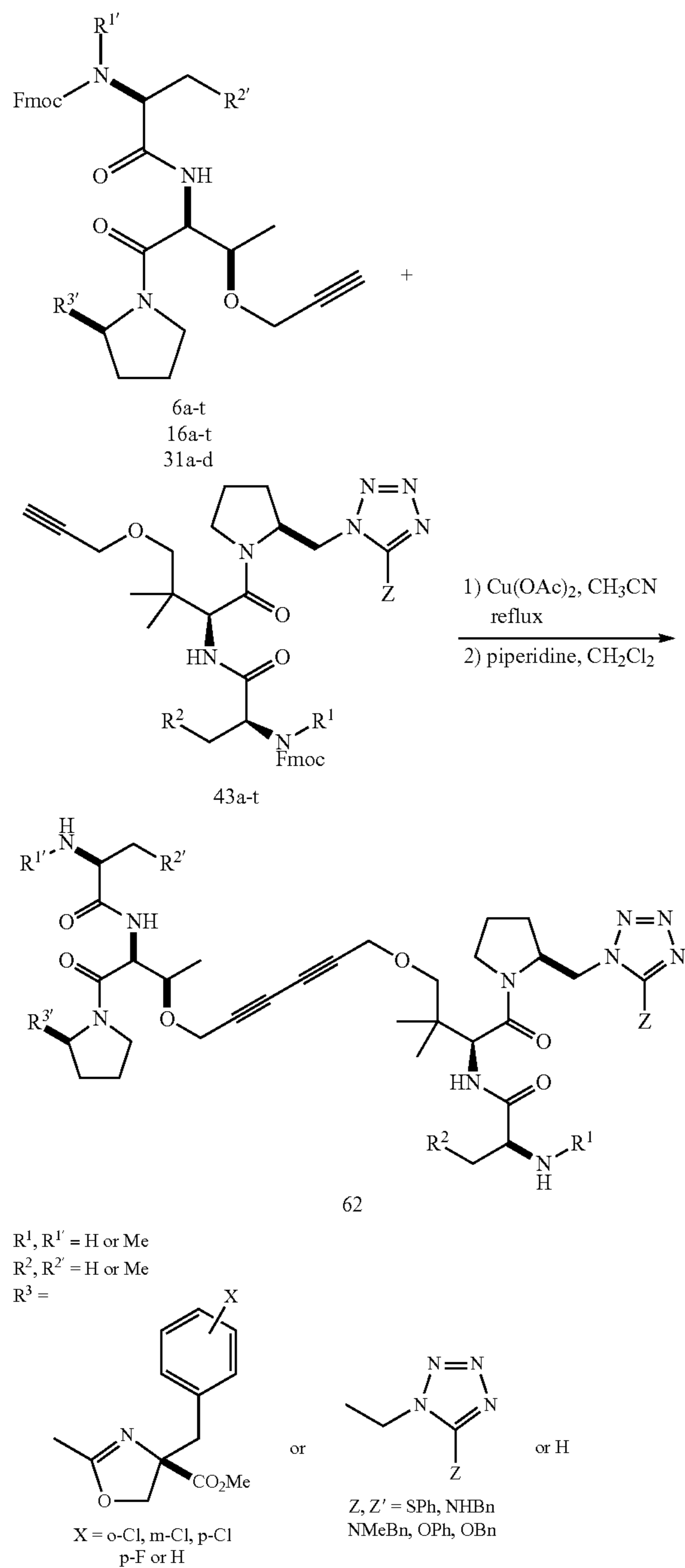
Scheme 17
