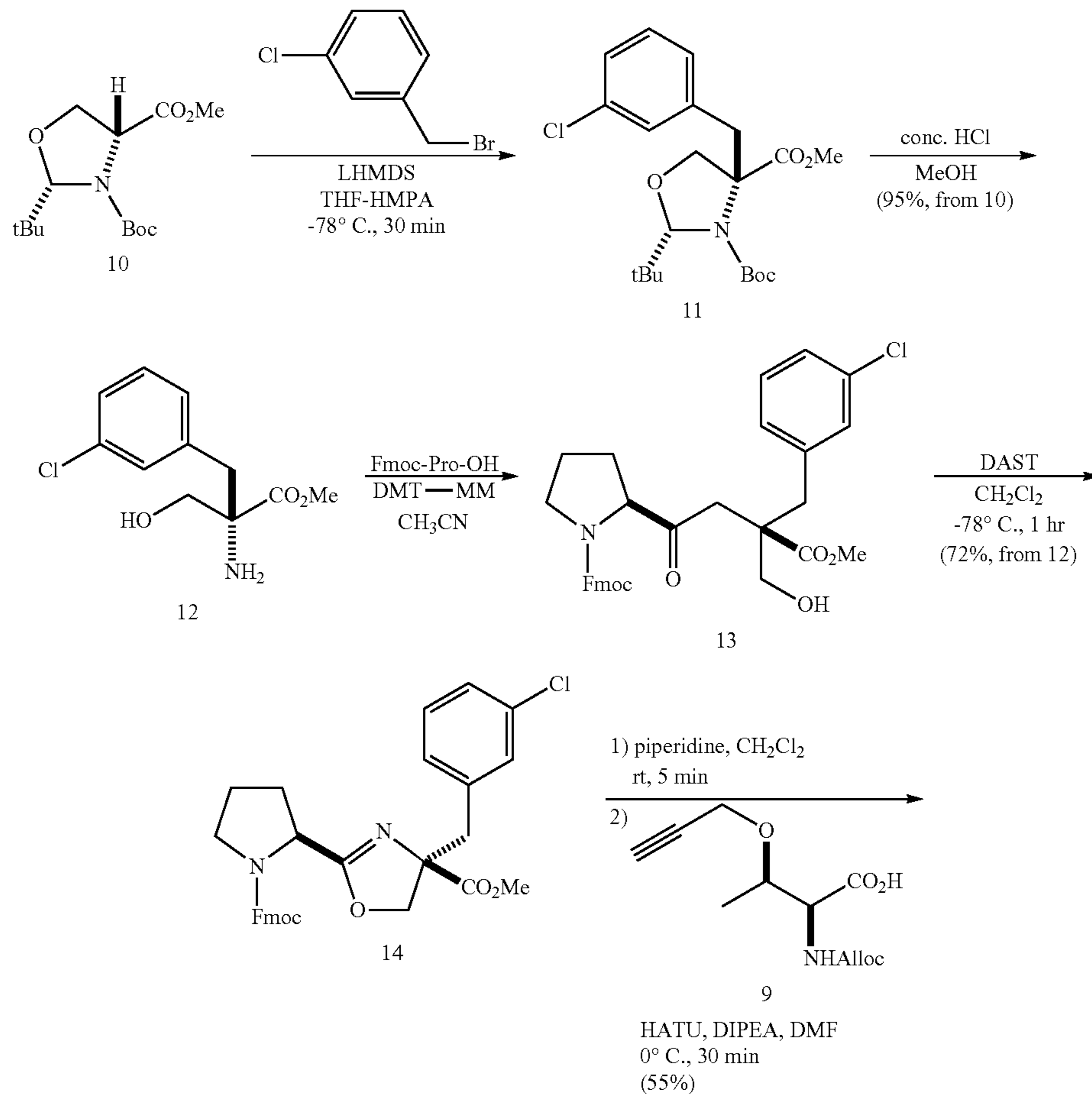
Scheme 6
