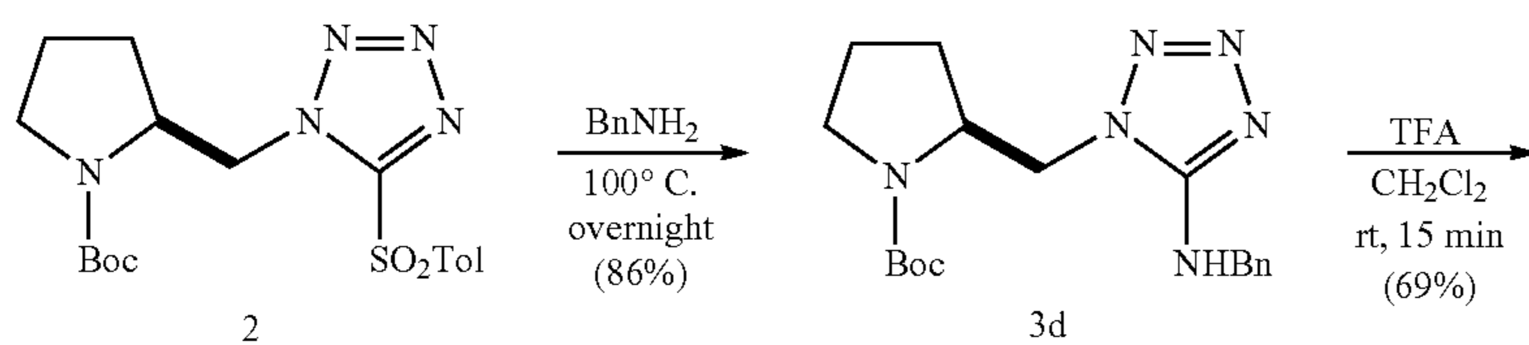
Scheme 4
