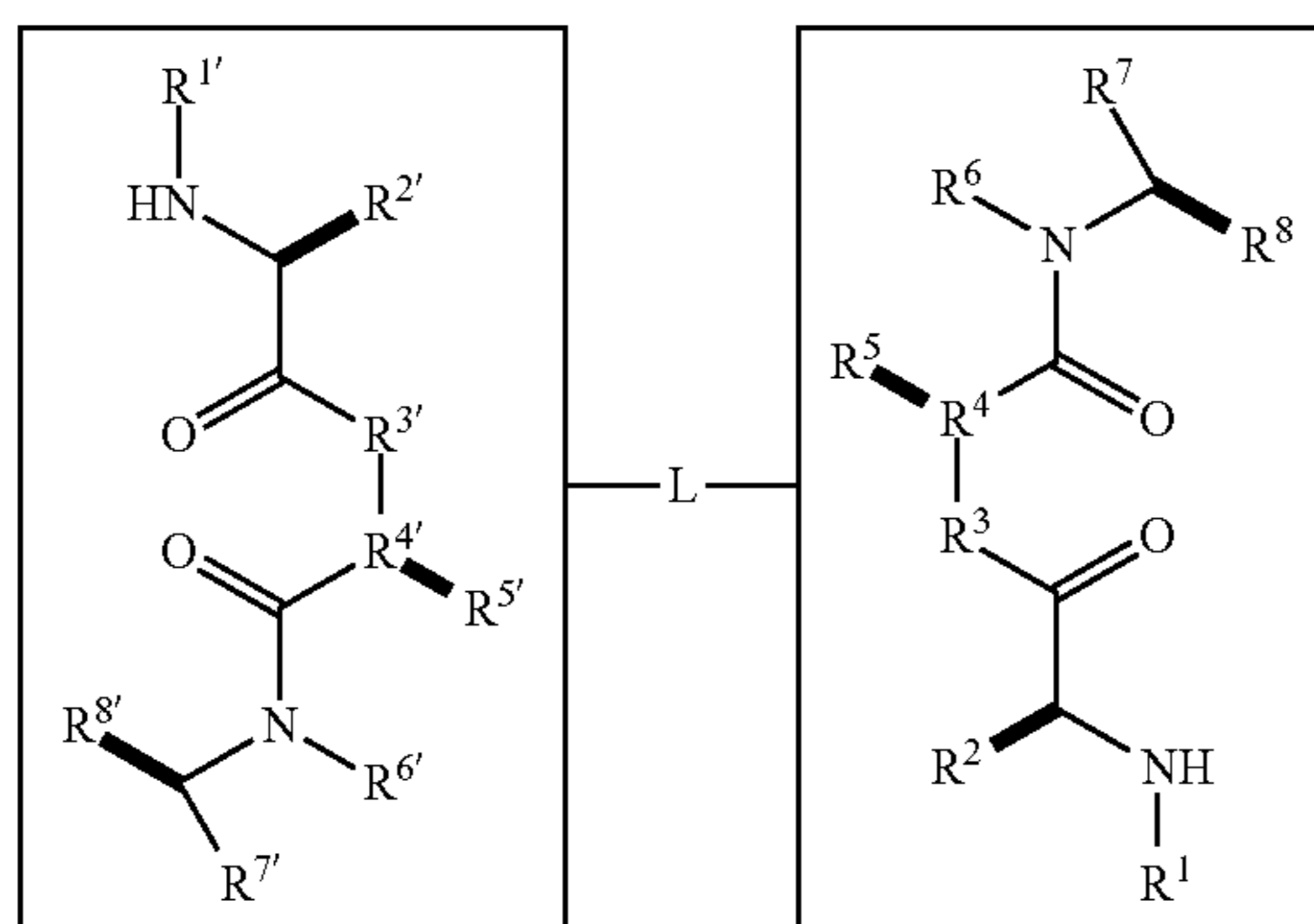
formula II
