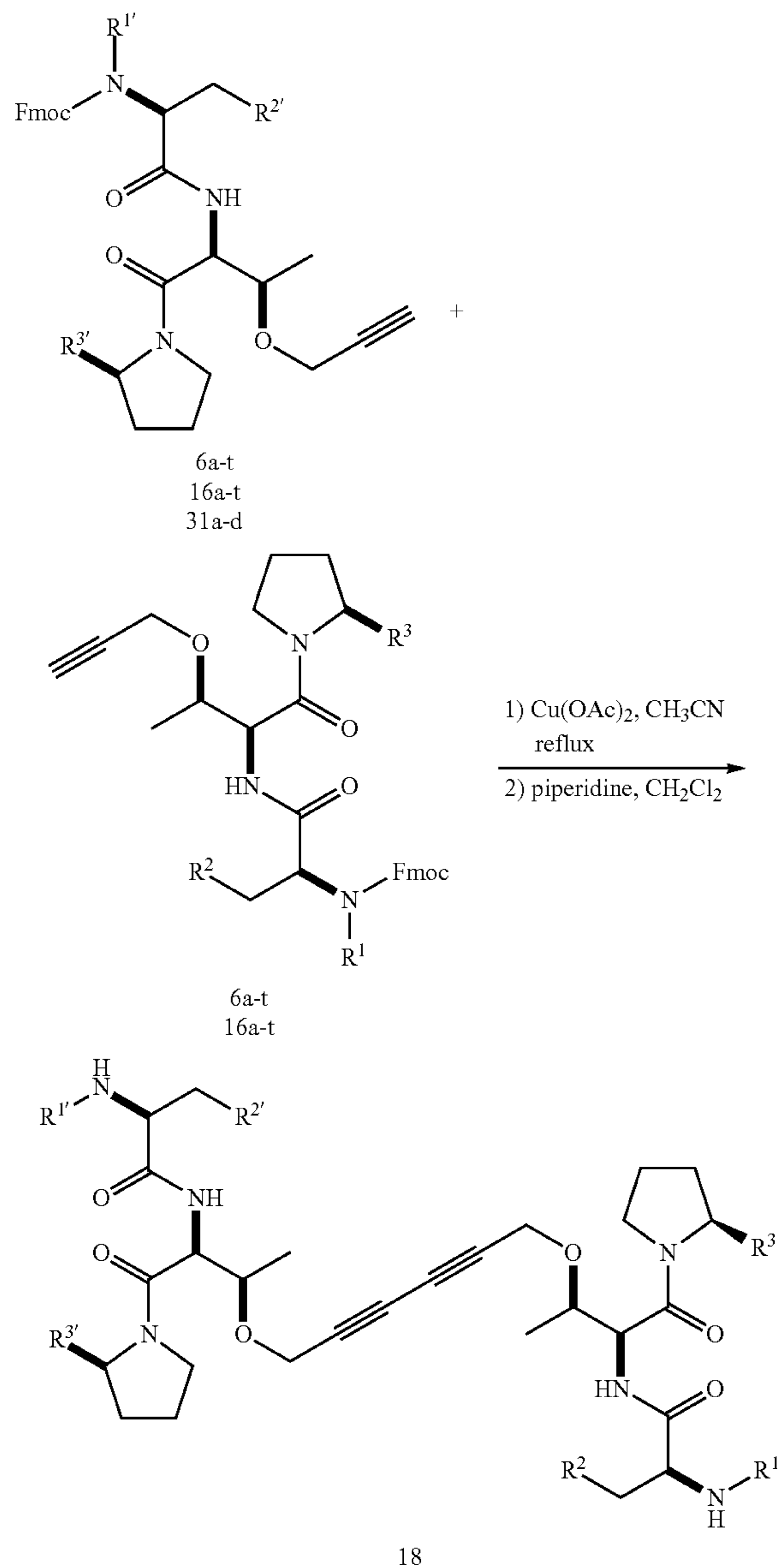
Scheme 12
