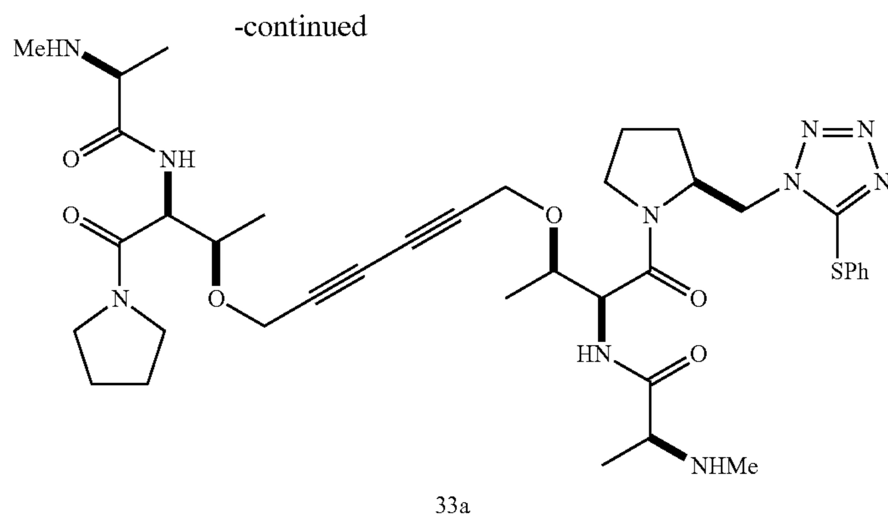
Compound 33a
