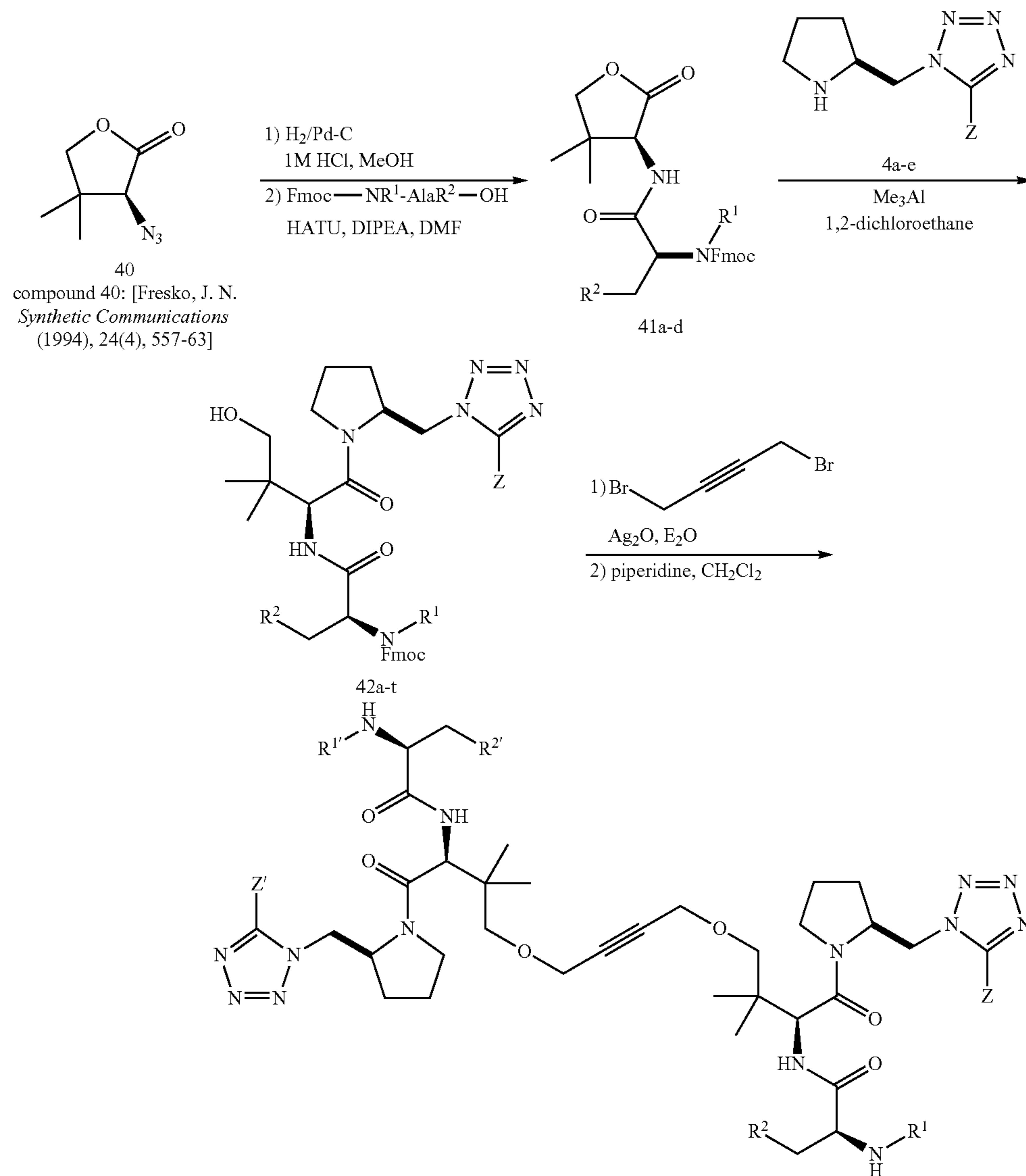
Scheme 14
