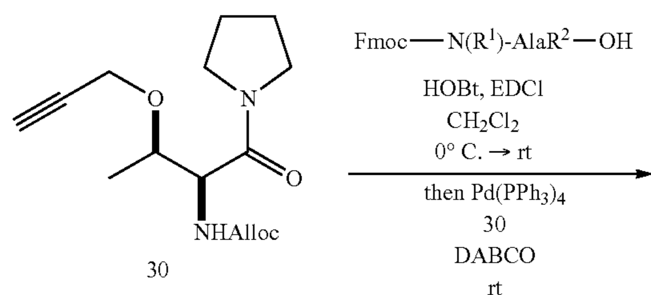
Scheme 11
