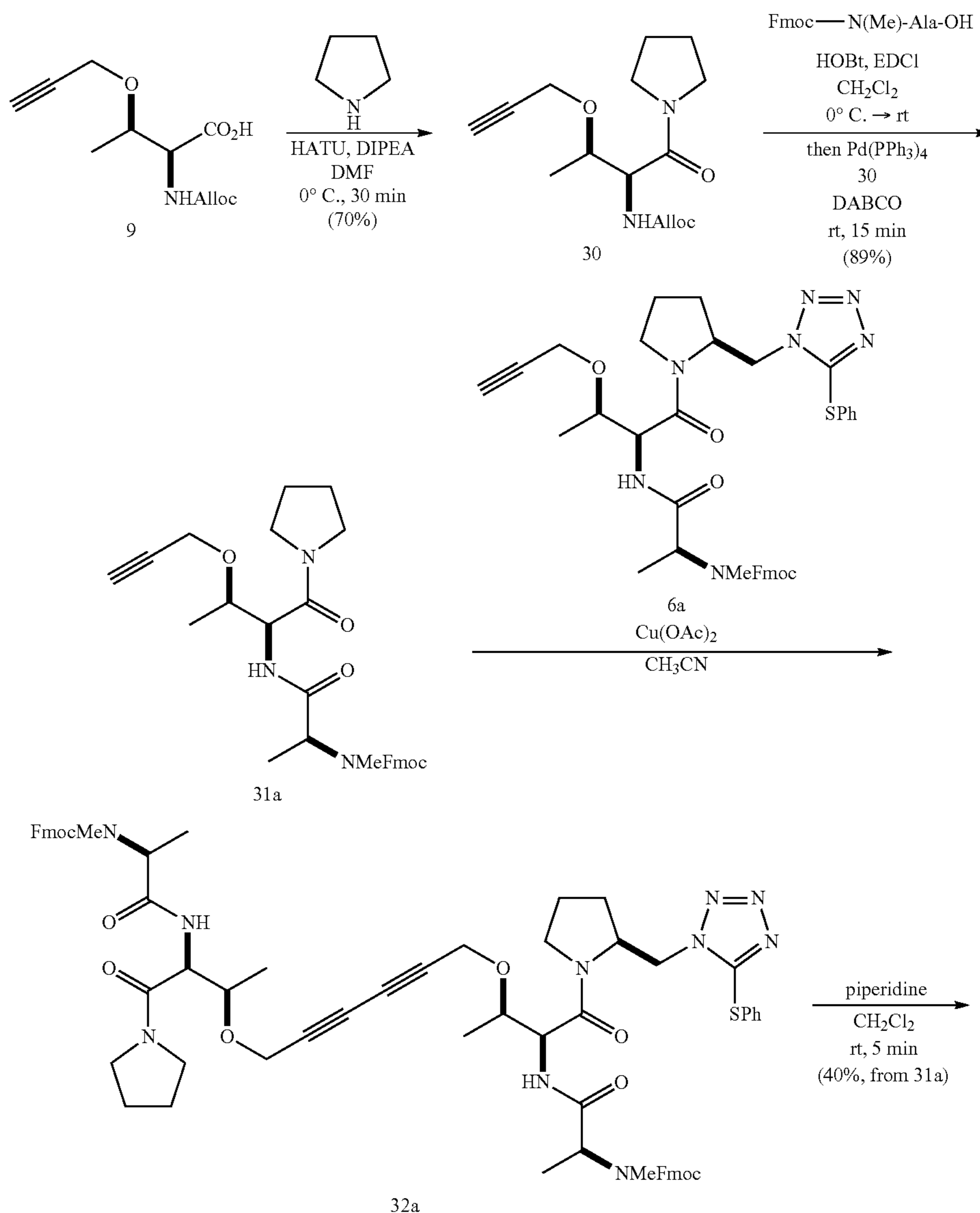
Scheme 8
