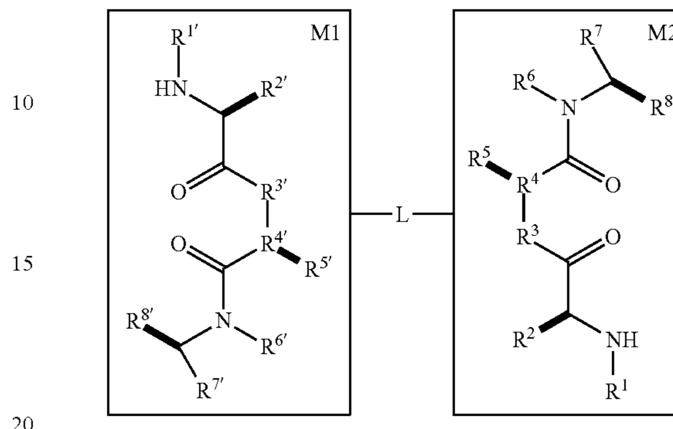
formula II
