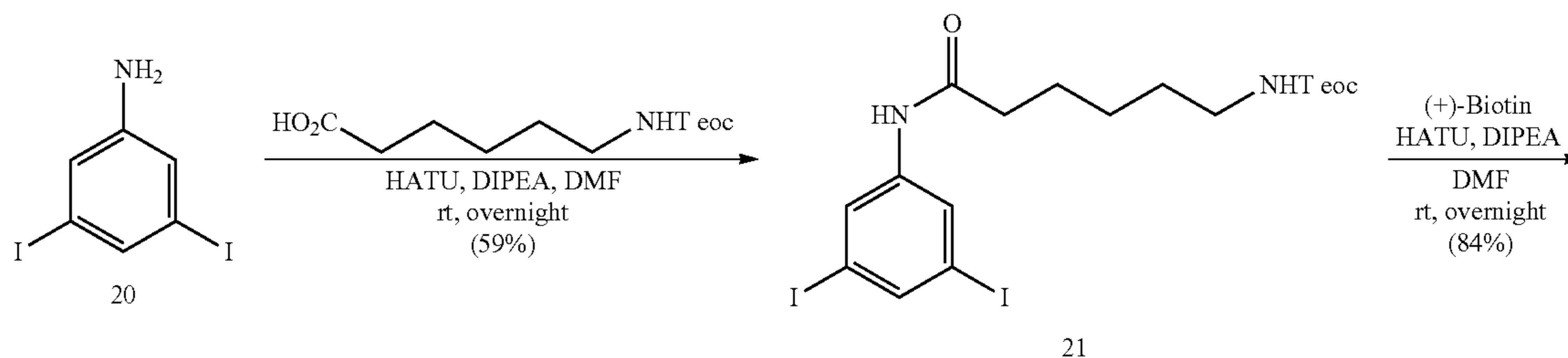
Scheme 7
