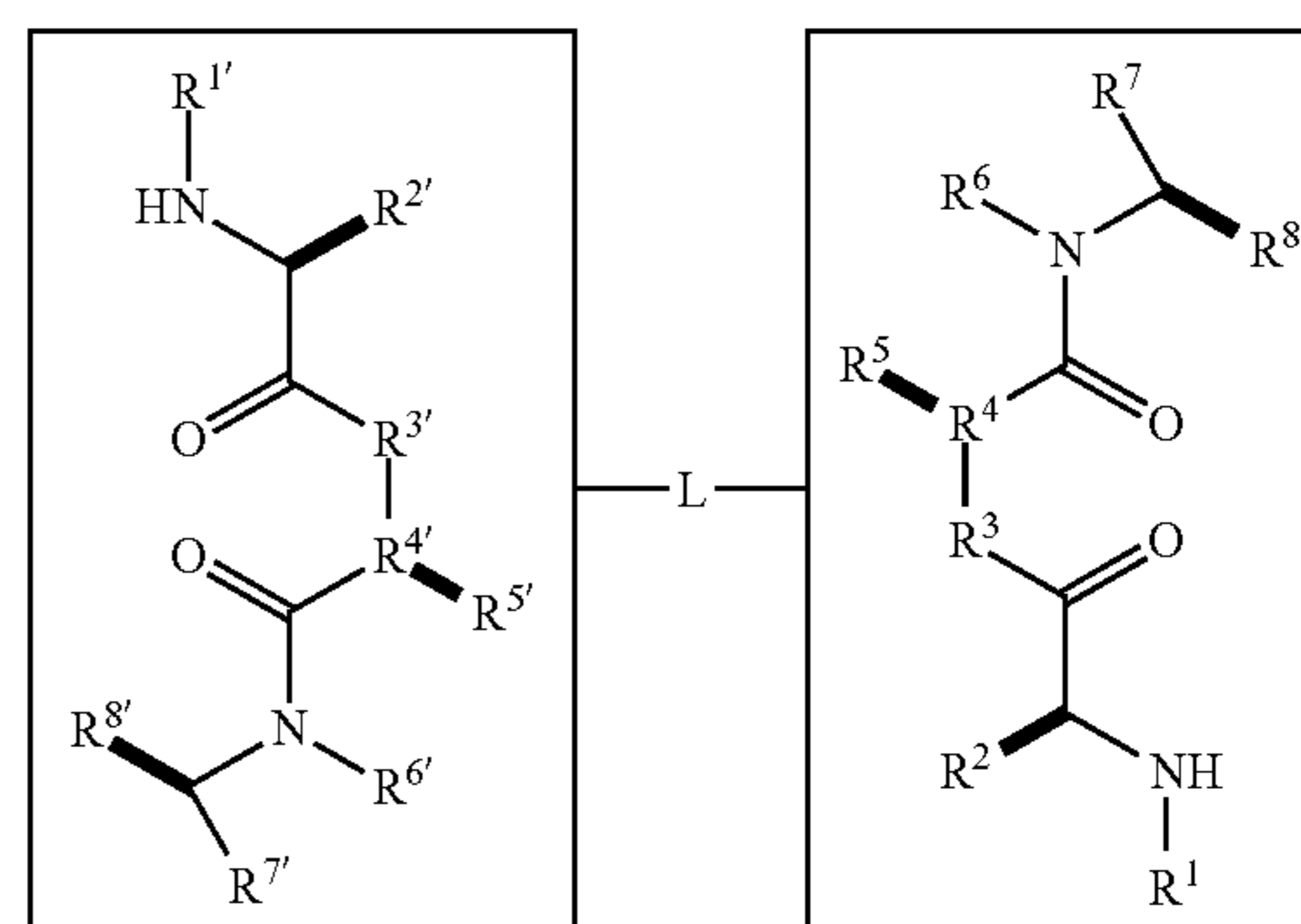
formula II
