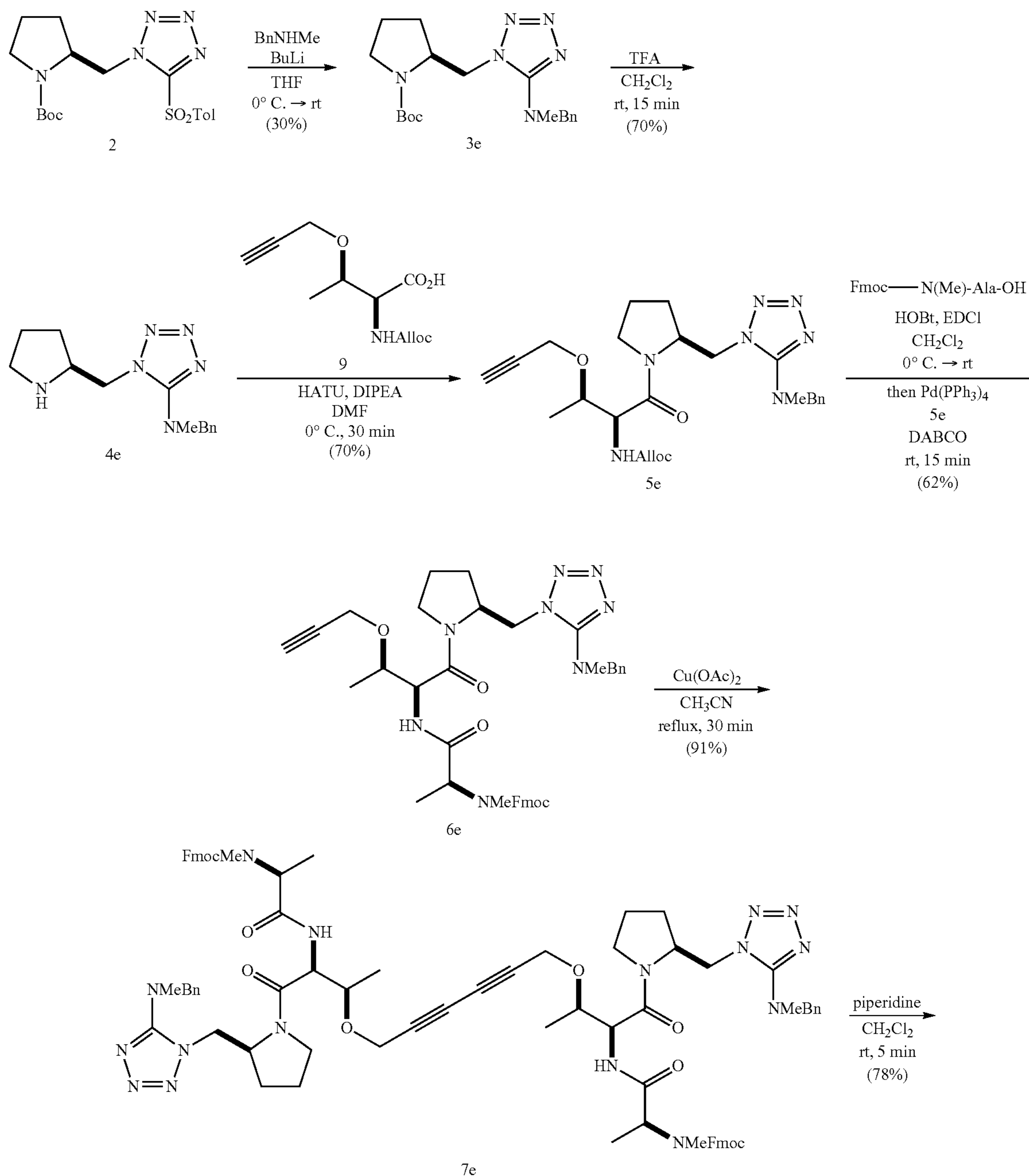
Scheme 5
