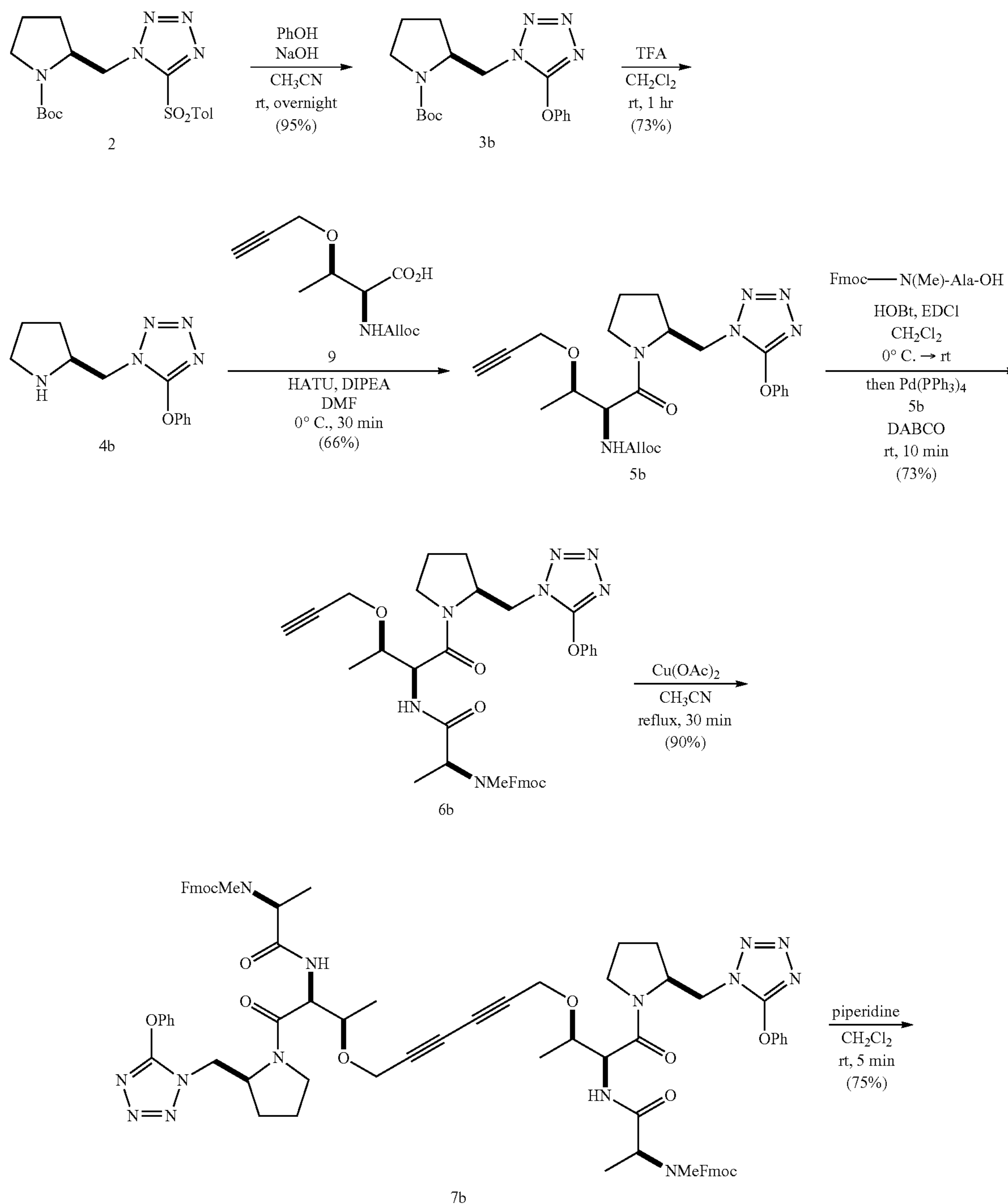
Scheme 2
