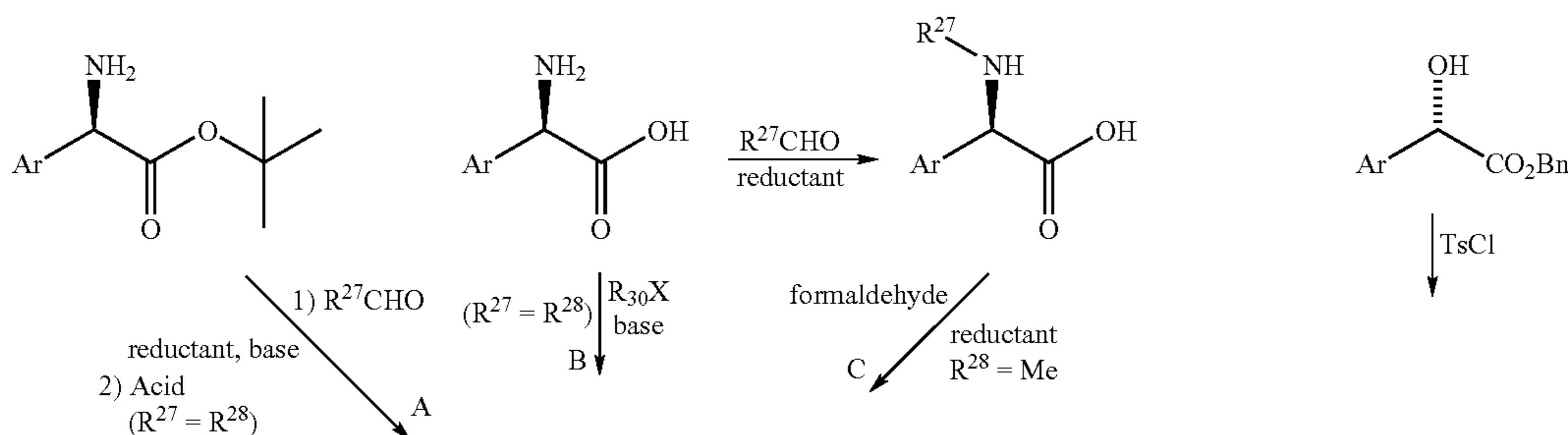
Scheme 2: Acylated Amino Acid Derivatives
