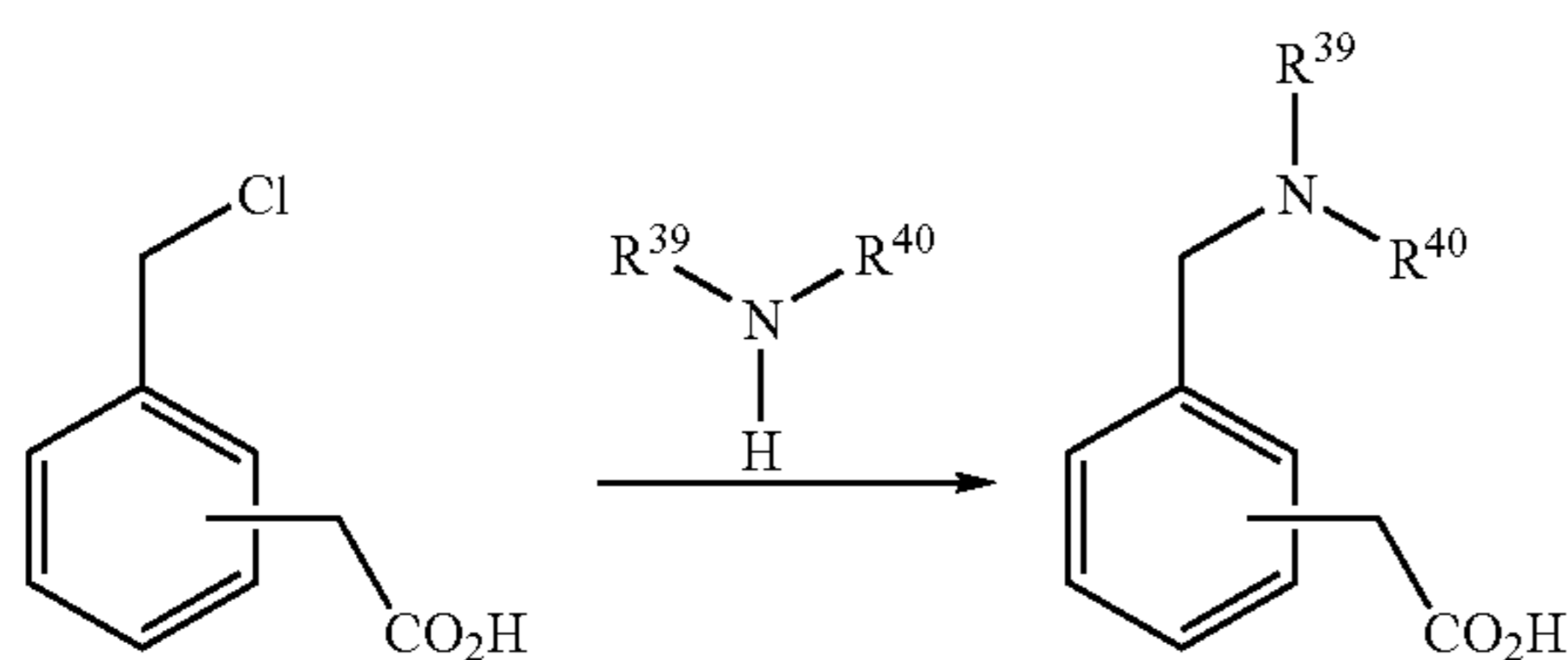
Synthesis of Common Acid Precursors
