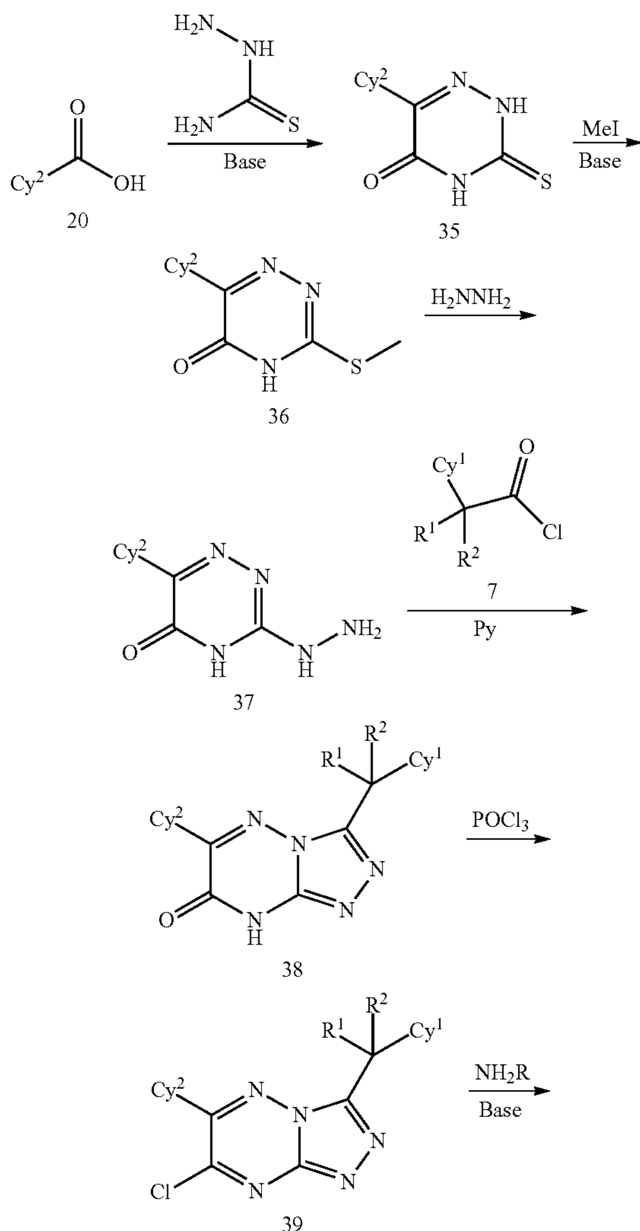
Scheme 9
