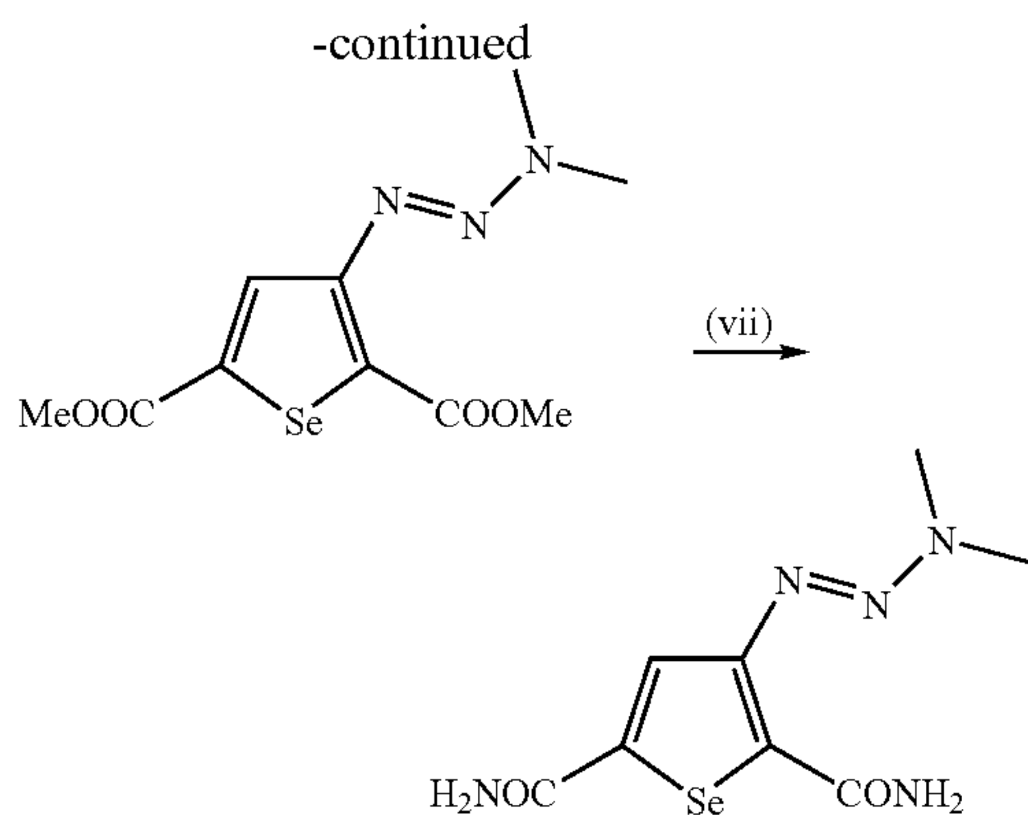
Compound 2
