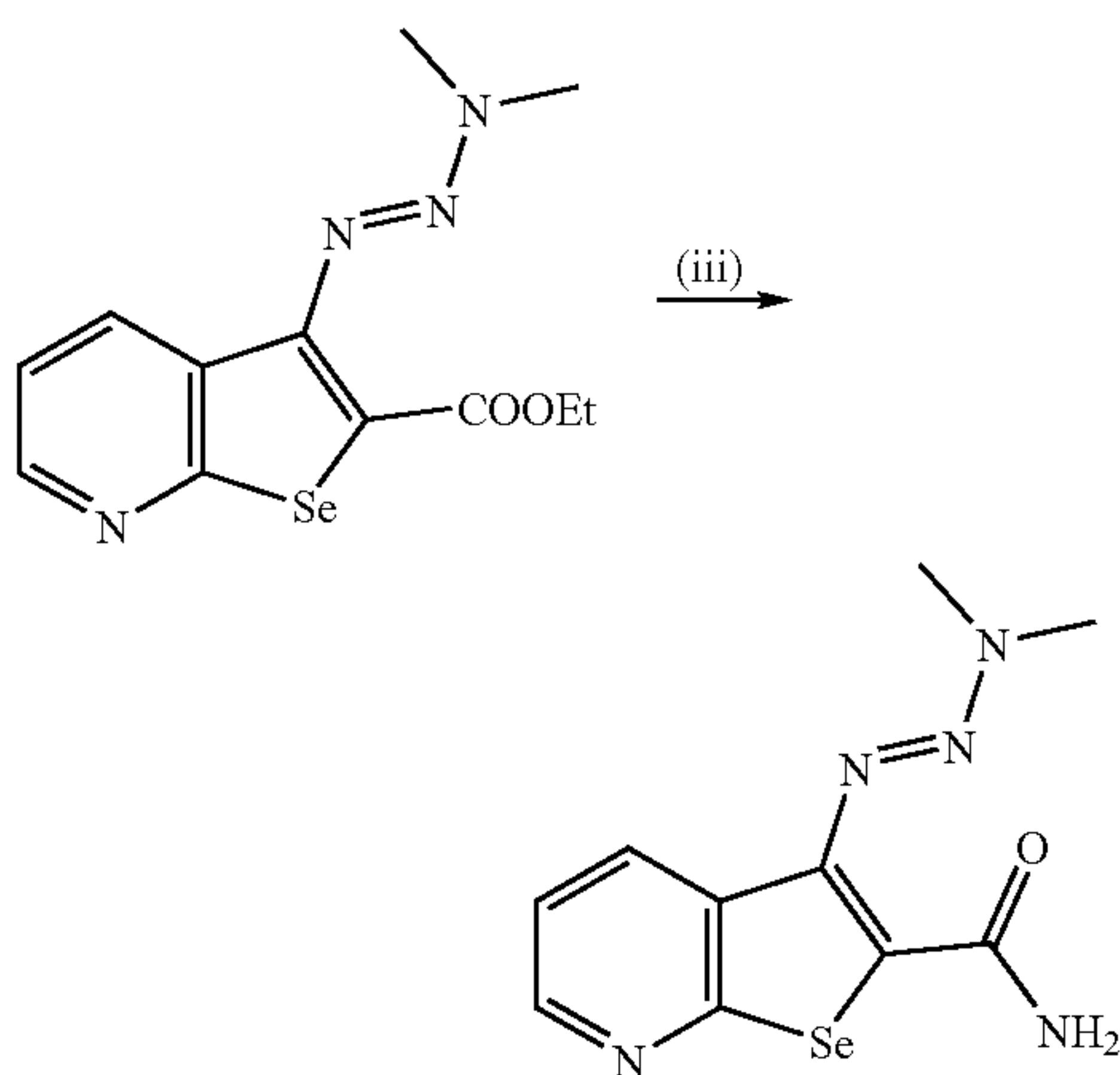
Compound 6
