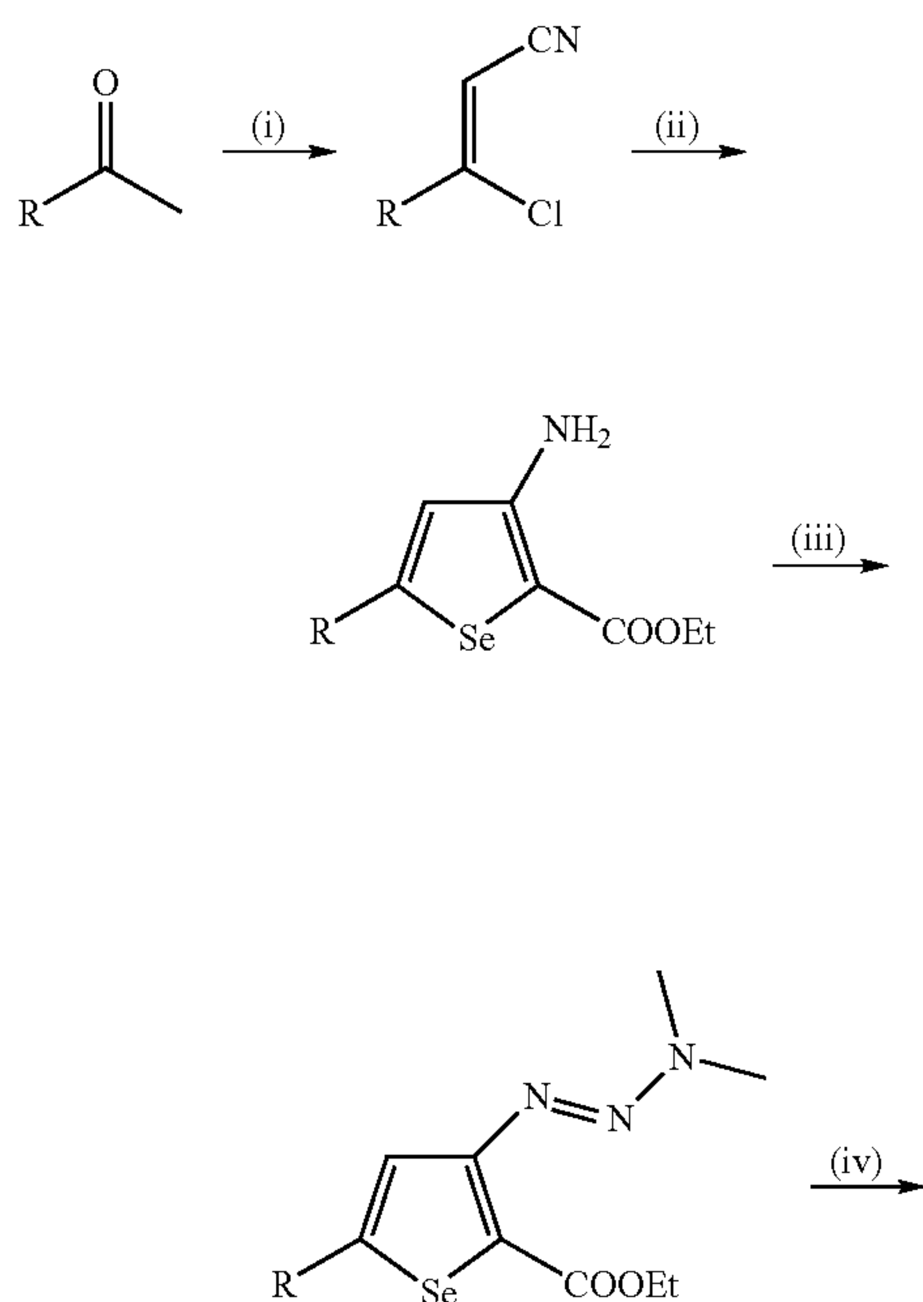
Scheme-C
