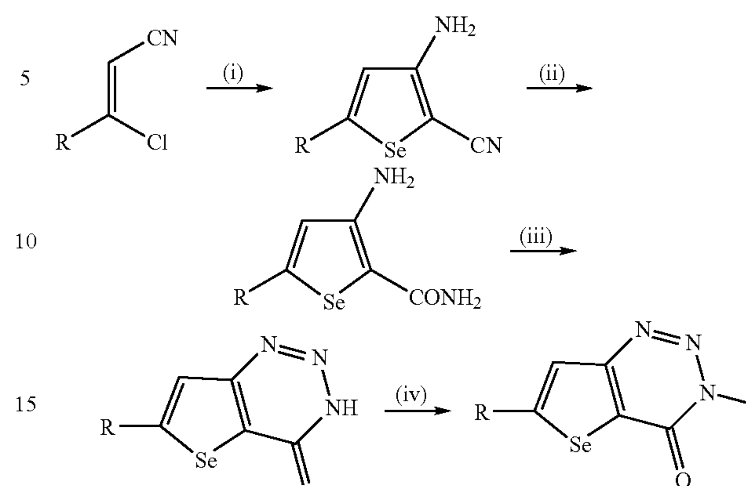
Compound 12: R = Ph Compound 13: R = tert-butyl
