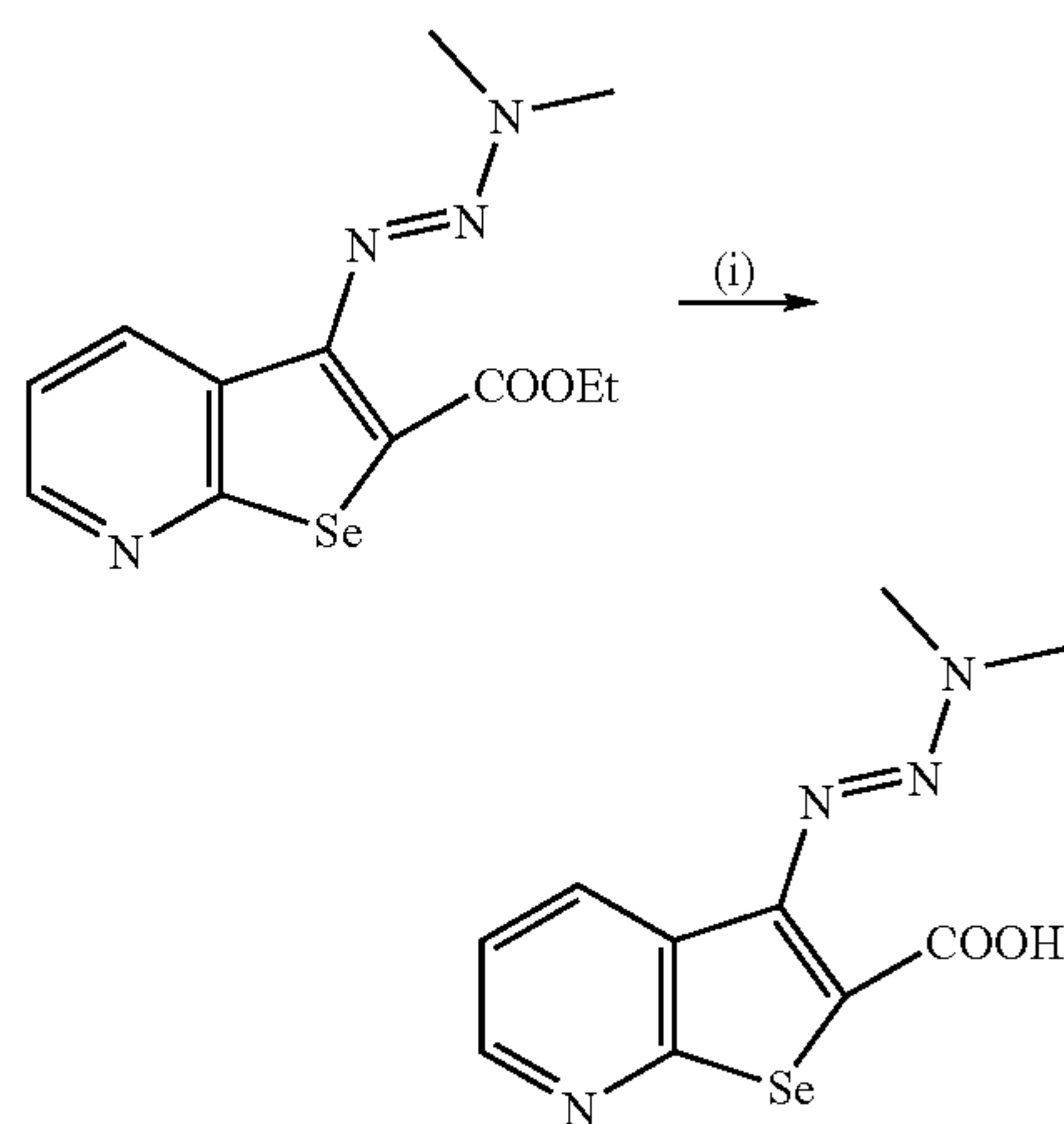
Compound 10
