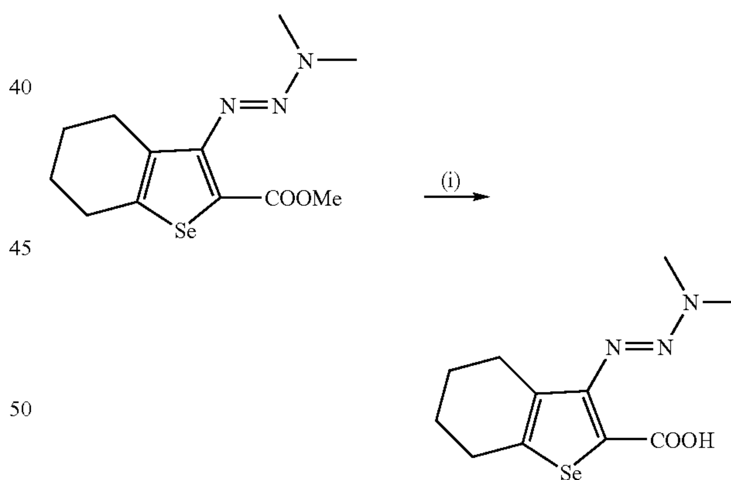
Compound 9
