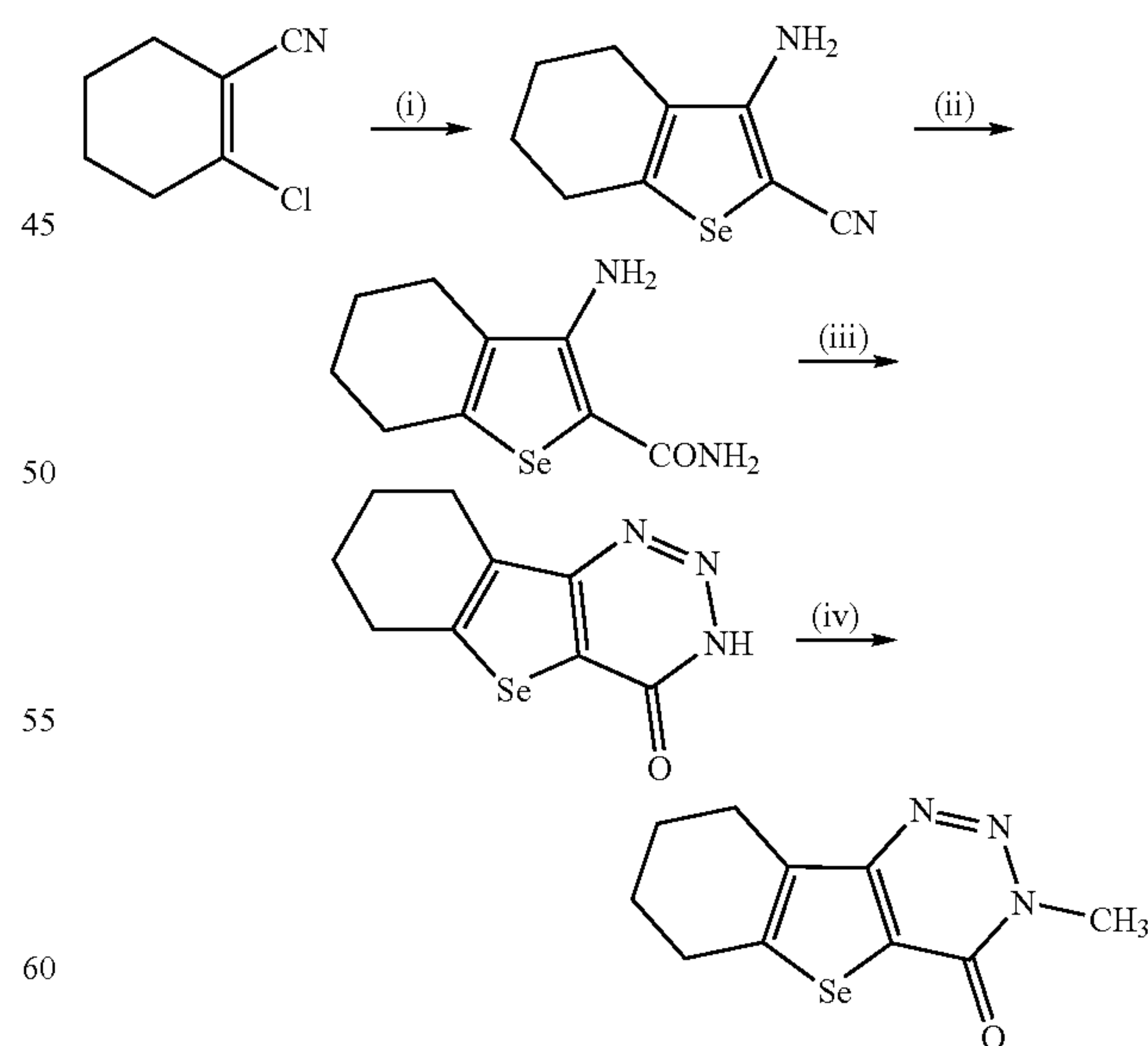
Compound 14
