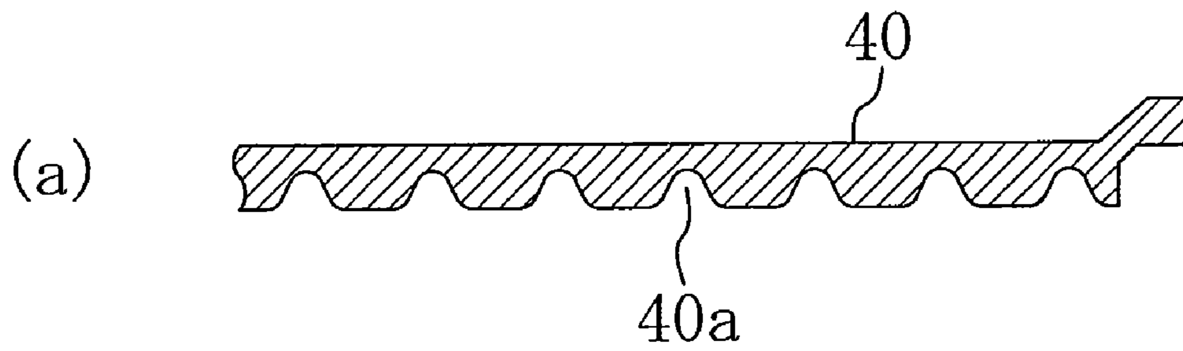
FIG. 16 PRIOR ART
