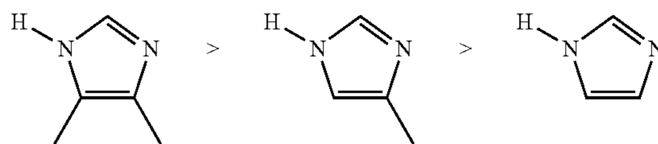
Ligand Field Strength
