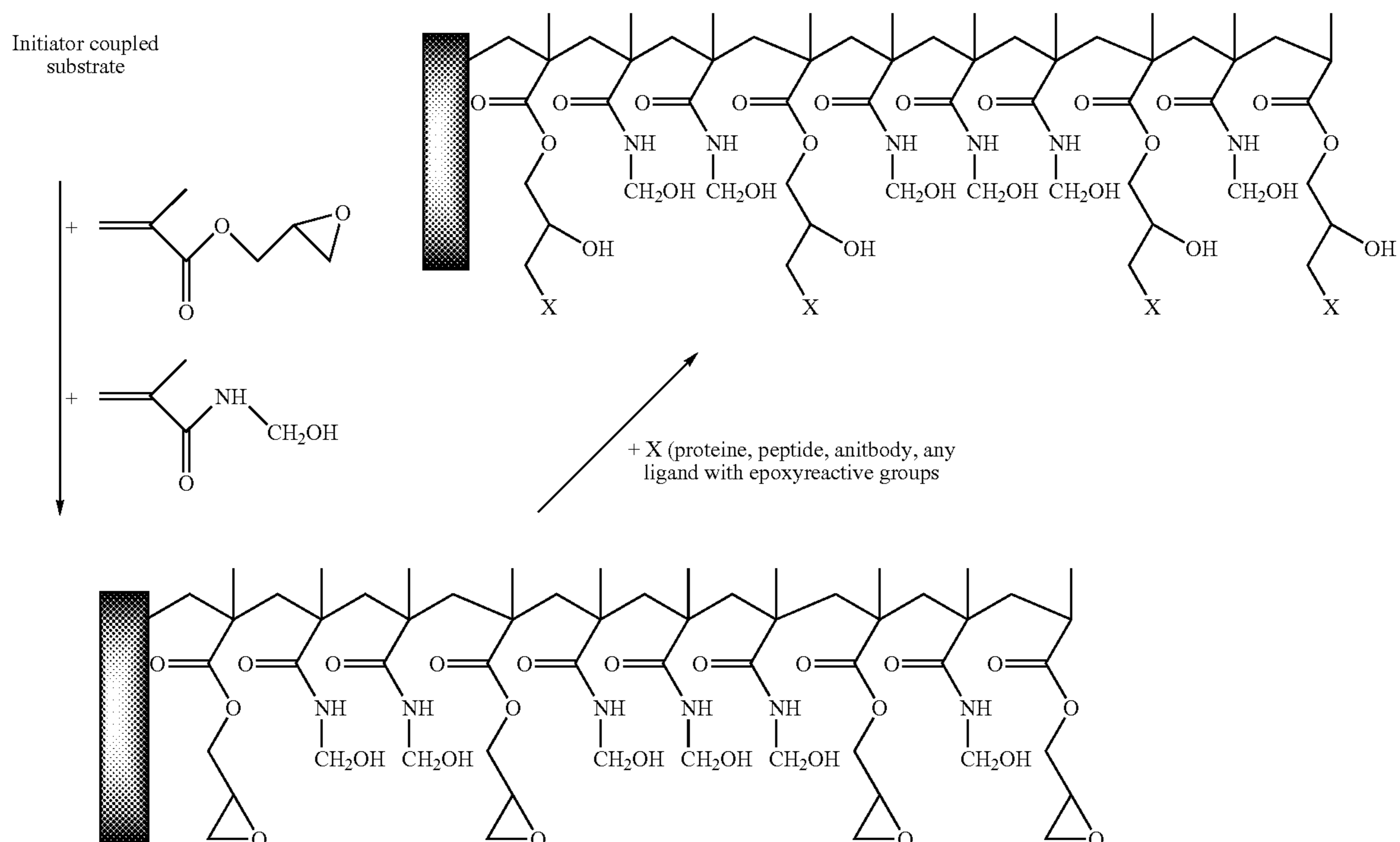
Reaction scheme 3
