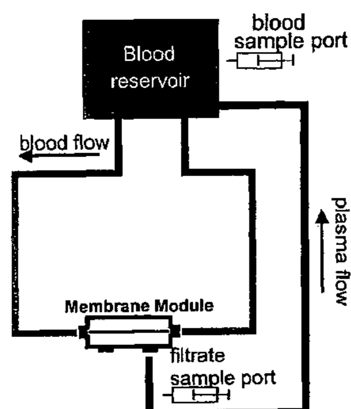
Experimental set-up for dynamic Endotoxin adsorption of grafted membranes from citrate-anticoagulated human blood (Example 10)
