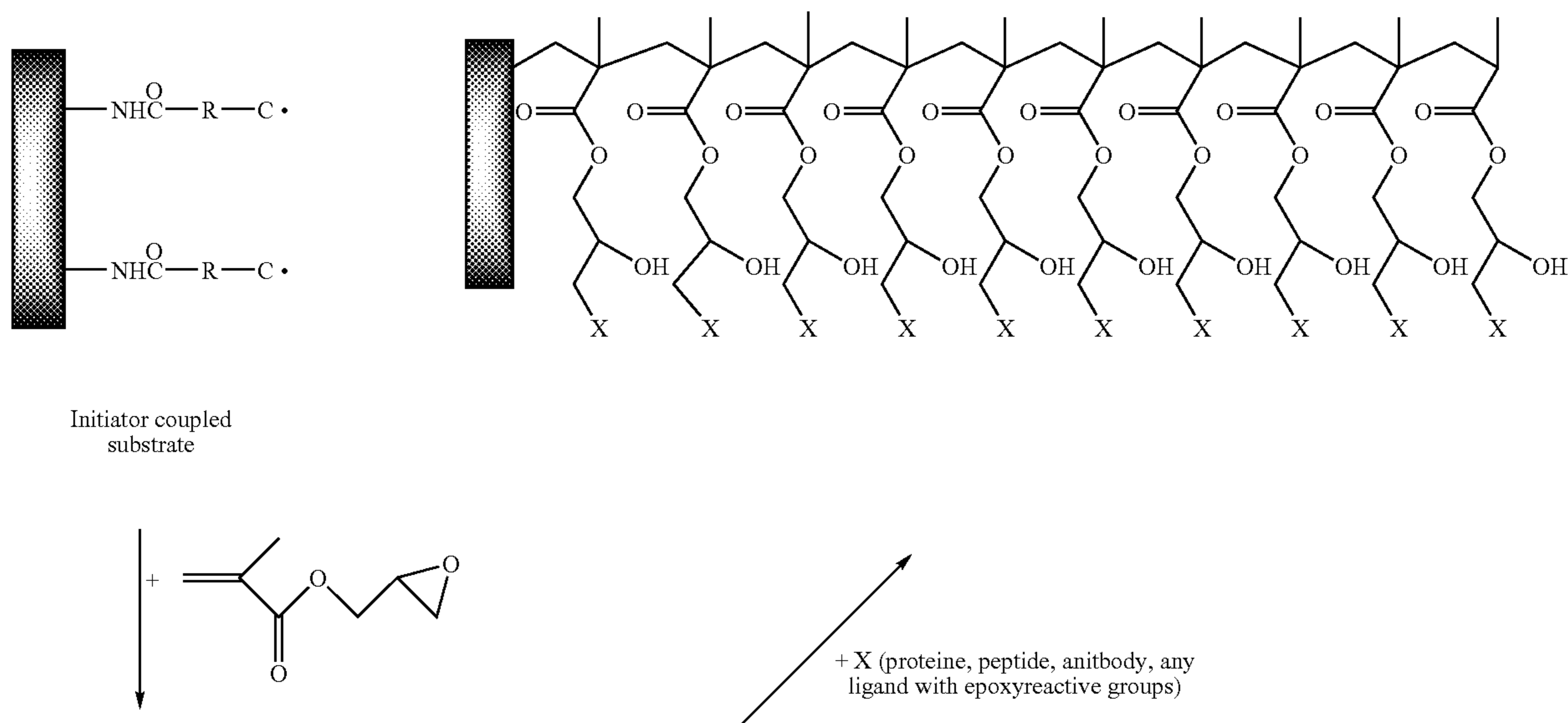
Reaction scheme 2
