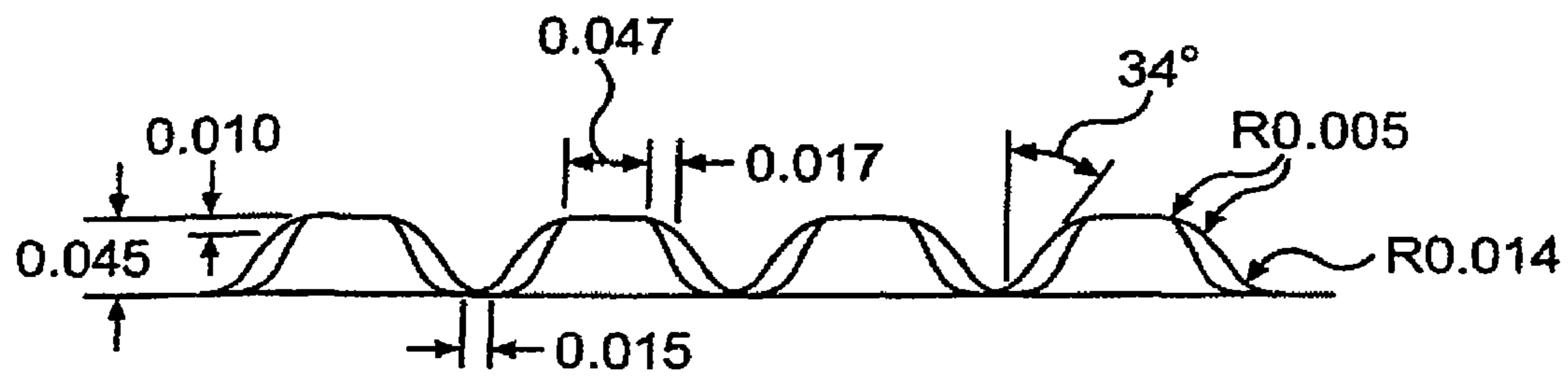
SIDE VIEW
