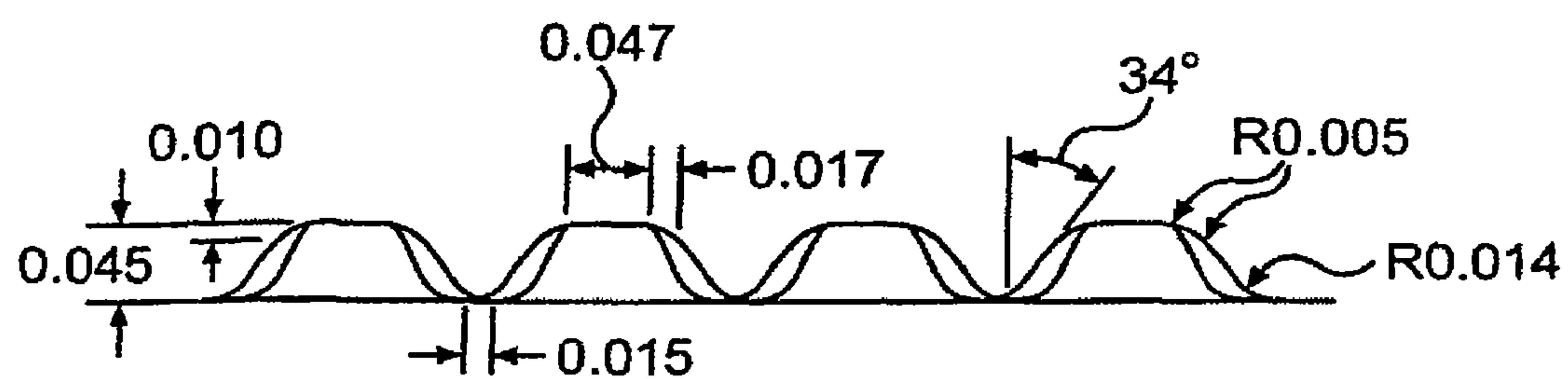
SIDE VIEW
