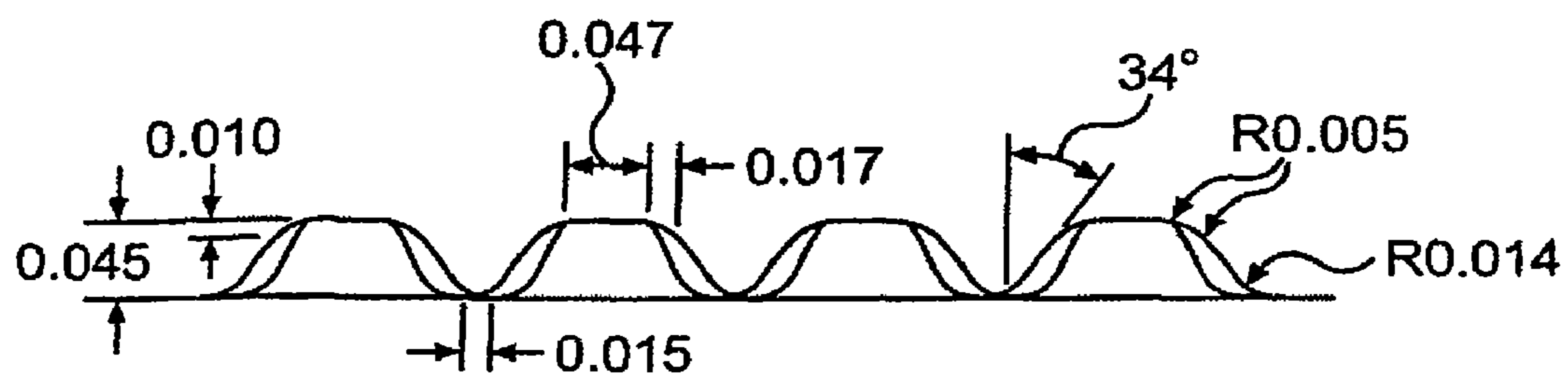
SIDE VIEW
