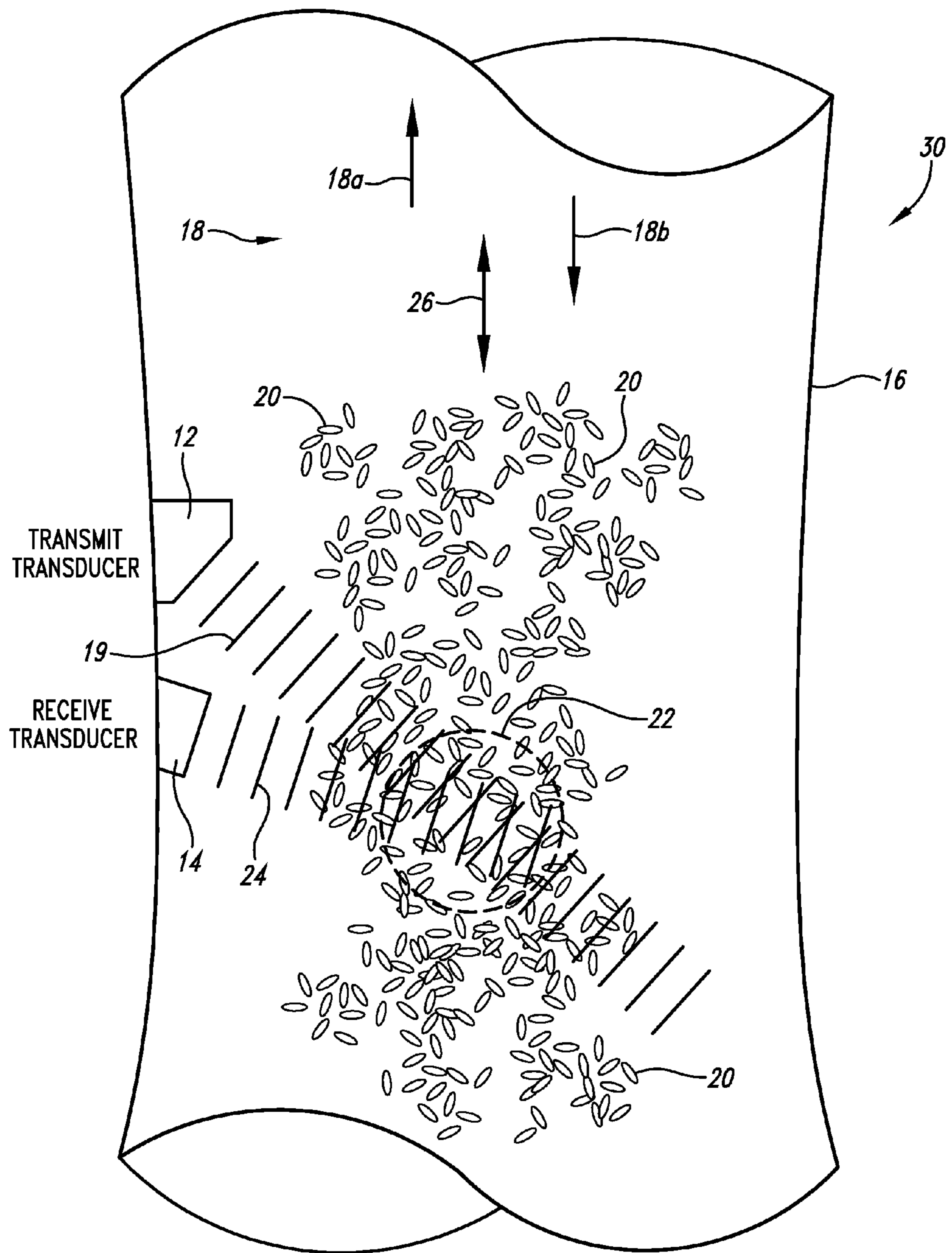
Fig. 2 (Prior Art)
