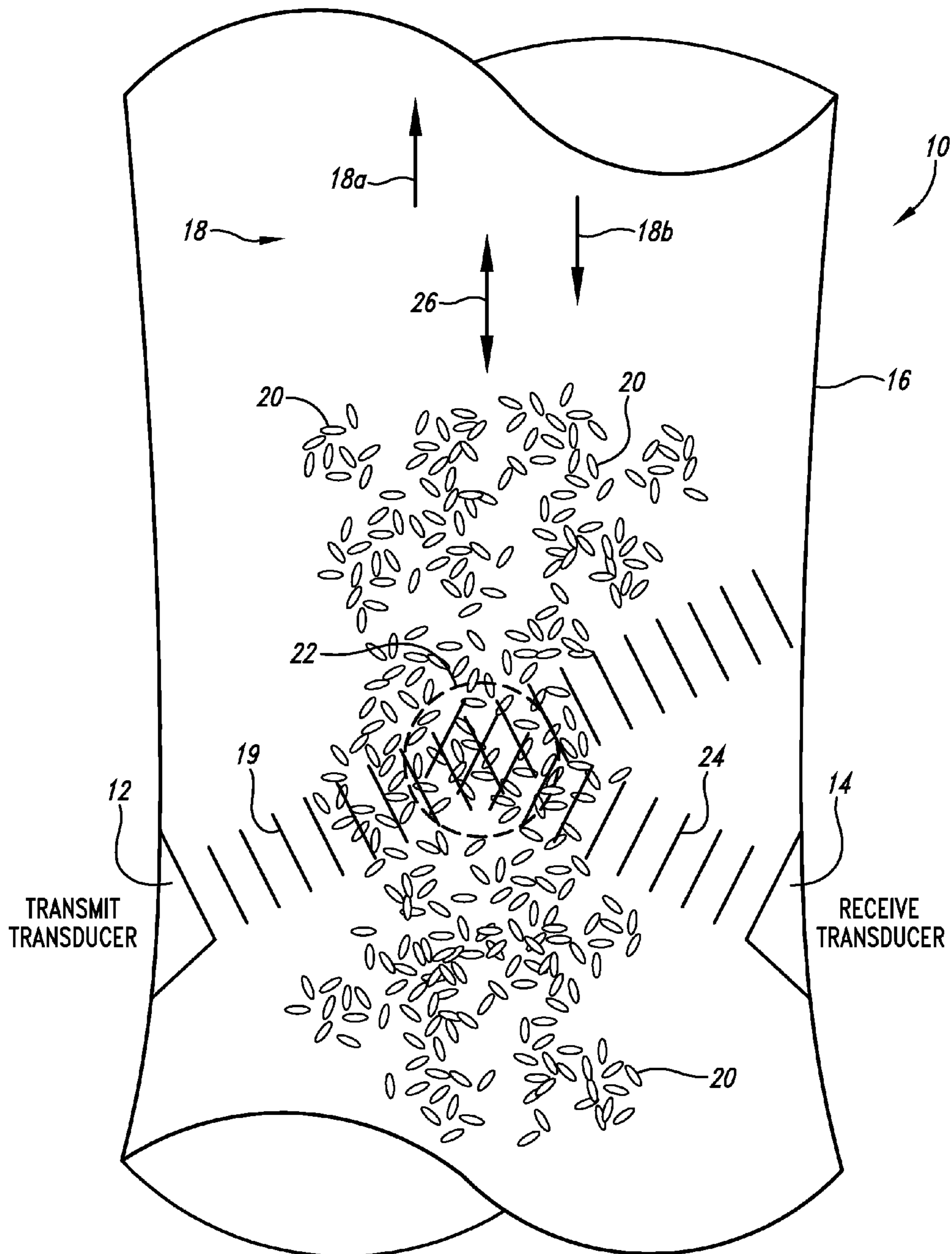
Fig. 1 (Prior Art)
