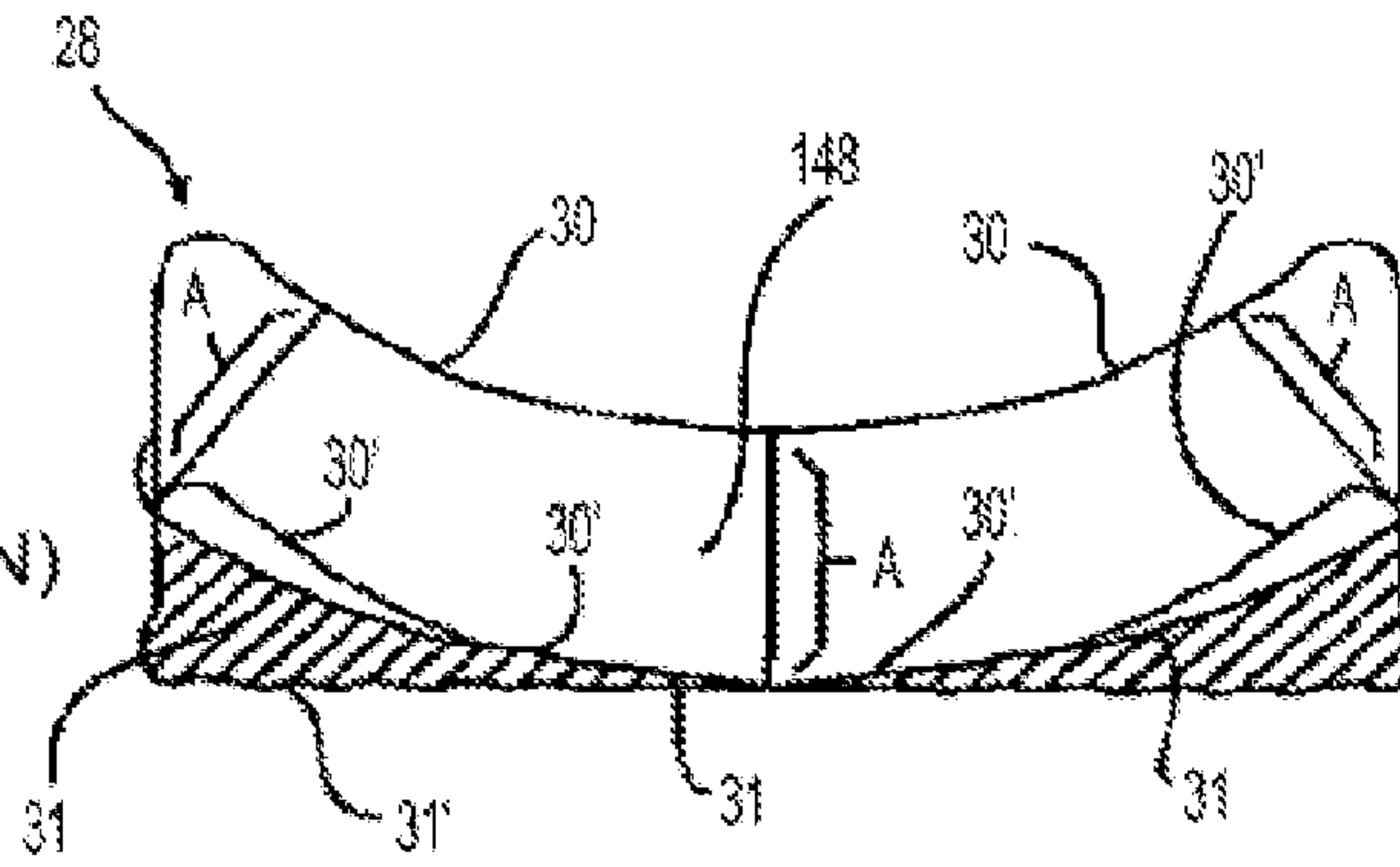
FIG. 78A PRIOR ART
