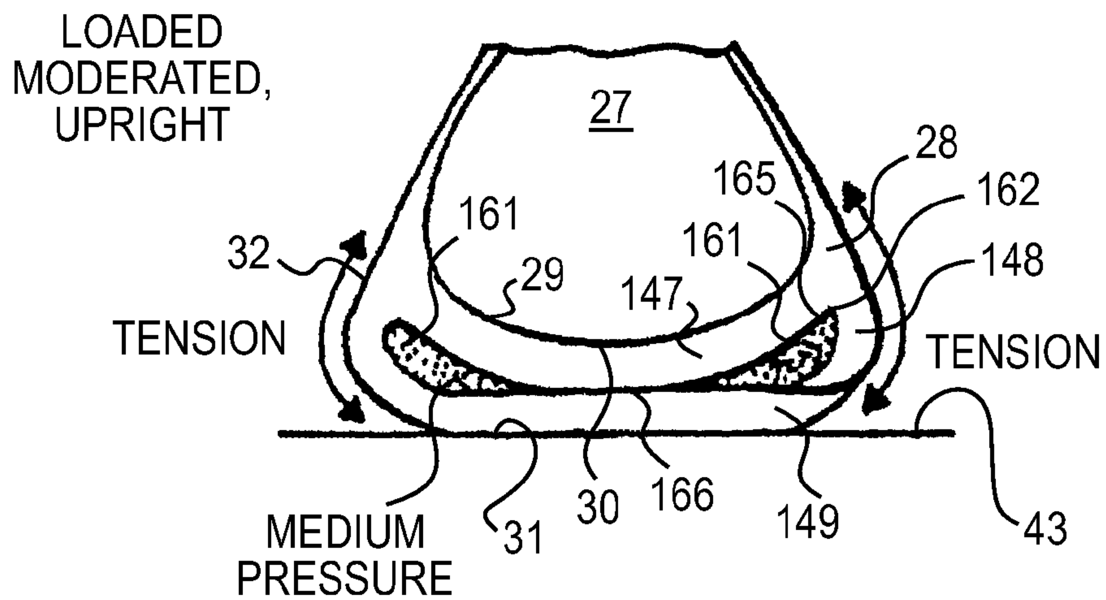
FIG. 9B PRIOR ART
