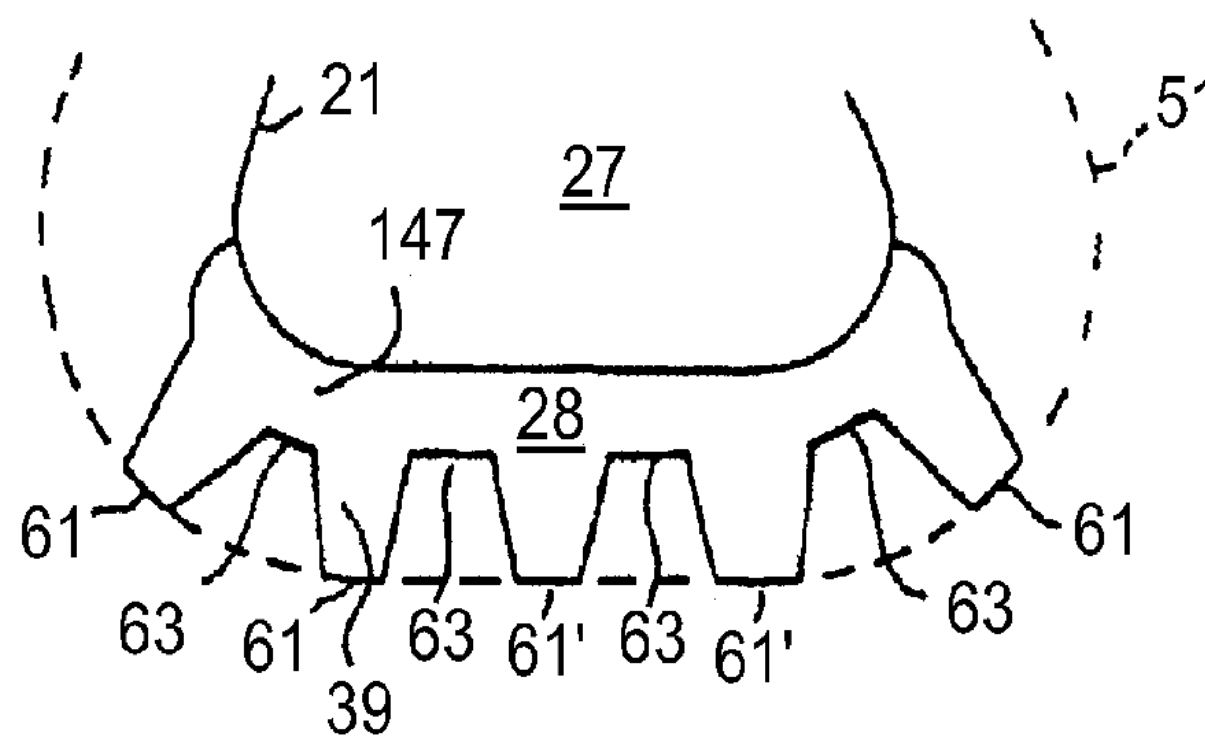
FIG. 35B PRIOR ART
