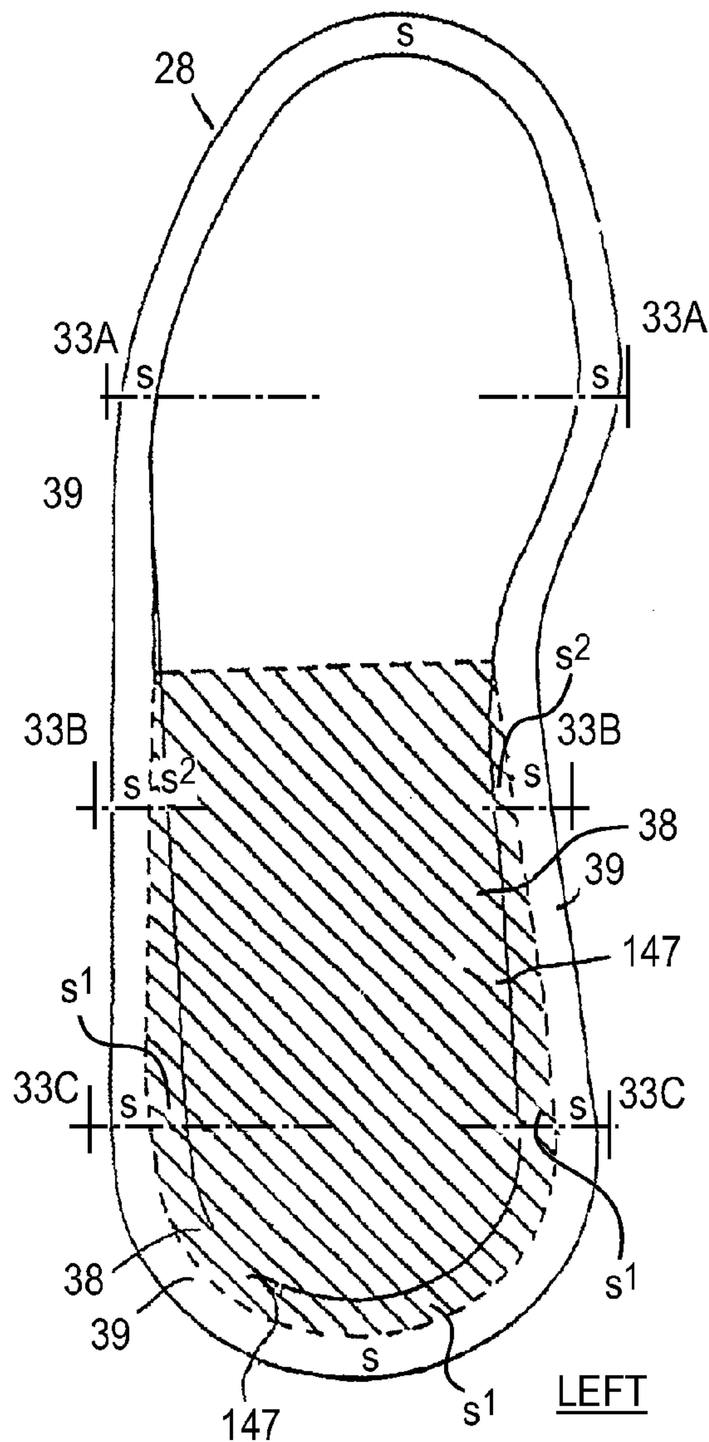
FIG. 33D PRIOR ART
