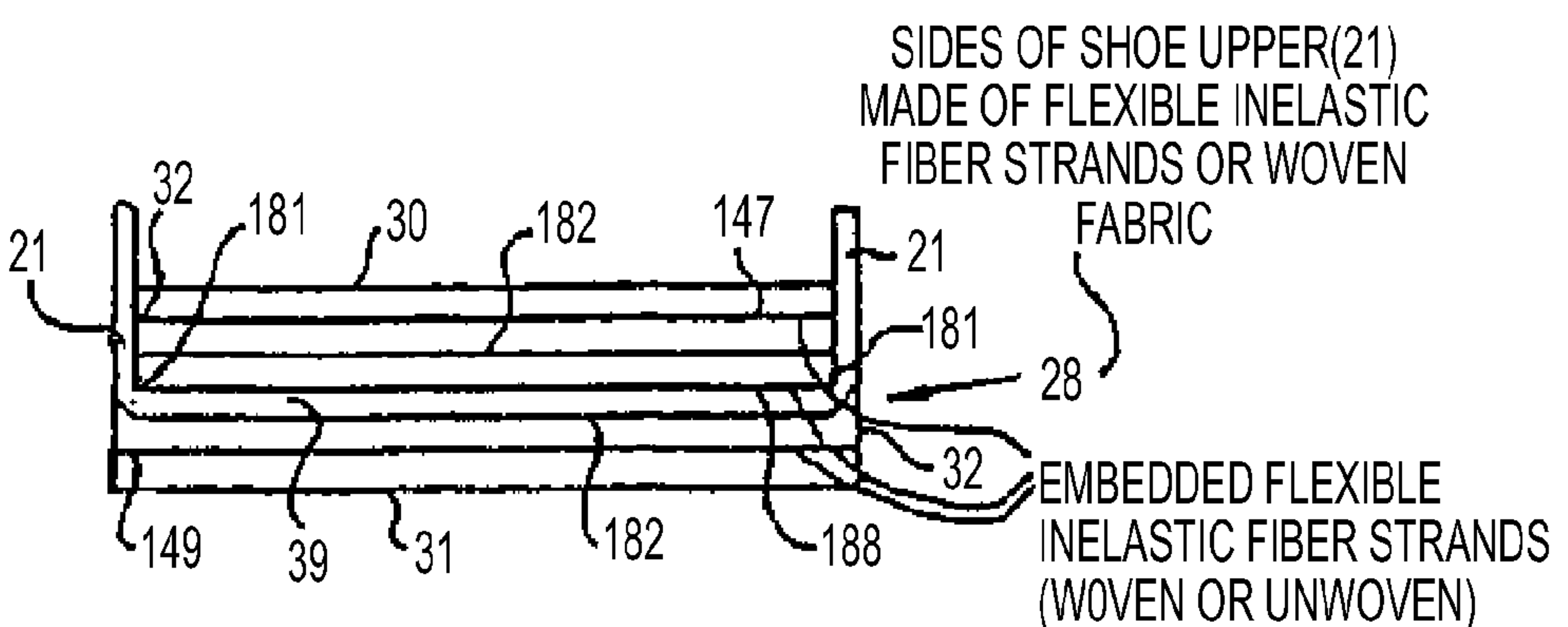
FIG. 60A PRIOR ART
