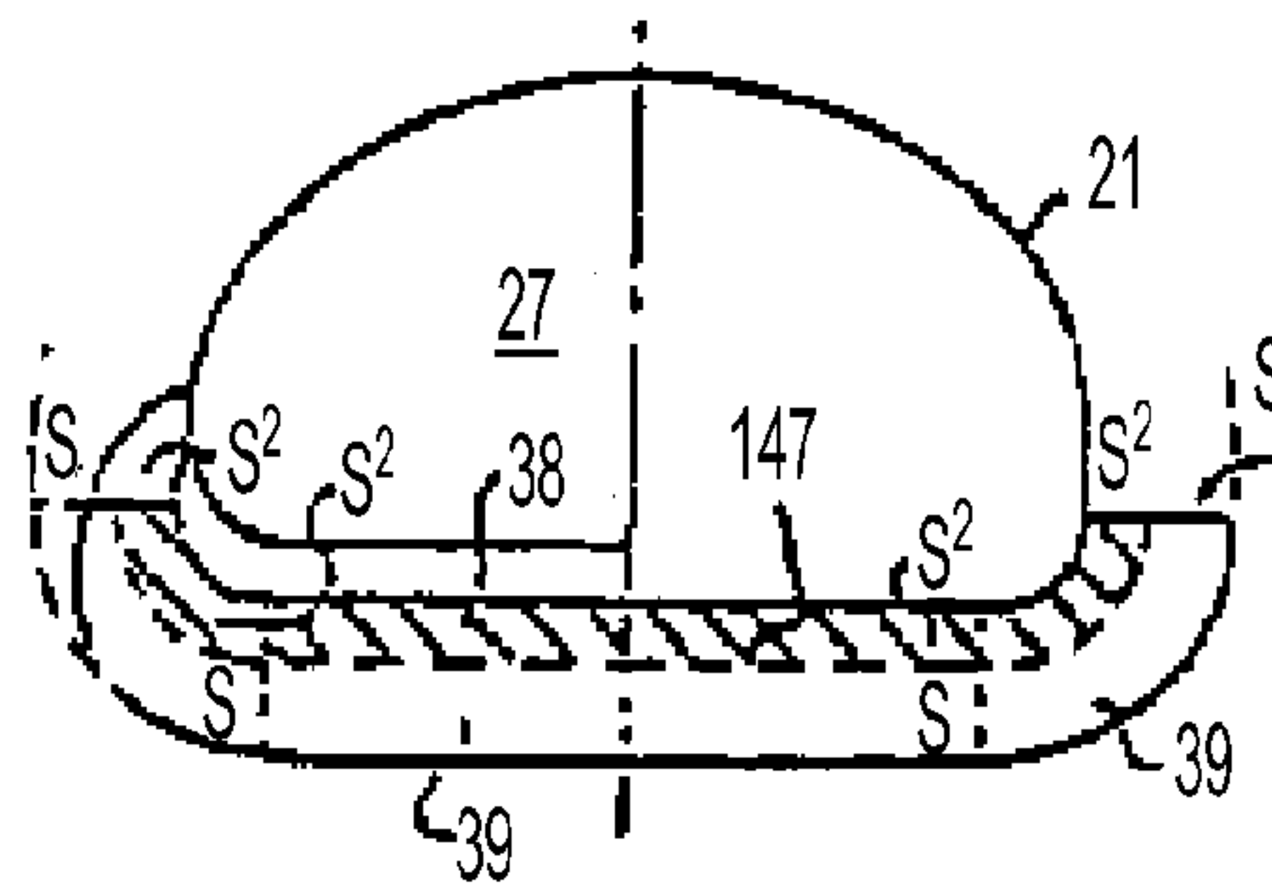
FIG. 69B PRIOR ART
