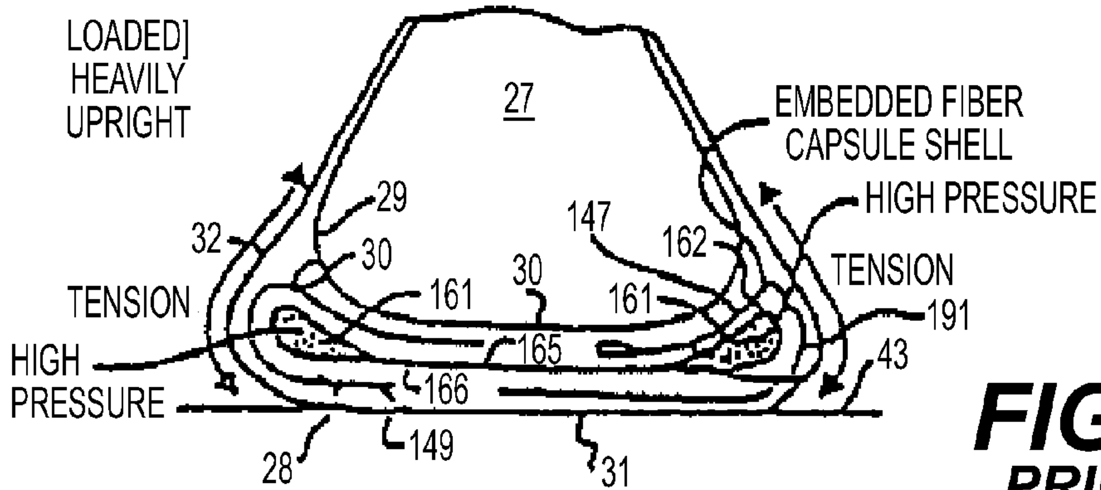
FIG. 59B PRIOR ART
