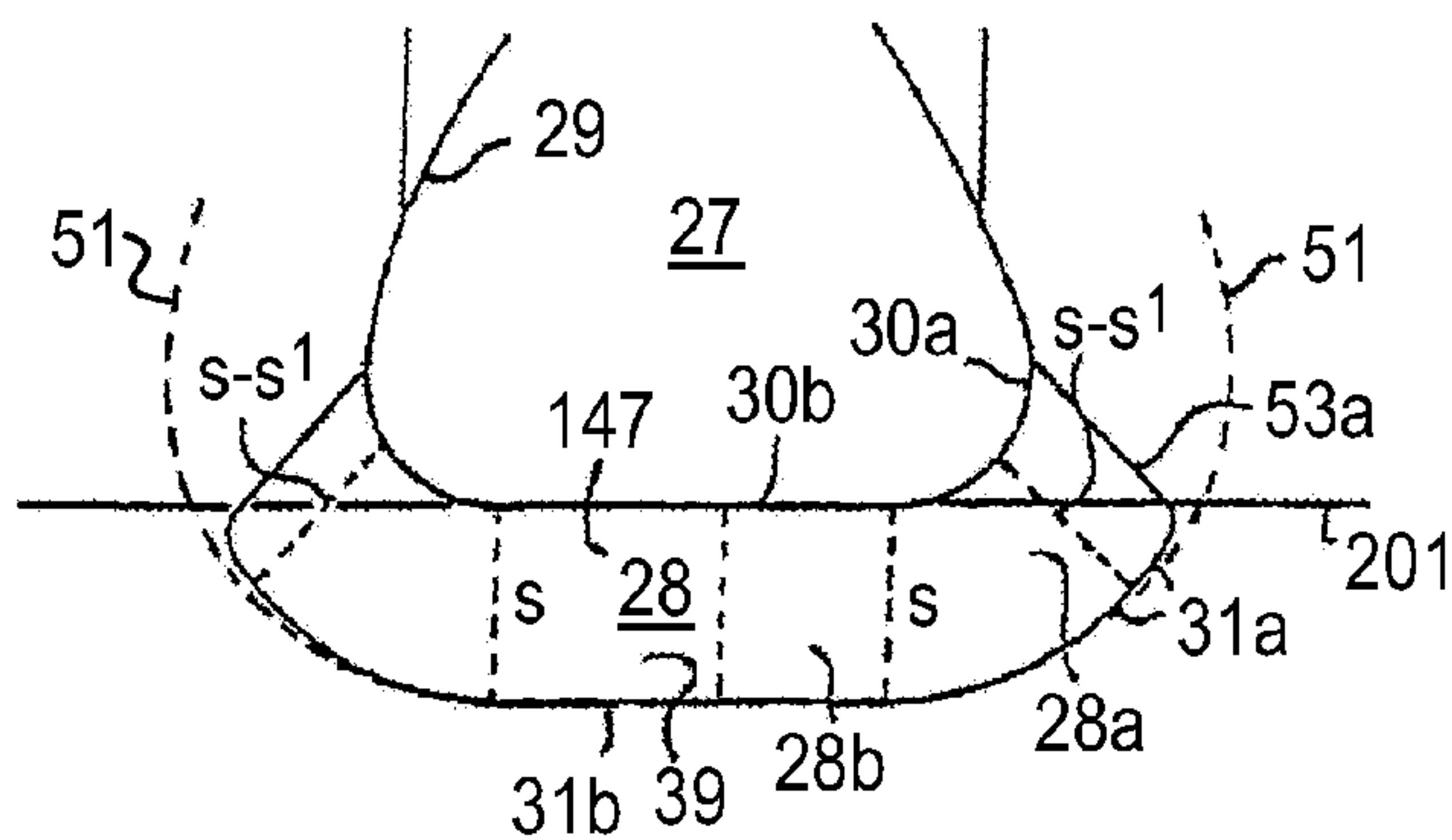
FIG. 27A PRIOR ART
