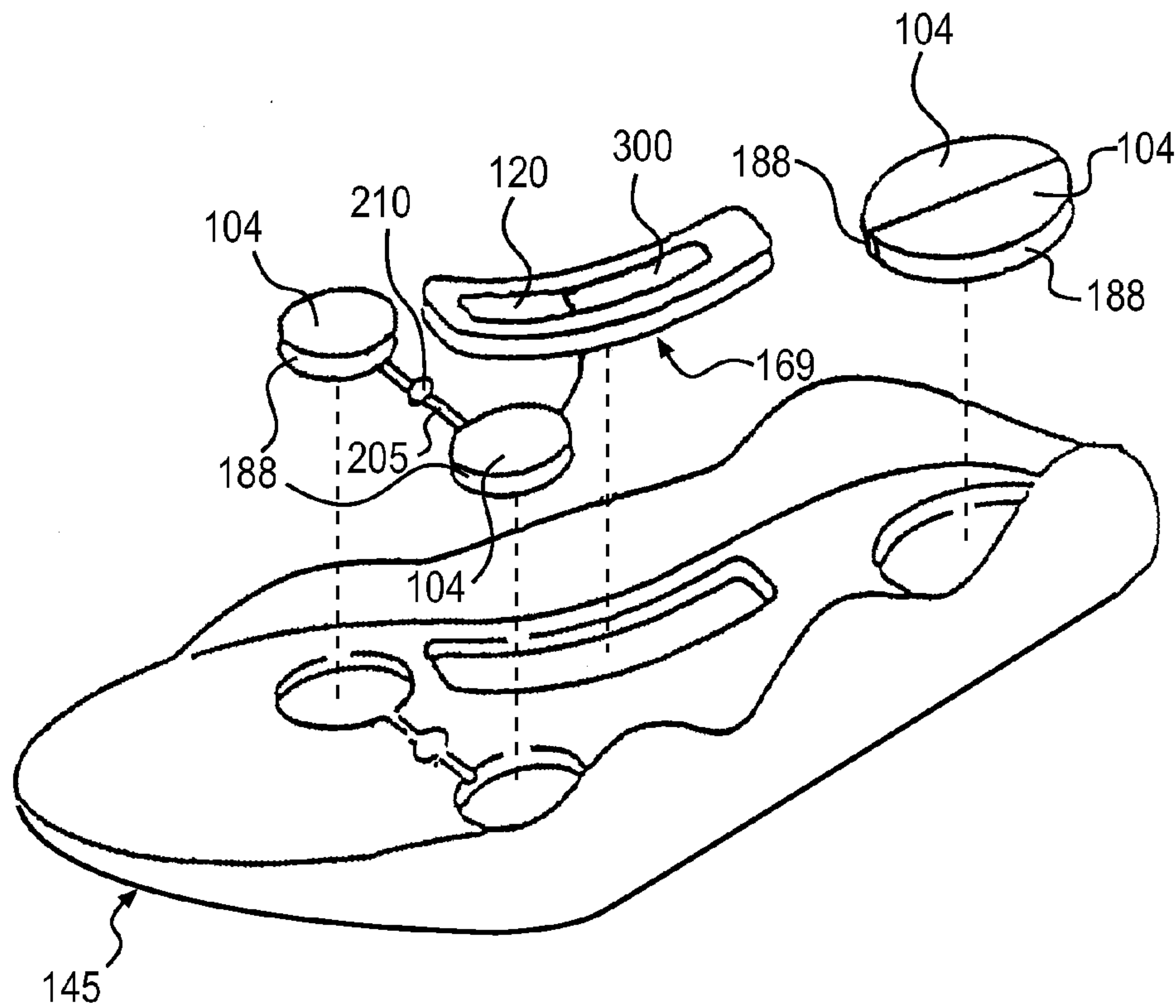
FIG. 11P PRIOR ART
