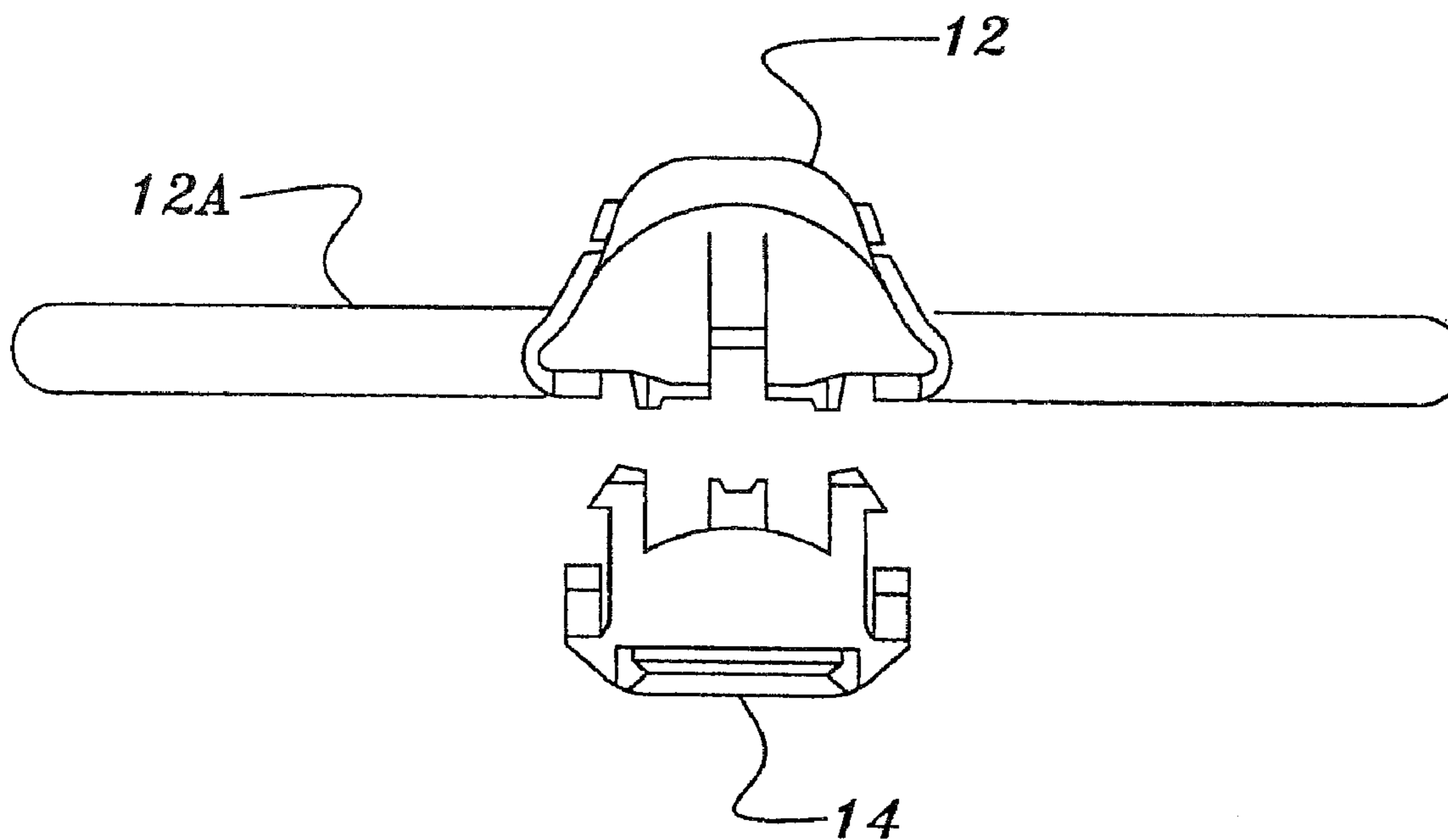
FIG. 6 BOTTOM EXPLODED
