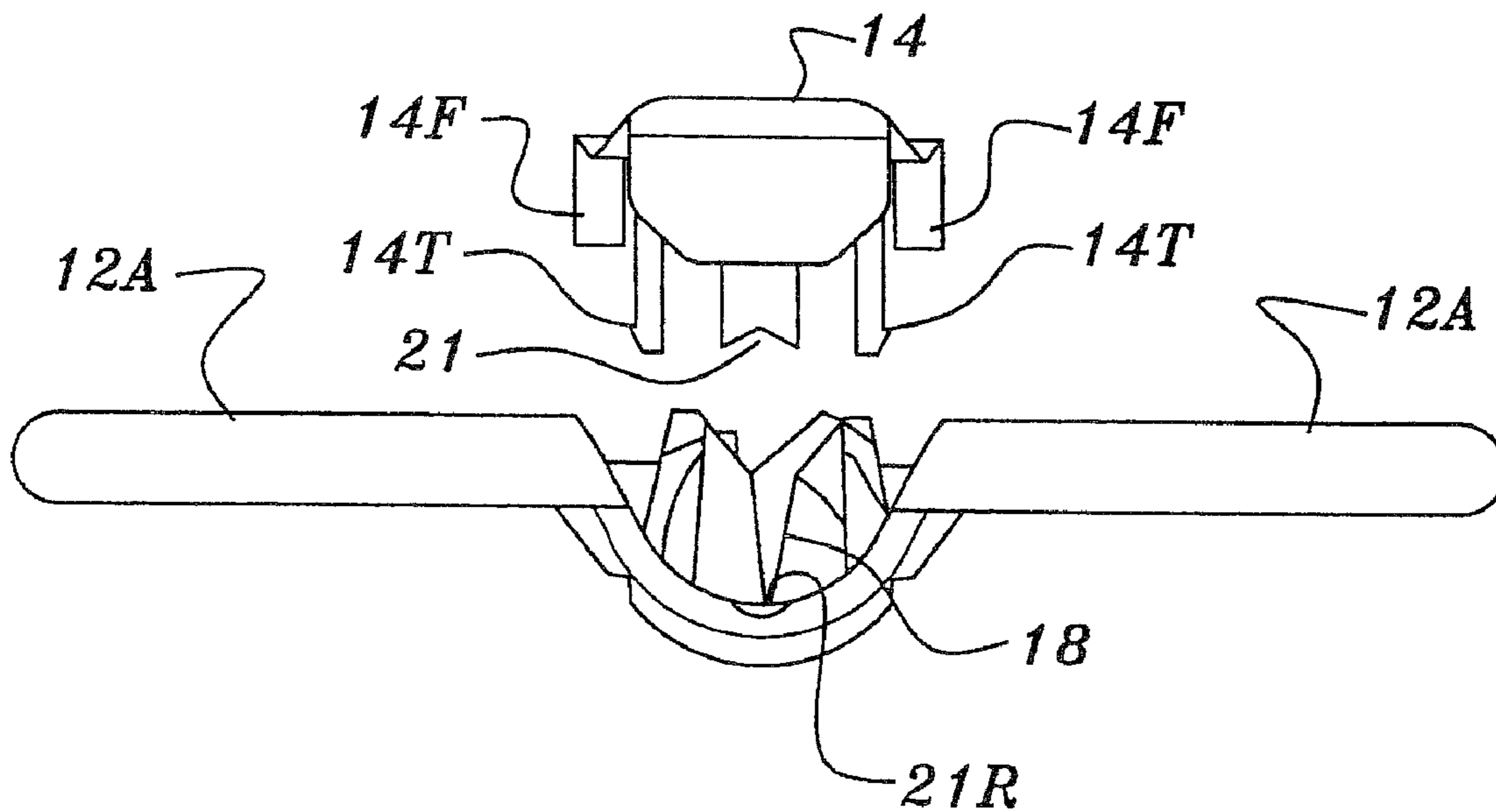
FIG. 5 TOP EXPLODED
