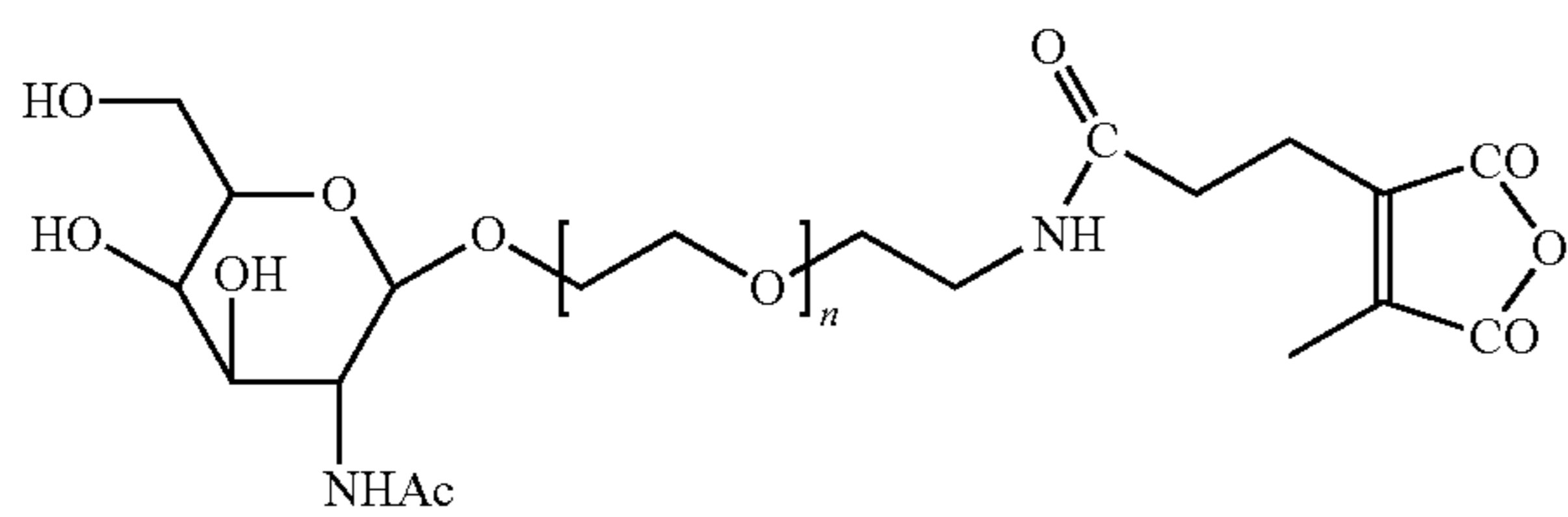
N-Acetyl-galactosamine-PEG-methyl maleic anhydride
