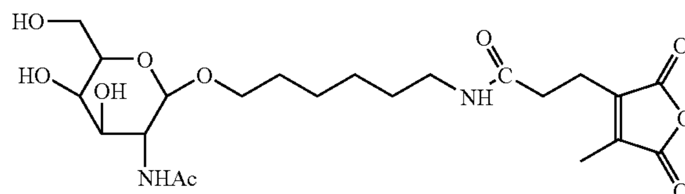
N-Acetyl-galactosamine-C 6 -methyl maleic anhydride masking agent
