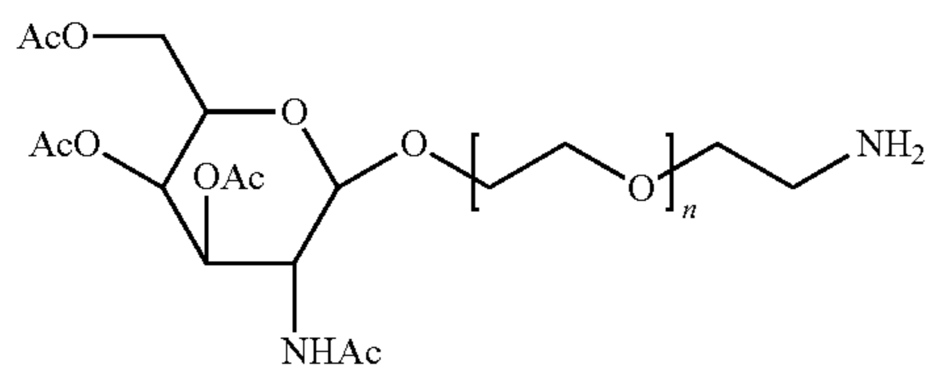
(Aminoethoxy)ethyl derivatives of 2-acetamido-3,4,6-tri-O-acetyl-2-deoxy-β-D-galactopyranoside
