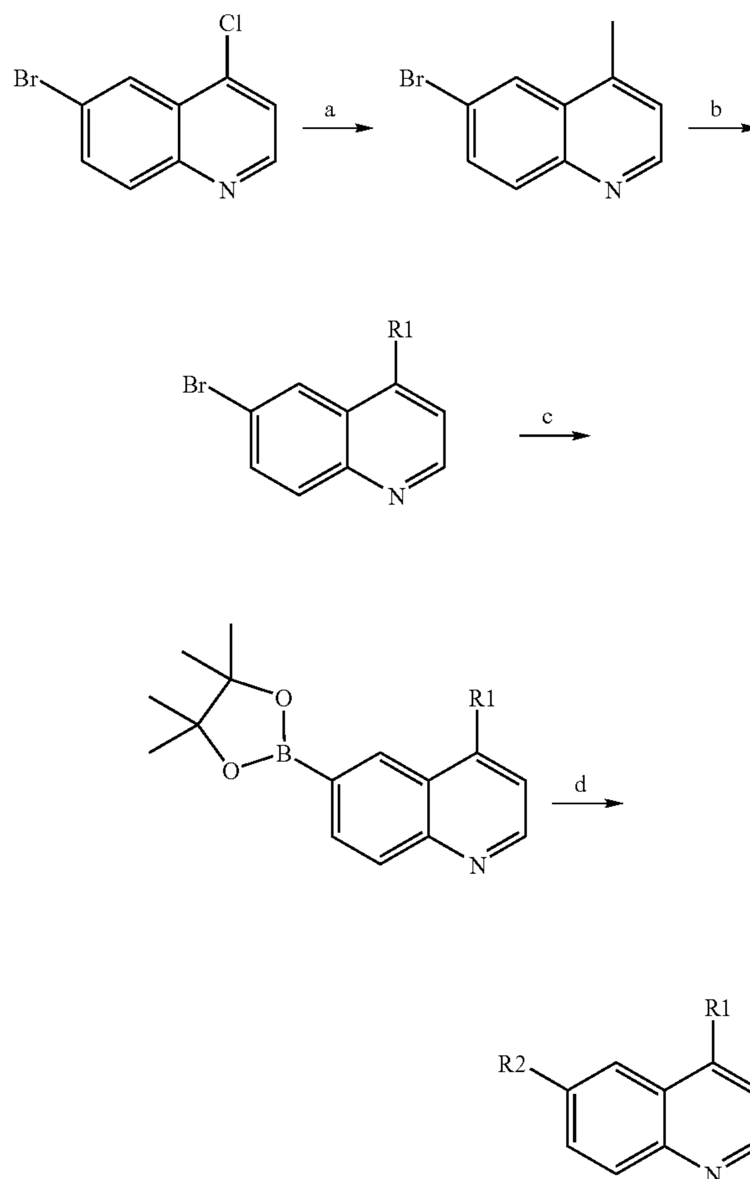
Scheme 1:
