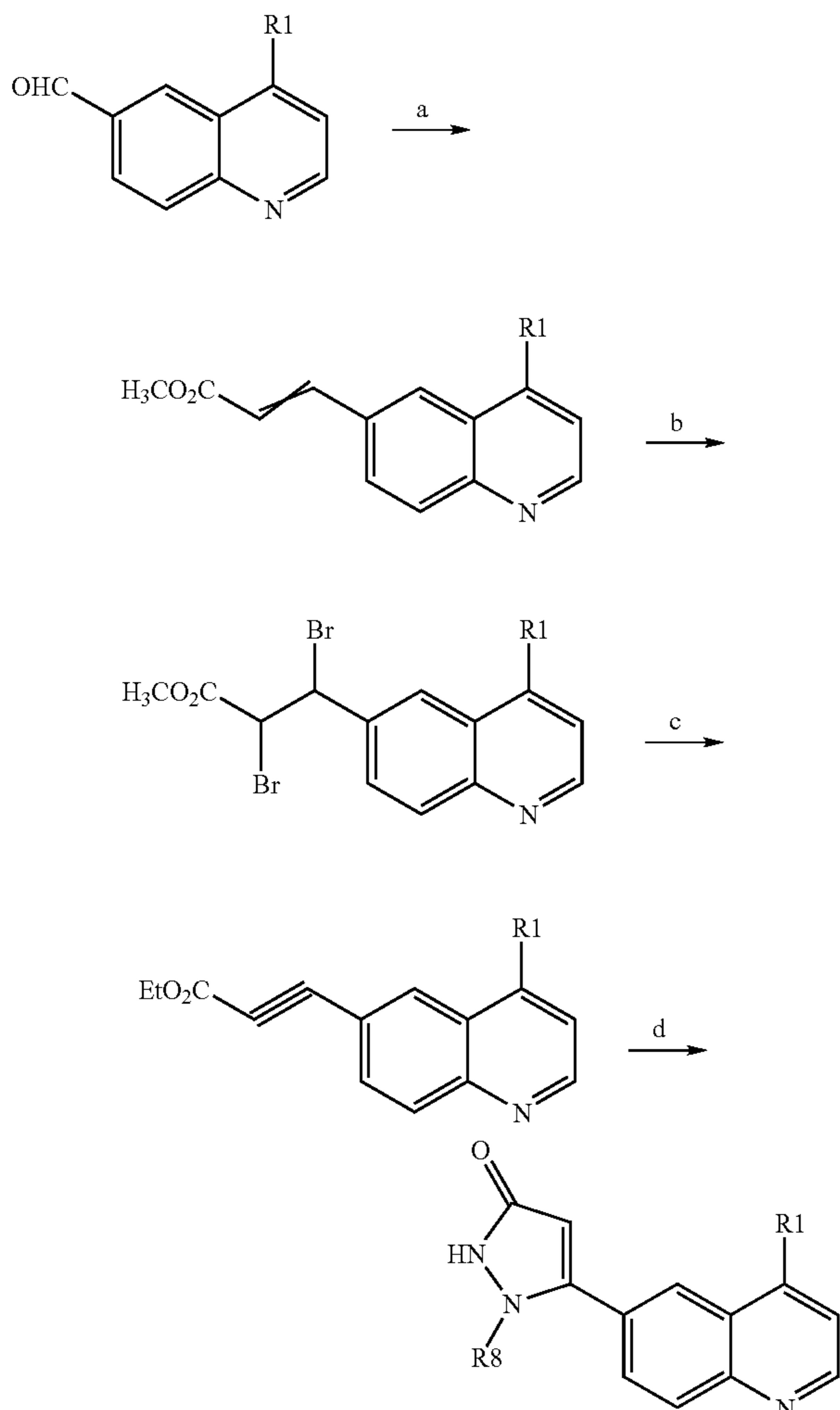
Scheme 15:
