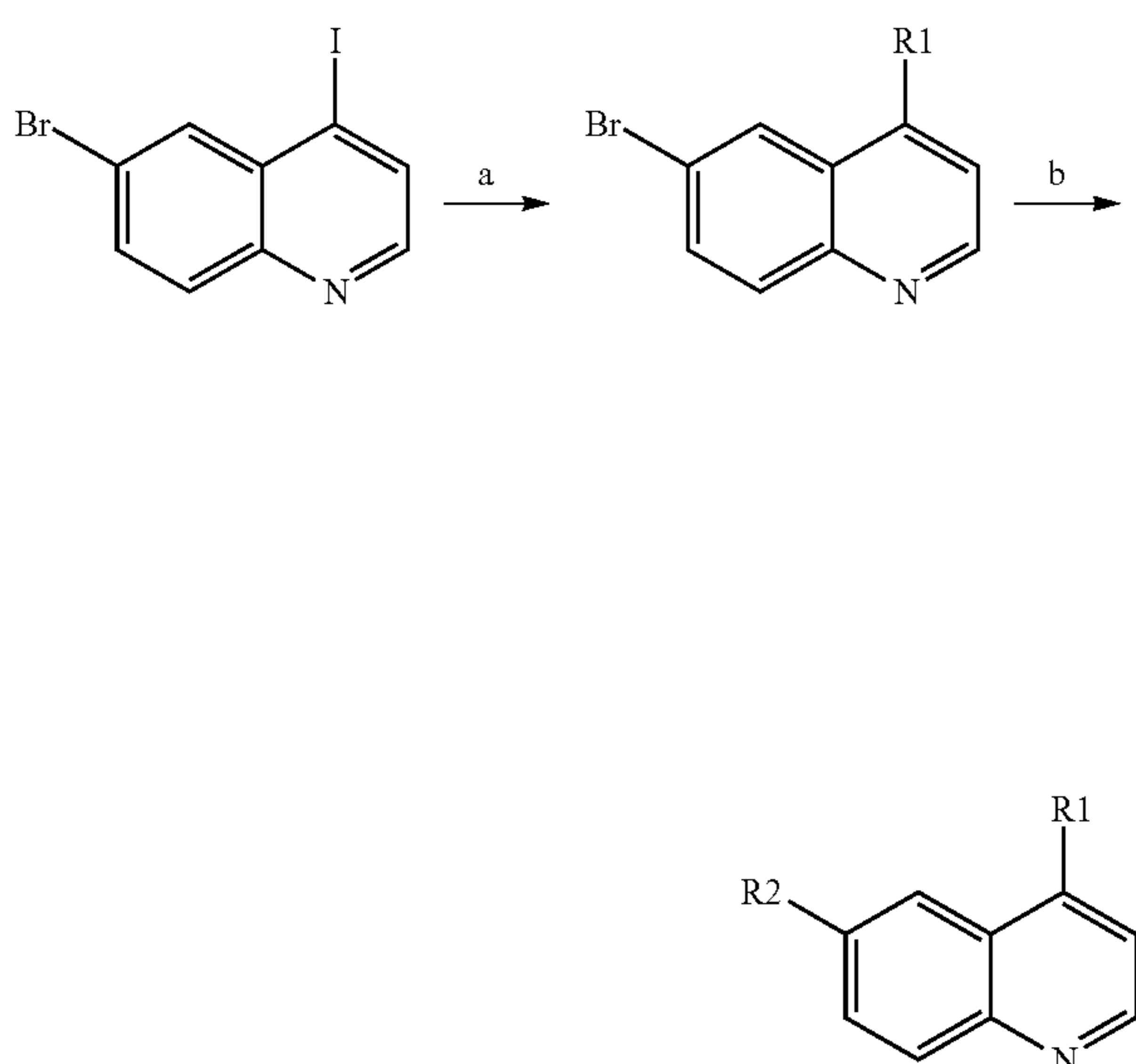
Scheme 4:
