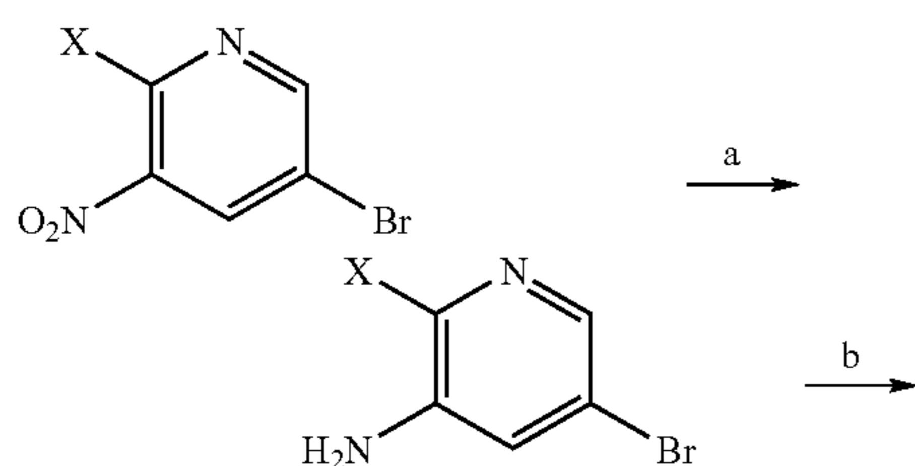
Scheme 14:
