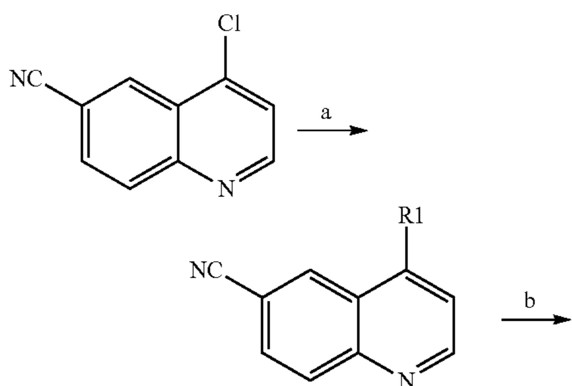
Scheme 9:
