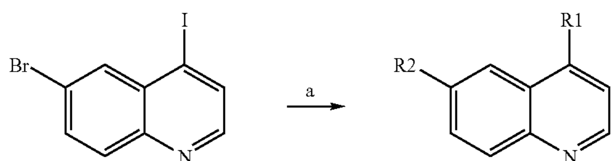
Scheme 3:
