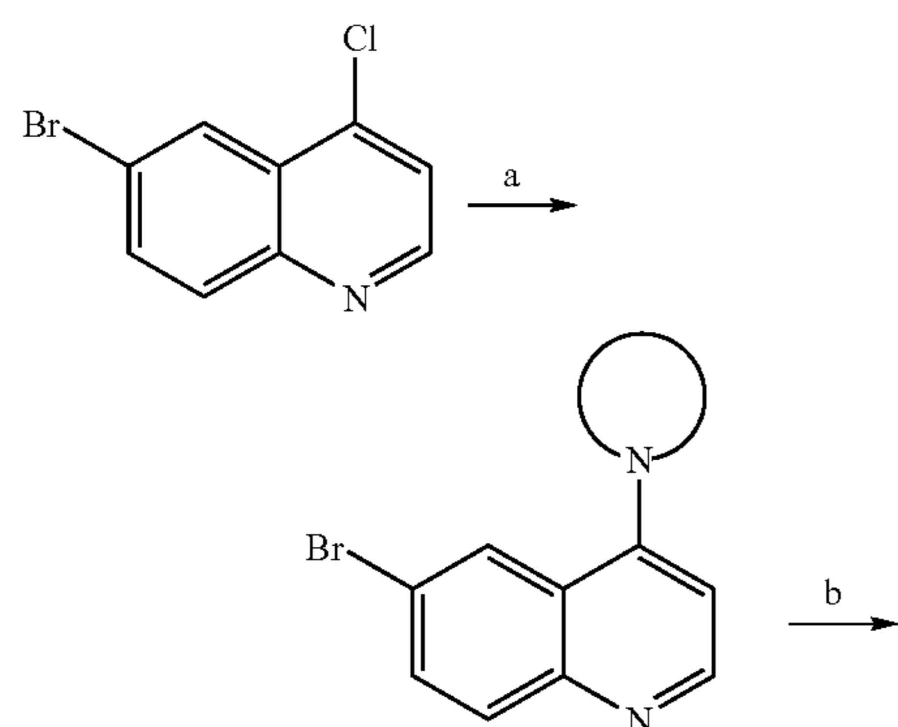
Scheme 10:
