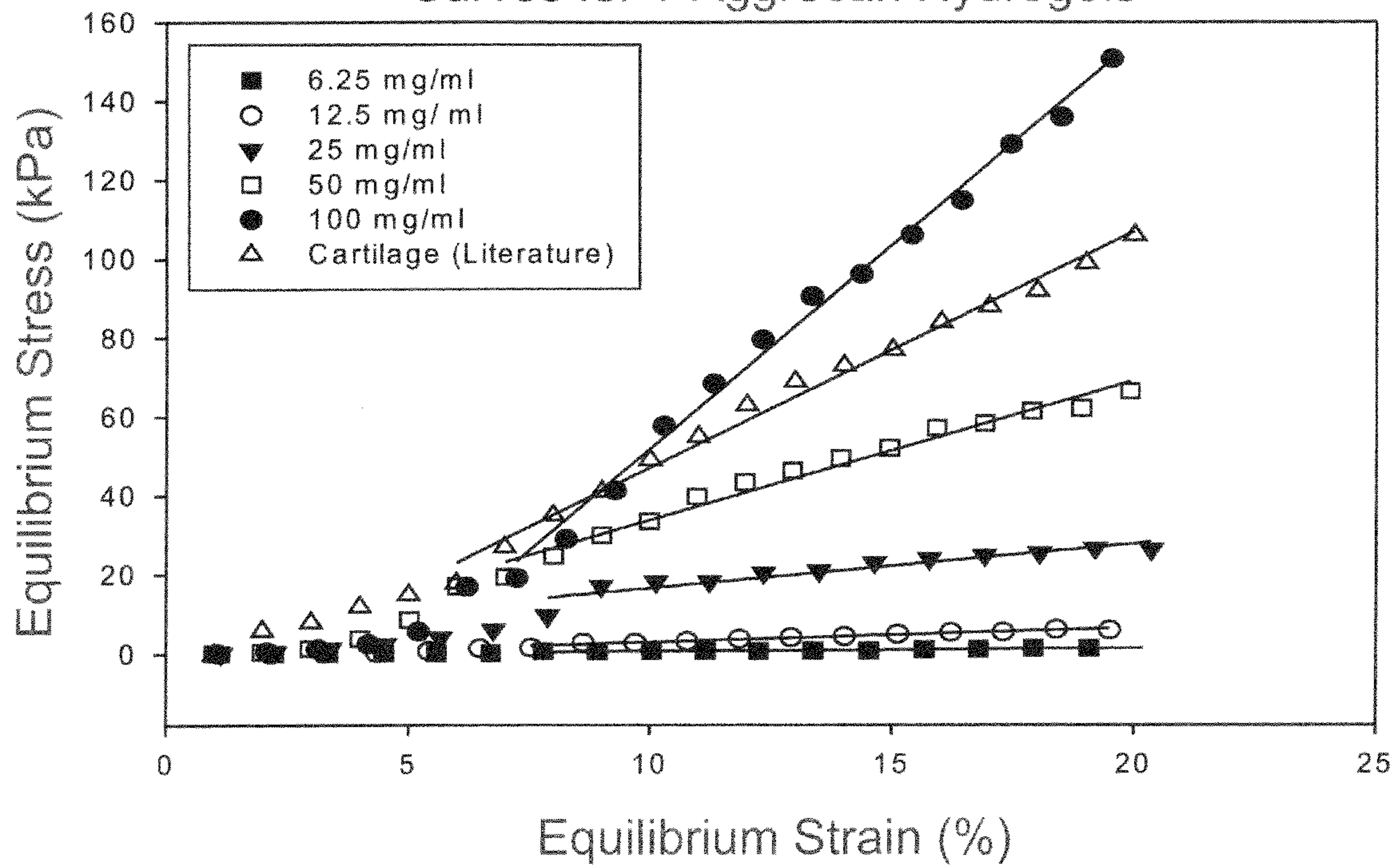
Fig. 4b Equilibrium Stress Versus Equilibrium Strain Curves for T-Aggregan Hydrogels
