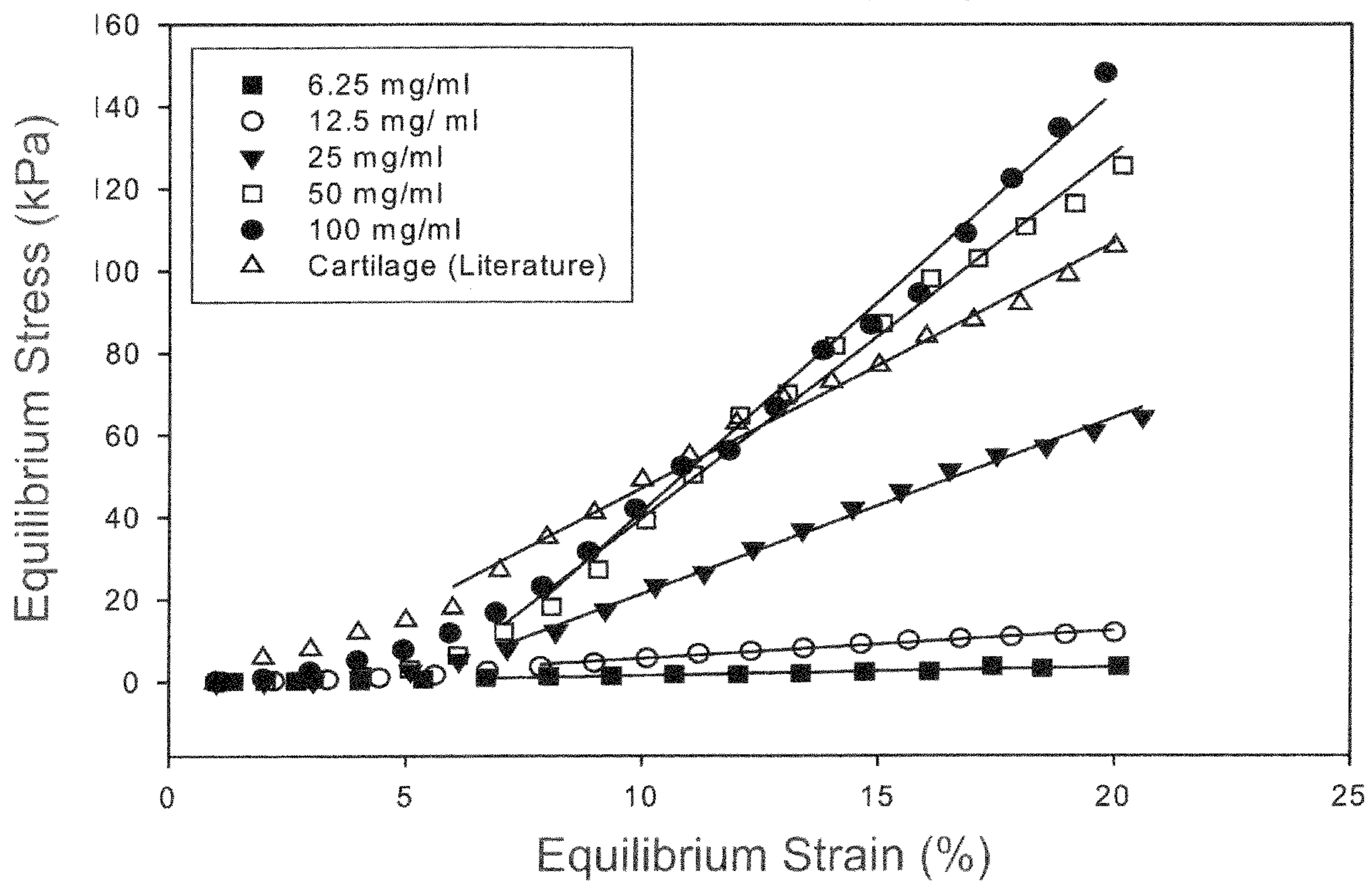
Fig. 4a Equilibrium Stress Versus Equilibrium Strain Curves for T-HA Hydrogels
