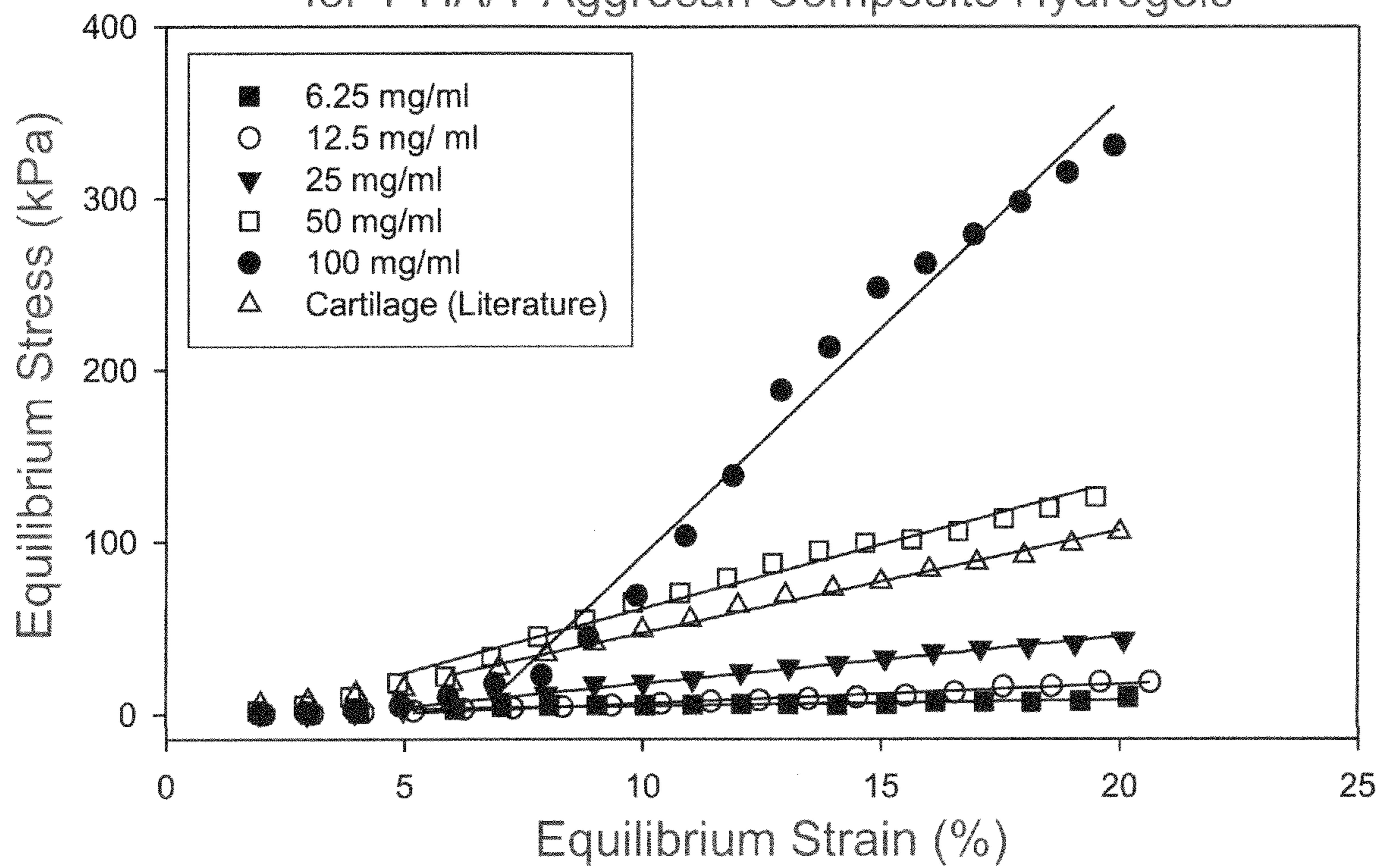
Fig. 4c Equilibrium Stress Versus Equilibrium Strain Curves for T-HA/T-Aggregan Composite Hydrogels
