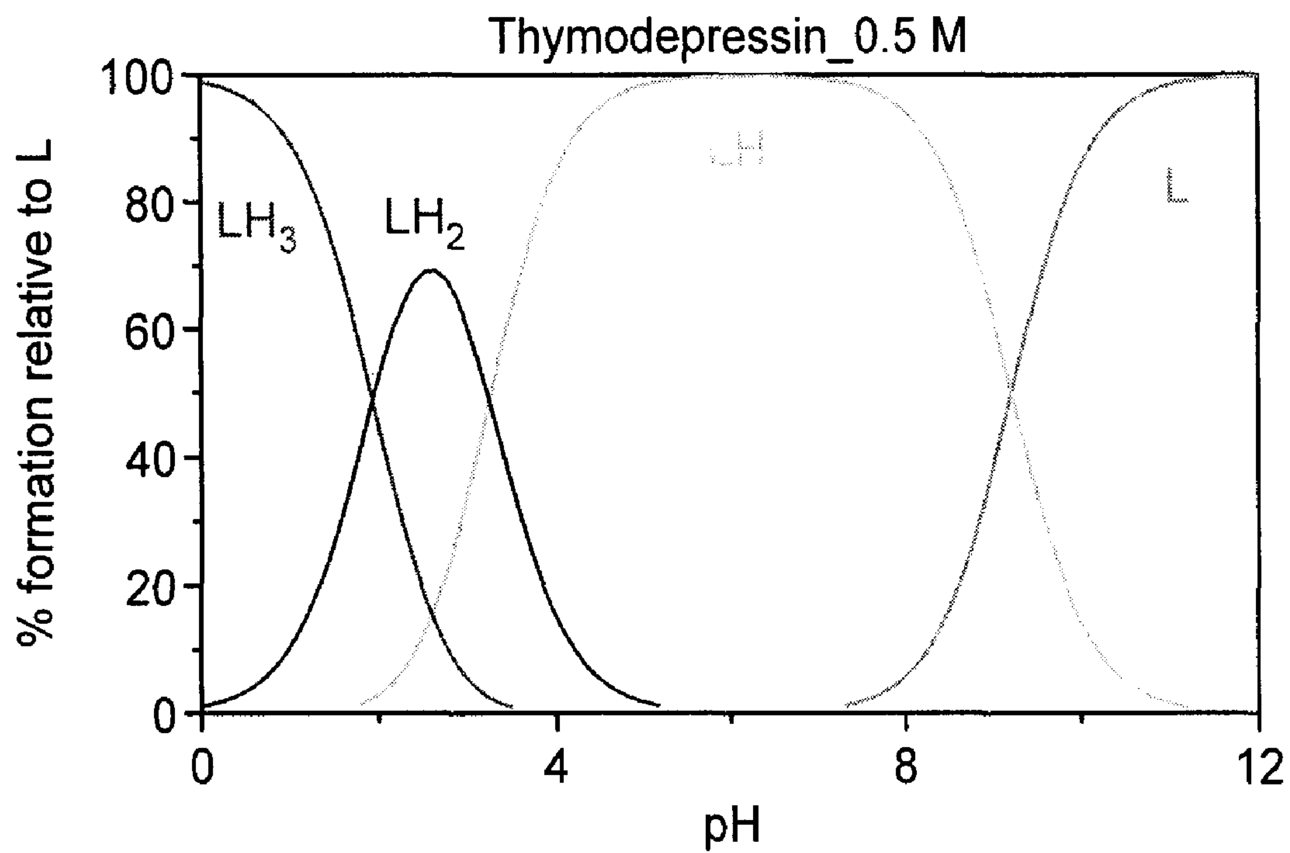
Fig. 5: Speciation plot of H-D-iGlu-D-Trp-OH from pH 0 to 12
