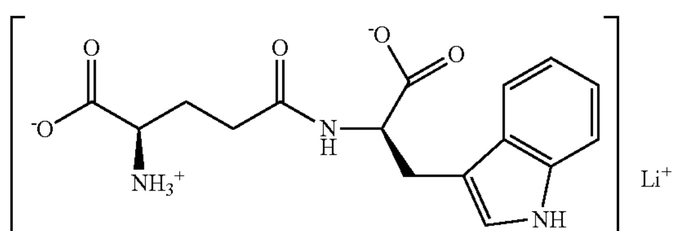
Lithium salt of Formula I
