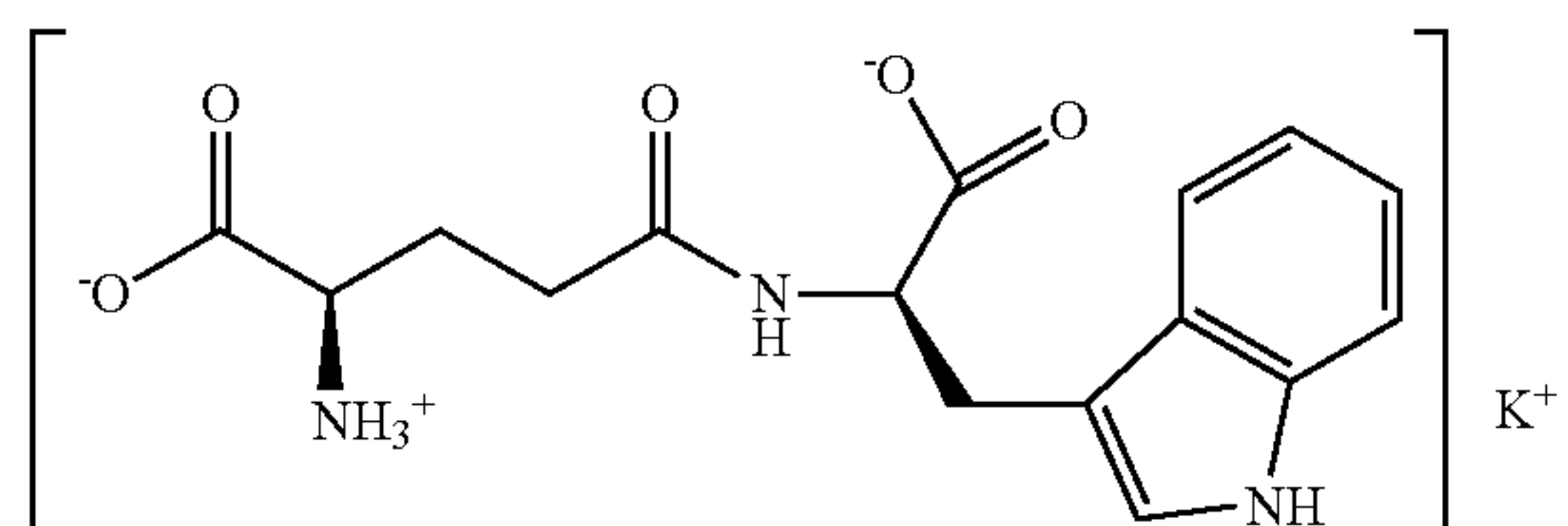
Potassium salt of Formula I
