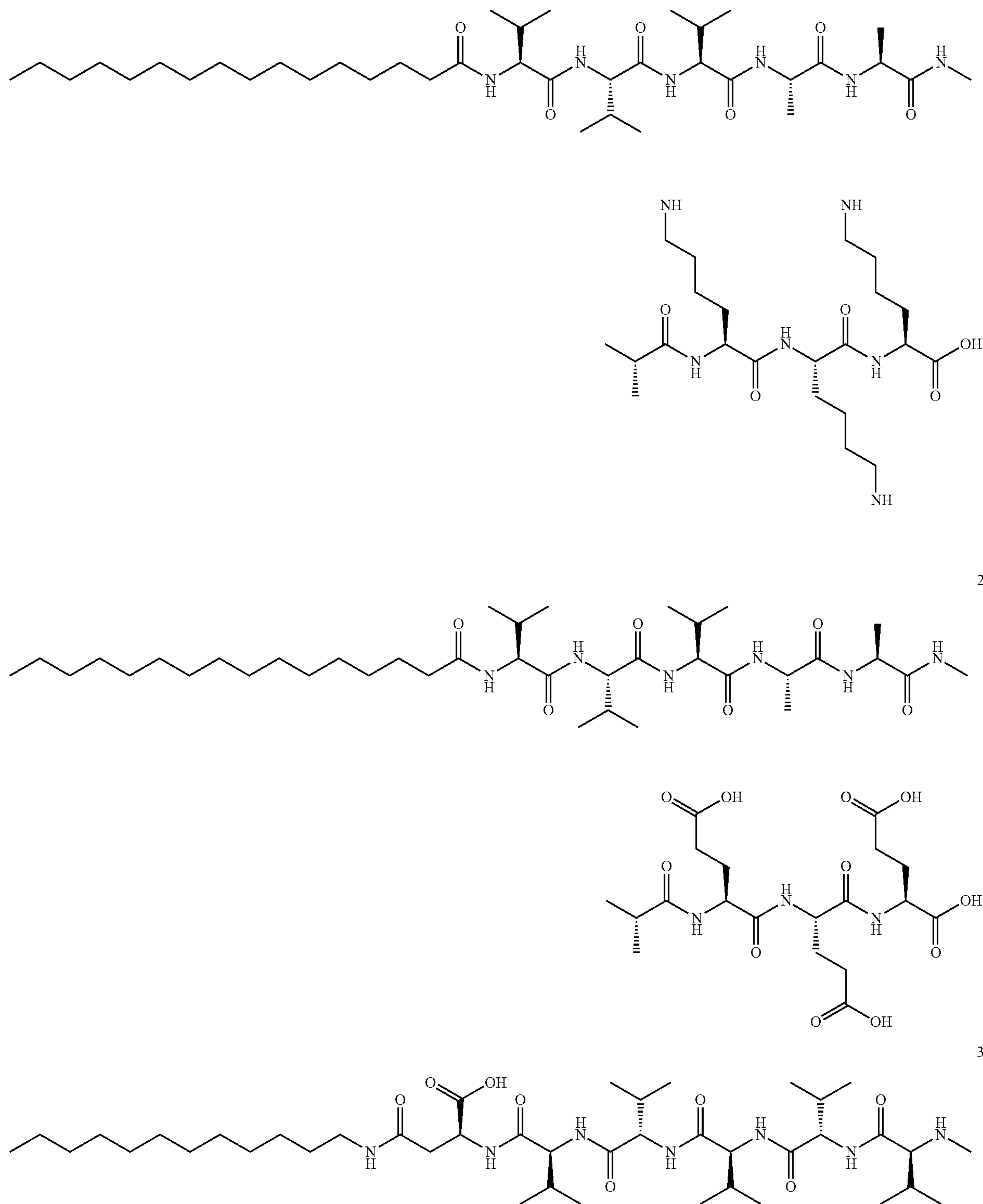
Scheme 1. Chemical structures of peptide amphiphiles
