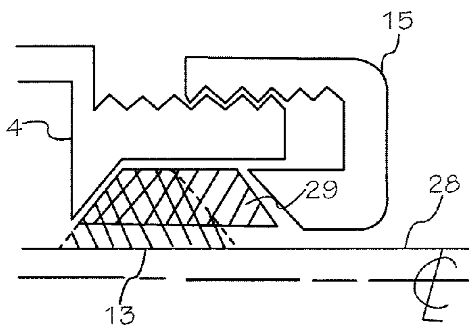
FIG 5C
