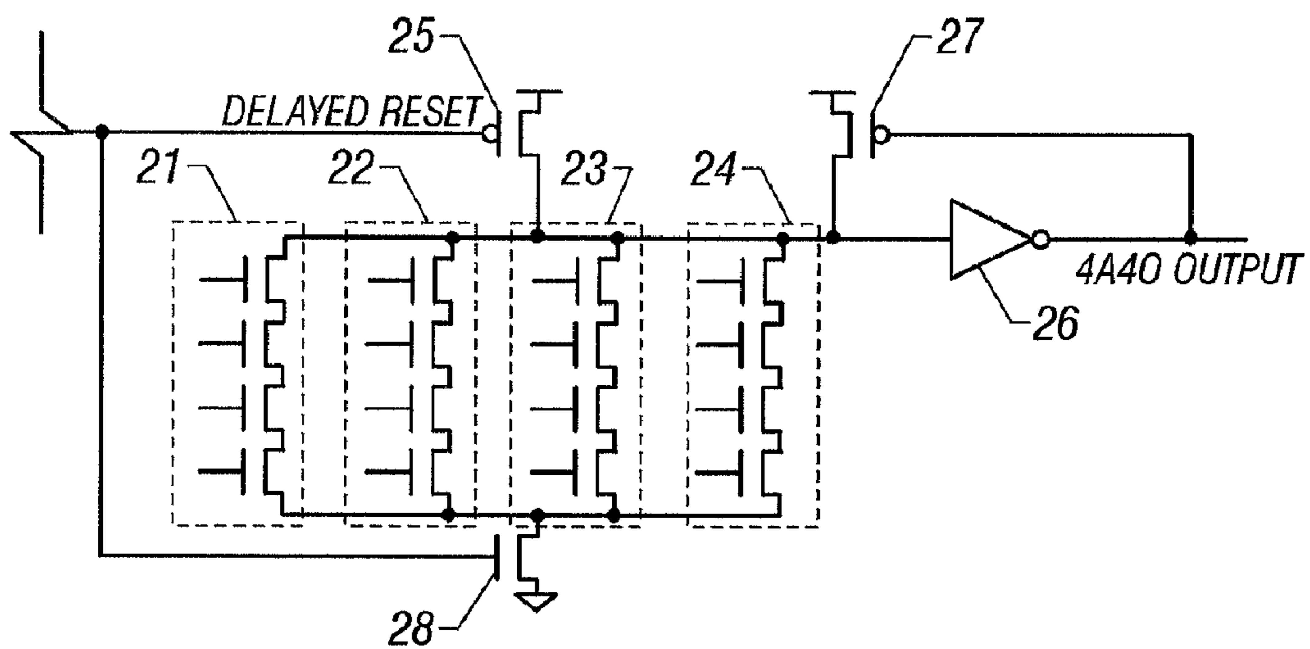
FIG. 3 (Prior Art)
