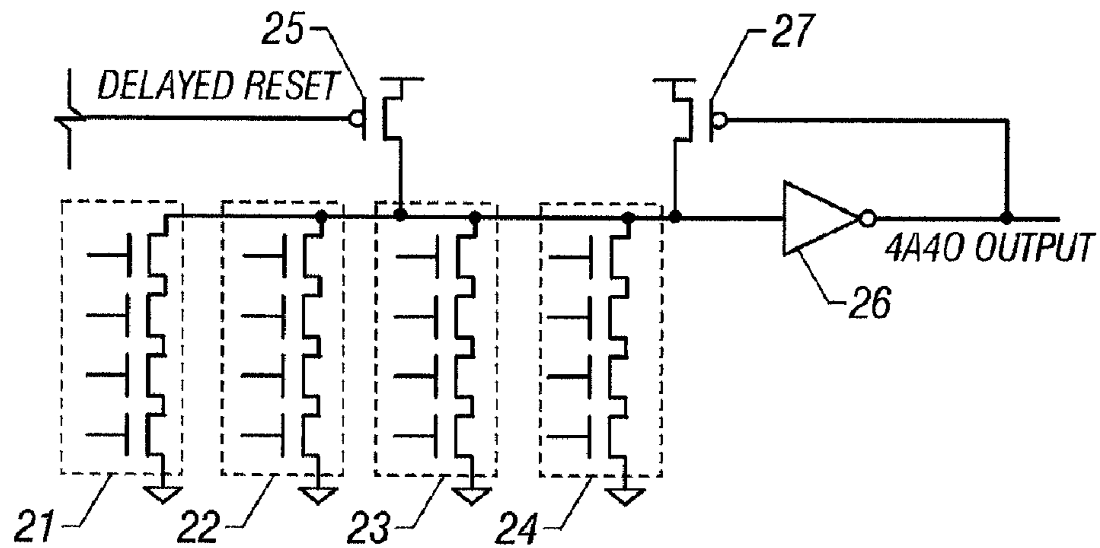
FIG. 2 (Prior Art)
