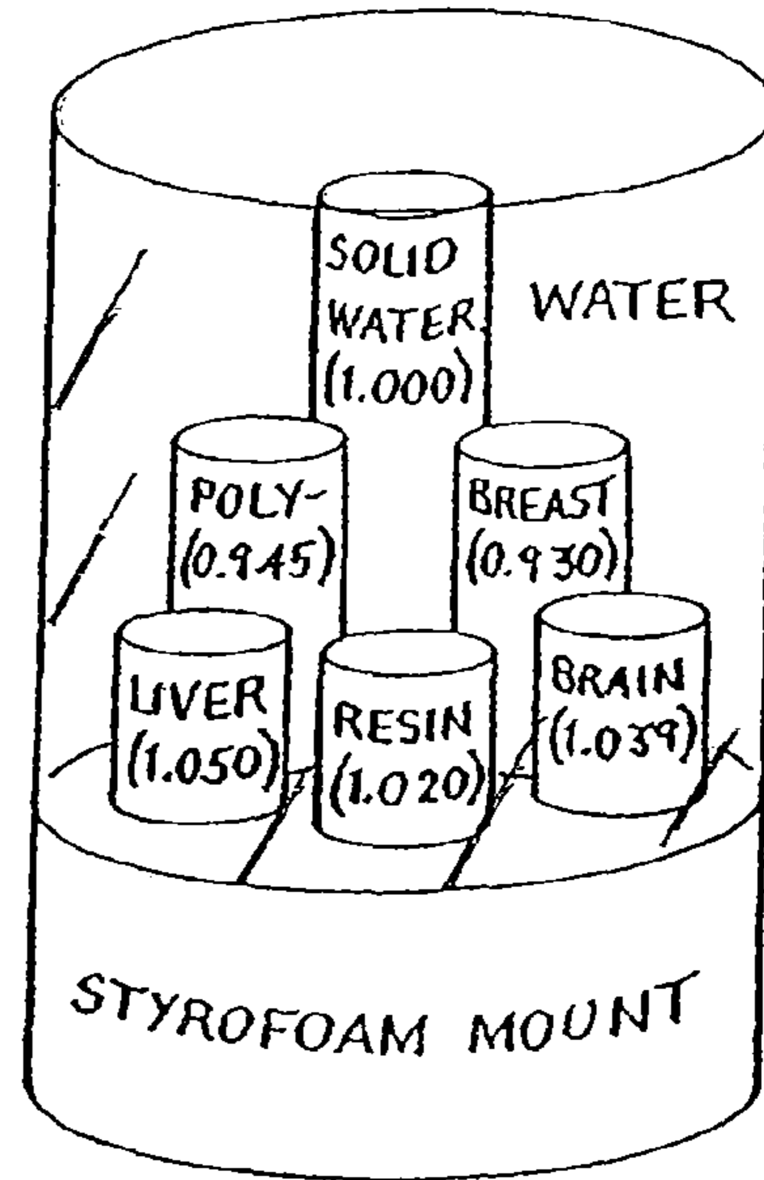
ELECTRON DENSITY PHANTHOM (CONTRAST, CT LINEARITY)
